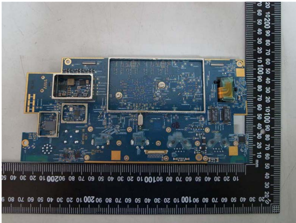
Figure 3 – PCB 1 RF CIRCUITRY (un-Shielded)
