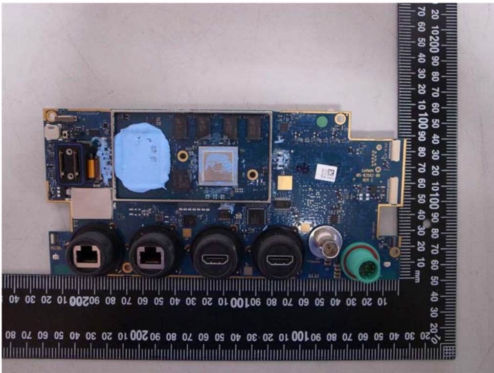
Figure 5 - PCB 3
