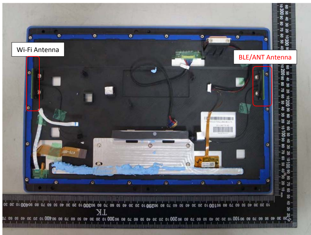
Figure 1 - ANTENNA LOCATION
