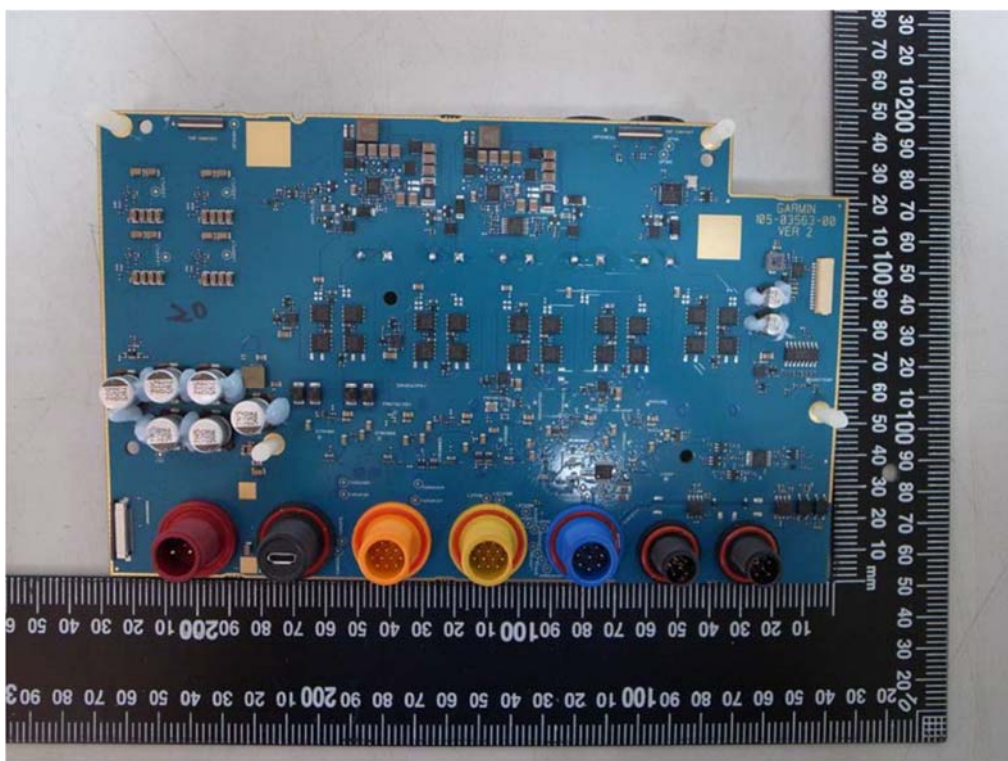
Figure 4 PCB 2
