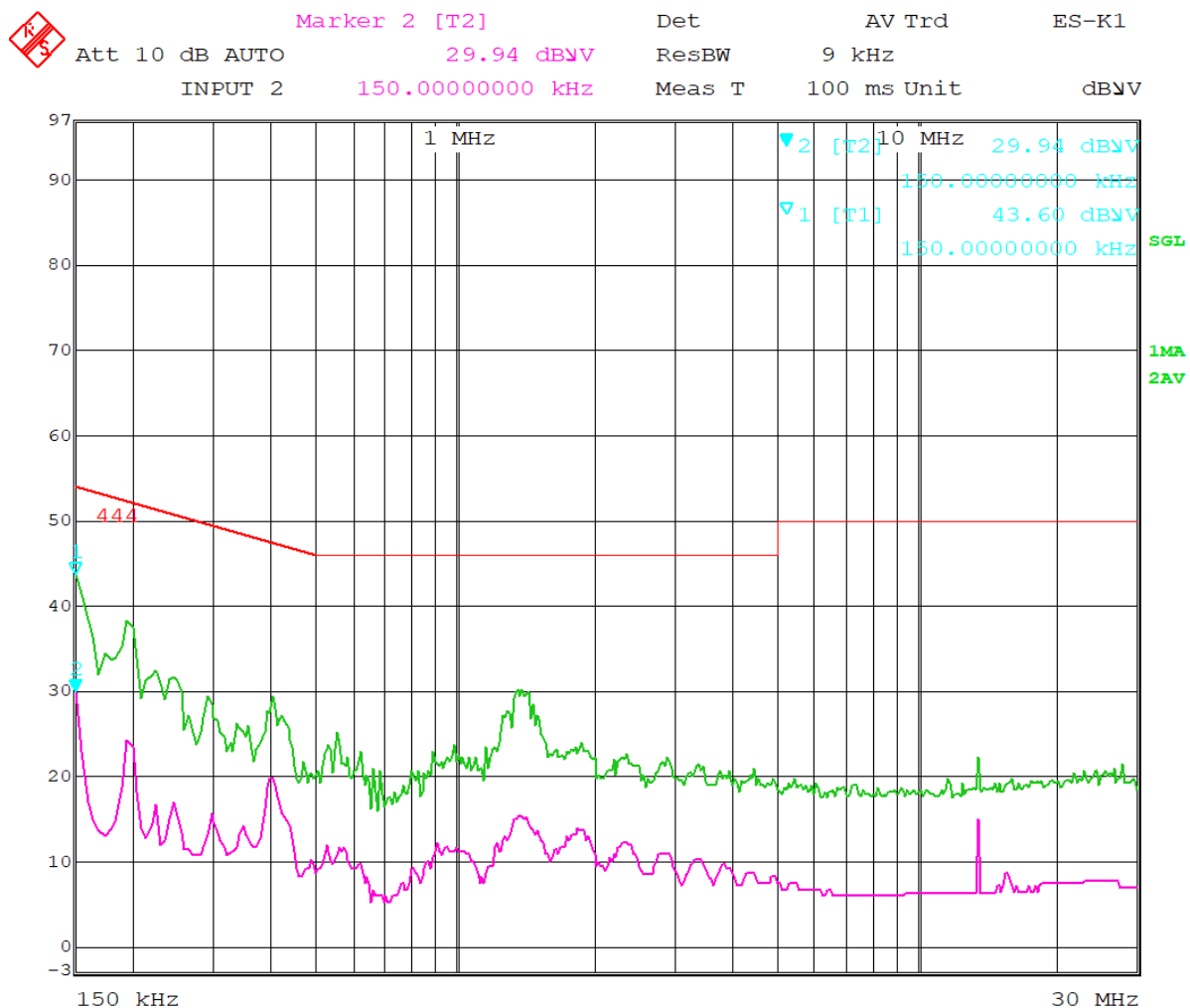
Figure 9 - Conducted Emissions, Line All Measurements were found to be at least 10 dB below the limits.
