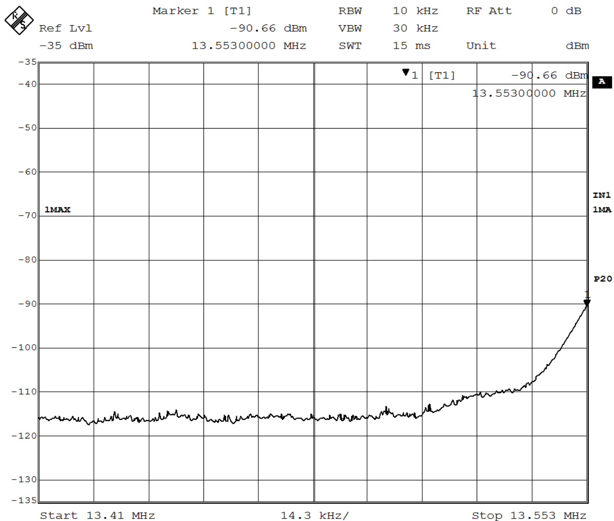
Figure 6 – Lower Bandedge
