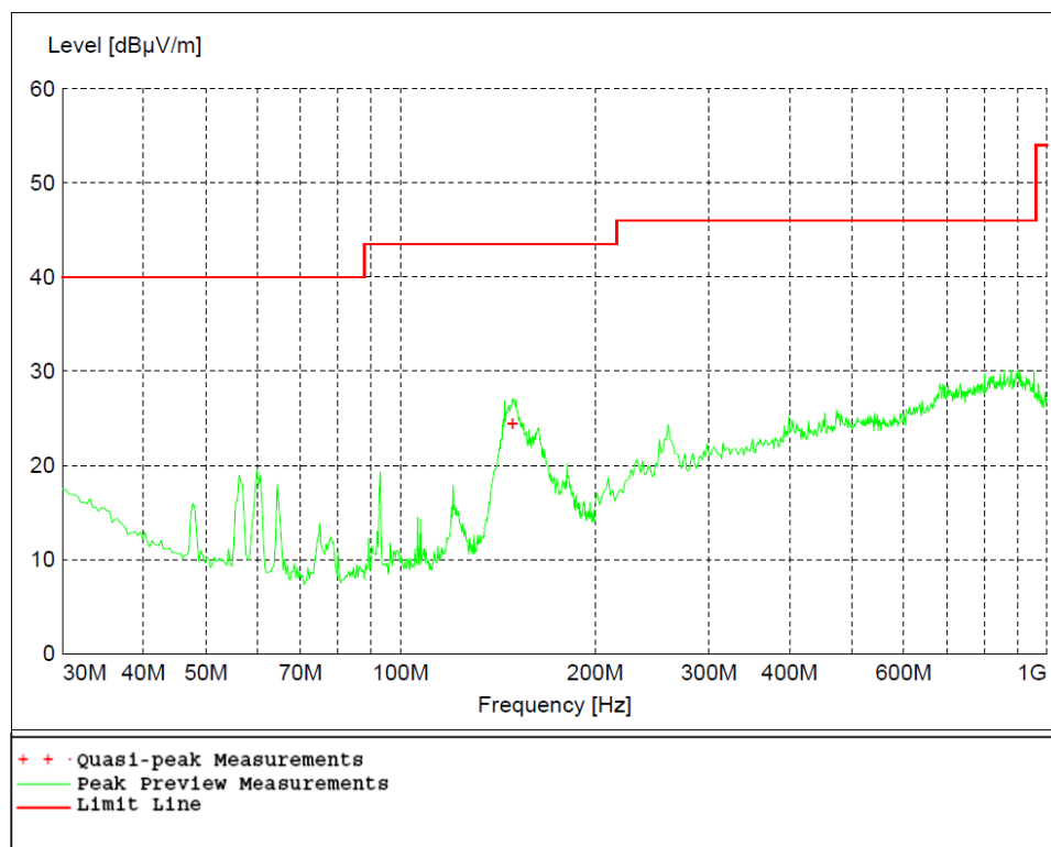
Figure 2 – Radiated Emissions Peak Plot, 30 MHz- 1 GHz
