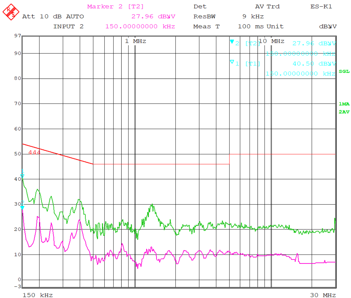
Figure 10 - Conducted Emissions, Neutral
