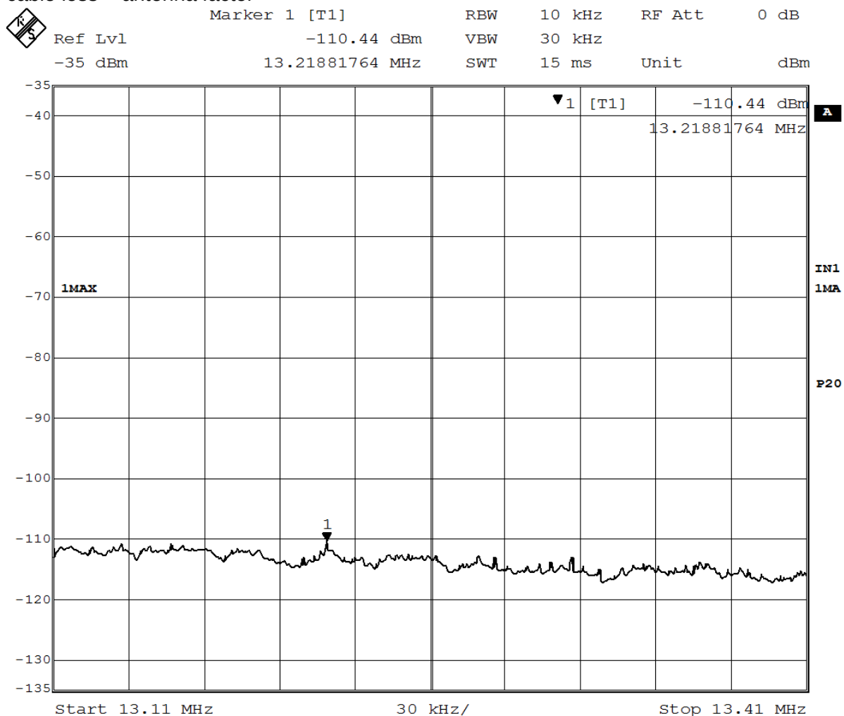
Figure 5 – Lower Bandedge
