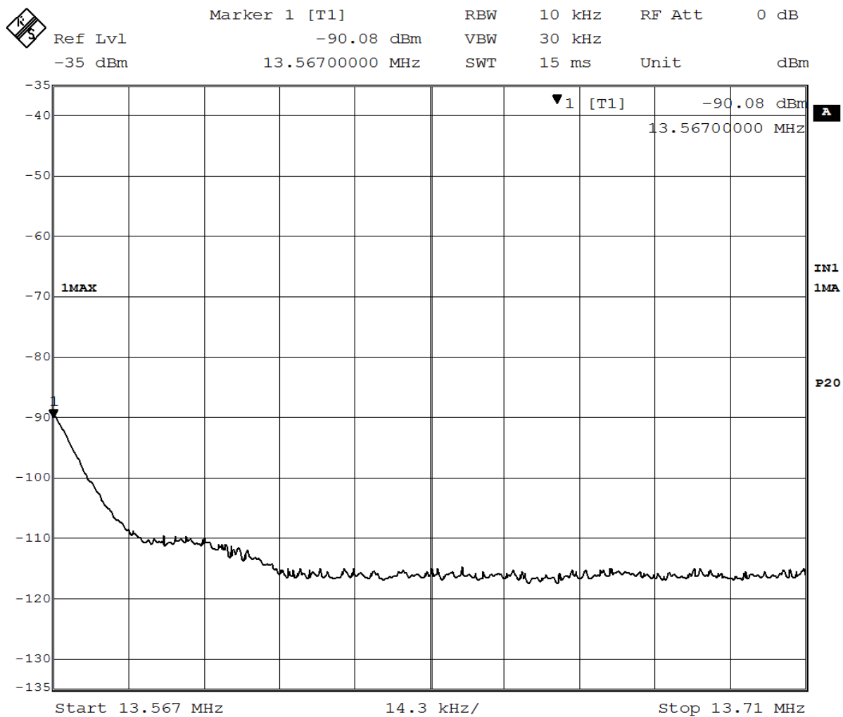
Figure 7 – Higher Band edge
