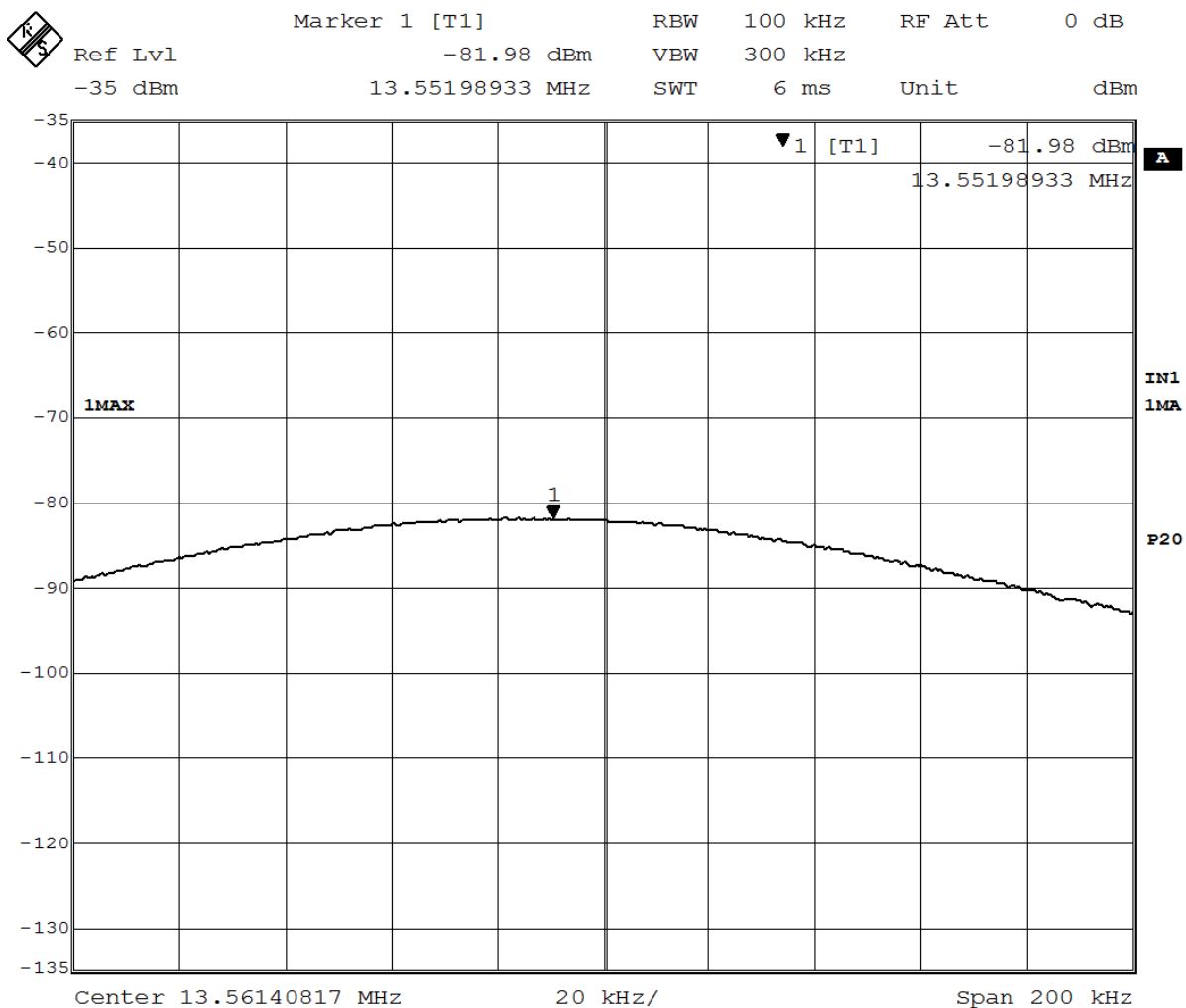
Figure 4 – Output Power
