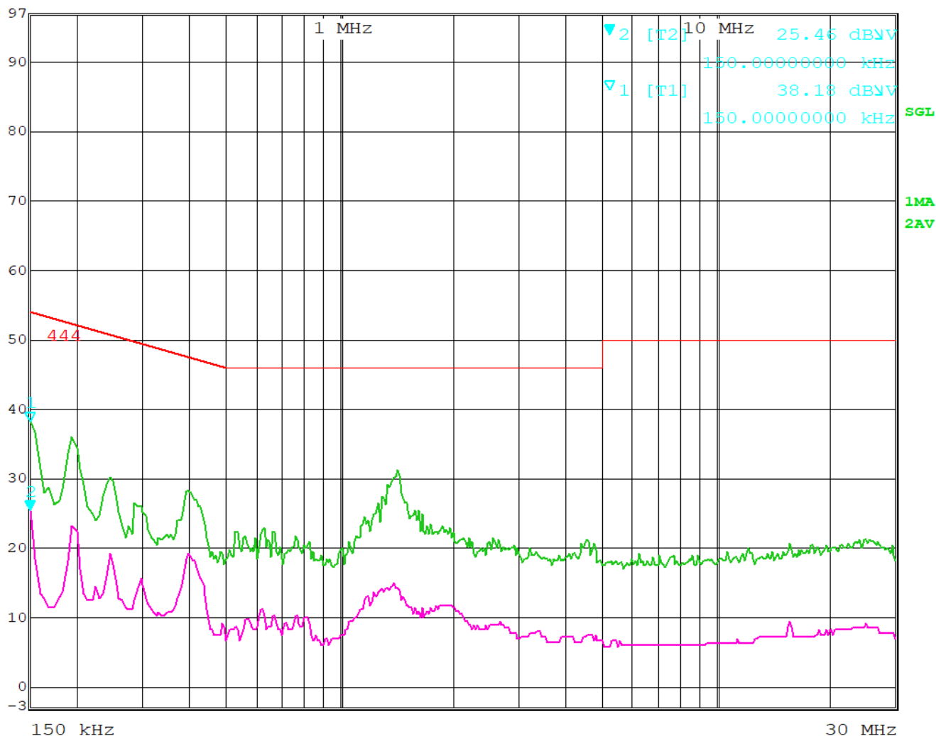
Figure 56 - Conducted Emissions Plot, Line
