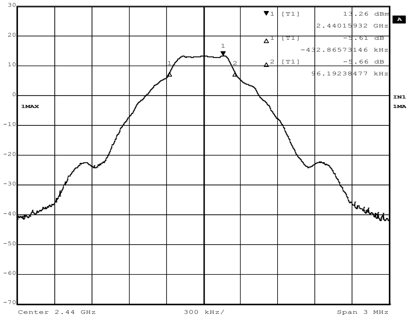
Figure 22 – 6dB Bandwidth, Mid Channel, BT BR (GFSK)
