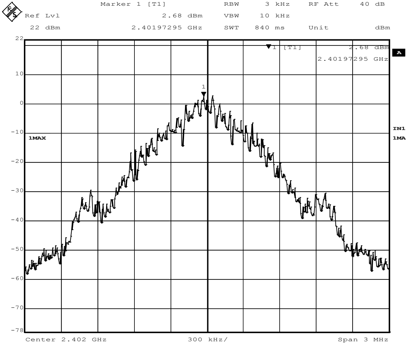
Figure 35 - Power Spectral Density, Low Channel, BT BR (GFSK)
