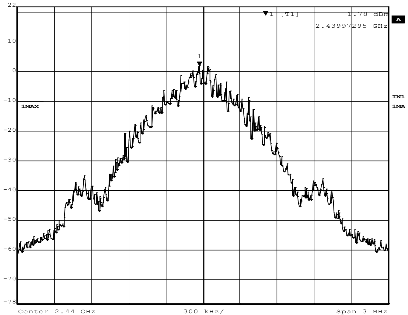
Figure 36 - Power Spectral Density, Mid Channel, BT BR (GFSK)
