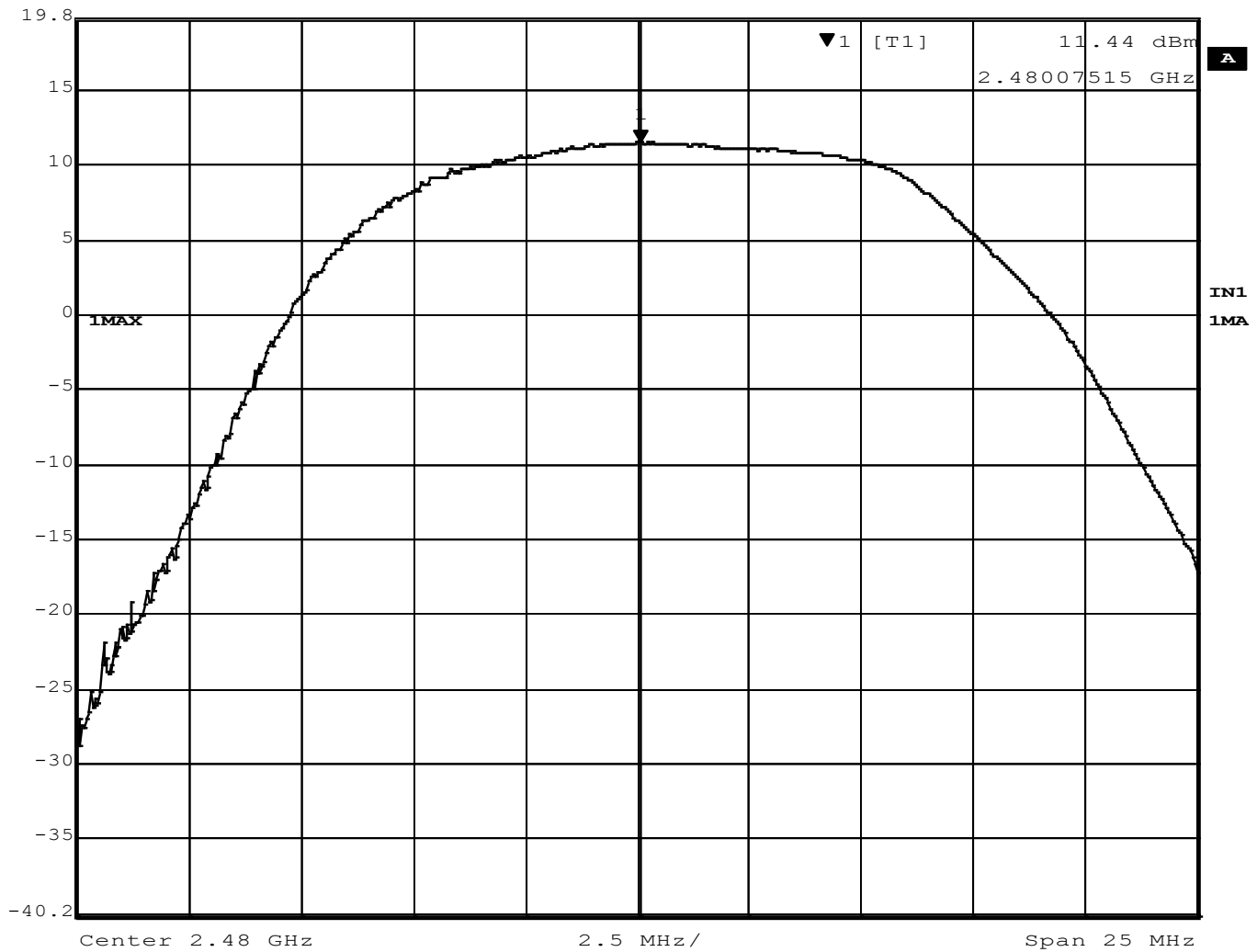
Figure 7 – Output Power, High Channel, BT EDR 2MB
