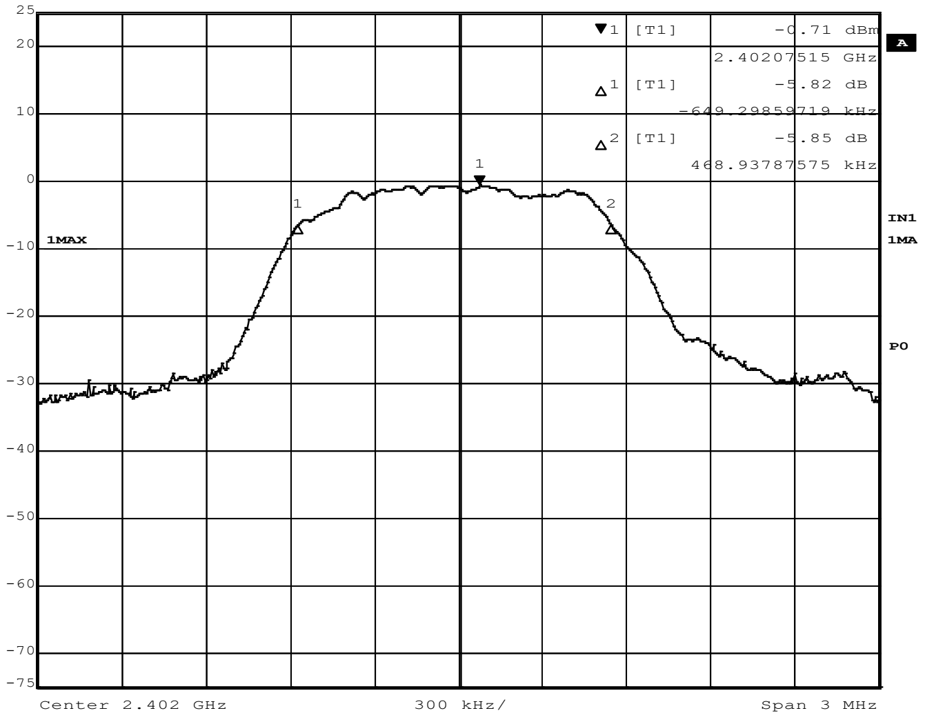
Figure 27 – 6dB Bandwidth, Low Channel, BT EDR 3MB
