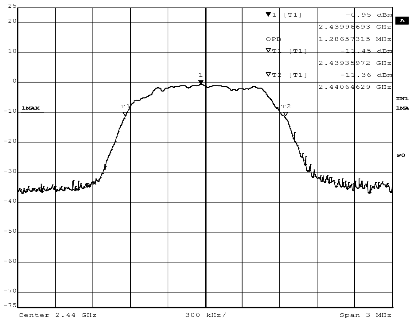
Figure 19 - Occupied Bandwidth, Mid Channel, BT EDR 3MB
