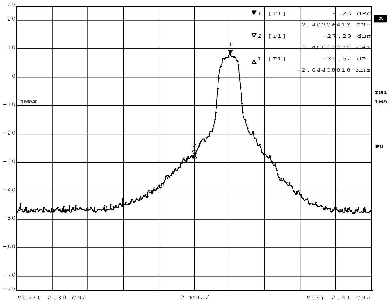
Figure 49 - Band-edge Measurement, Low Channel, Fundamental, Peak
