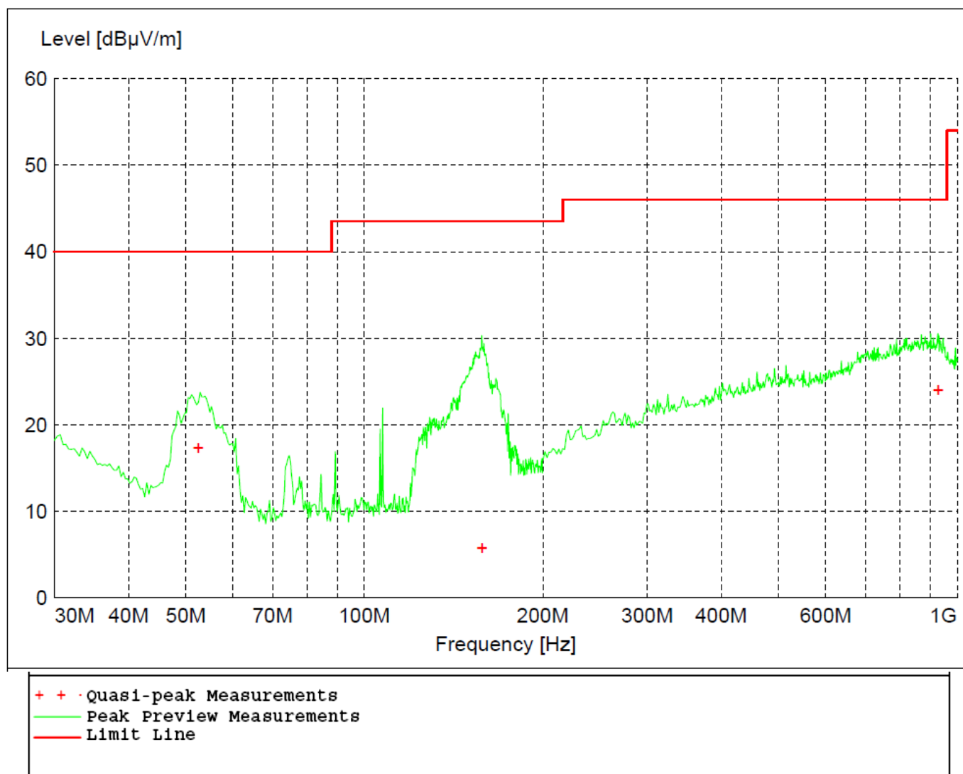
Figure 34 - Radiated Emissions Plot, BT EDR 3MB
