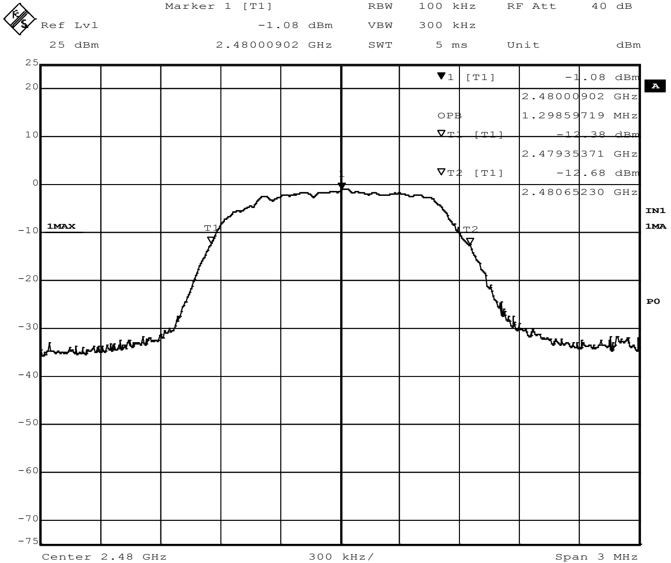
Figure 20 - Occupied Bandwidth, High Channel, BT EDR 3MB
