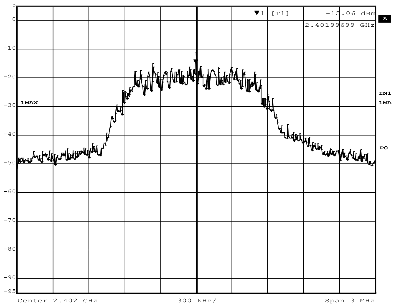
Figure 38 - Power Spectral Density, Low Channel, BT EDR 2MB
