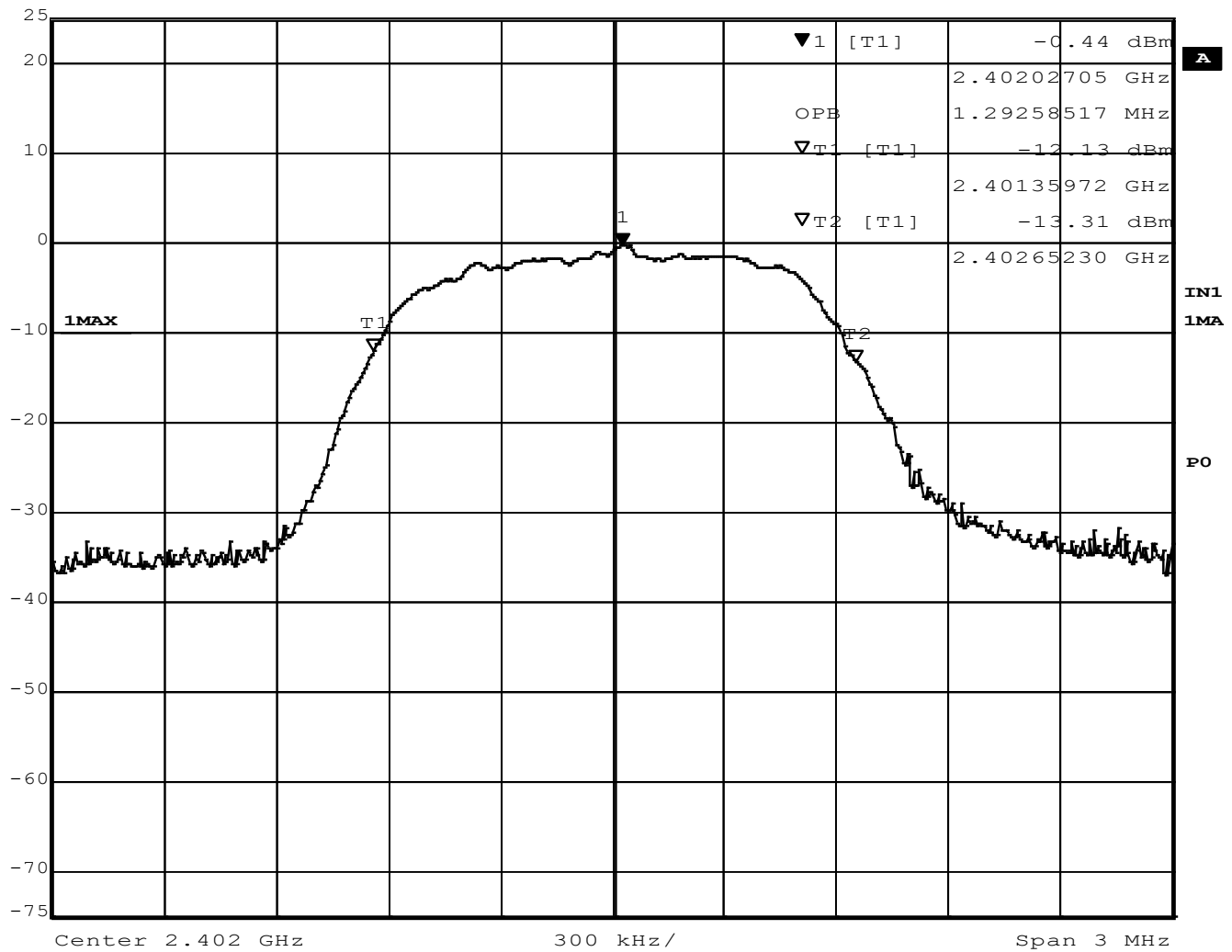
Figure 15 – Occupied Bandwidth, Low Channel, BT EDR 2MB
