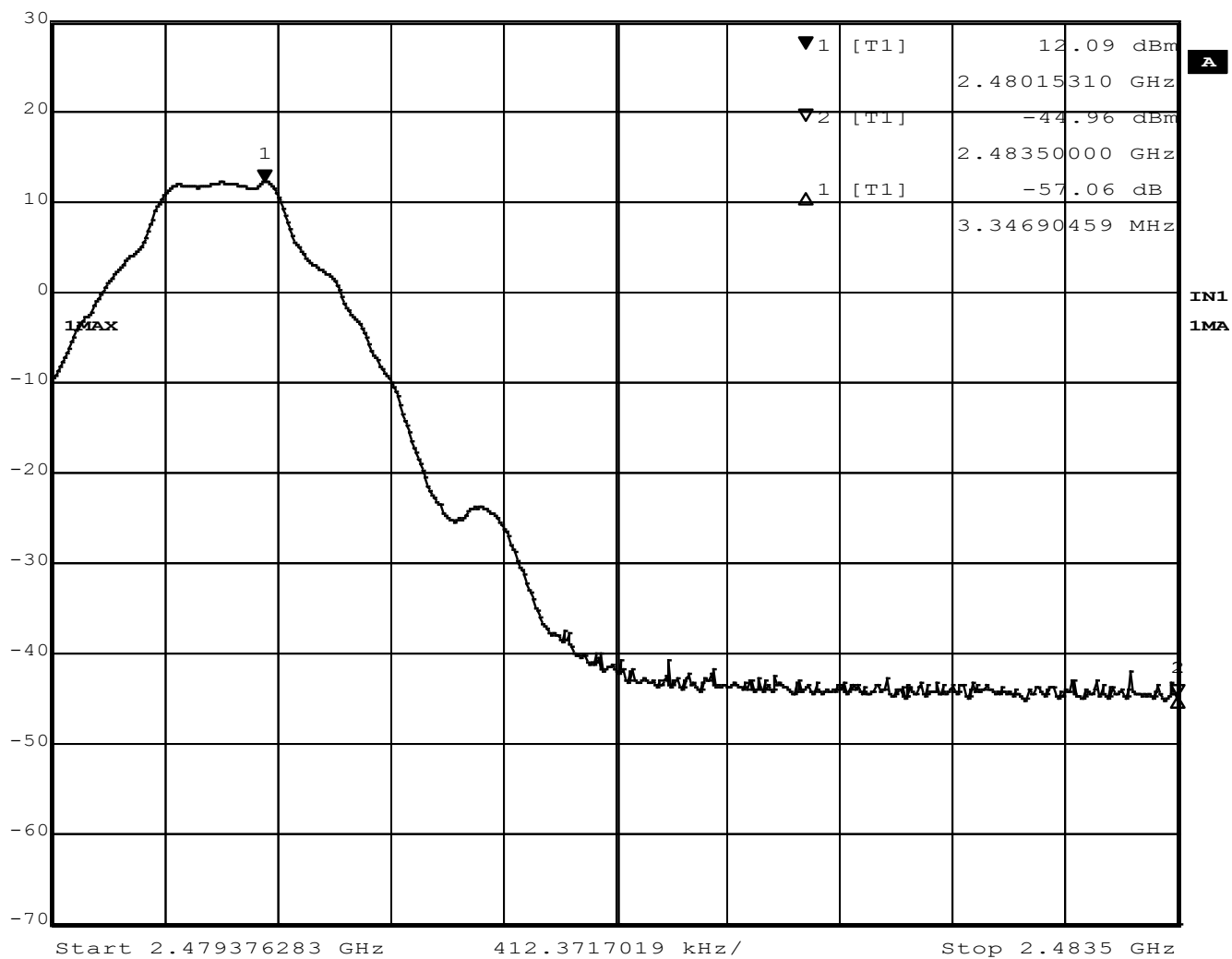
Figure 47 - Band-edge Measurement, High Channel, Fundamental, Peak
