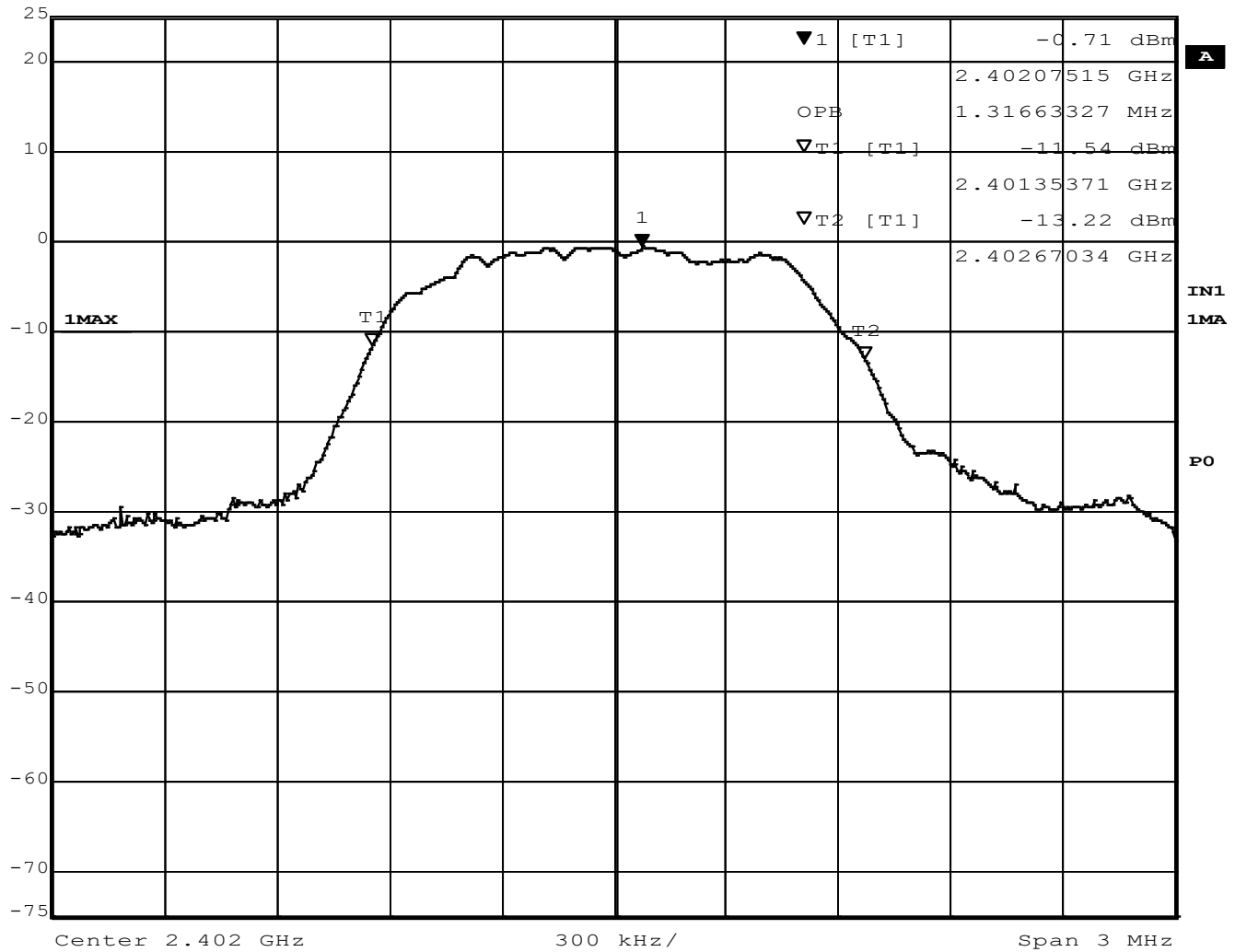
Figure 18 – Occupied Bandwidth, Low Channel, BT EDR 3MB
