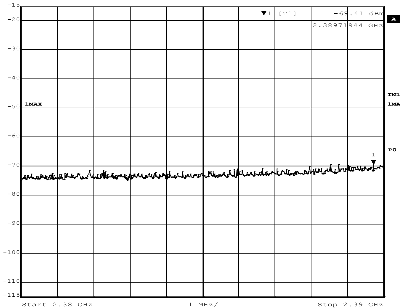
Figure 48 - Band-edge Measurement, Low Channel, Restricted Frequency, Peak
