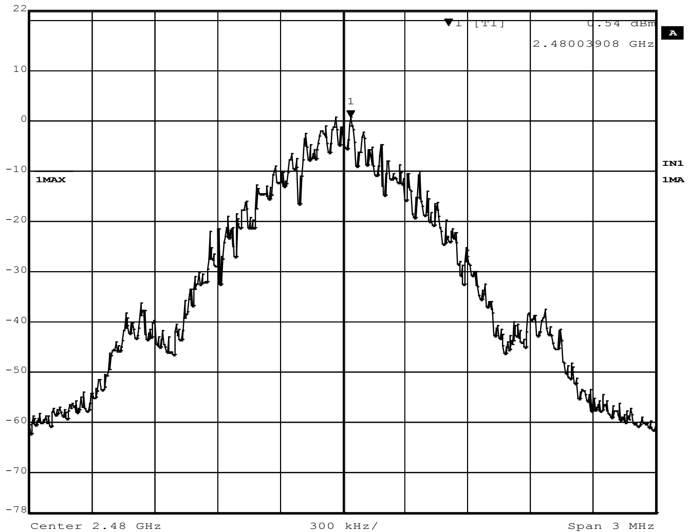
Figure 37 - Power Spectral Density, High Channel, BT BR (GFSK)
