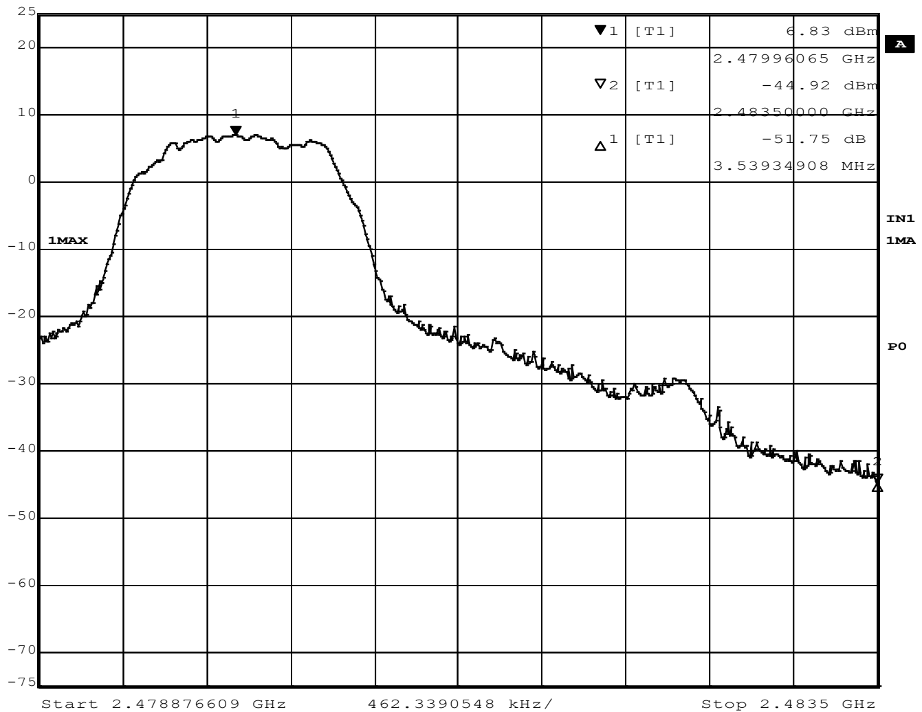
Figure 55 - Band-edge Measurement, High Channel, Fundamental, Peak
