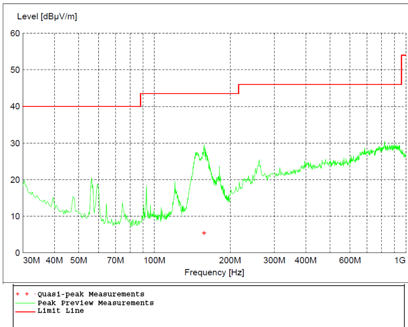
Figure 31 - Radiated Emissions Plot, Receive
