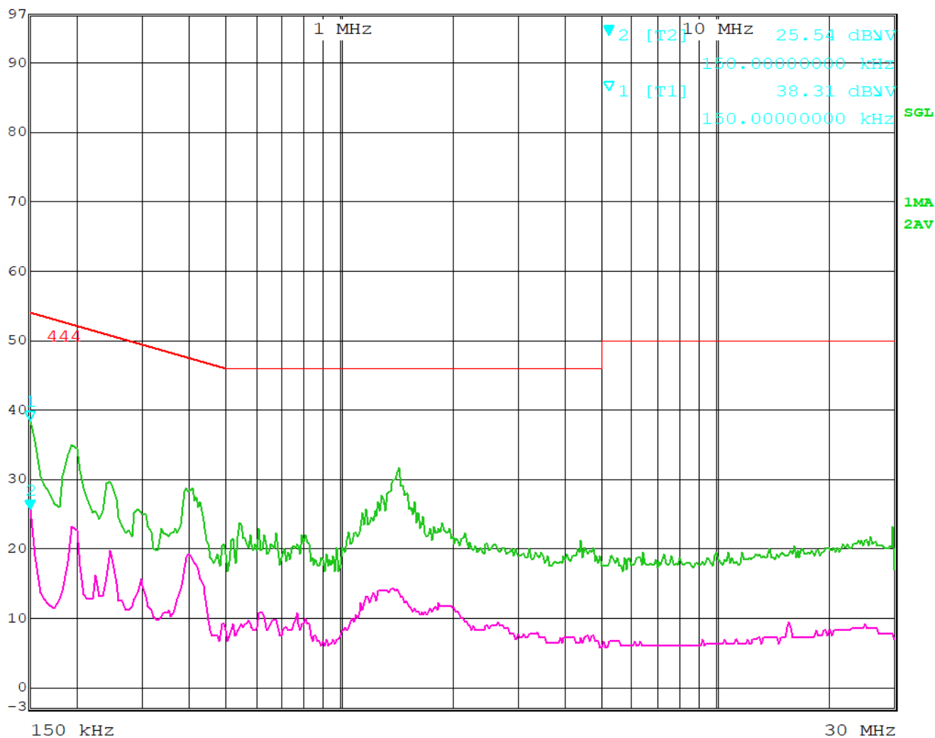
Figure 57 - Conducted Emissions Plot, Neutral
