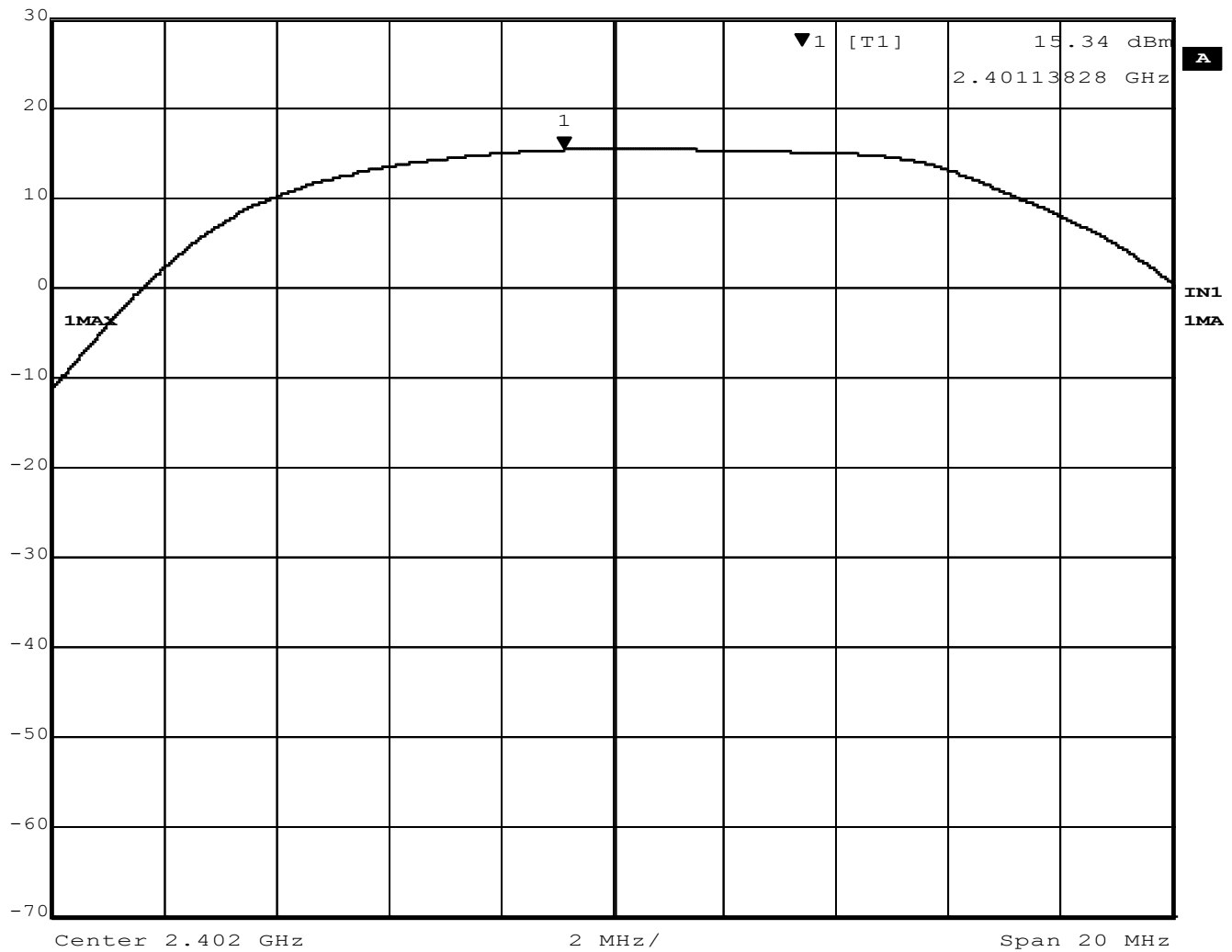
Figure 2 – Output Power, Low Channel, BT BR (GFSK)
