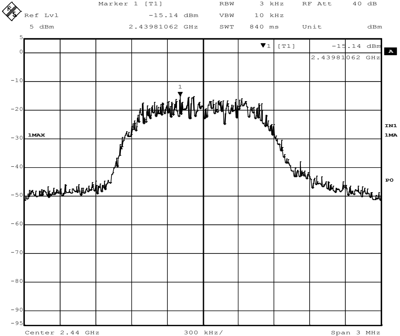
Figure 42 - Power Spectral Density, Mid Channel, BT EDR 3MB
