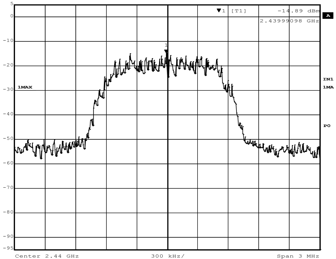
Figure 39 - Power Spectral Density, Mid Channel, BT EDR 2MB
