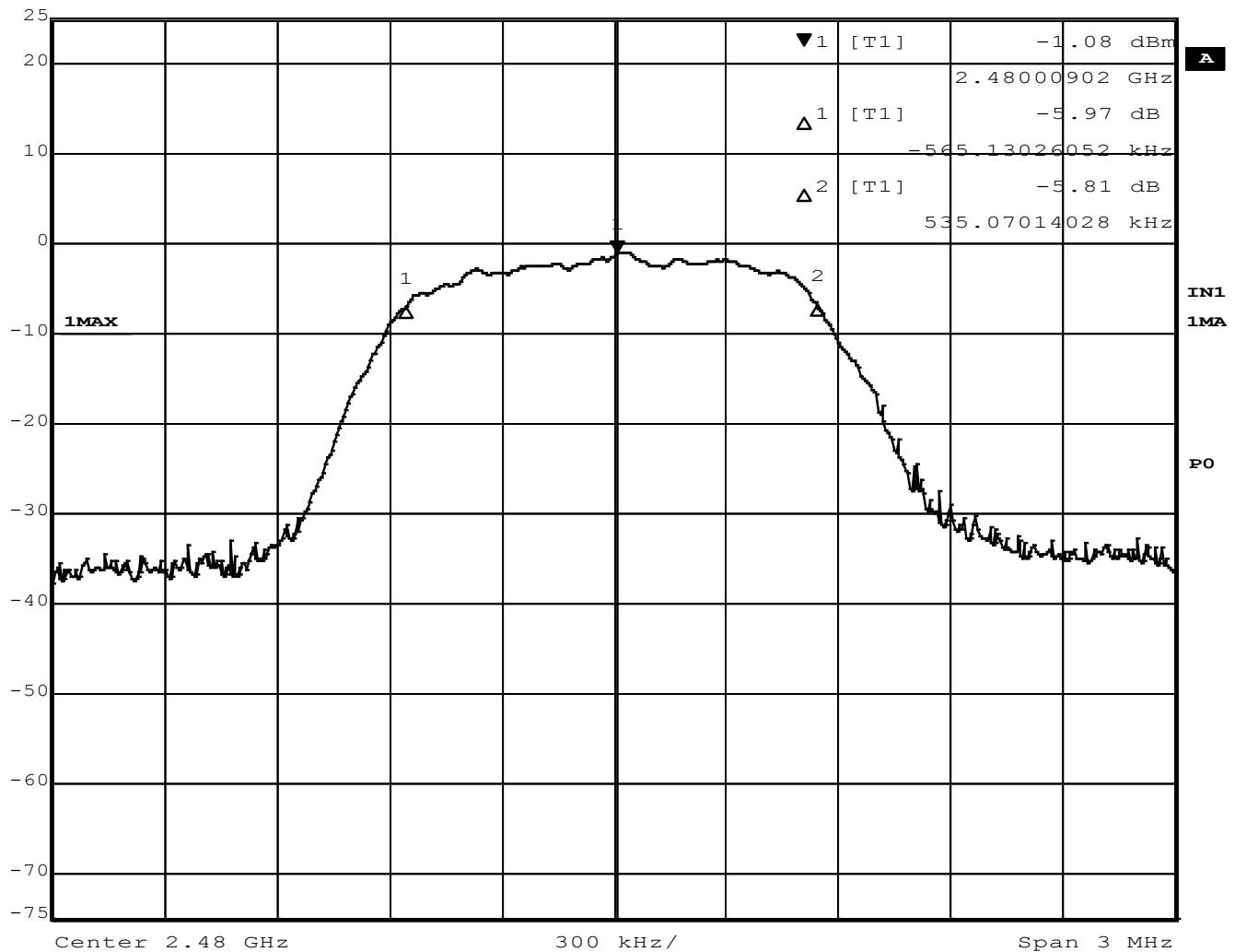
Figure 26 – 6dB Bandwidth, High Channel, BT EDR 2MB
