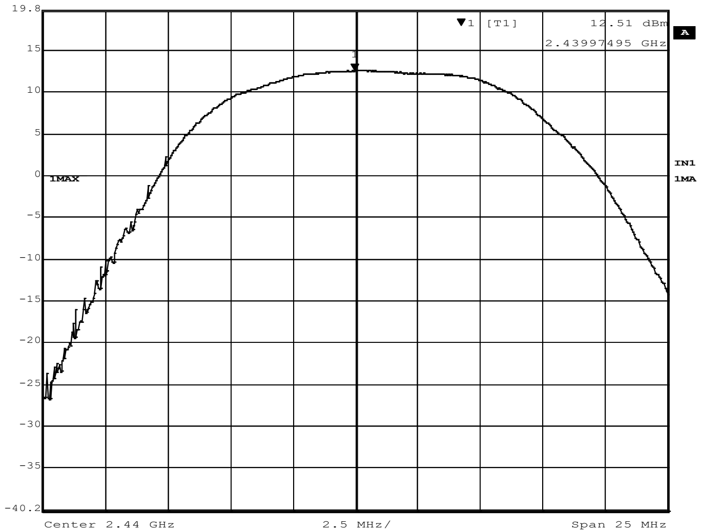
Figure 6 – Output Power, Mid Channel, BT EDR 2MB
