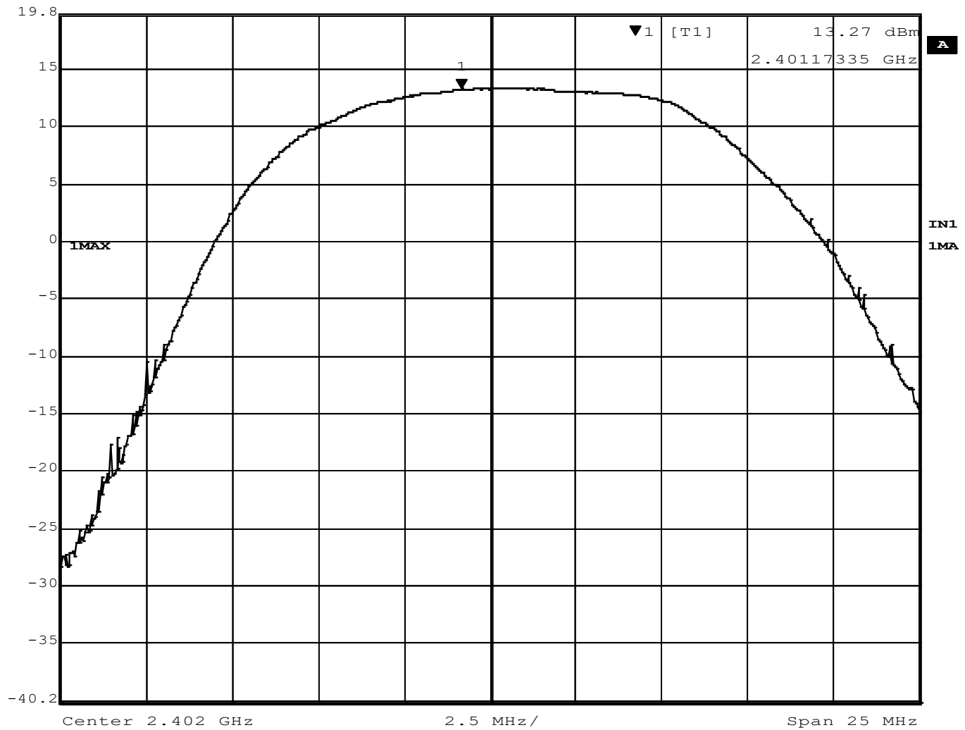
Figure 5 – Output Power, Low Channel, BT EDR 2MB
