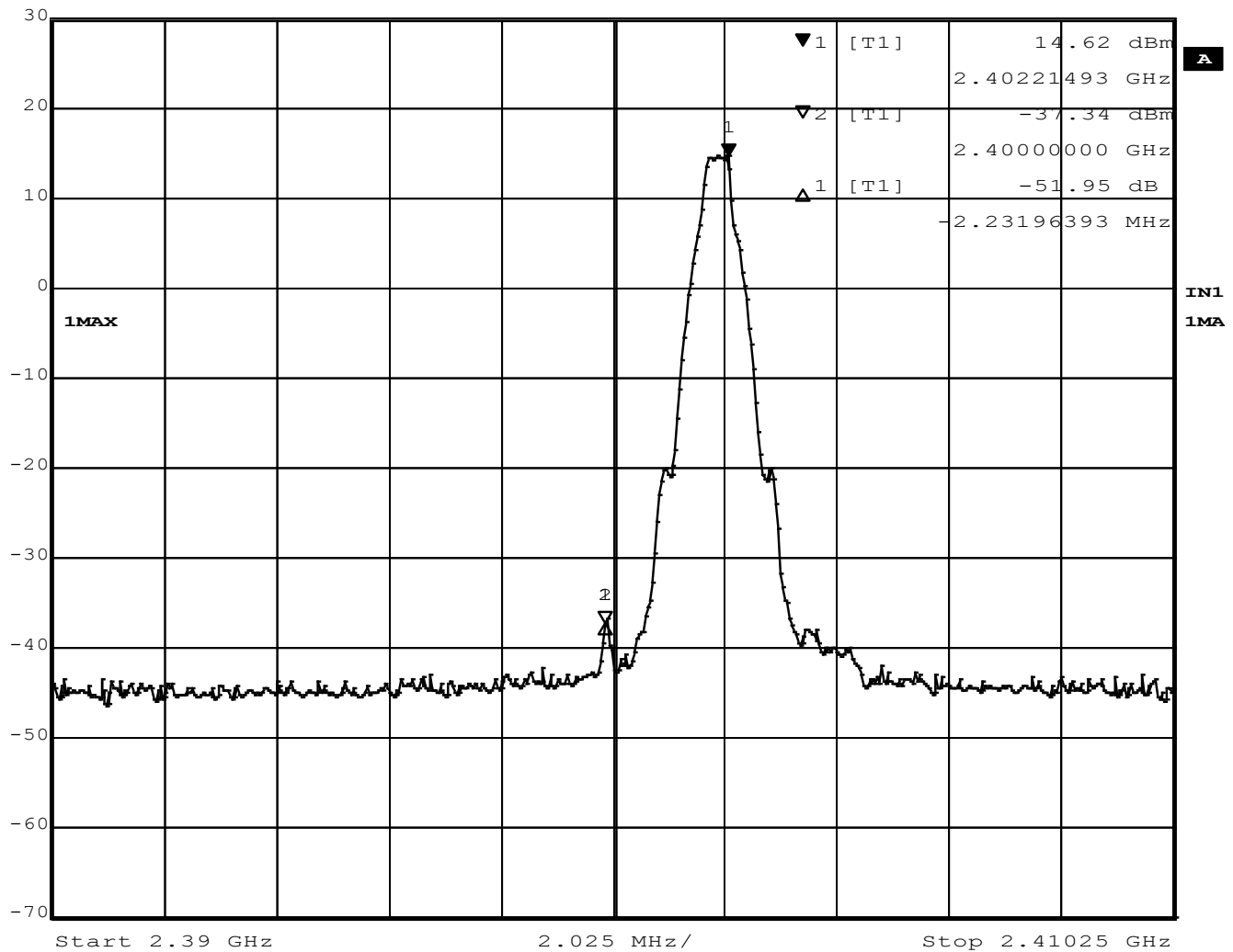
Figure 45 - Band-edge Measurement, Low Channel, Fundamental, Peak
