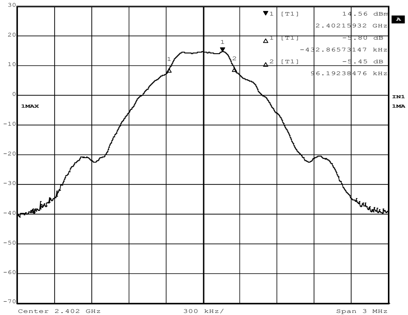
Figure 21 – 6dB Bandwidth, Low Channel, BT BR (GFSK)
