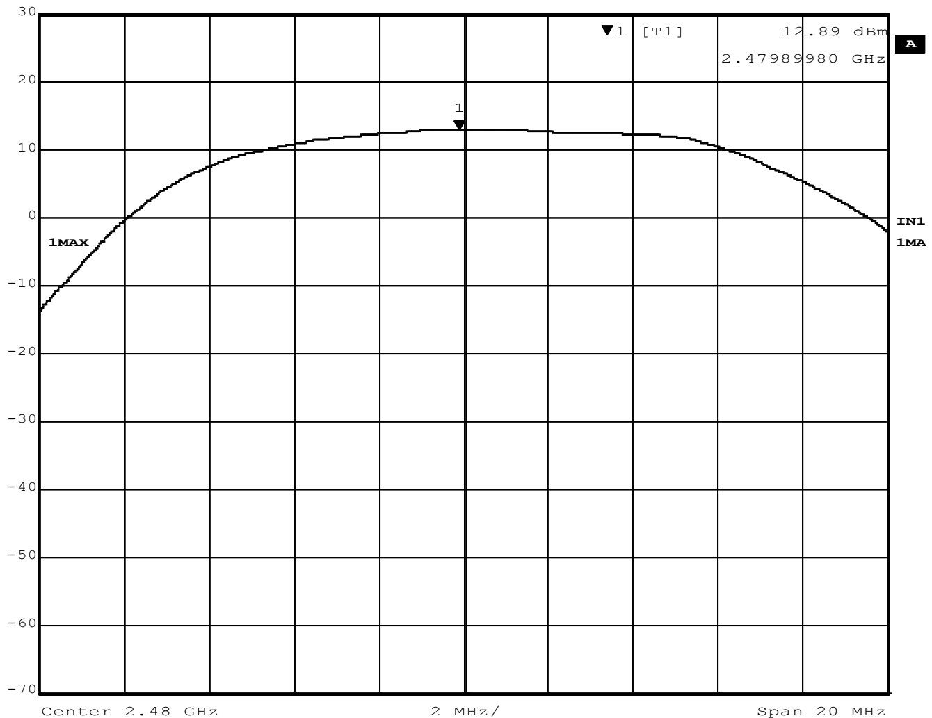
Figure 4 – Output Power, High Channel, BT BR (GFSK)
