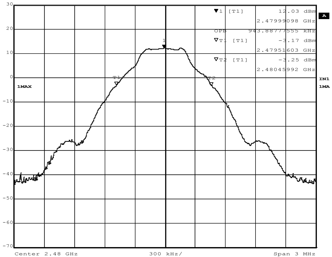
Figure 14 - Occupied Bandwidth, High Channel, BT BR (GFSK)
