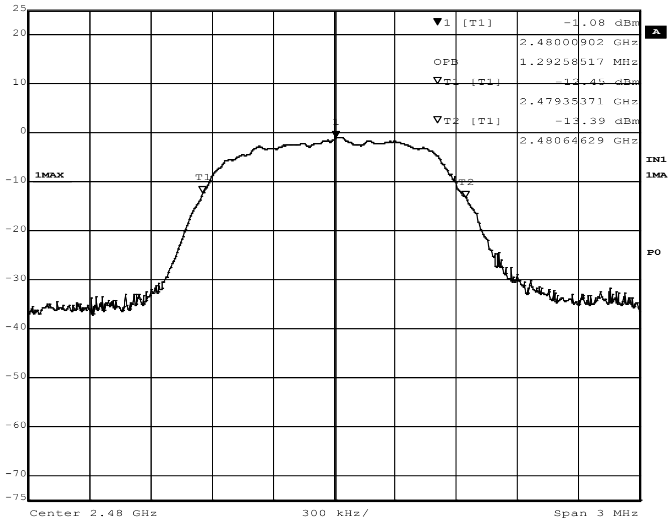
Figure 17 - Occupied Bandwidth, High Channel, BT EDR 2MB
