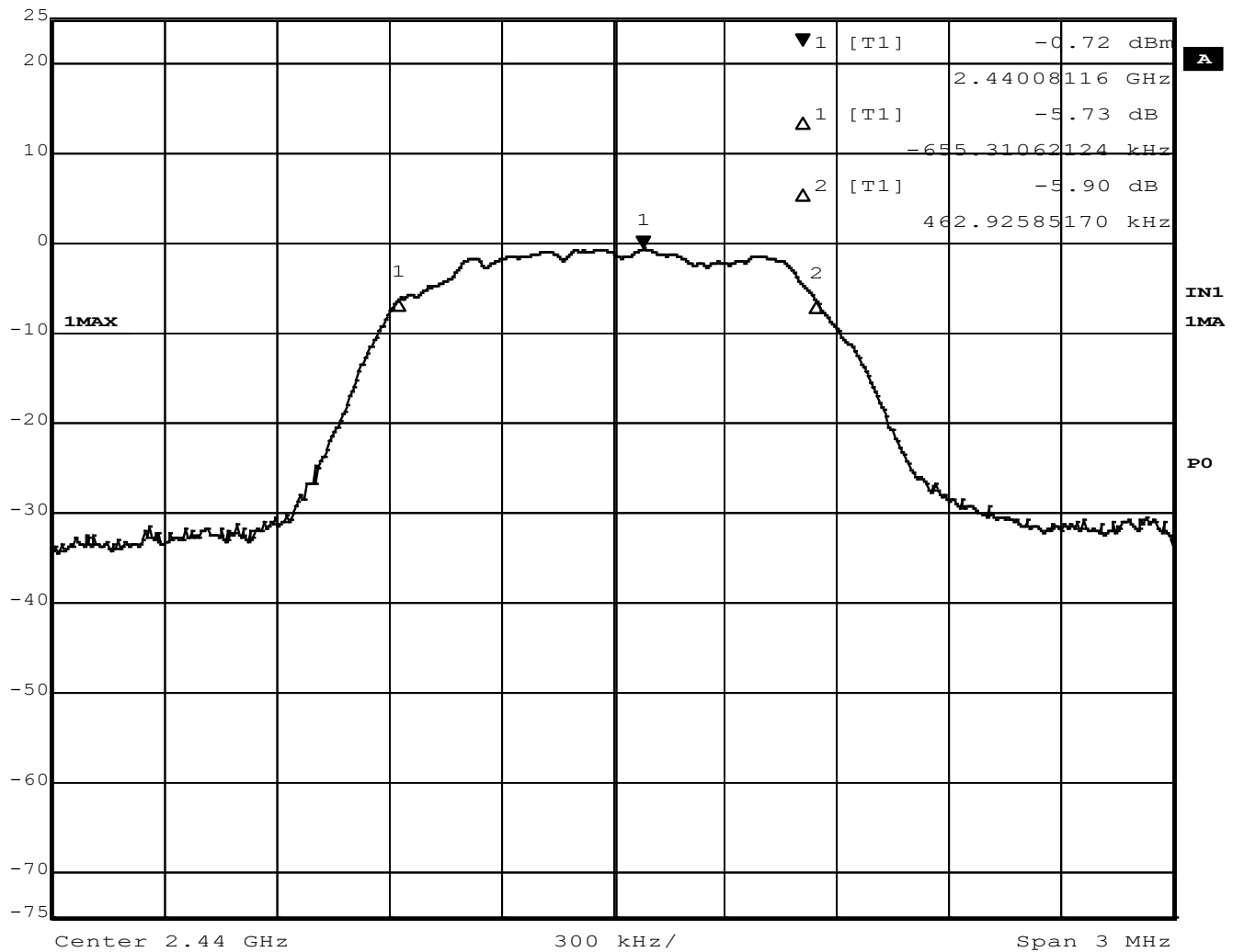
Figure 28 – 6dB Bandwidth, Mid Channel, BT EDR 3MB
