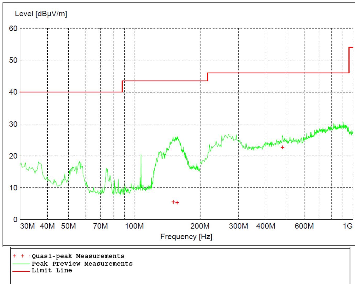
Figure 32 - Radiated Emissions Plot, BT BR (GFSK)
