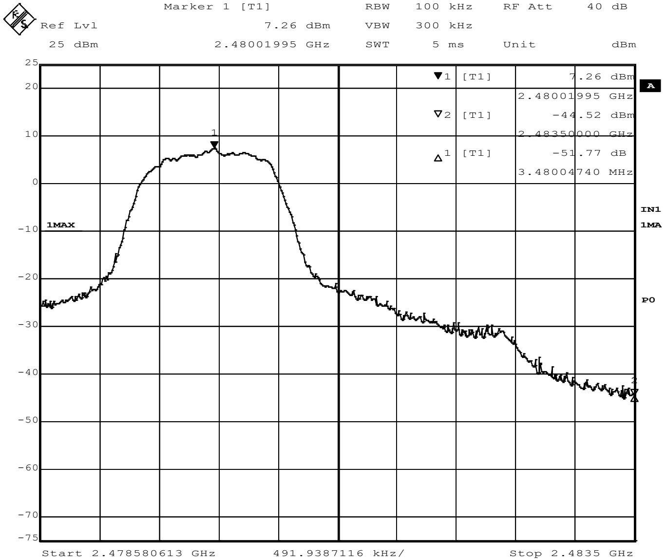
Figure 51 - Band-edge Measurement, High Channel, Fundamental, Peak
