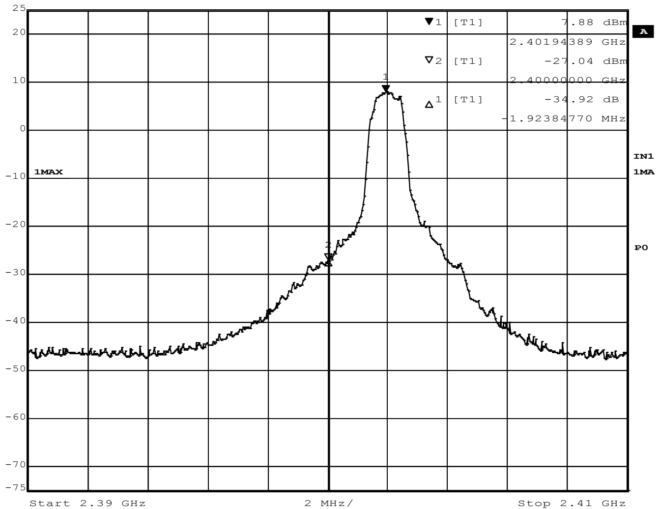
Figure 53 - Band-edge Measurement, Low Channel, Fundamental, Peak
