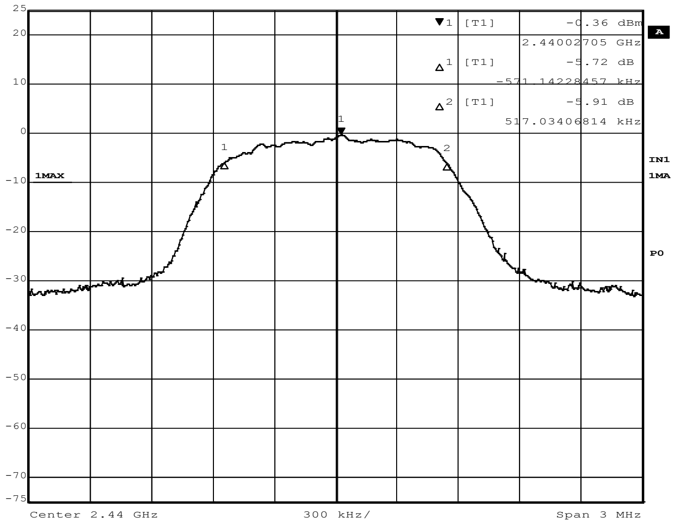
Figure 25 – 6dB Bandwidth, Mid Channel, BT EDR 2MB
