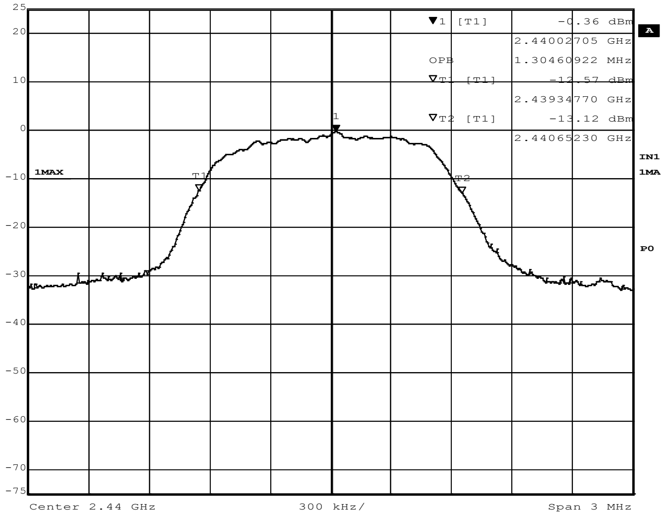
Figure 16 - Occupied Bandwidth, Mid Channel, BT EDR 2MB
