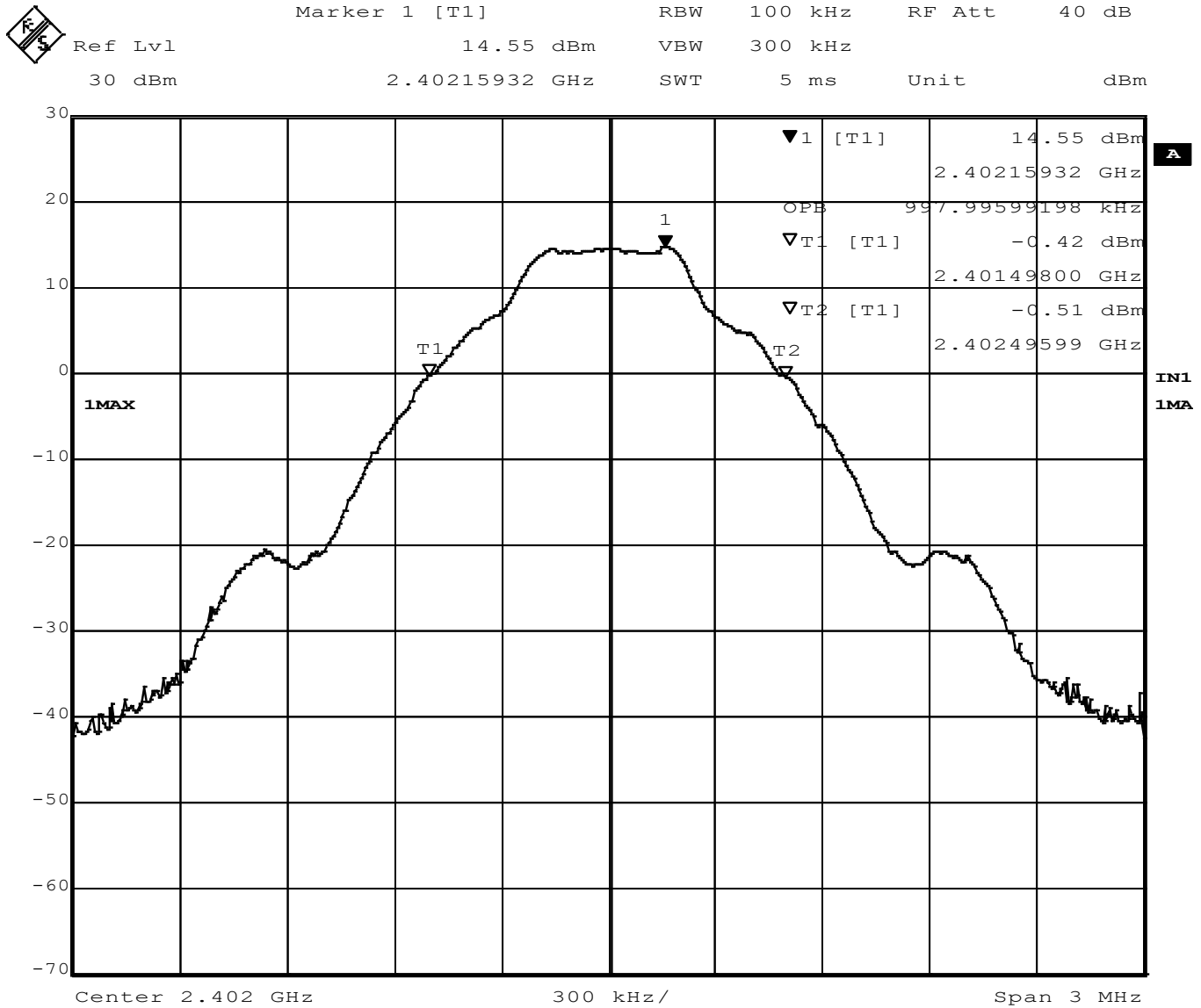
Figure 12 – Occupied Bandwidth, Low Channel, BT BR (GFSK)
