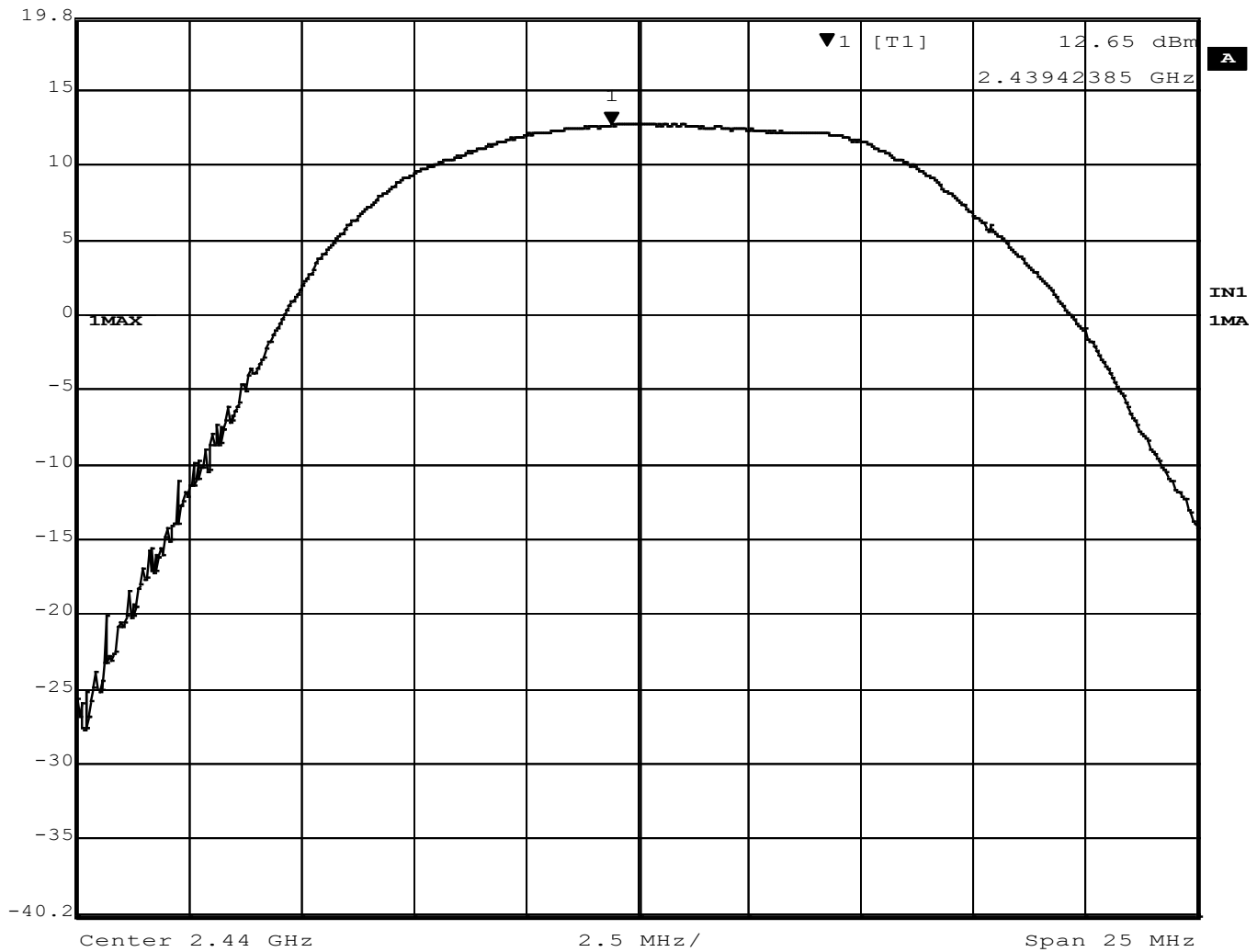
Figure 9 – Output Power, Mid Channel, BT EDR 3MB
