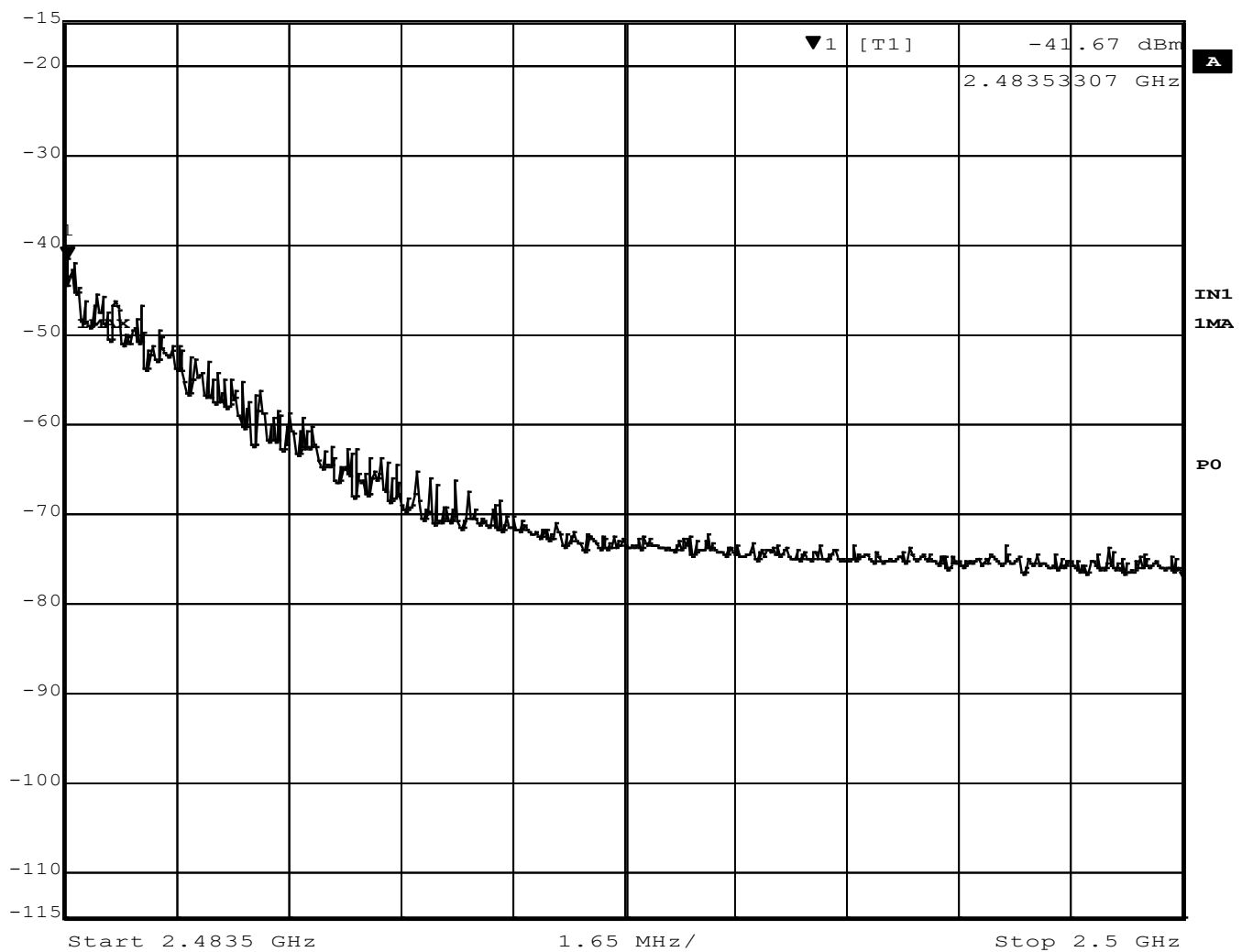
Figure 50 - Band-edge Measurement, High Channel, Restricted Frequency, Peak
