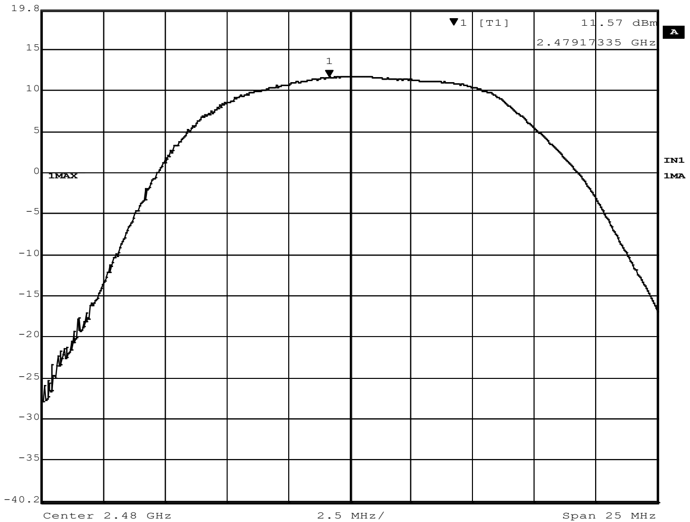
Figure 10 – Output Power, High Channel, BT EDR 3MB
