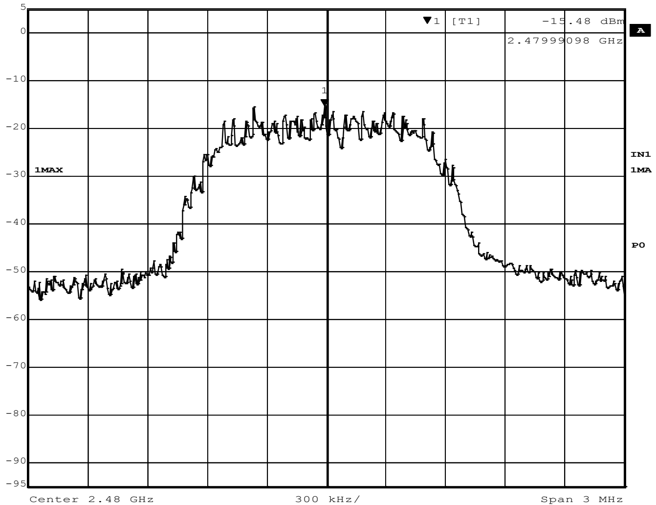
Figure 40 - Power Spectral Density, High Channel, BT EDR 2MB
