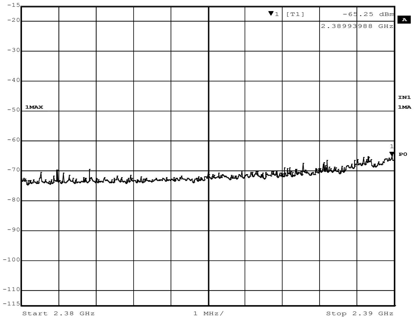
Figure 52 - Band-edge Measurement, Low Channel, Restricted Frequency, Peak
