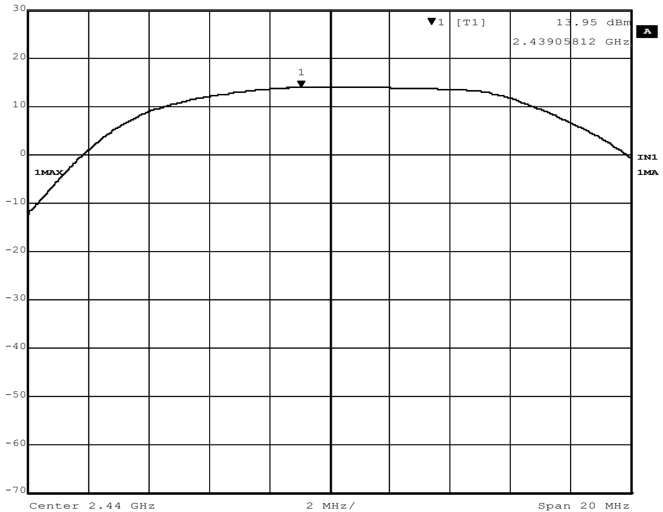
Figure 3 – Output Power, Mid Channel, BT BR (GFSK)
