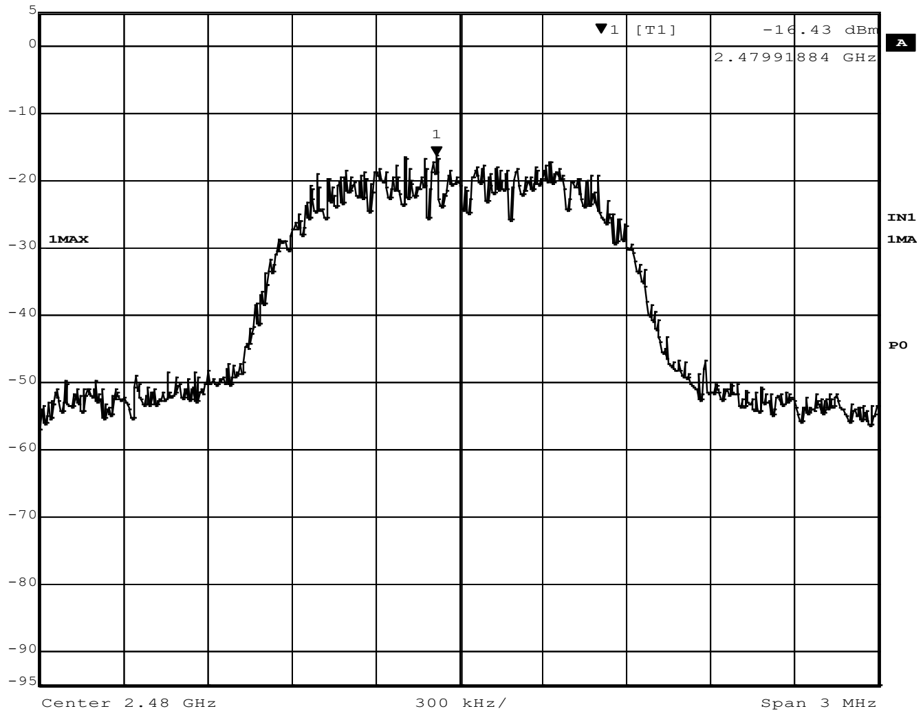
Figure 43 - Power Spectral Density, High Channel, BT EDR 3MB
