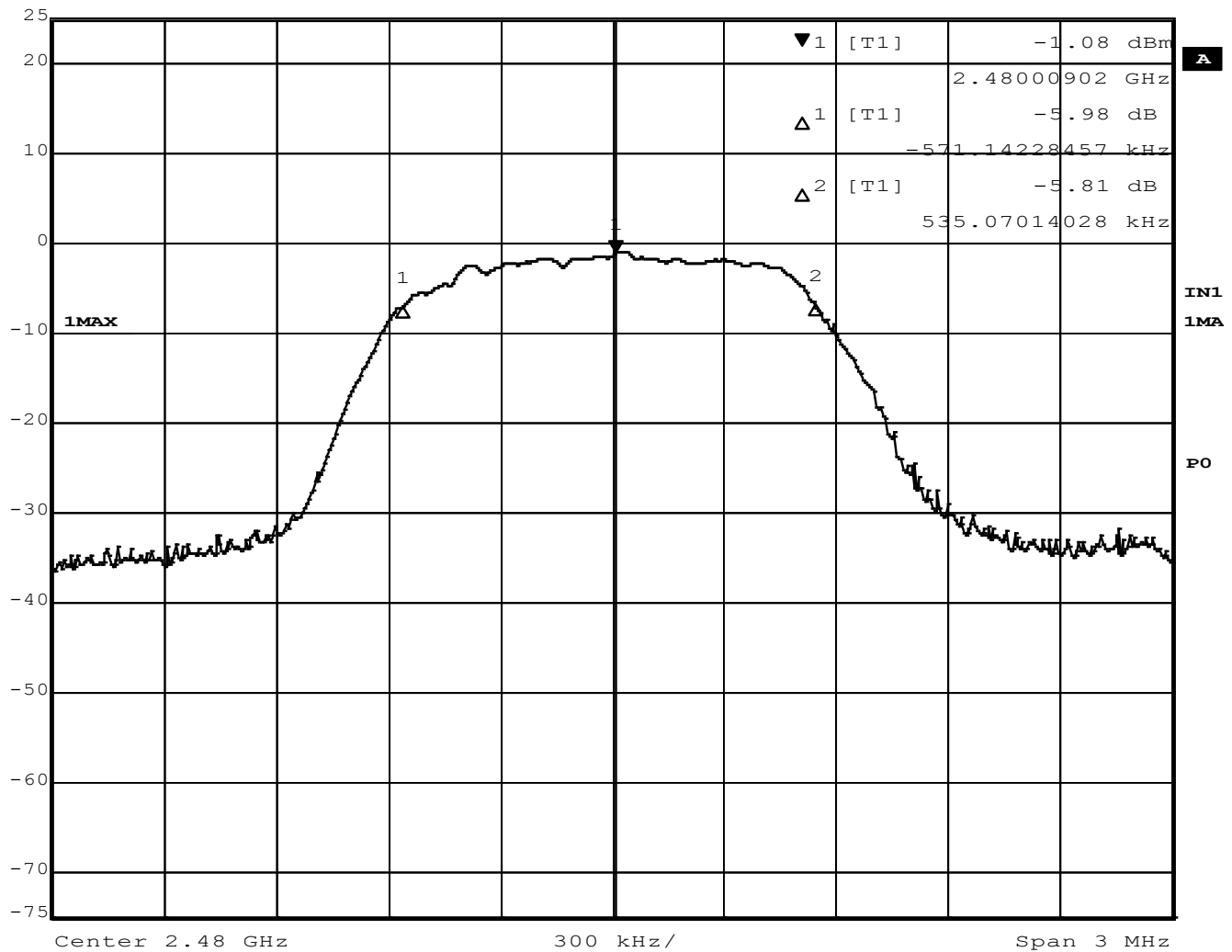
Figure 29 – 6dB Bandwidth, High Channel, BT EDR 3MB
