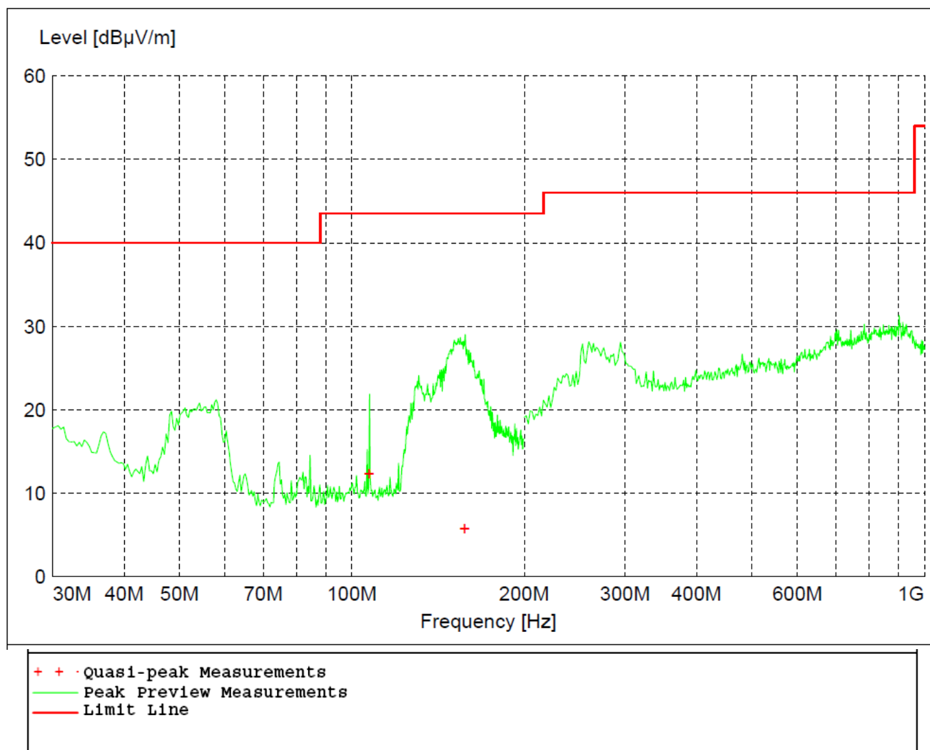
Figure 33 - Radiated Emissions Plot, BT EDR 2MB
