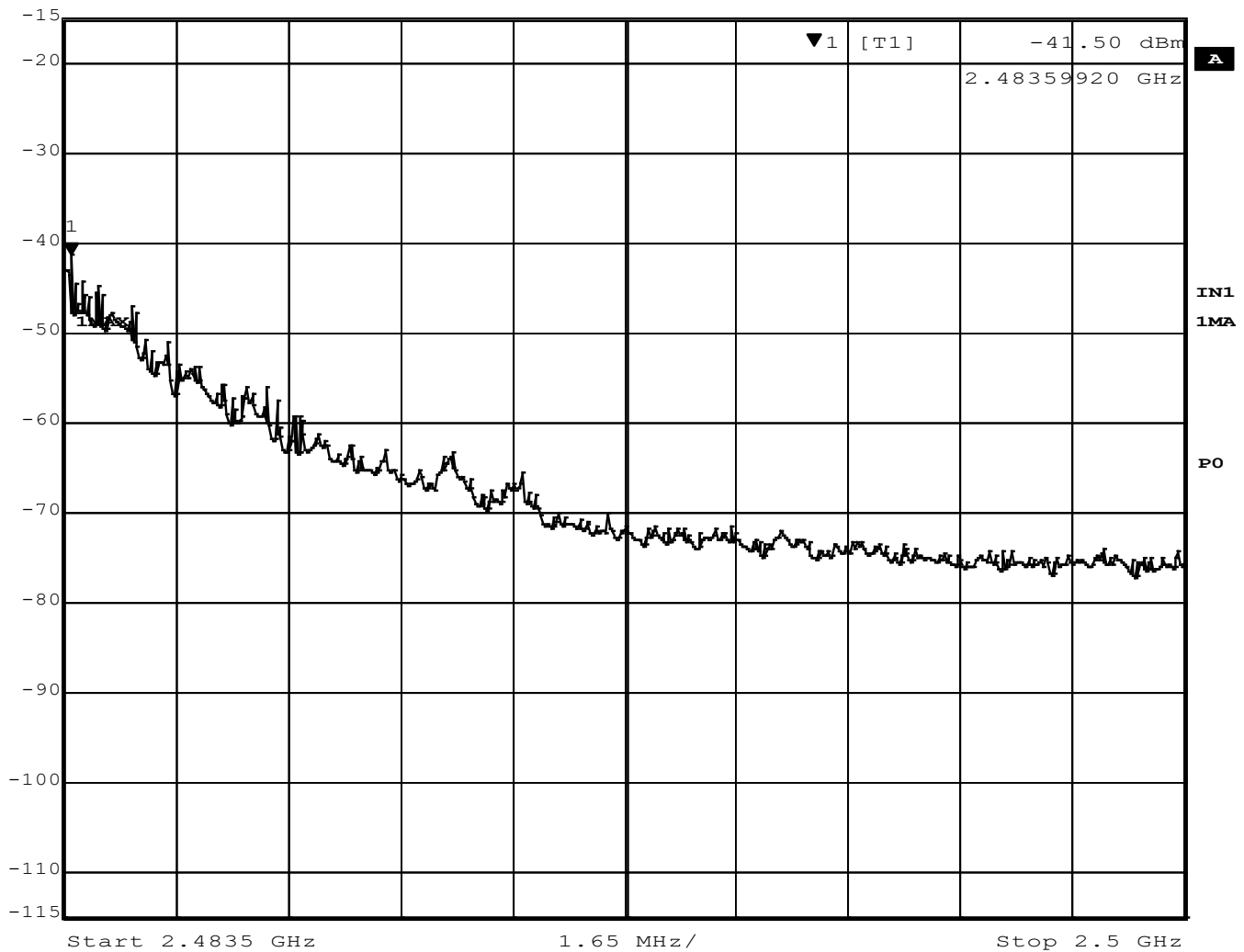
Figure 54 - Band-edge Measurement, High Channel, Restricted Frequency, Peak
