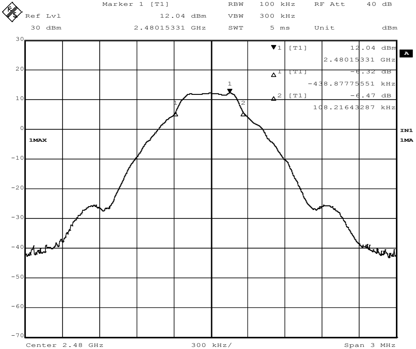
Figure 23 – 6dB Bandwidth, High Channel, BT BR (GFSK)
