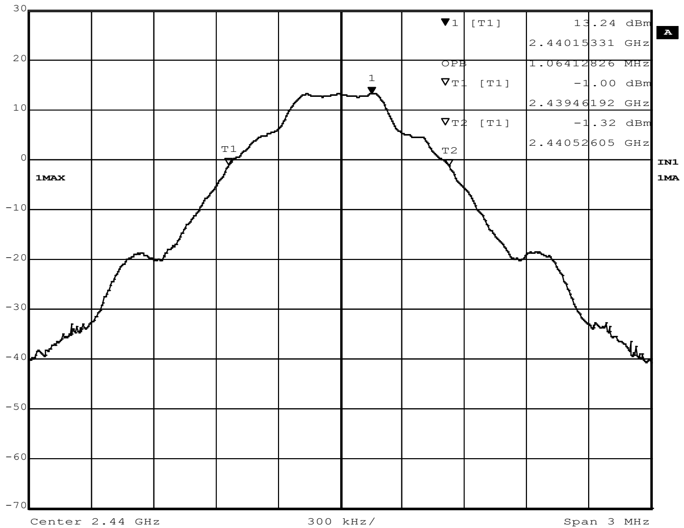
Figure 13 - Occupied Bandwidth, Mid Channel, BT BR (GFSK)
