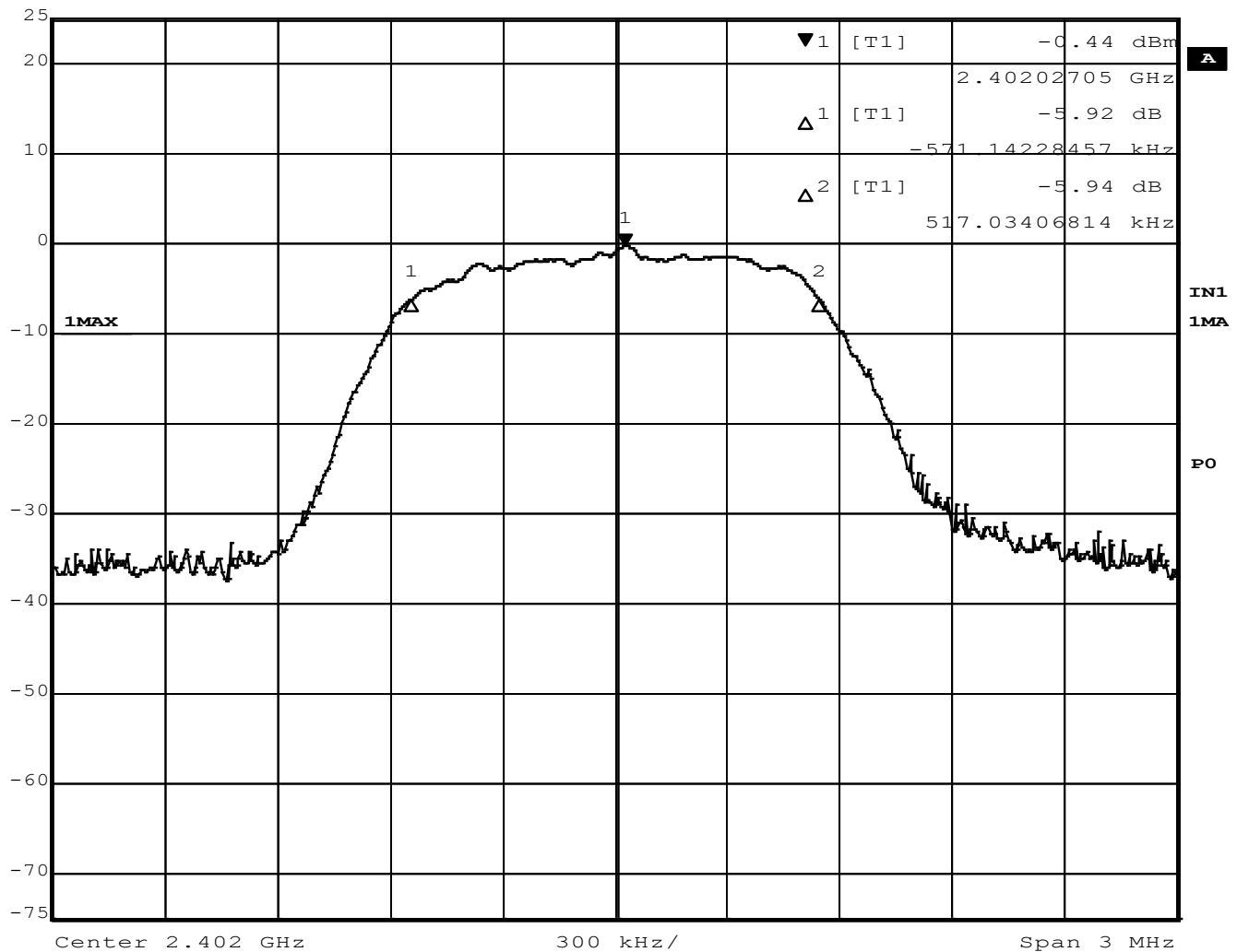
Figure 24 – 6dB Bandwidth, Low Channel, BT EDR 2MB
