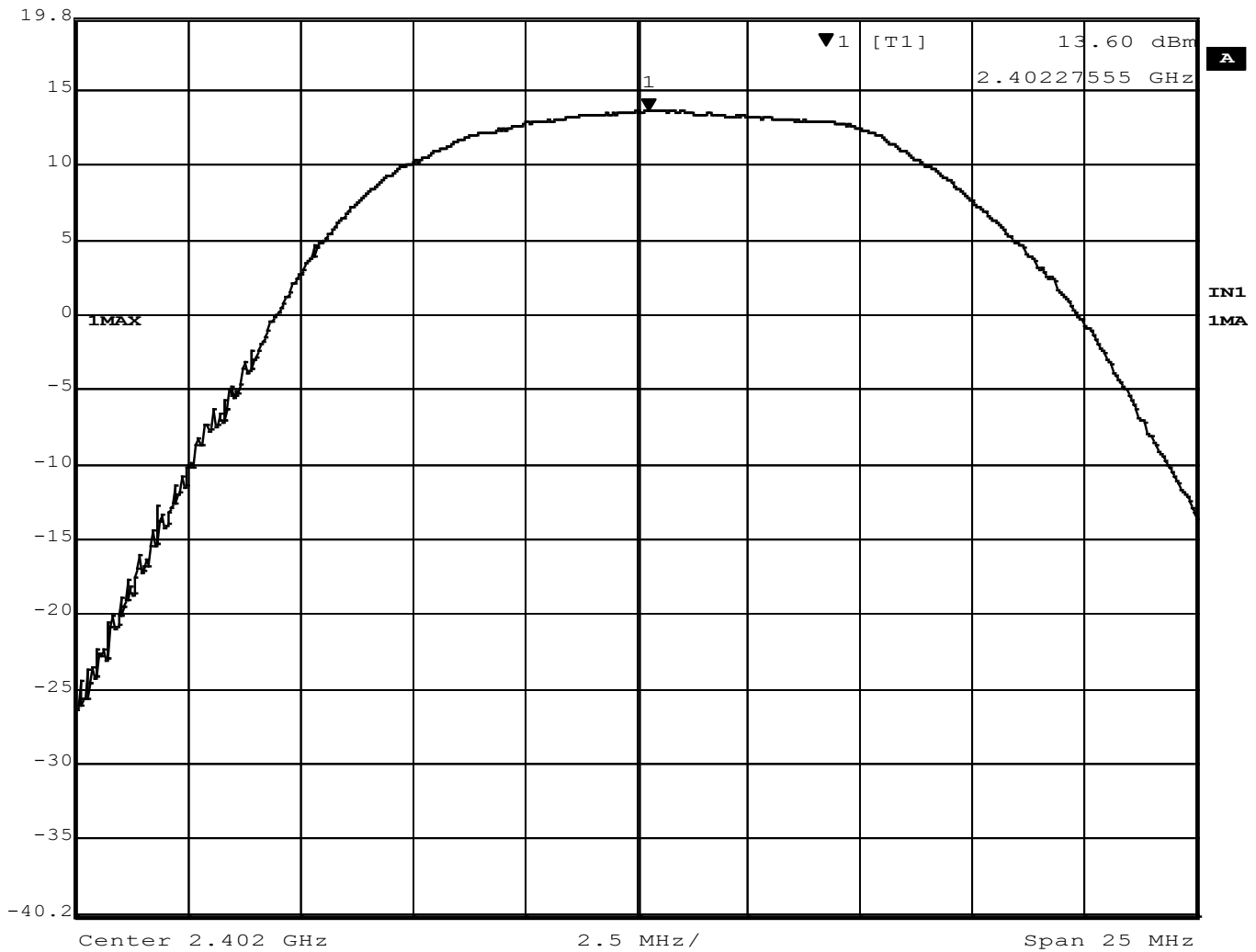
Figure 8 – Output Power, Low Channel, BT EDR 3MB
