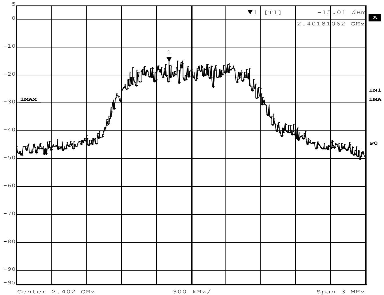
Figure 41 - Power Spectral Density, Low Channel, BT EDR 3MB
