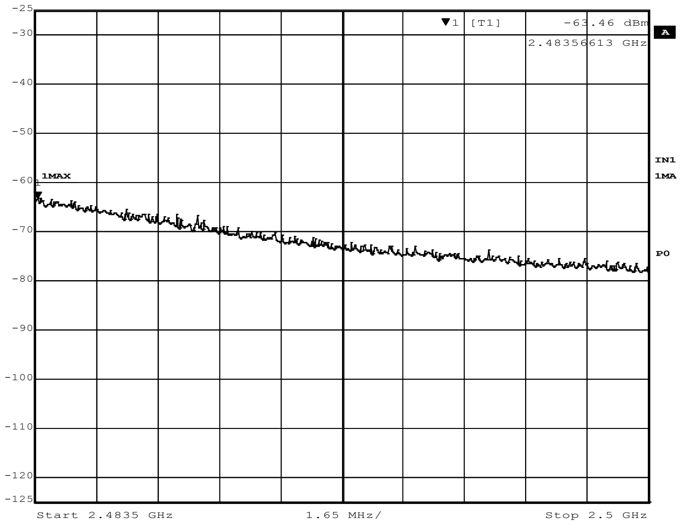
Figure 46 - Band-edge Measurement, High Channel, Restricted Frequency, Peak
