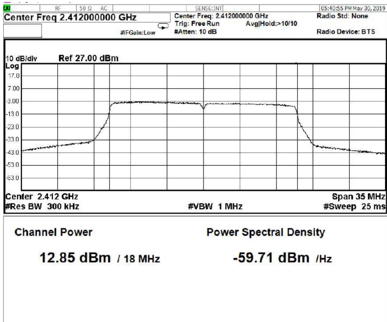
Figure 12 – Highest Measured Average Output Power, 802.11n
