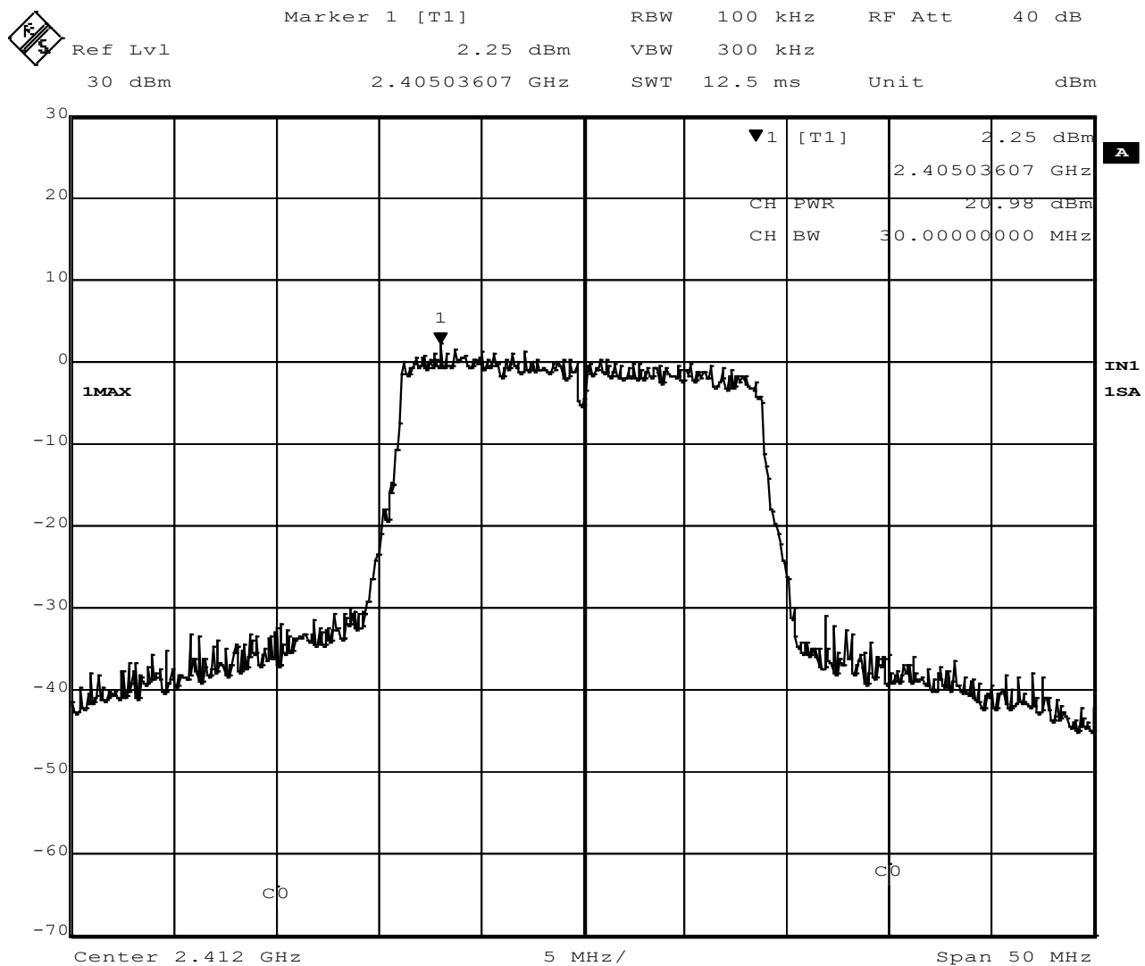
Figure 9 – Highest Measured Peak Output Power, 802.11n
