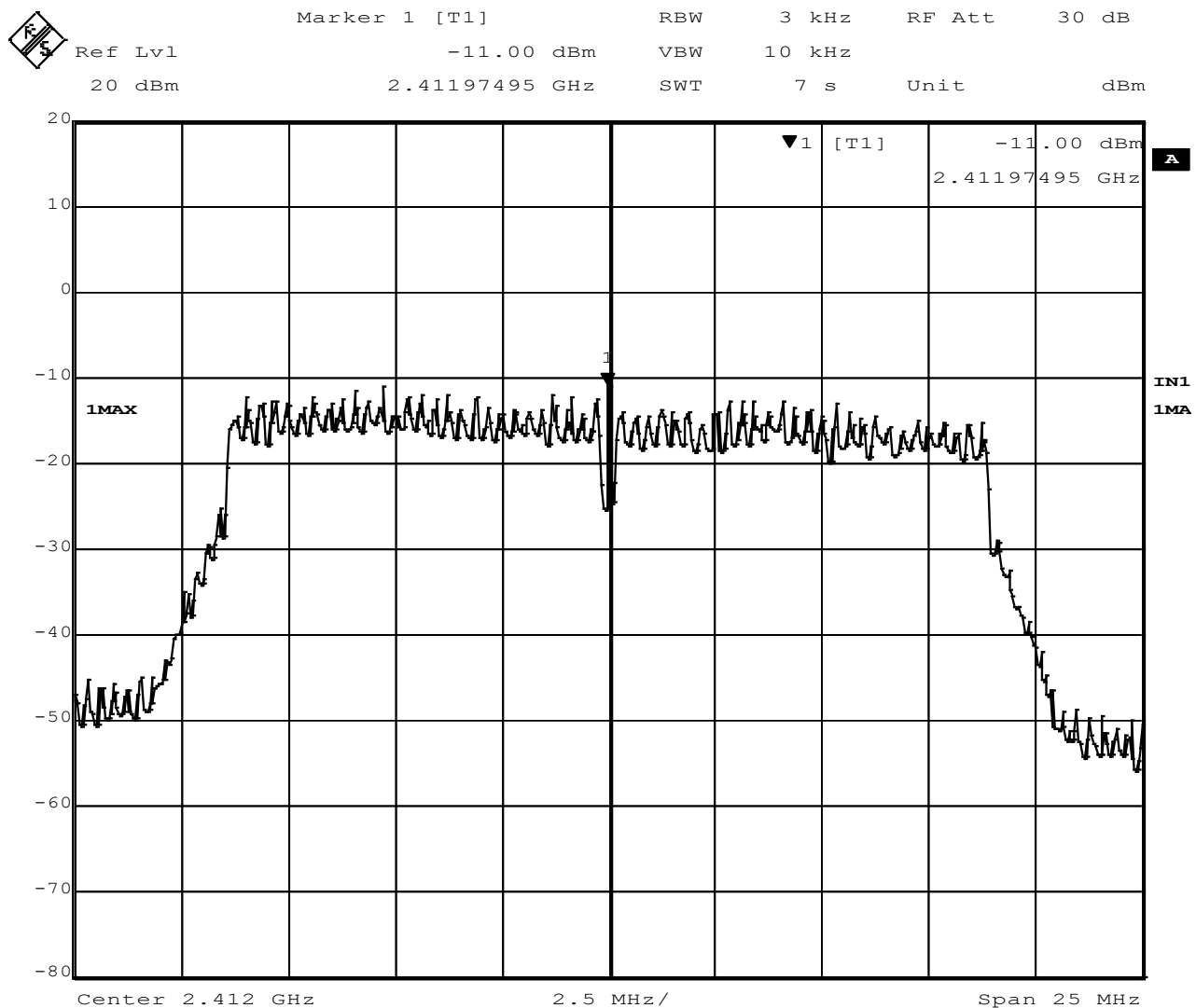
Figure 62 - Power Spectral Density, Low Channel, 802.11n
