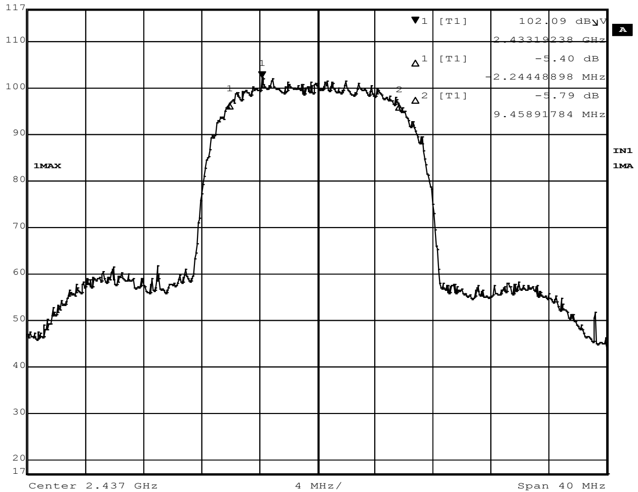
Figure 24 - 6dB Bandwidth, Mid Channel, 802.11b
