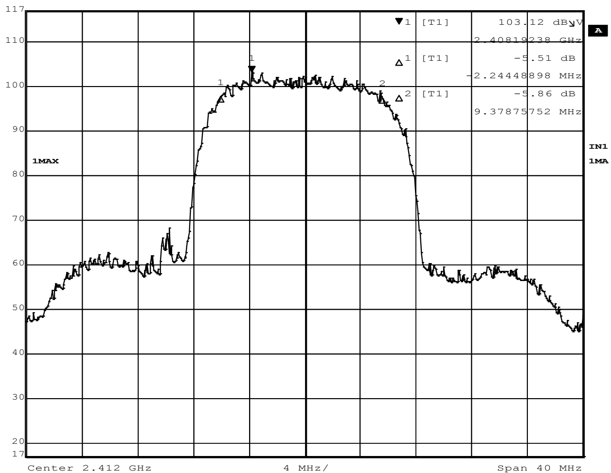
Figure 23 - 6dB Bandwidth, Low Channel, 802.11b
