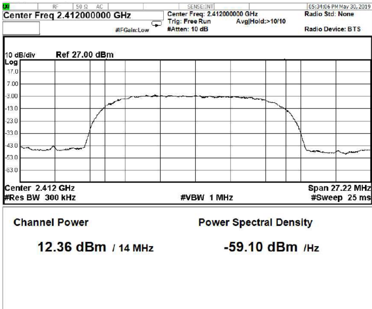
Figure 10 – Highest Measured Average Output Power, 802.11b
