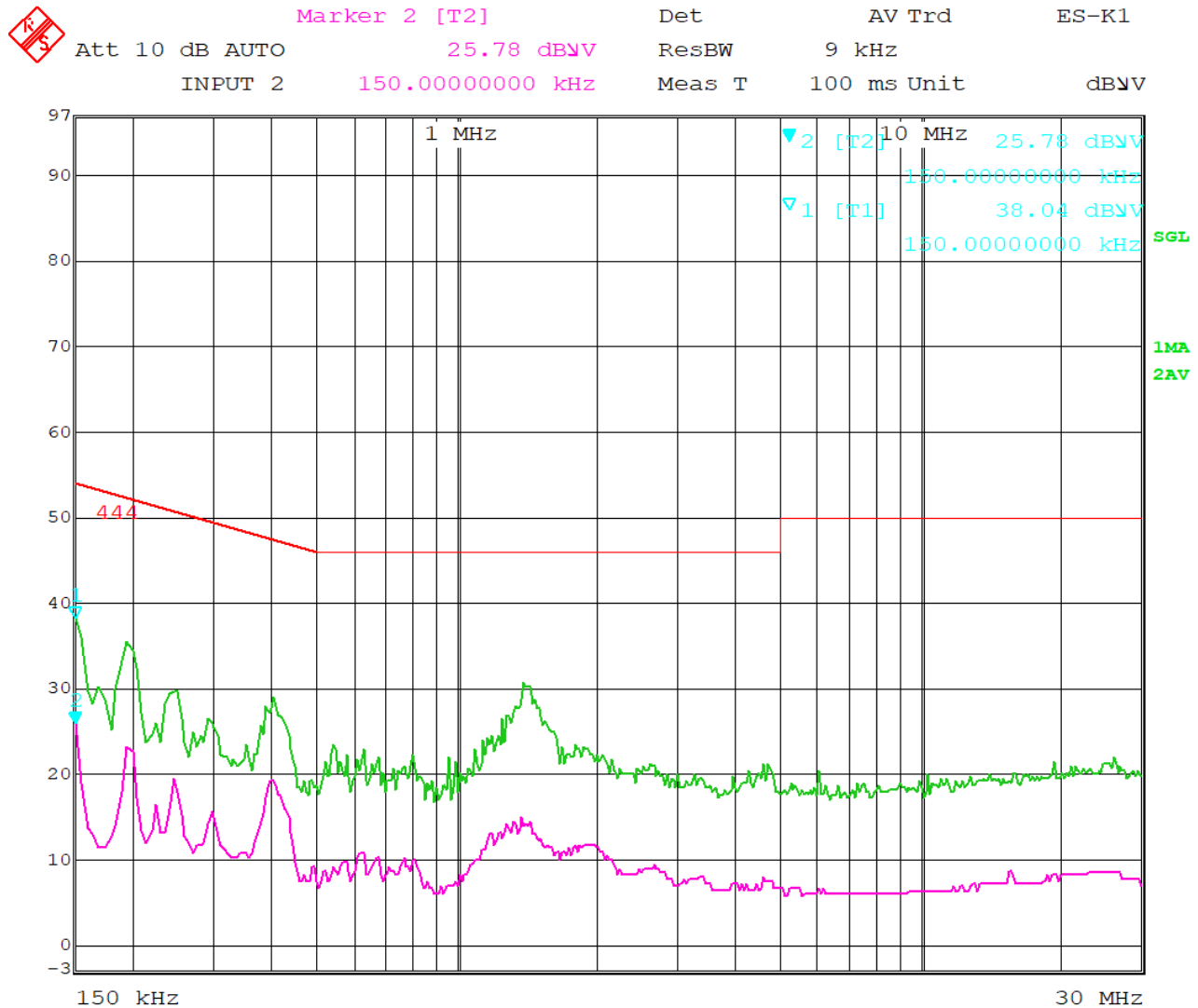
. Figure 66 - Conducted Emissions Plot, Neutral
