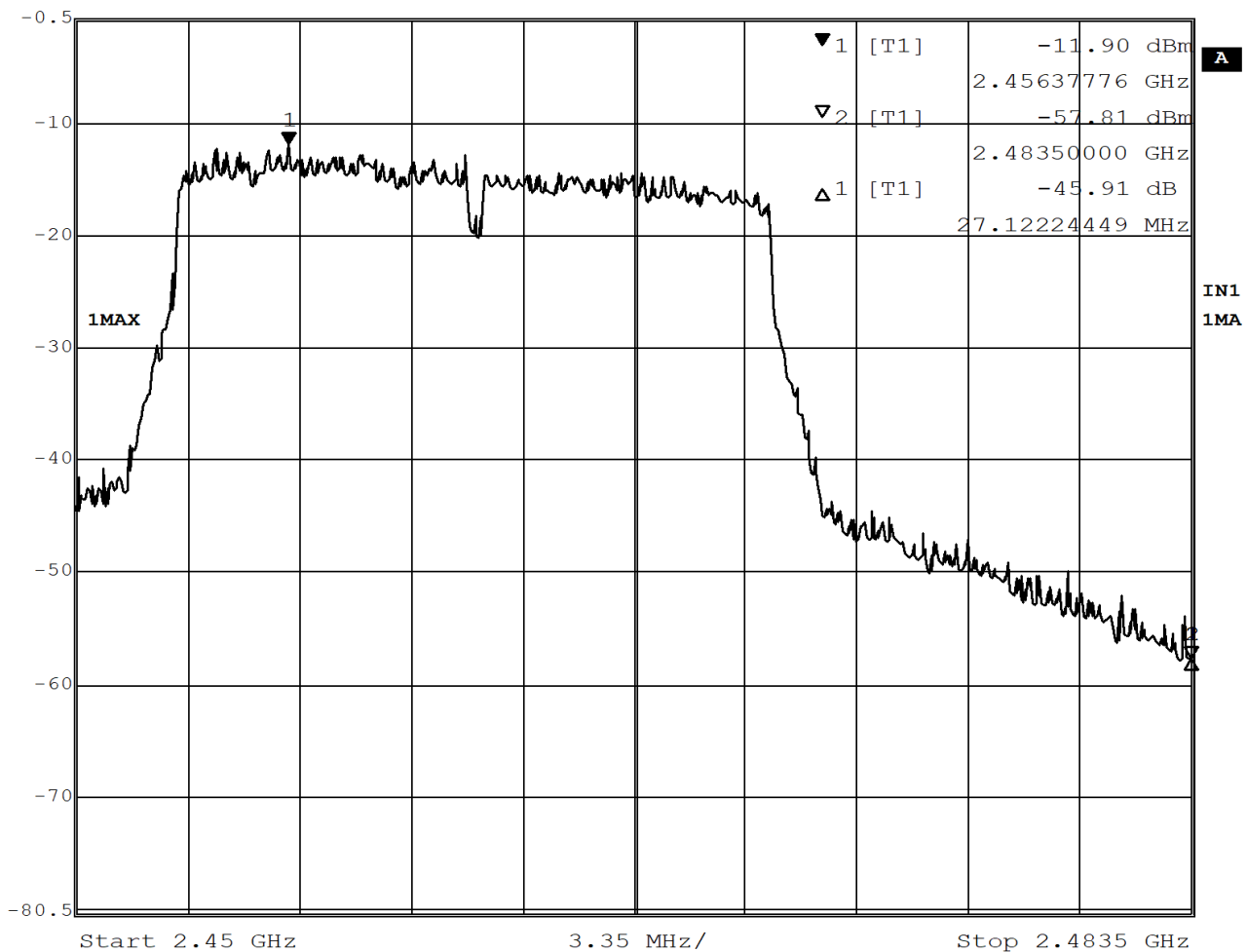
Figure 53 - Band-edge Measurement, High Channel, Fundamental, Peak
