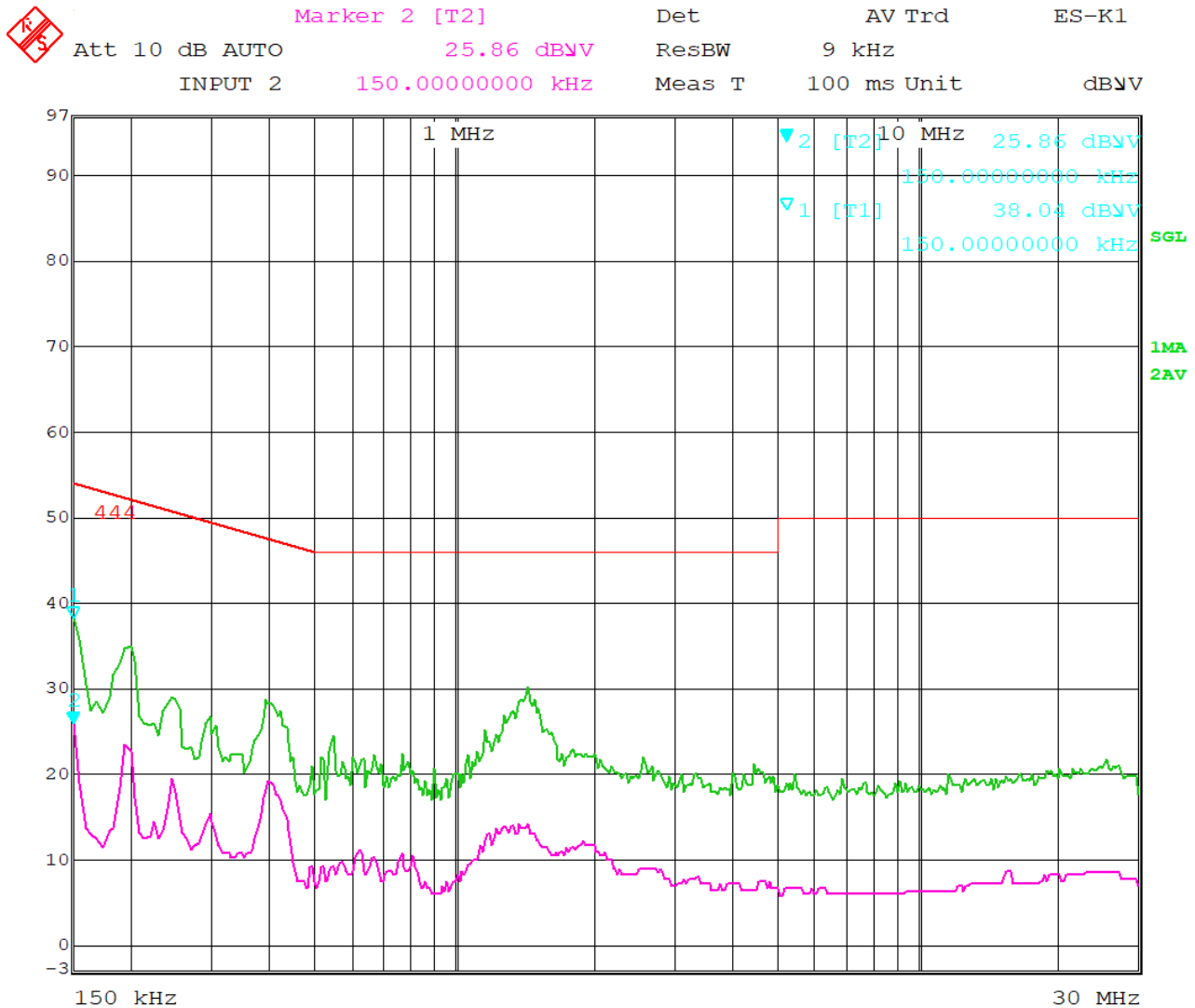
Figure 65 - Conducted Emissions Plot, Line
