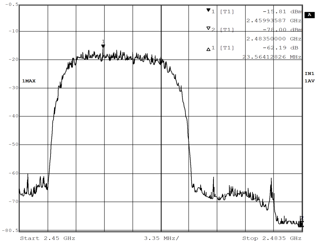
Figure 39 - Band-edge Measurement, High Channel, Fundamental, Average
