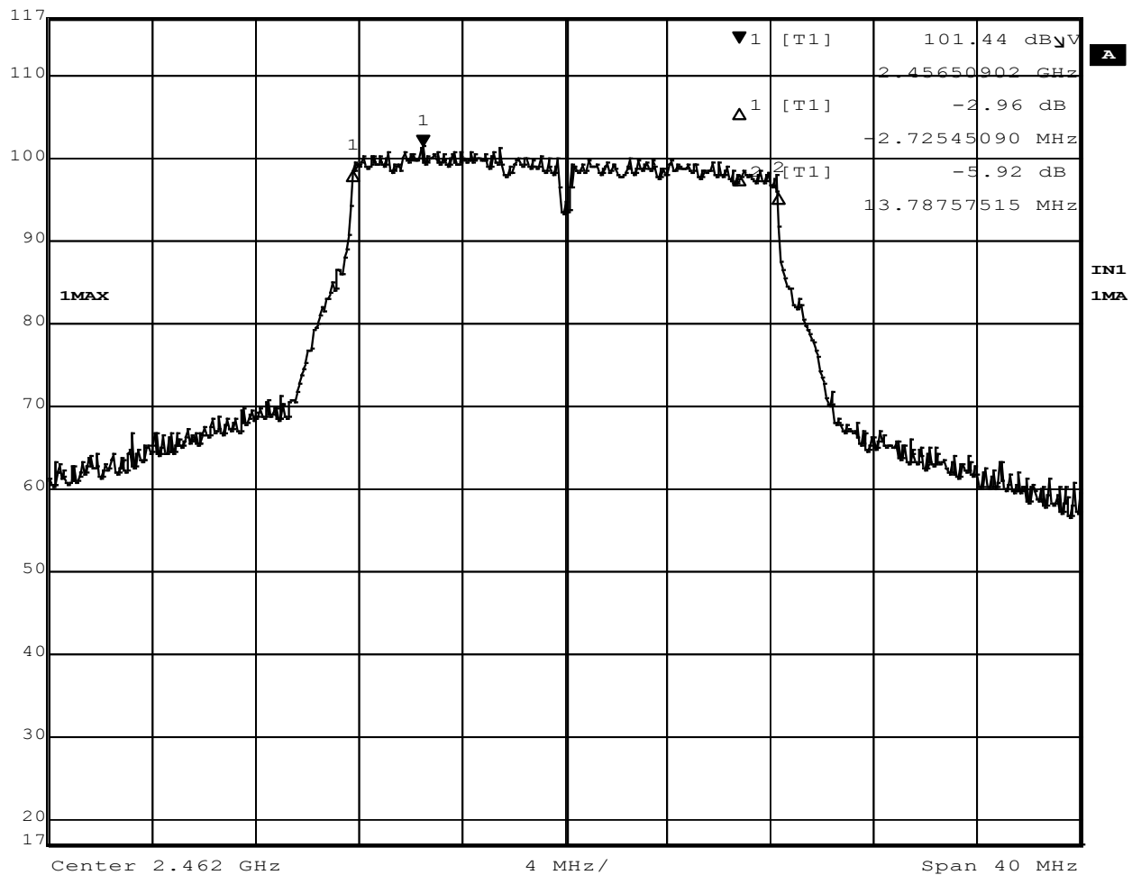
Figure 28 - 6dB Bandwidth, High Channel, 802.11g
