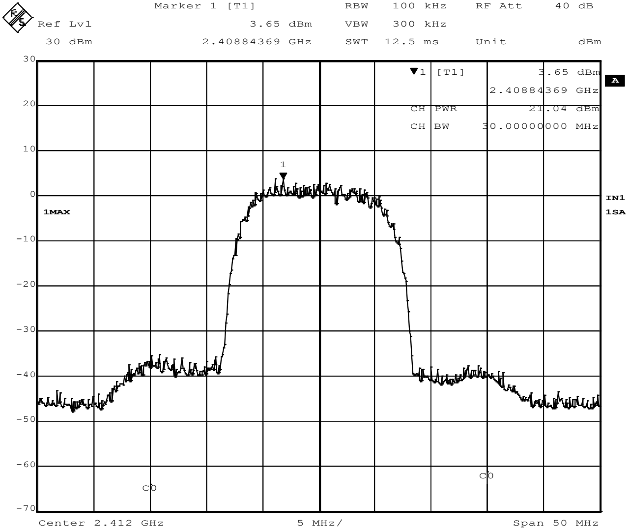
Figure 7 – Highest Measured Peak Output Power, 802.11b
