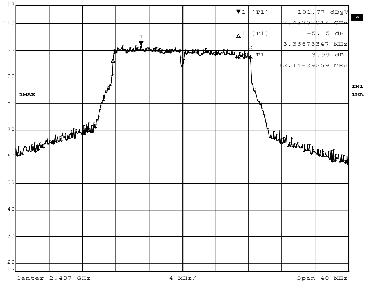
Figure 27 - 6dB Bandwidth, Mid Channel, 802.11g
