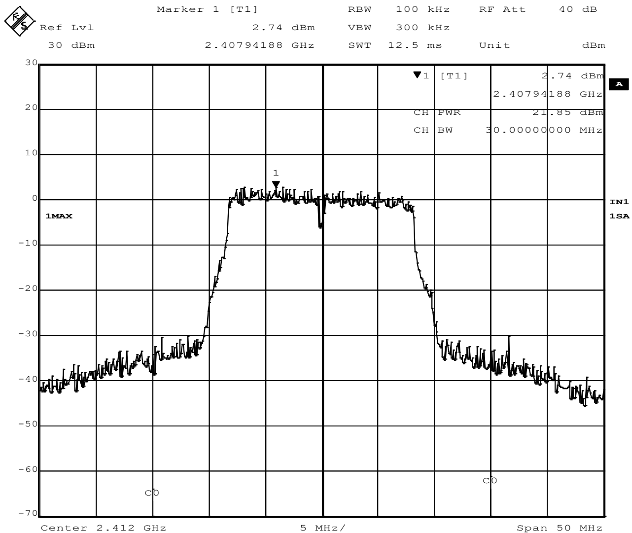
Figure 8 – Highest Measured Peak Output Power, 802.11g
