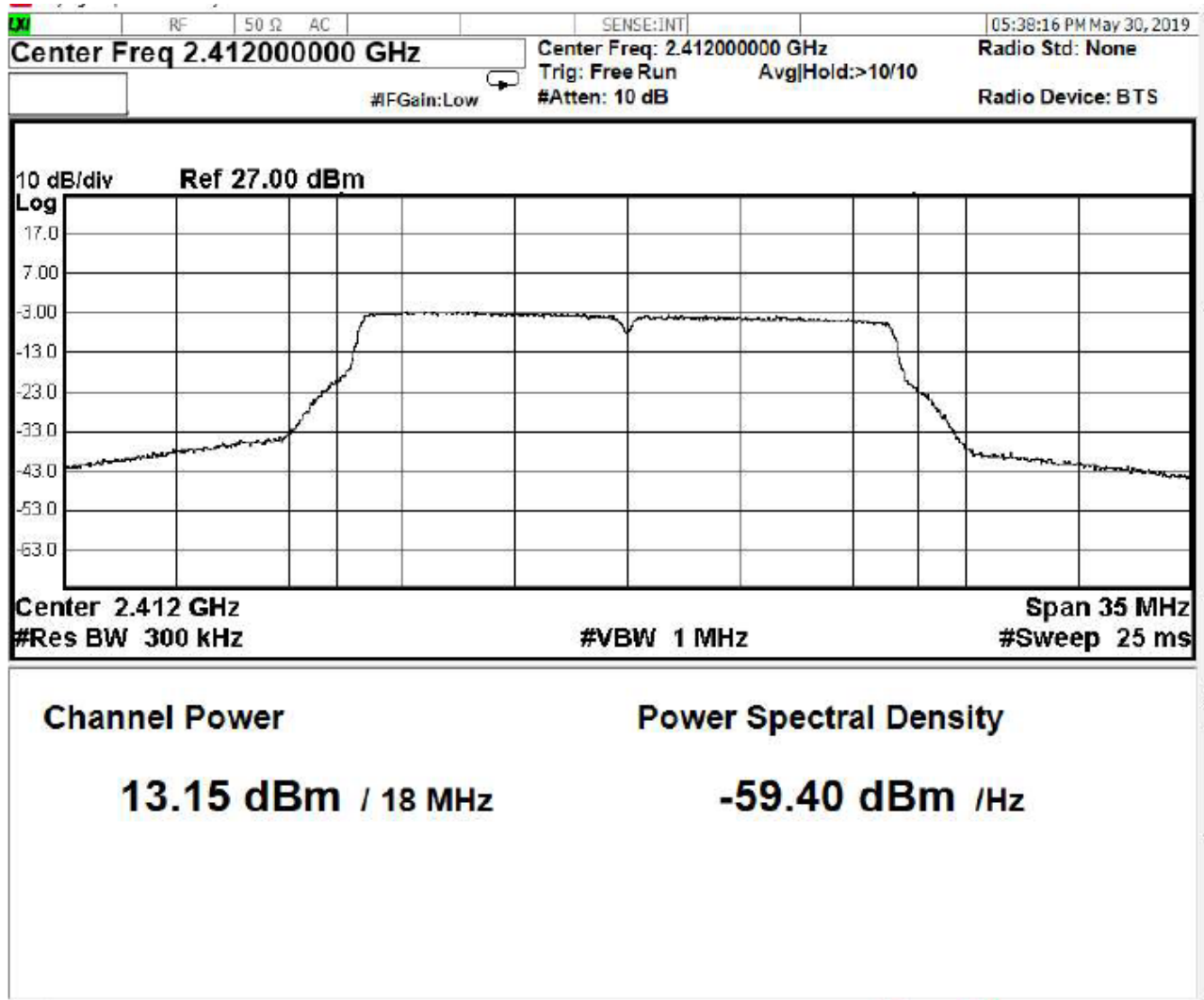
Figure 11 – Highest Measured Average Output Power, 802.11g
