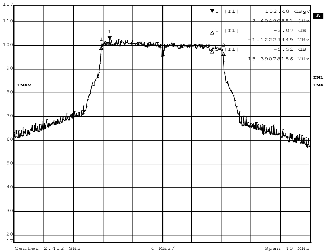
Figure 26 - 6dB Bandwidth, Low Channel, 802.11g
