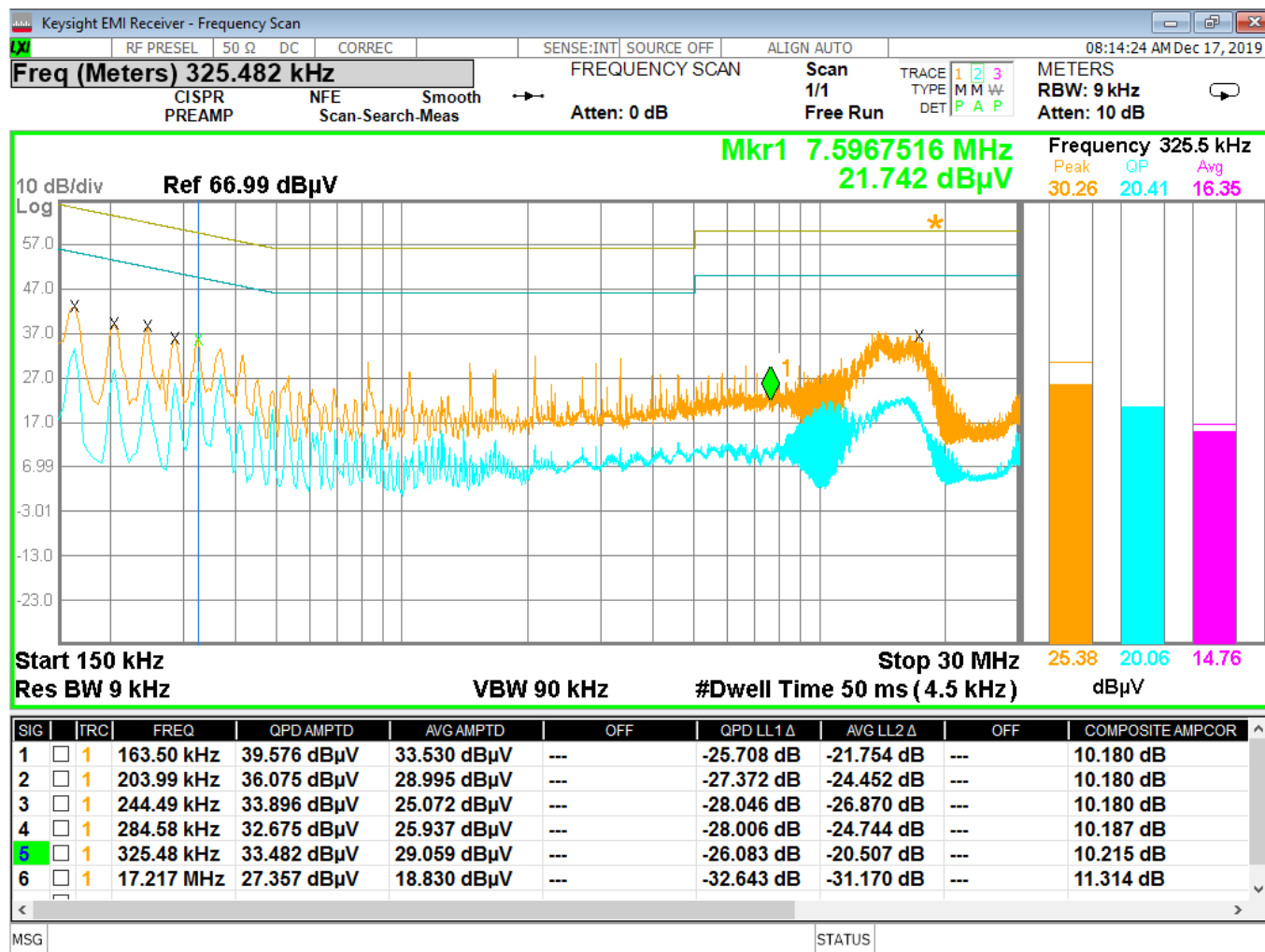
Figure 21 - Conducted Emissions Plot, Neutral
