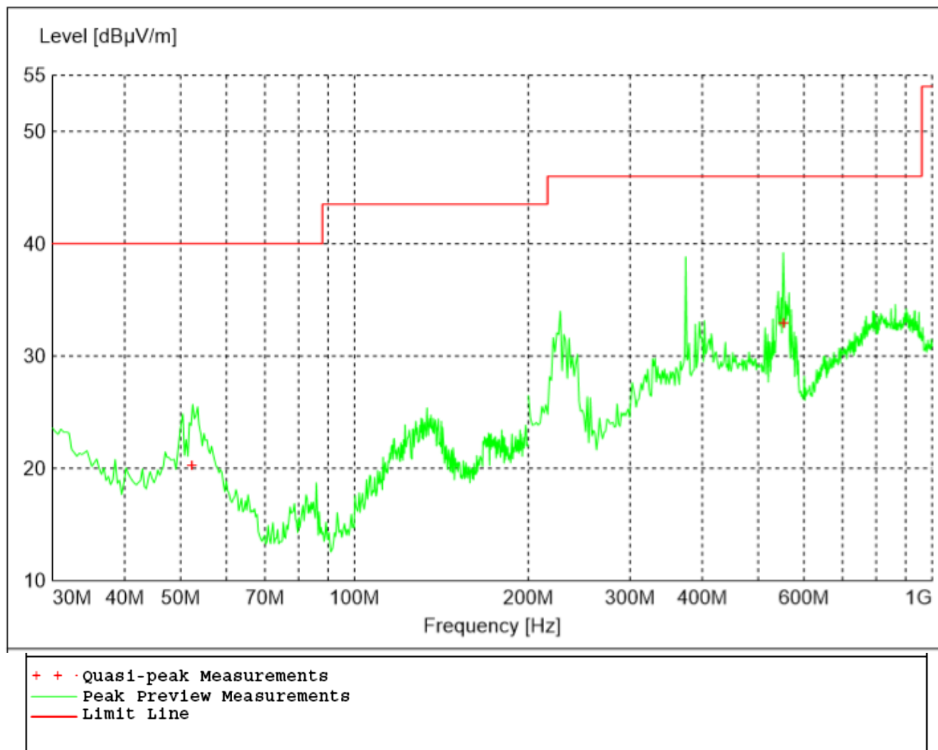
Figure 10 - Radiated Emissions Plot, GMSK
