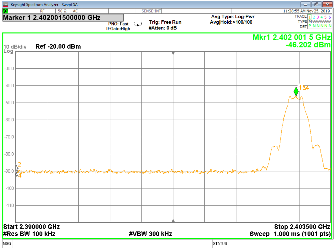
Figure 17 - Band-edge Measurement, Low Channel, Fundamental, Peak, GMSK
