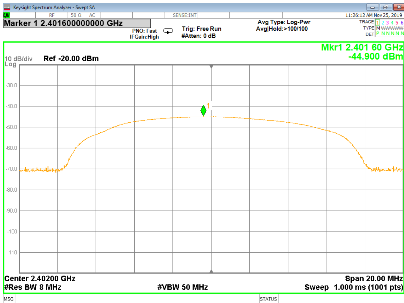
Figure 2 – Output Power, Low Channel, GMSK
