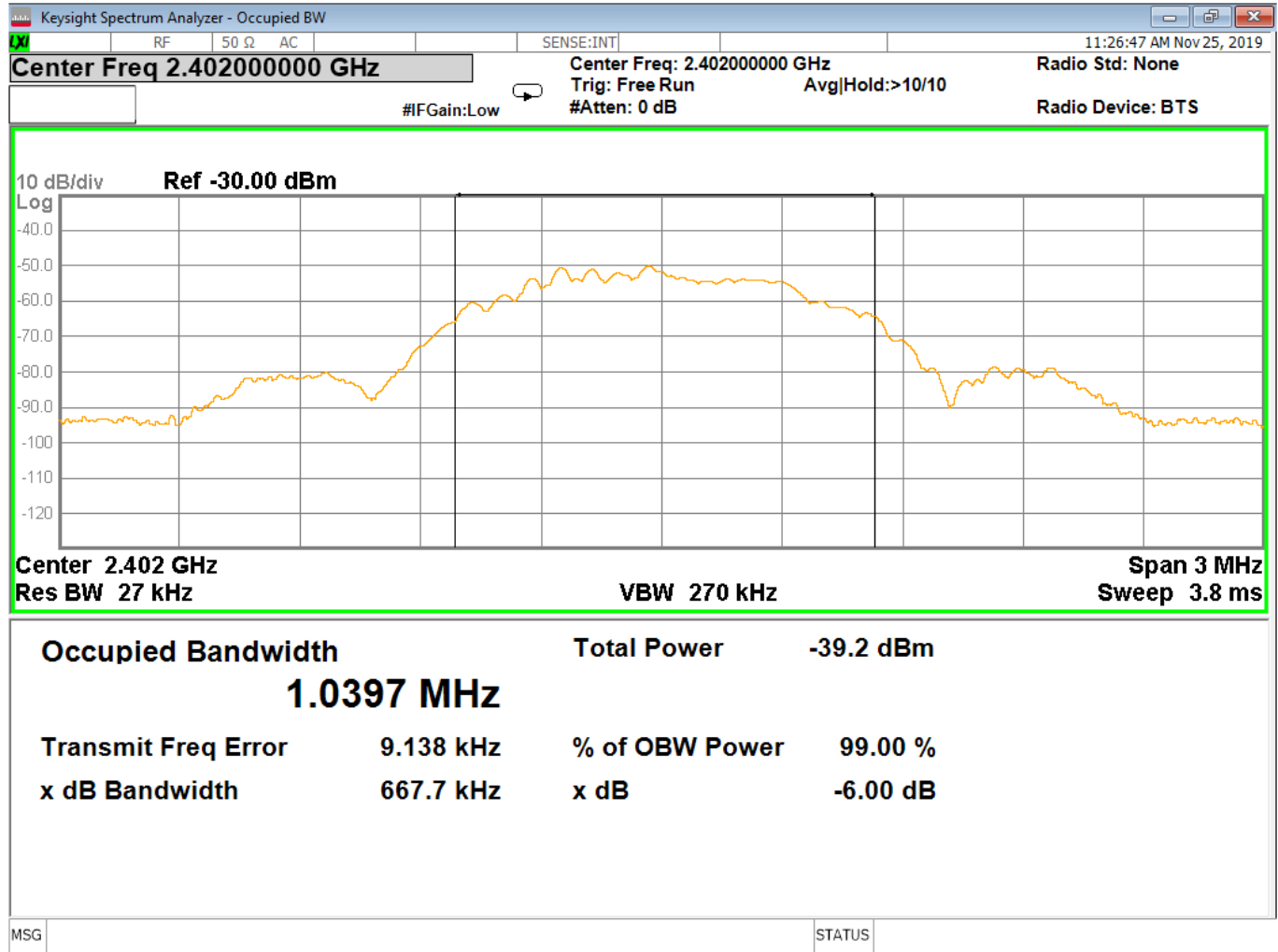
Figure 6 - Bandwidth, Low Channel, GMSK
