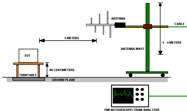
Figure 5 – Peak Output Power Measurements Test Setup
