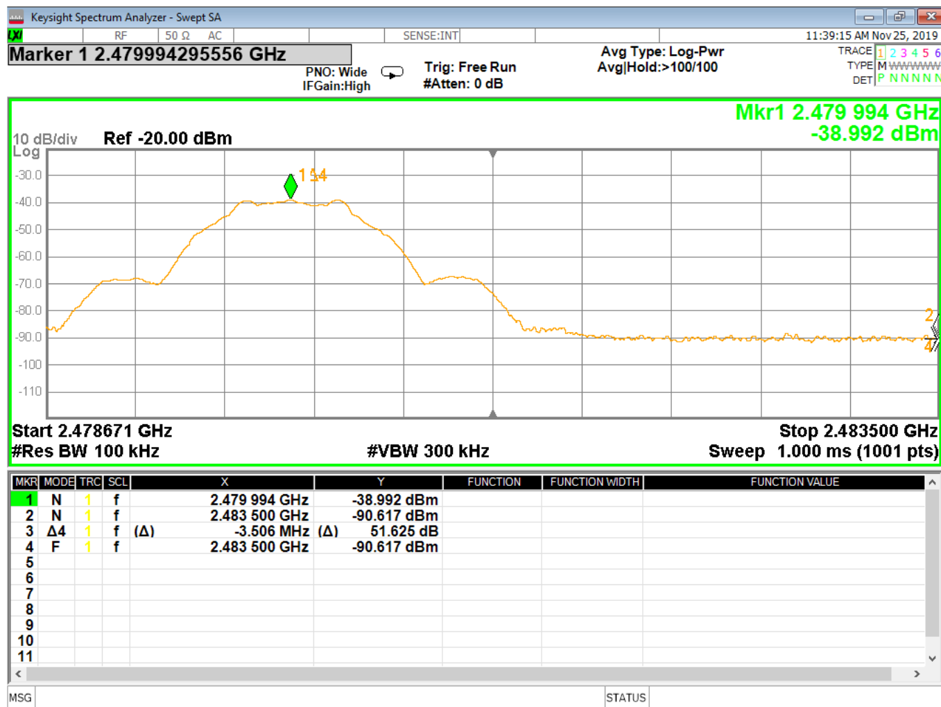
Figure 19 - Band-edge Measurement, High Channel, Fundamental, Peak, GMSK
