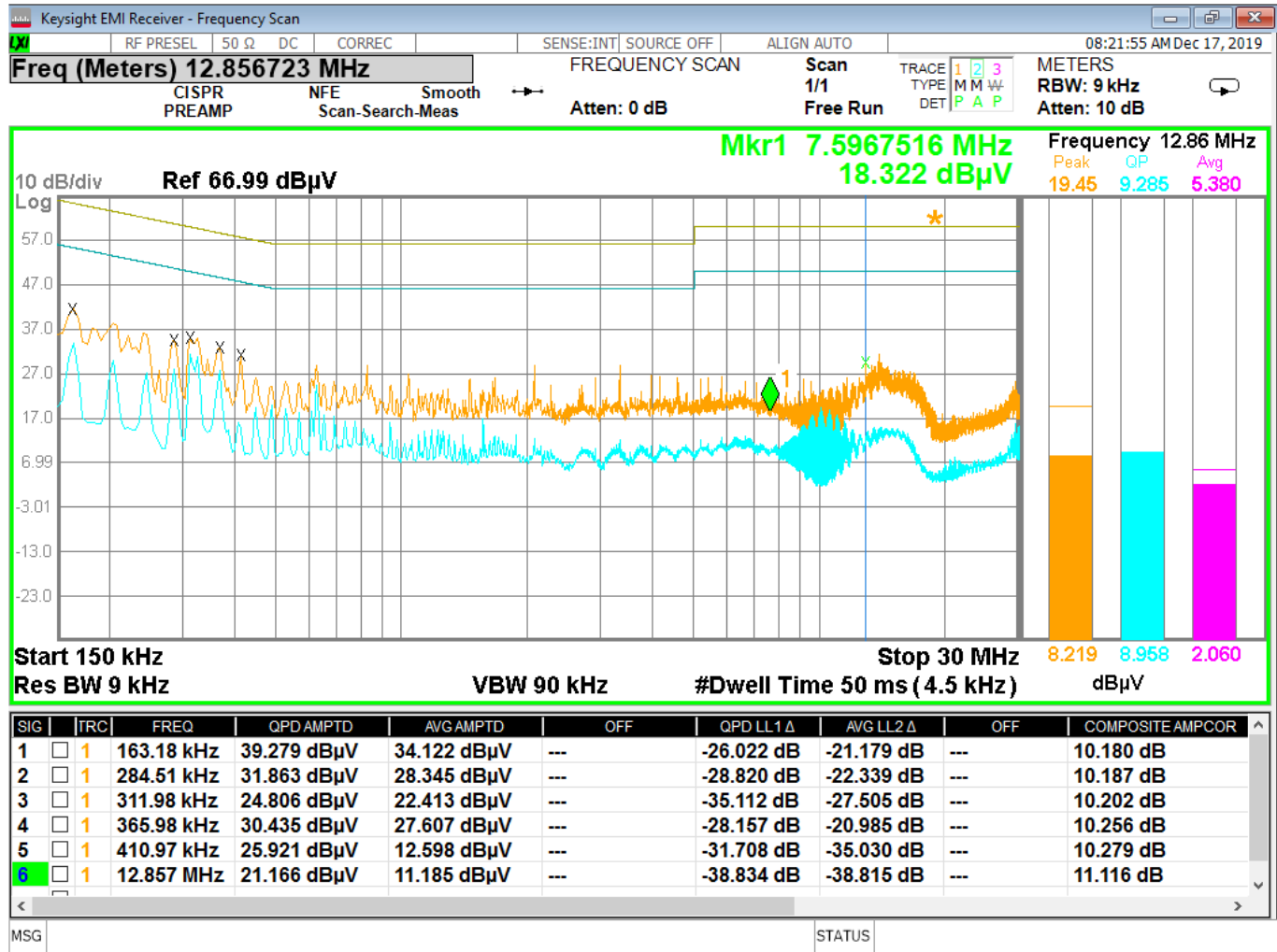
Figure 20 - Conducted Emissions Plot, Line
