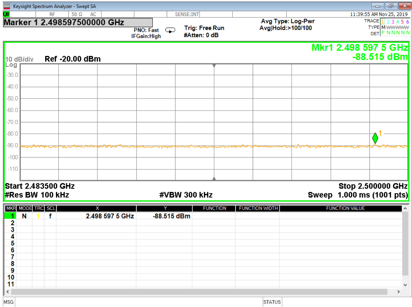
Figure 18 - Band-edge Measurement, High Channel, Restricted Frequency, Peak, GMSK
