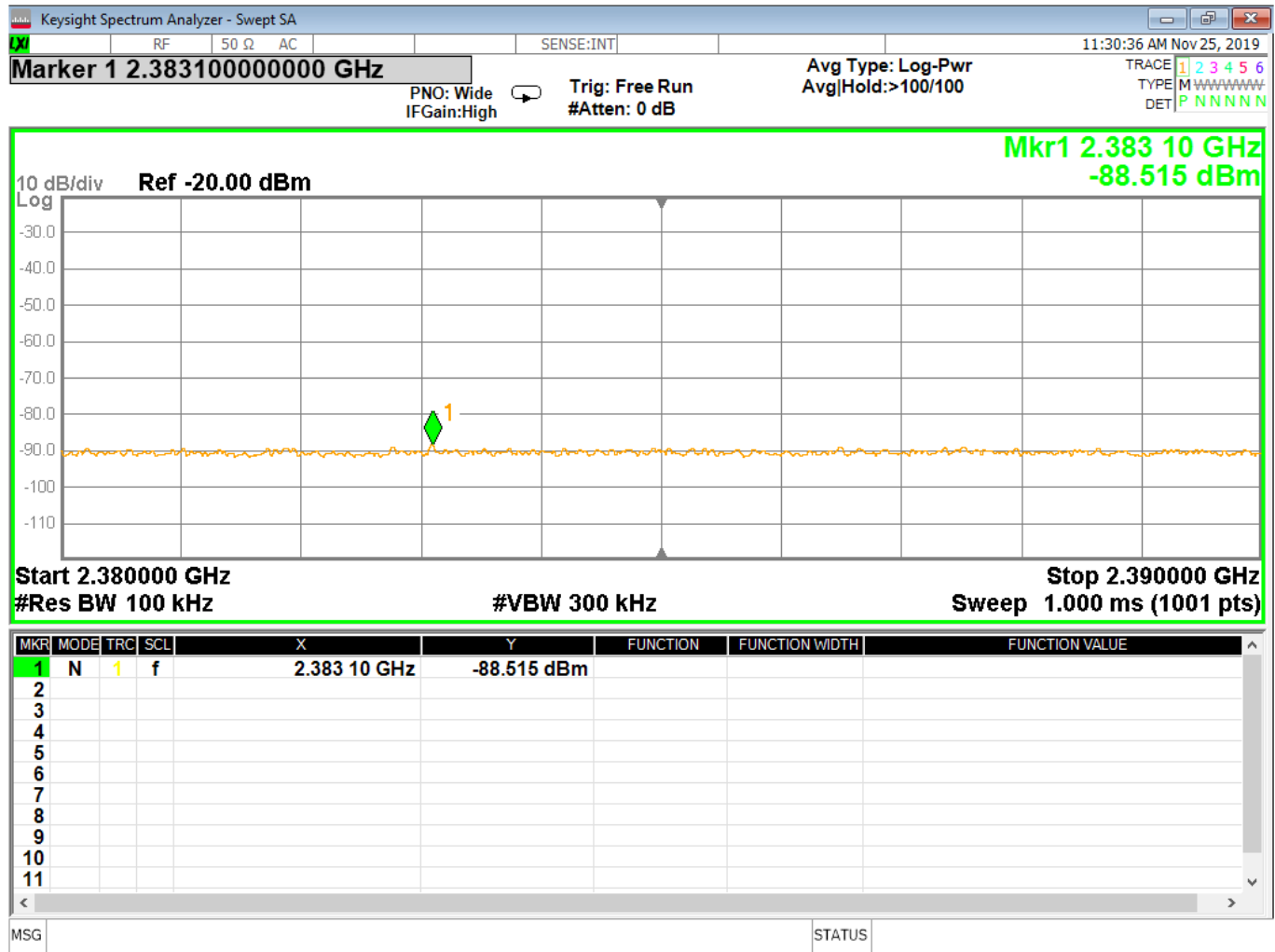
Figure 16 - Band-edge Measurement, Low Channel, Restricted Frequency, Peak, GMSK
