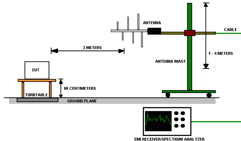
Figure 11 – Power Spectral Density Measurements Test Setup
