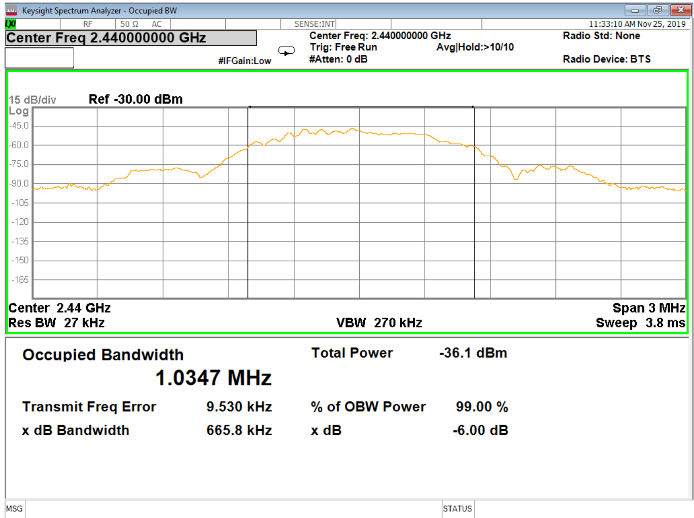
Figure 7 - Bandwidth, Mid Channel, GMSK
