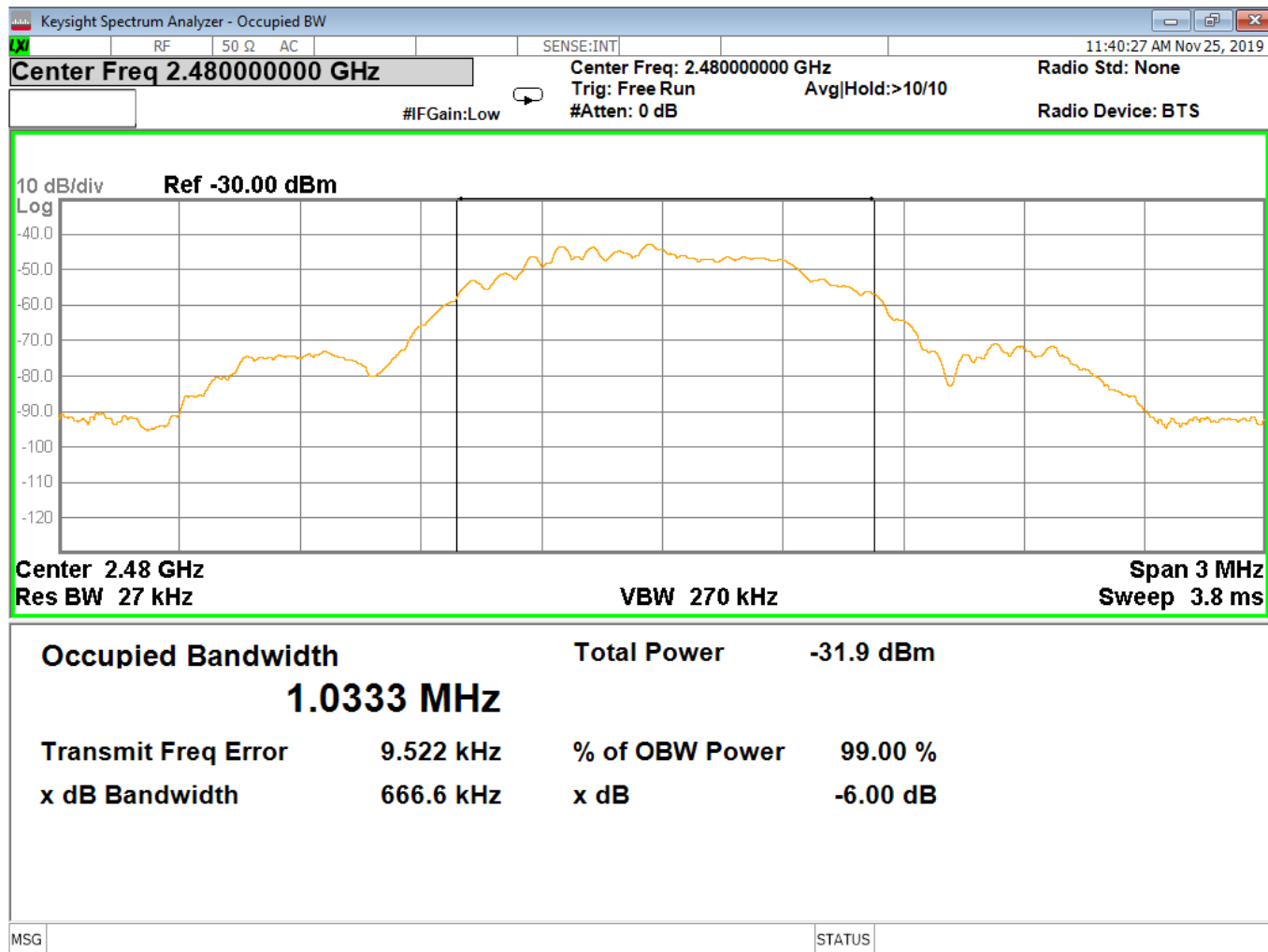
Figure 8 - Bandwidth, High Channel, GMSK
