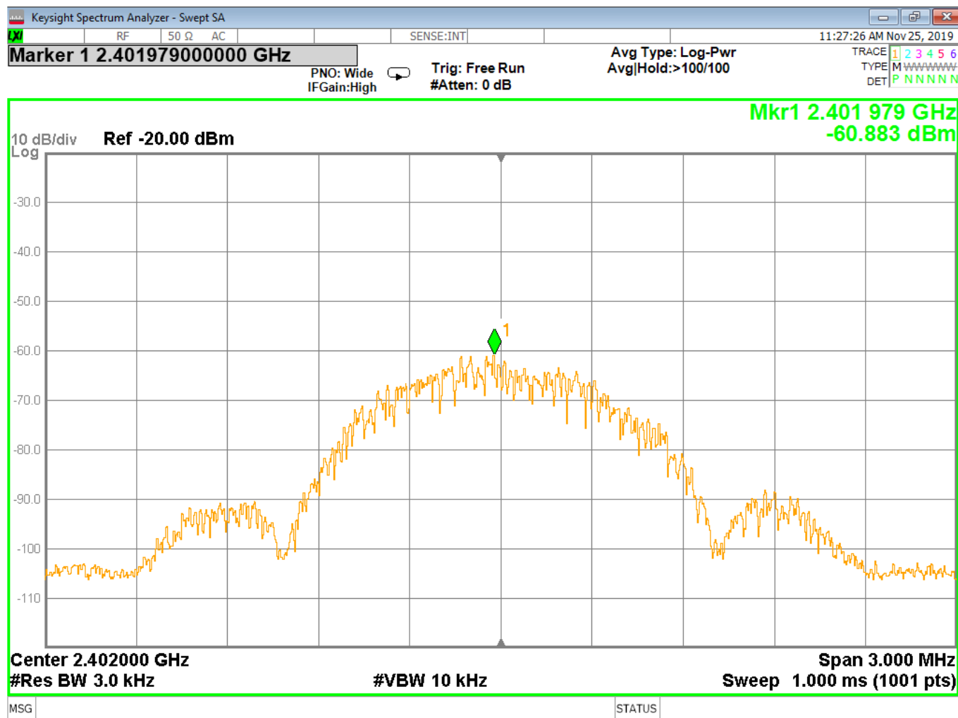
Figure 12 - Power Spectral Density, Low Channel, GMSK
