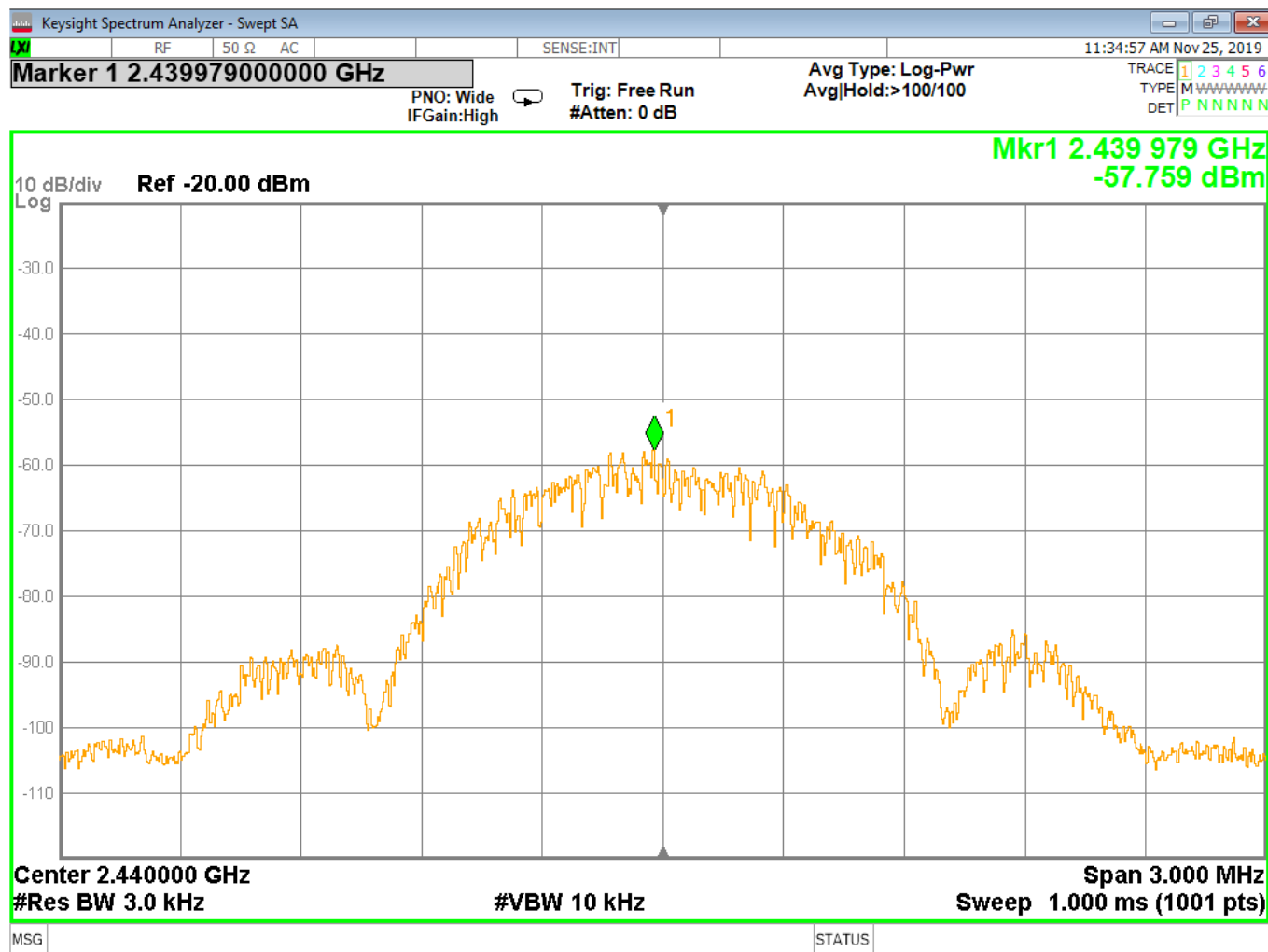
Figure 13 - Power Spectral Density, Mid Channel, GMSK
