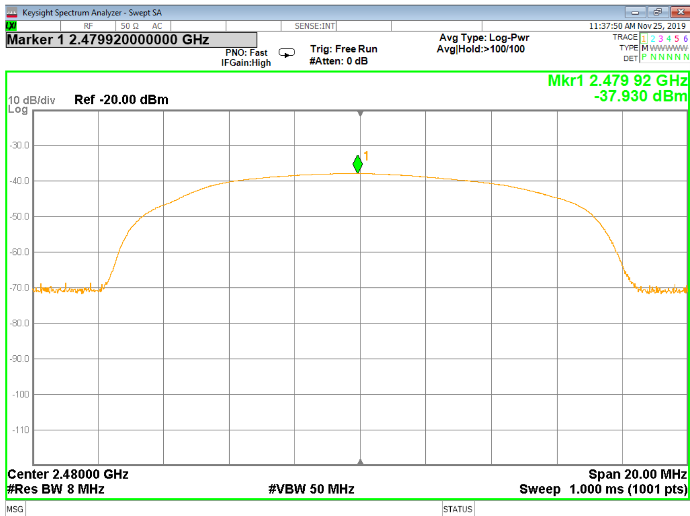
Figure 4 – Output Power, High Channel, GMSK
