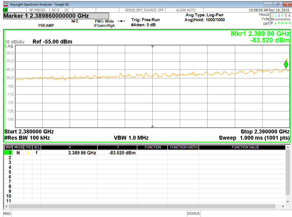
Figure 32 - Band-edge Measurement, Low Channel, Restricted Frequency, Peak
