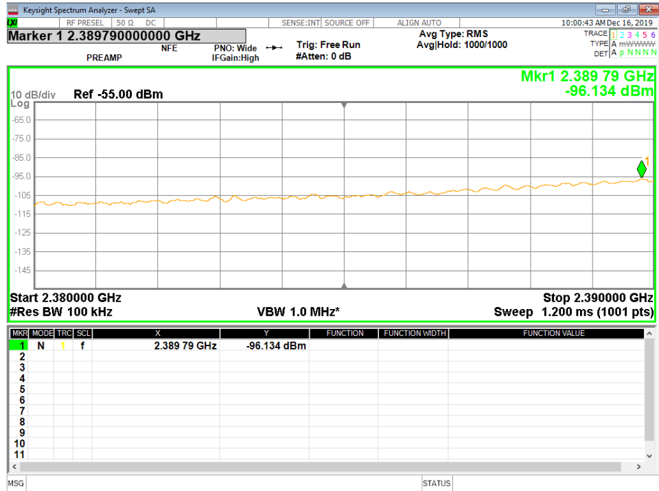
Figure 42 - Band-edge Measurement, Low Channel, Restricted Frequency, Average
