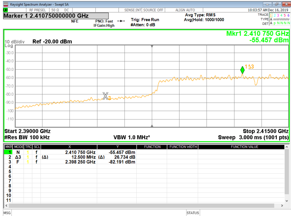
Figure 43 - Band-edge Measurement, Low Channel, Fundamental, Average
