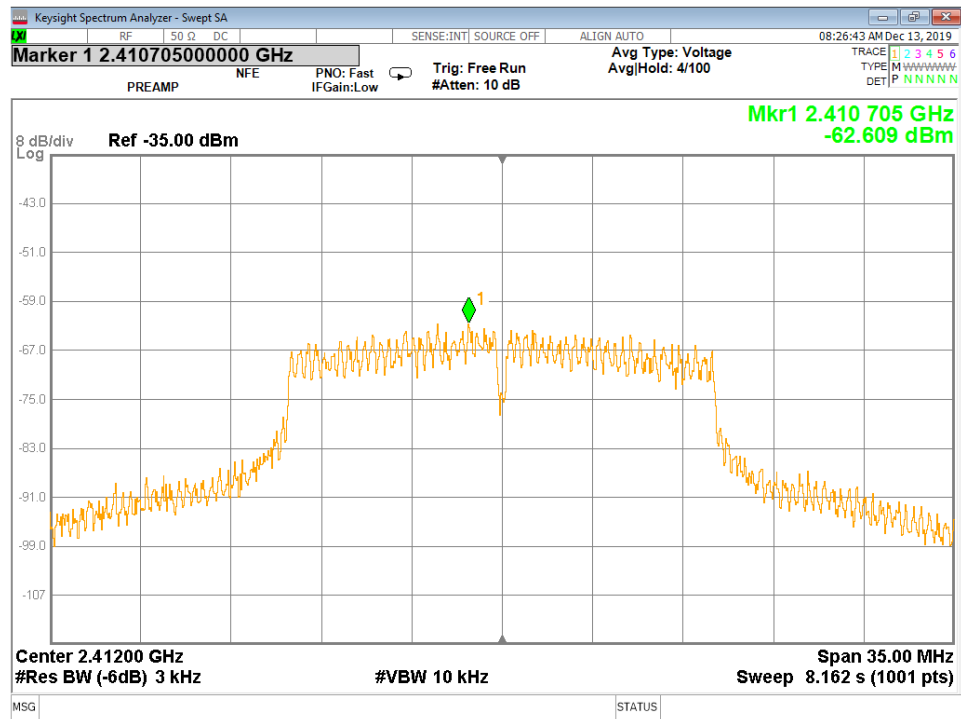
Figure 52 - Power Spectral Density, Low Channel, 802.11g
