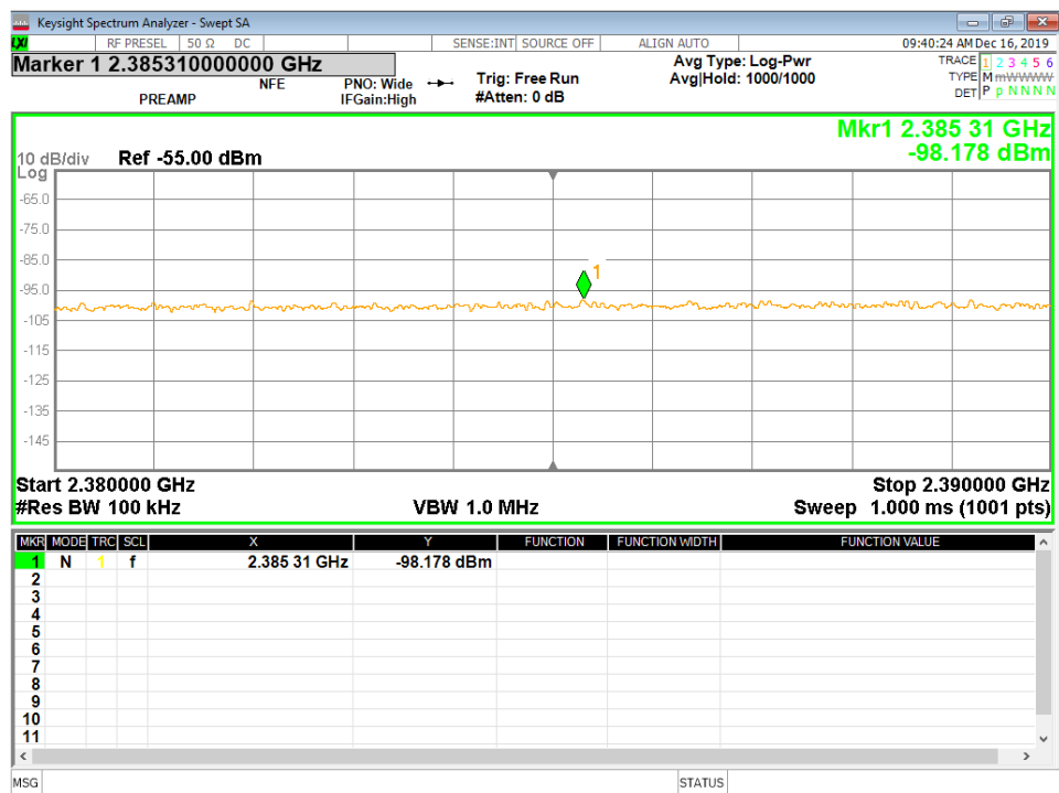
Figure 24 - Band-edge Measurement, Low Channel, Restricted Frequency, Peak
