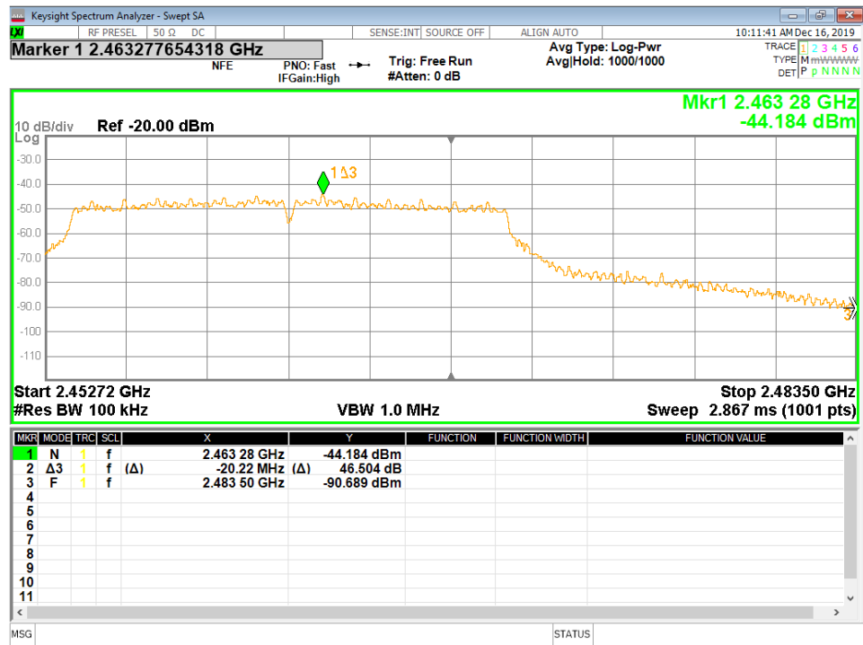
Figure 37 - Band-edge Measurement, High Channel, Fundamental, Peak
