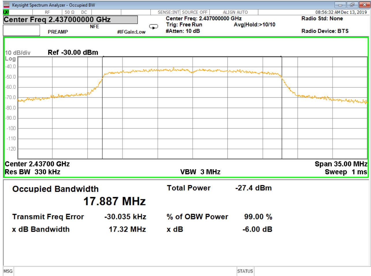
Figure 21 - 99% Occupied Bandwidth and 6dB Bandwidth, Mid Channel, 802.11n
