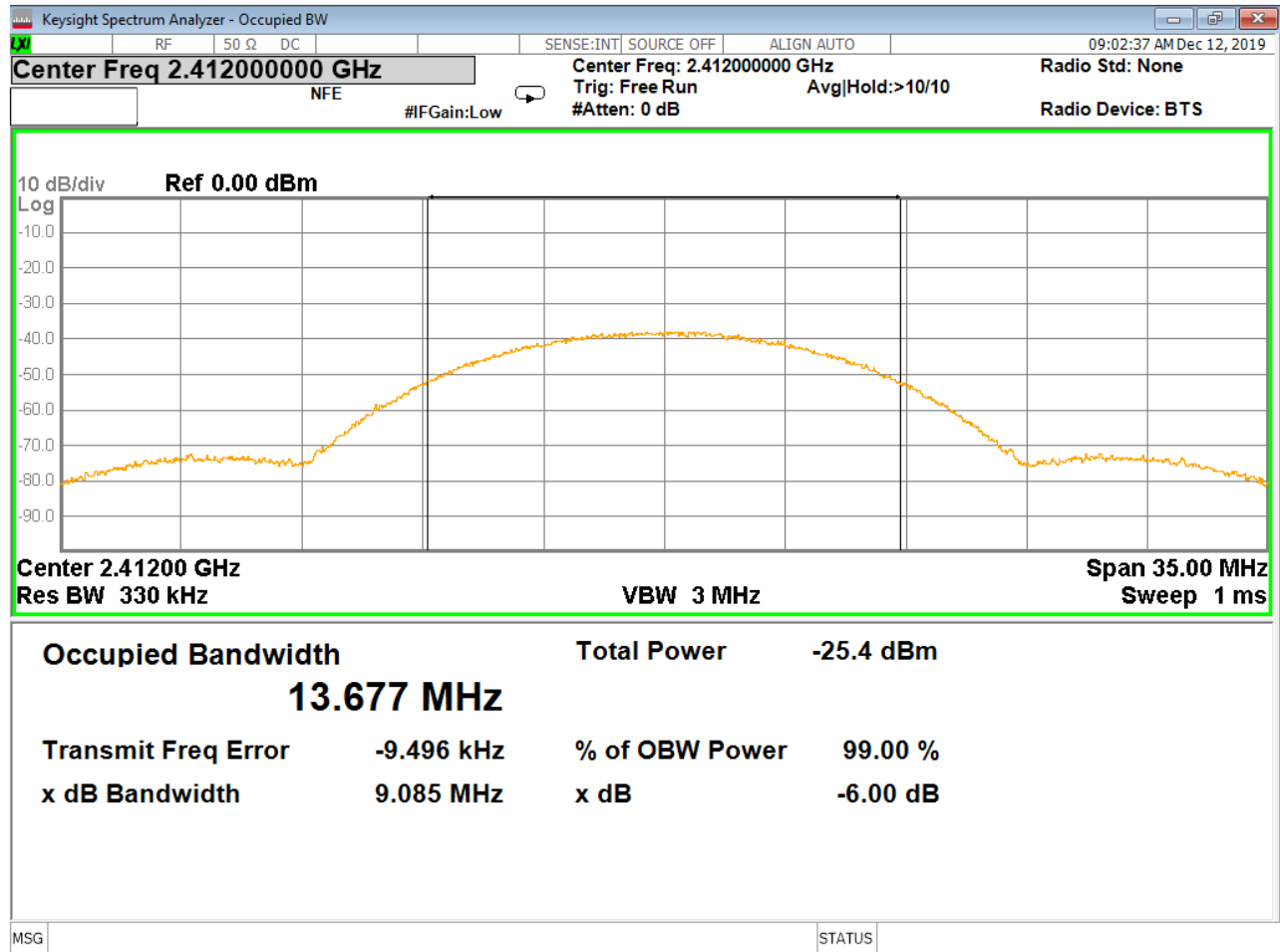
Figure 14 - 99% Occupied Bandwidth and 6dB Bandwidth, Low Channel, 802.11b
