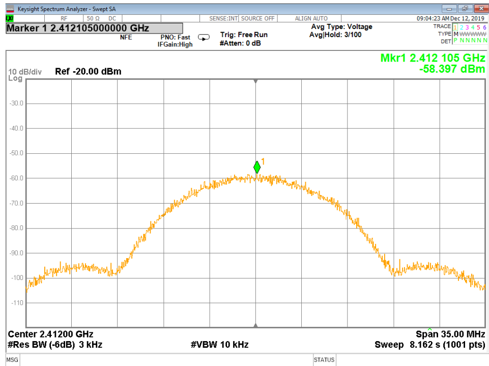
Figure 49 - Power Spectral Density, Low Channel, 802.11b
