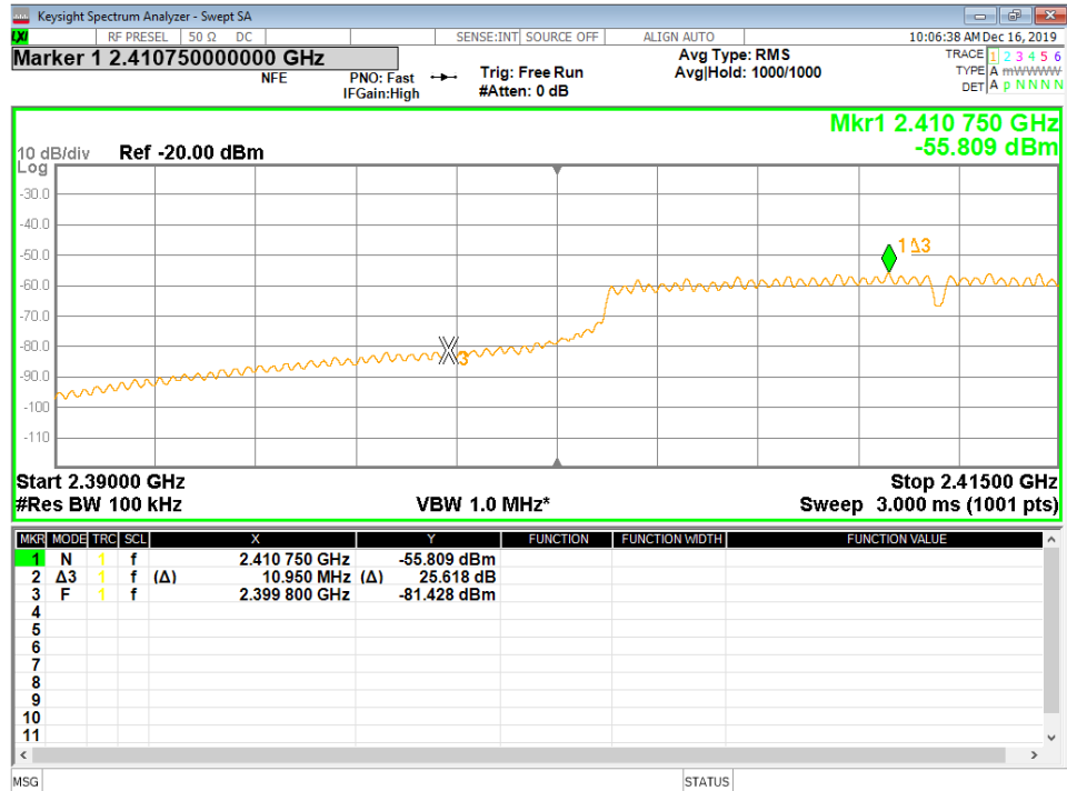
Figure 35 - Band-edge Measurement, Low Channel, Fundamental, Average
