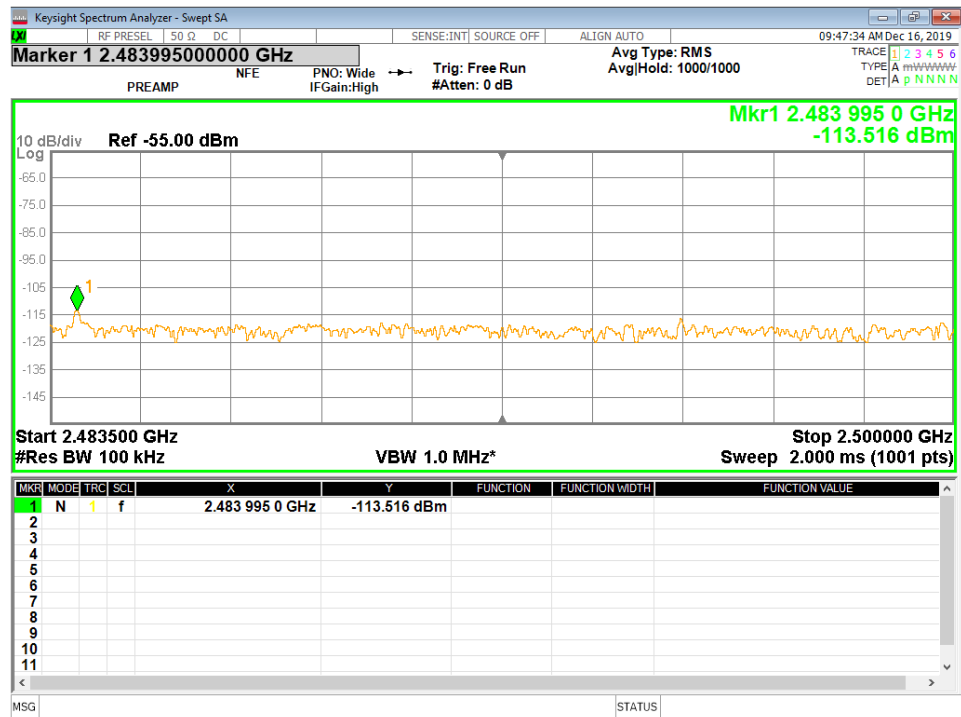
Figure 30 - Band-edge Measurement, High Channel, Restricted Frequency, Average
