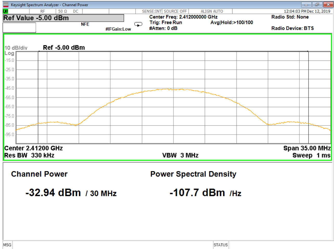
Figure 8 – Highest Average Output Power, 802.11b
