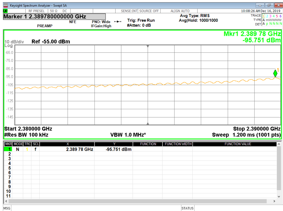
Figure 34 - Band-edge Measurement, Low Channel, Restricted Frequency, Average
