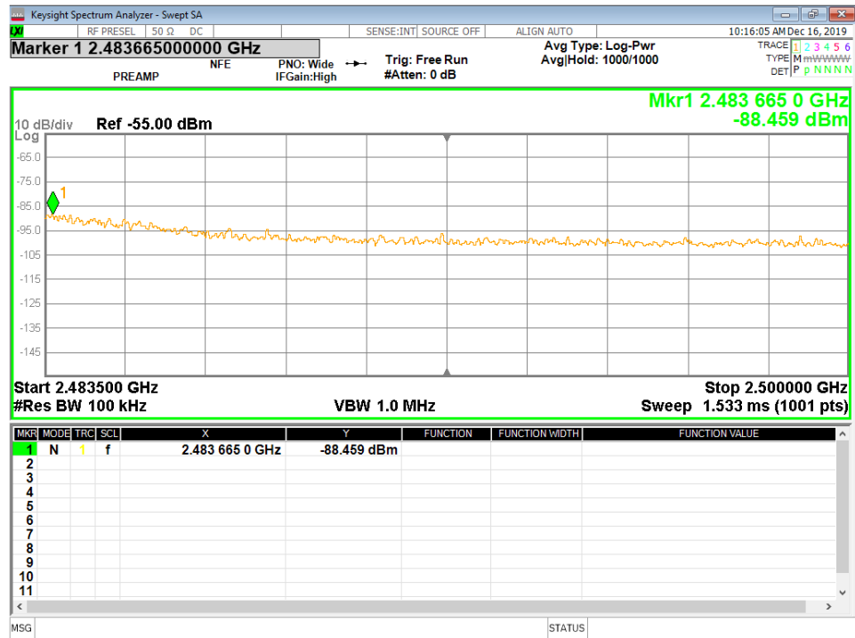
Figure 44 - Band-edge Measurement, High Channel, Restricted Frequency, Peak
