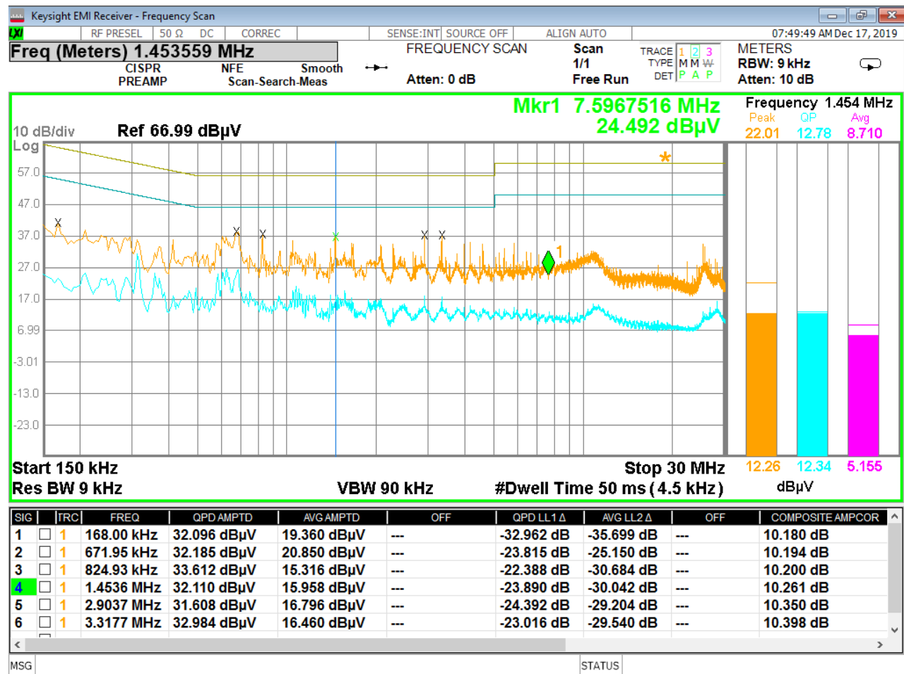
Figure 60 - Conducted Emissions Plot, Line, Dual USB
