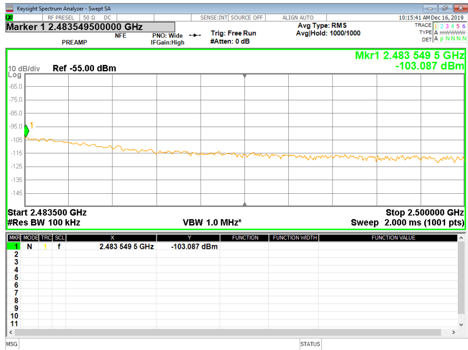
Figure 46 - Band-edge Measurement, High Channel, Restricted Frequency, Average
