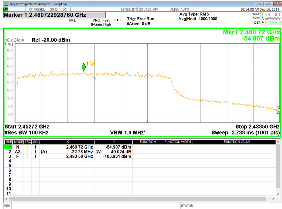
Figure 47 - Band-edge Measurement, High Channel, Fundamental, Average
