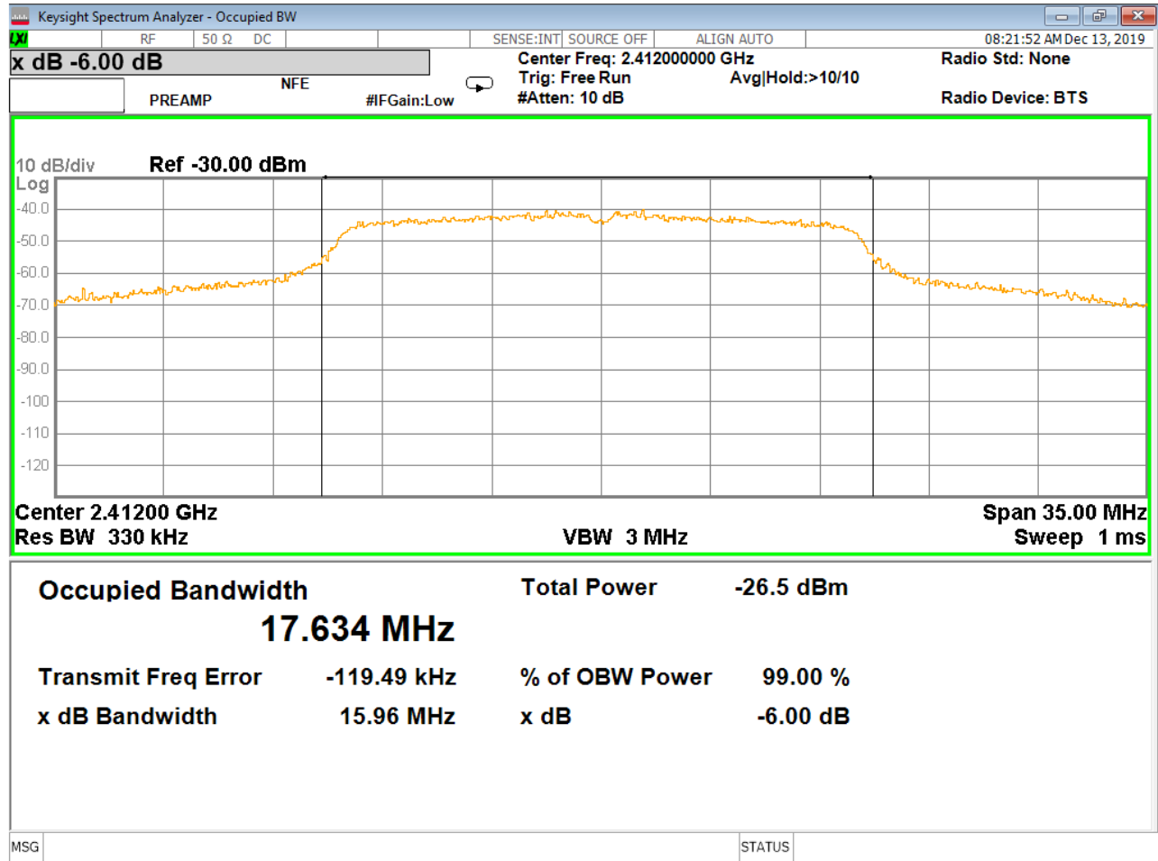
Figure 17 - 99% Occupied Bandwidth and 6dB Bandwidth, Low Channel, 802.11g
