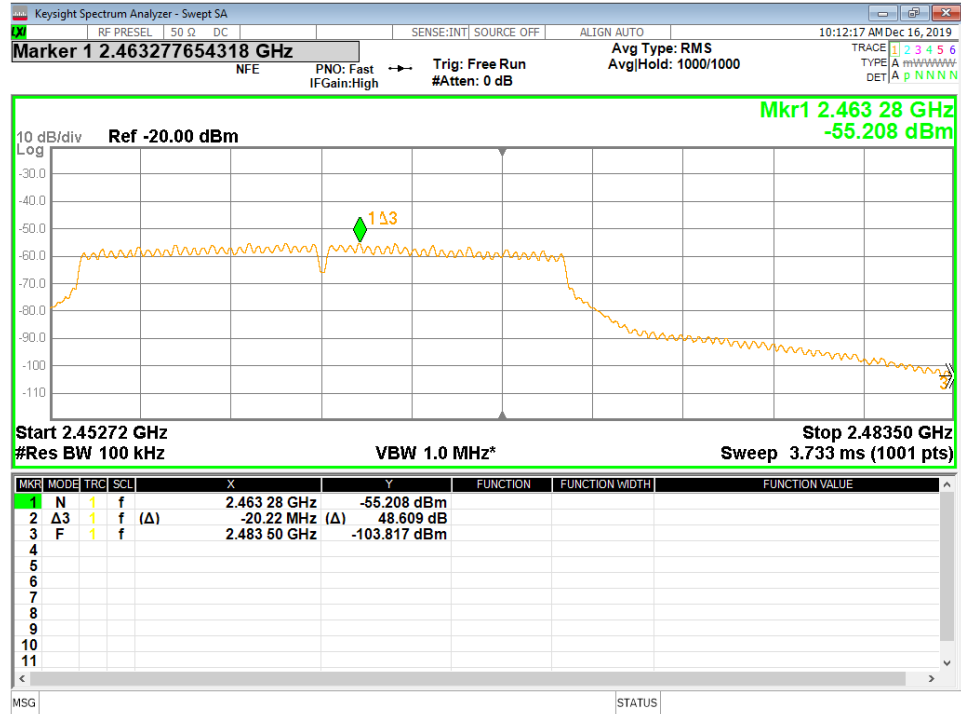
Figure 39 - Band-edge Measurement, High Channel, Fundamental, Average
