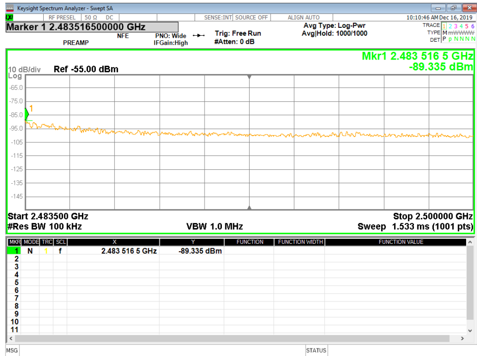
Figure 36 - Band-edge Measurement, High Channel, Restricted Frequency, Peak
