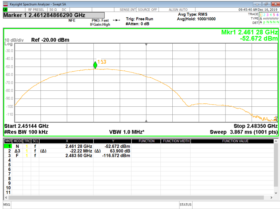
Figure 31 - Band-edge Measurement, High Channel, Fundamental, Average
