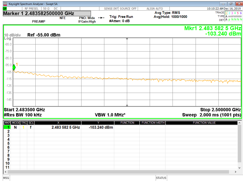
Figure 38 - Band-edge Measurement, High Channel, Restricted Frequency, Average
