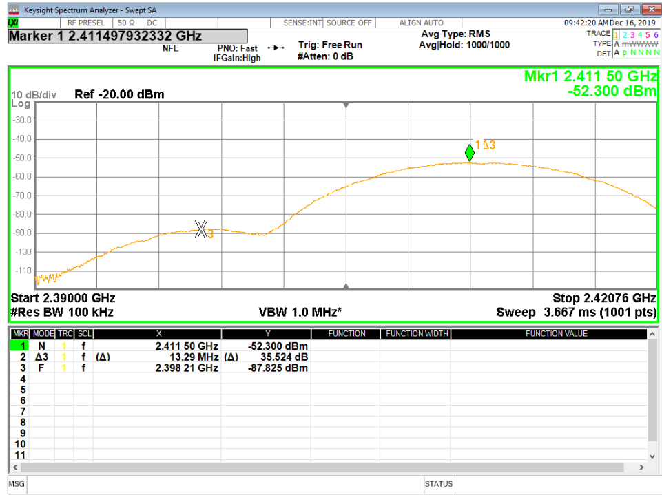
Figure 27 - Band-edge Measurement, Low Channel, Fundamental, Average
