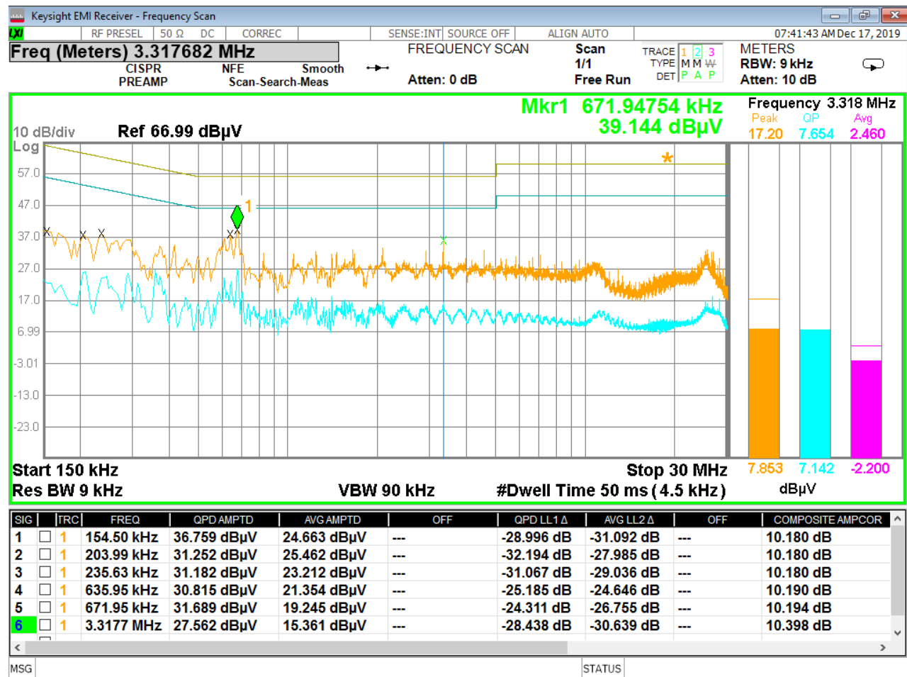
. Figure 61 - Conducted Emissions Plot, Neutral, Dual USB
