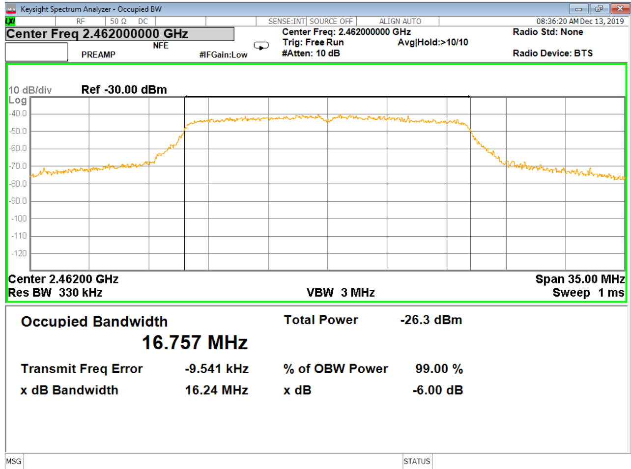
Figure 19 - 99% Occupied Bandwidth and 6dB Bandwidth, High Channel, 802.11g
