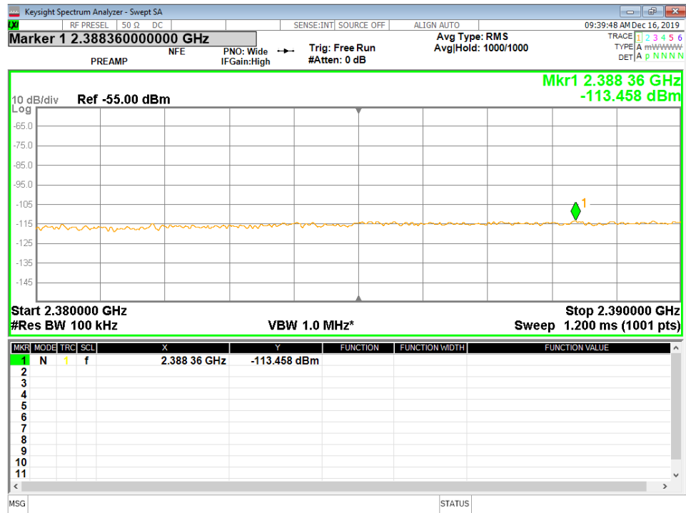
Figure 26 - Band-edge Measurement, Low Channel, Restricted Frequency, Average
