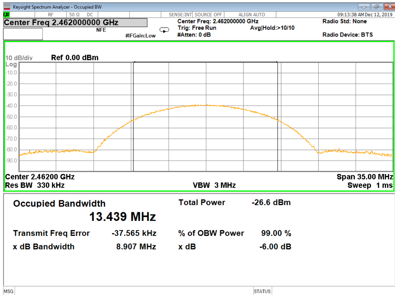
Figure 16 - 99% Occupied Bandwidth and 6dB Bandwidth, High Channel, 802.11b
