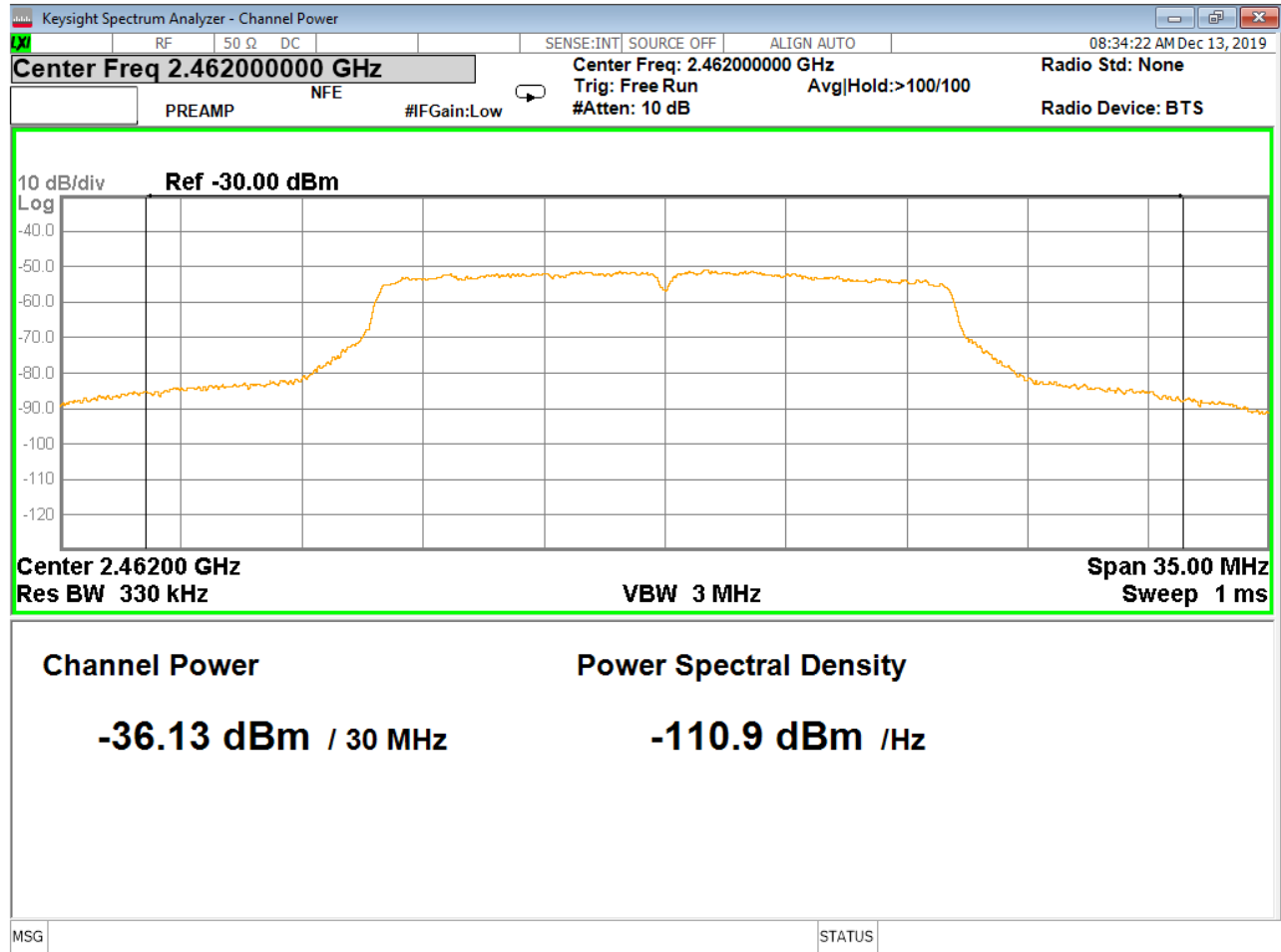
Figure 10 – Highest Average Output Power, 802.11g
