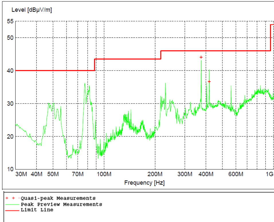
Figure 2 - Radiated Emissions Plot, Receive, 30-1G
