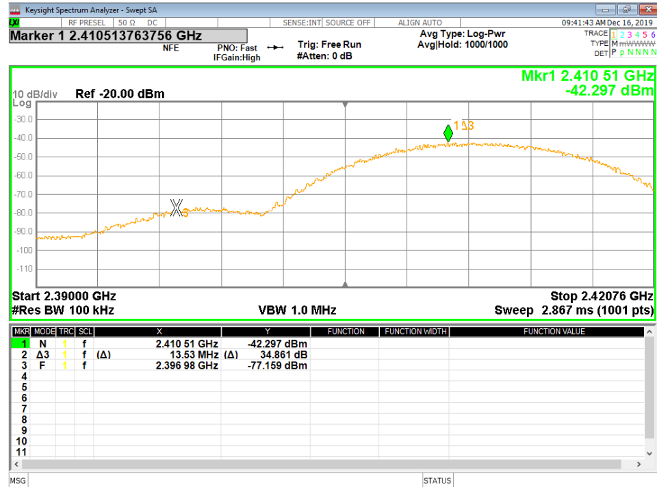
Figure 25 - Band-edge Measurement, Low Channel, Fundamental, Peak
