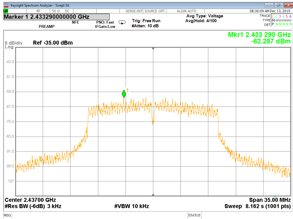
Figure 53 - Power Spectral Density, Mid Channel, 802.11g
