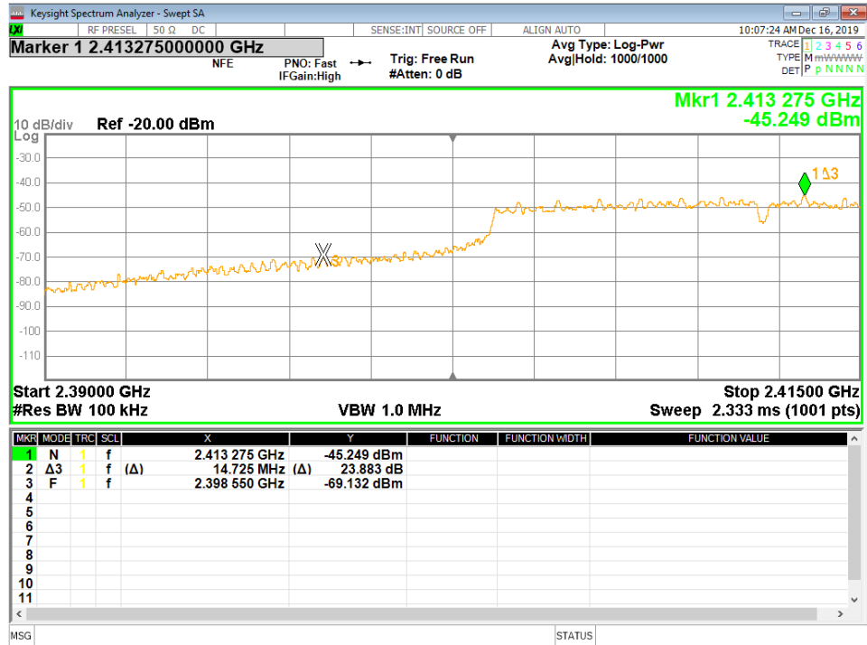
Figure 33 - Band-edge Measurement, Low Channel, Fundamental, Peak
