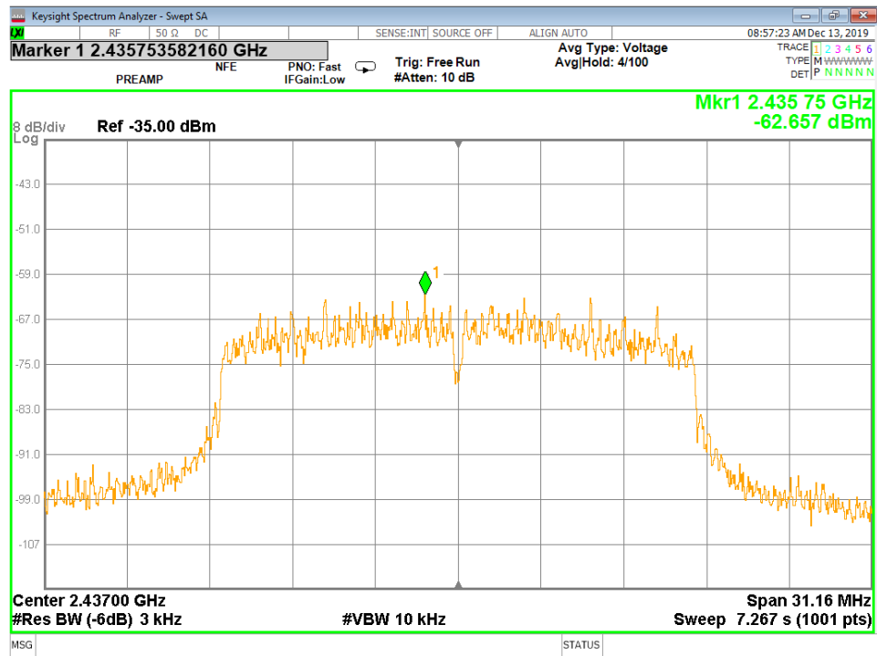
Figure 56 - Power Spectral Density, Mid Channel, 802.11n
