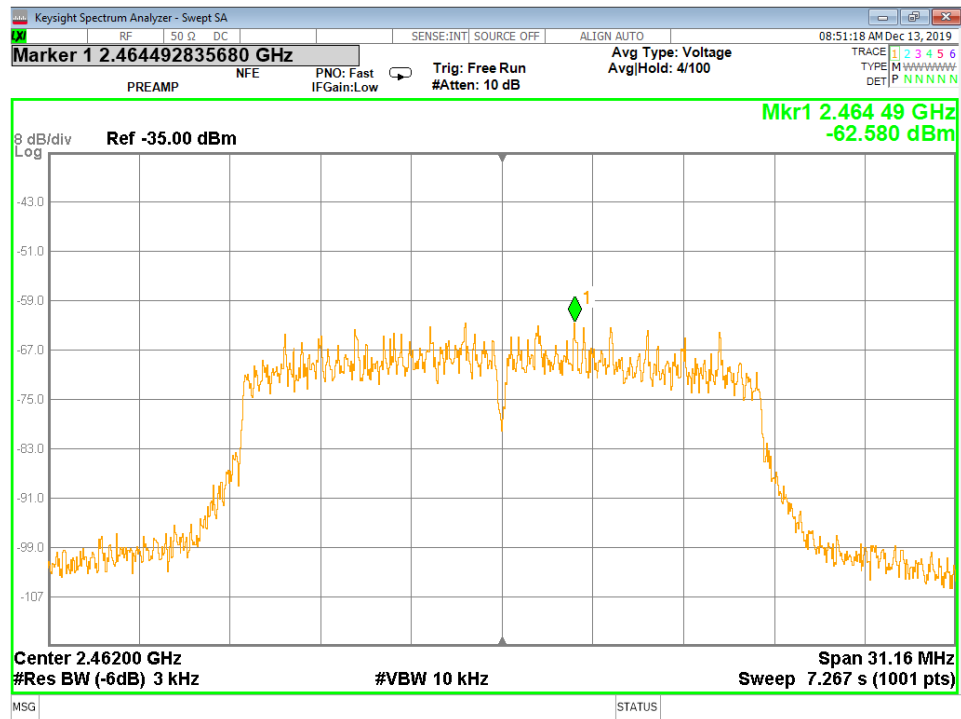
Figure 57 - Power Spectral Density, High Channel, 802.11n
