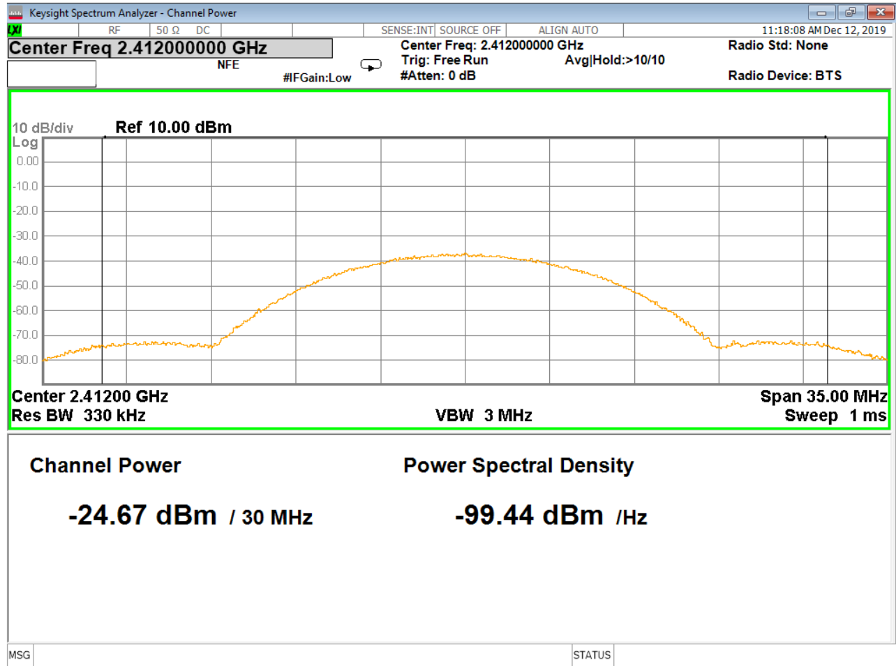
Figure 7 – Highest Peak Output Power, 802.11b
