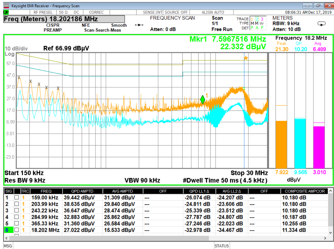
. Figure 59 - Conducted Emissions Plot, Neutral, Single USB
