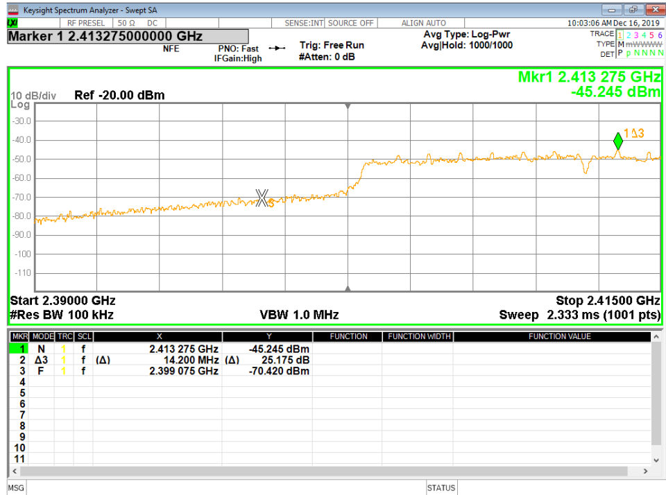
Figure 41 - Band-edge Measurement, Low Channel, Fundamental, Peak
