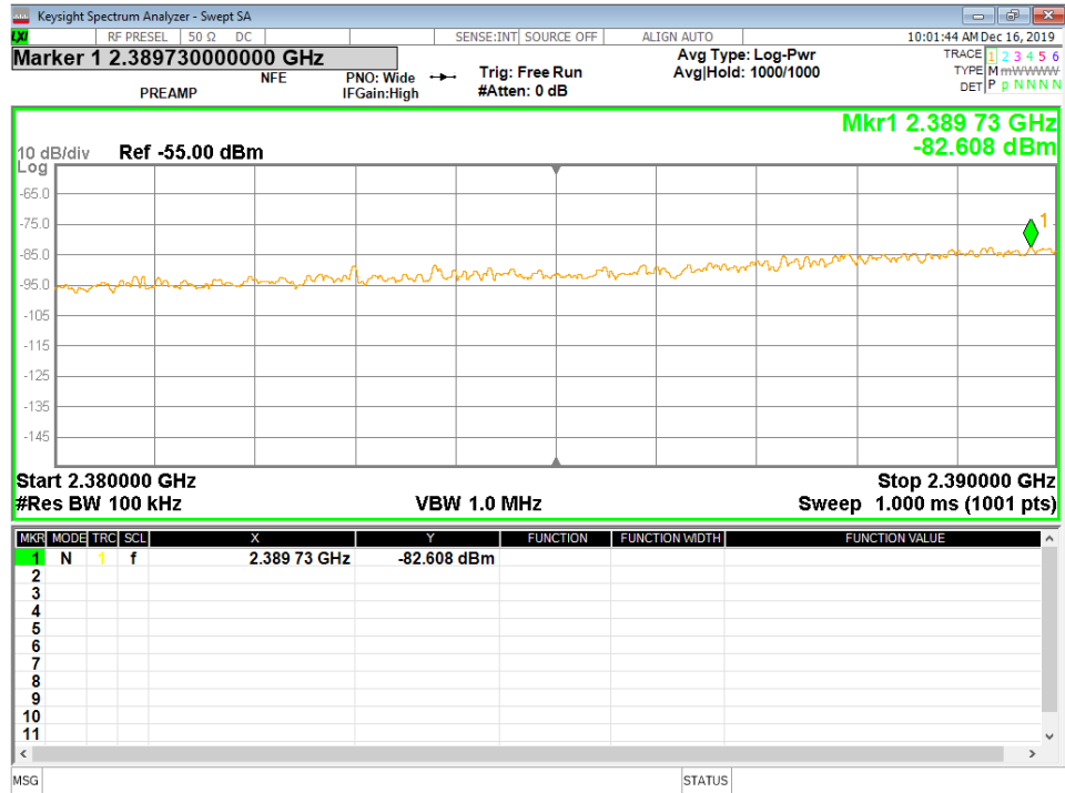
Figure 40 - Band-edge Measurement, Low Channel, Restricted Frequency, Peak
