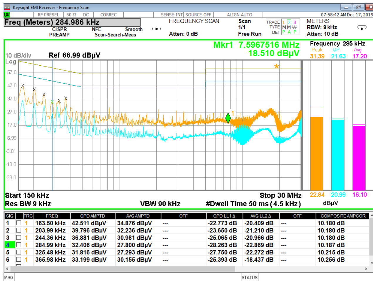
Figure 58 - Conducted Emissions Plot, Line, Single USB
