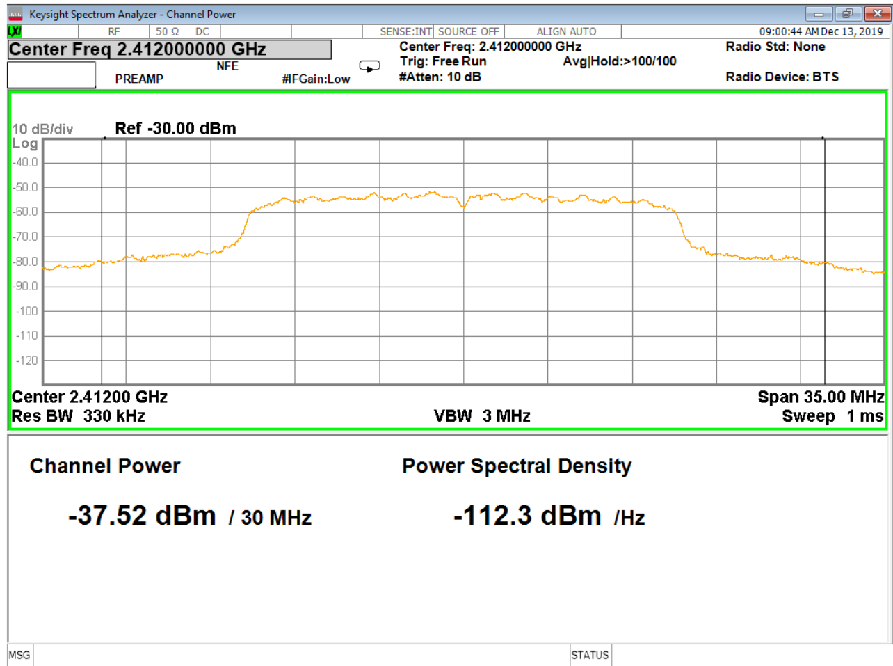
Figure 12 – Highest Average Output Power, 802.11n
