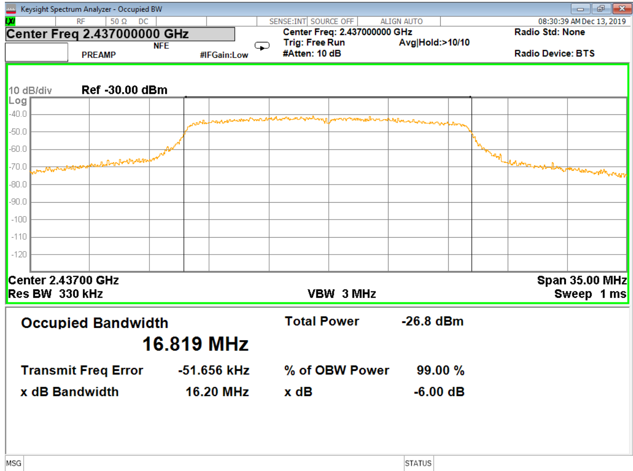
Figure 18 - 99% Occupied Bandwidth and 6dB Bandwidth, Mid Channel, 802.11g
