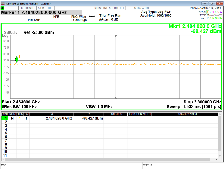
Figure 28 - Band-edge Measurement, High Channel, Restricted Frequency, Peak
