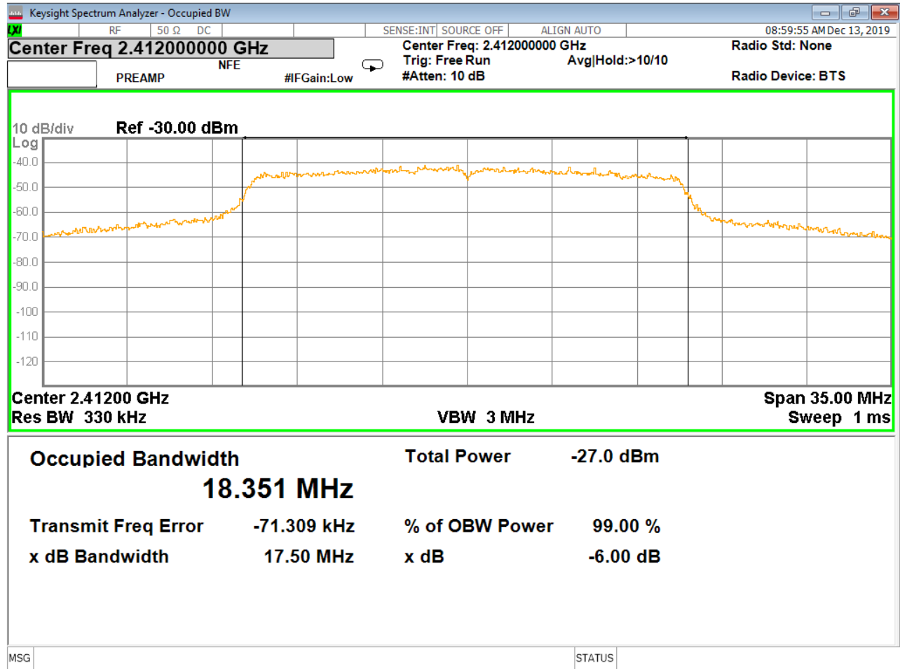
Figure 20 - 99% Occupied Bandwidth and 6dB Bandwidth, Low Channel, 802.11n
