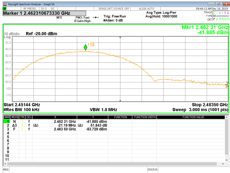
Figure 29 - Band-edge Measurement, High Channel, Fundamental, Peak
