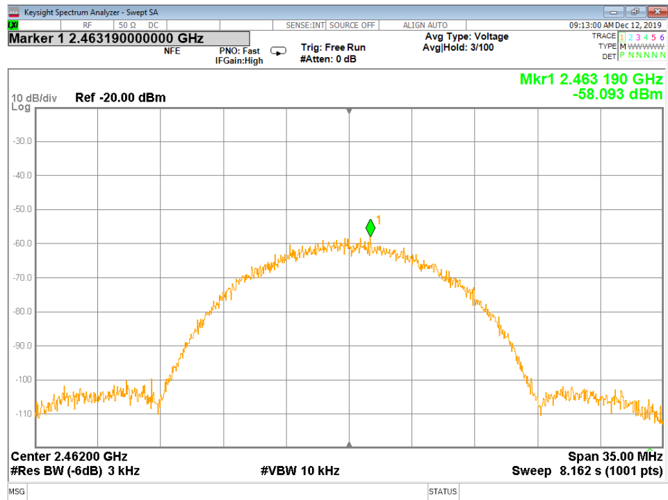
Figure 51 - Power Spectral Density, High Channel, 802.11b
