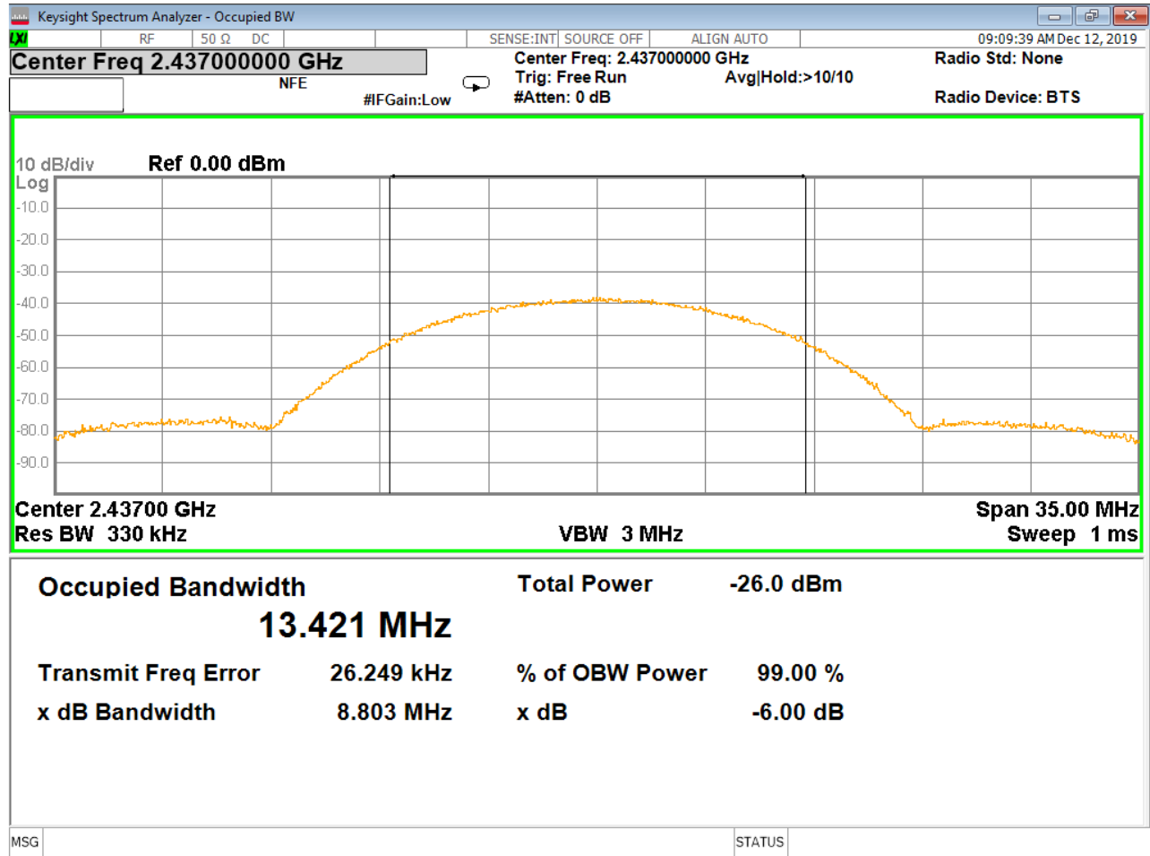
Figure 15 - 99% Occupied Bandwidth and 6dB Bandwidth, Mid Channel, 802.11b
