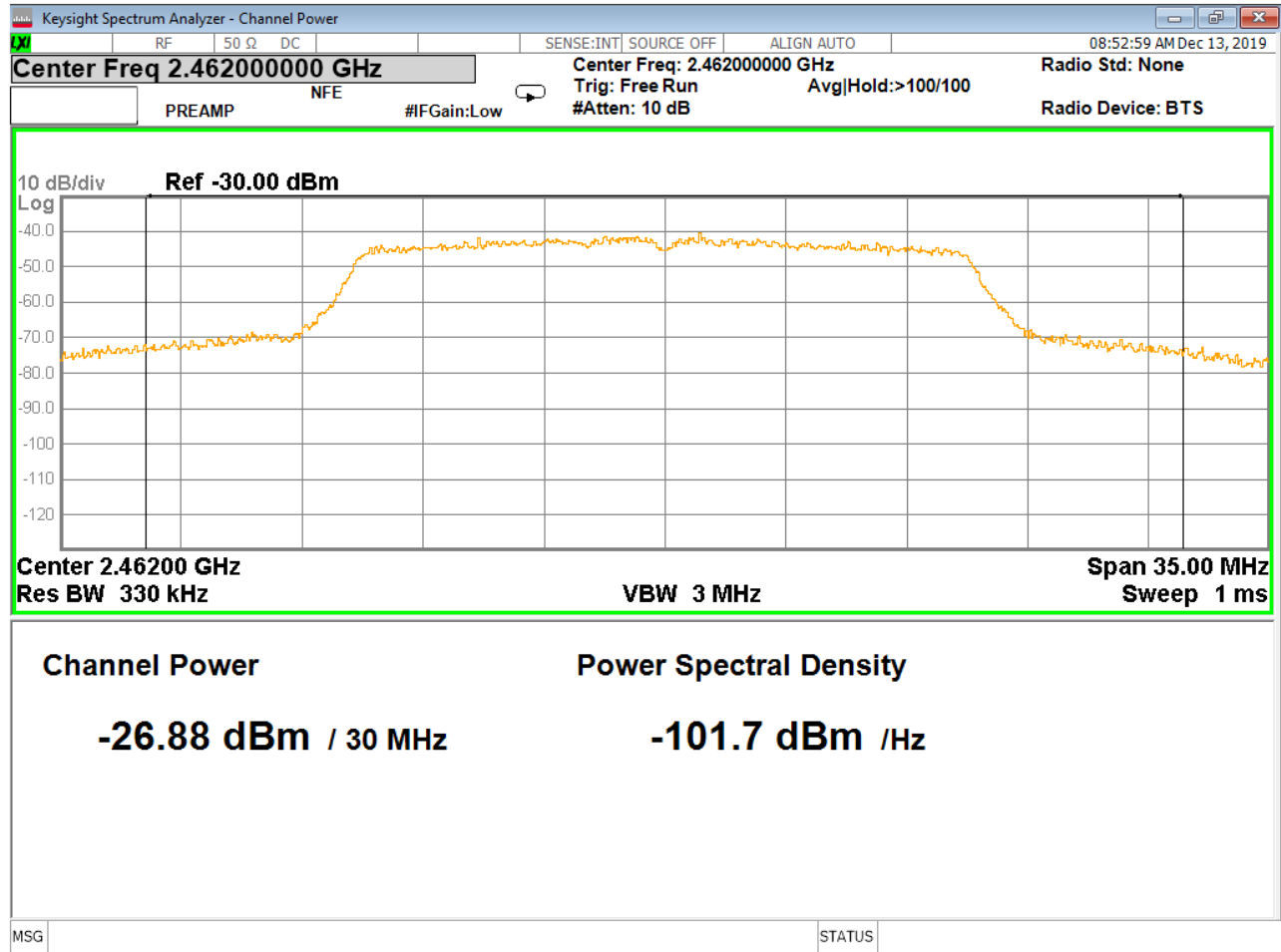
Figure 11 – Highest Peak Output Power, 802.11n
