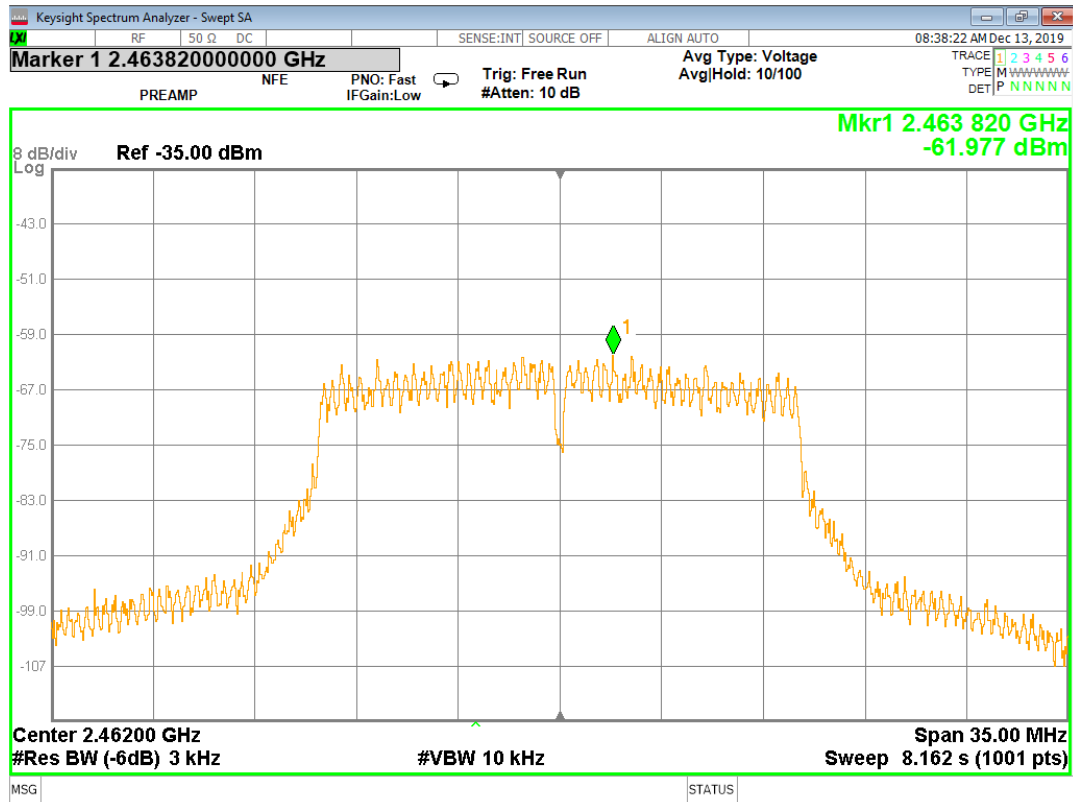
Figure 54 - Power Spectral Density, High Channel, 802.11g
