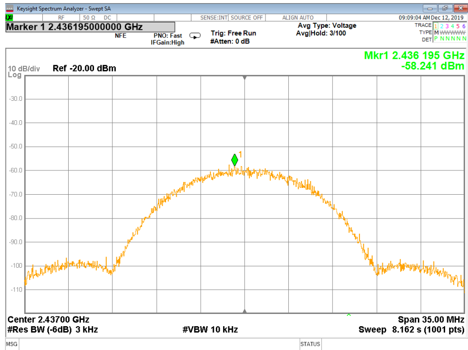
Figure 50 - Power Spectral Density, Mid Channel, 802.11b
