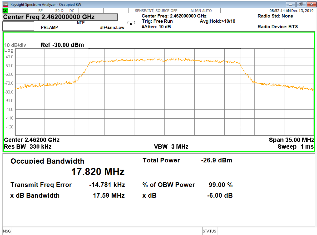
Figure 22 - 99% Occupied Bandwidth and 6dB Bandwidth, High Channel, 802.11n
