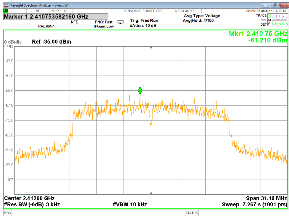
Figure 55 - Power Spectral Density, Low Channel, 802.11n
