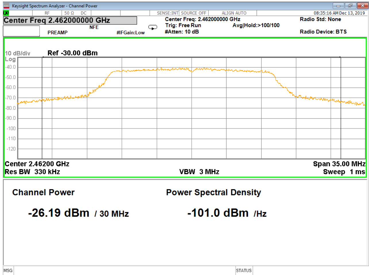
Figure 9 – Highest Peak Output Power, 802.11g
