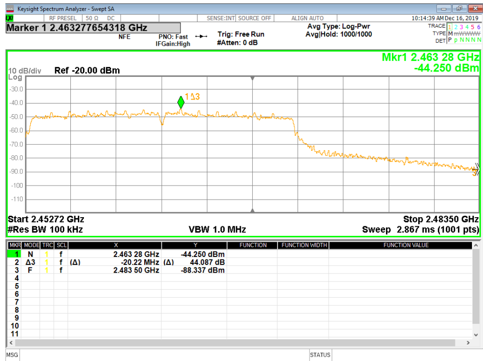
Figure 45 - Band-edge Measurement, High Channel, Fundamental, Peak
