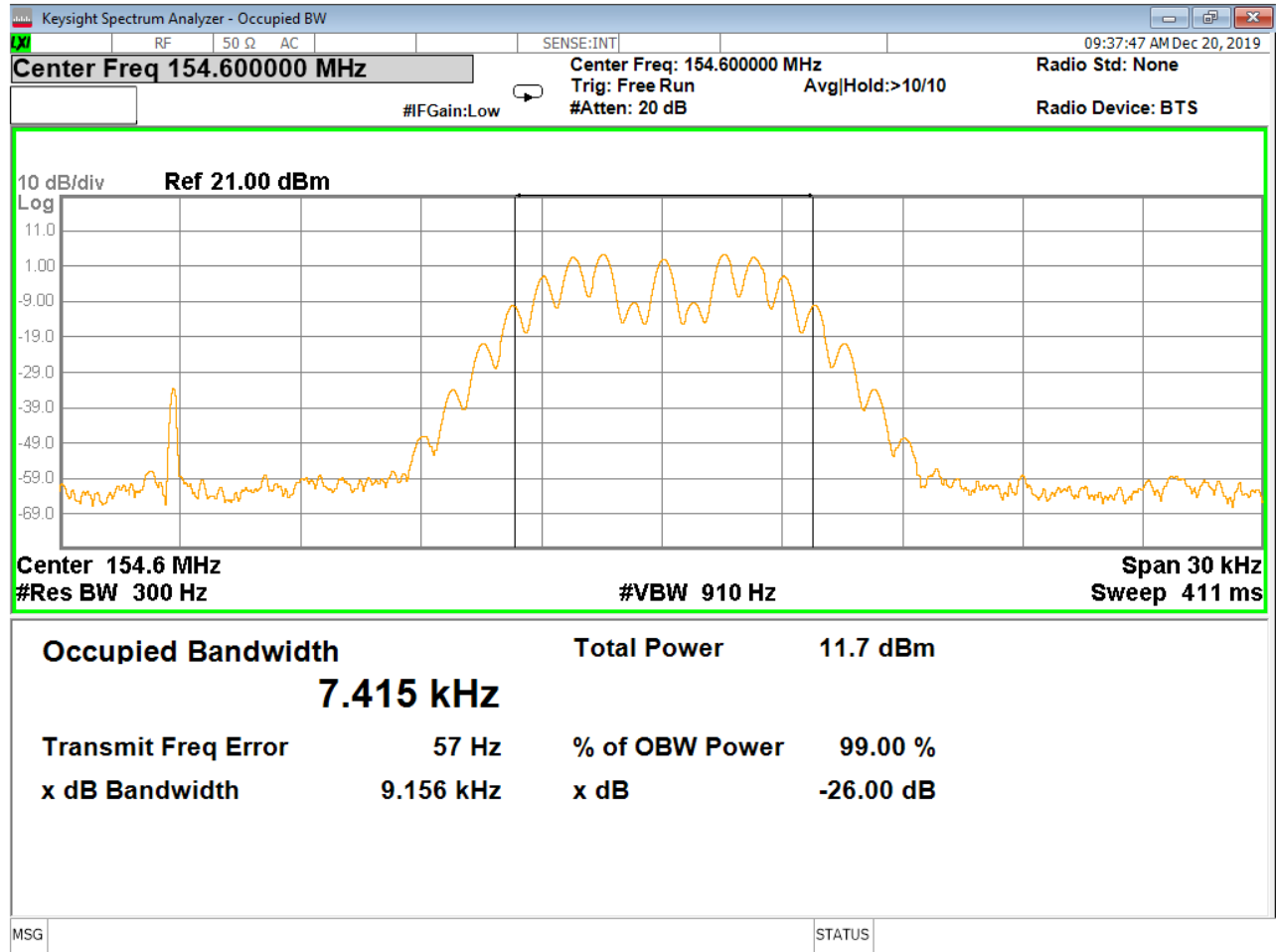
Figure 13 - Bandwidth, 154.600 MHz
