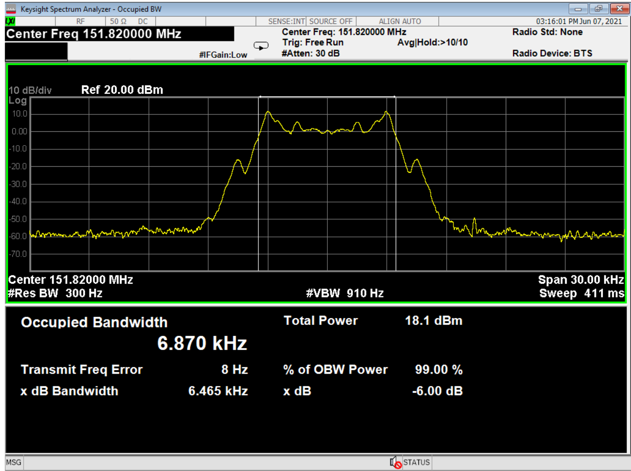
Figure 9 - Bandwidth, 151.820 MHz
