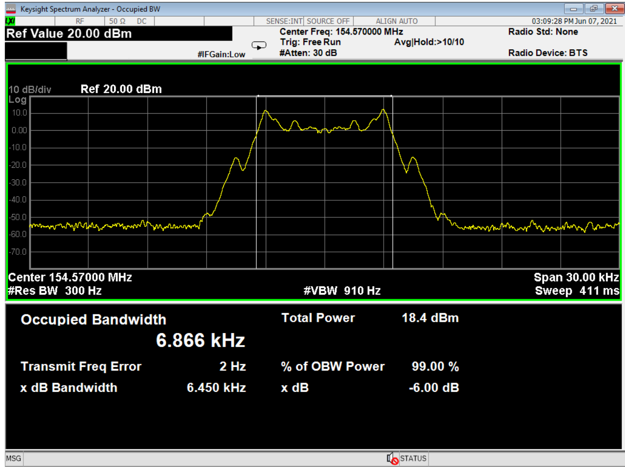
Figure 12 - Bandwidth, 154.570 MHz
