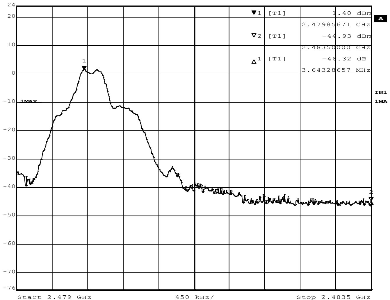
Figure 26 – Band Edge Measurement, High Channel, GFSK
