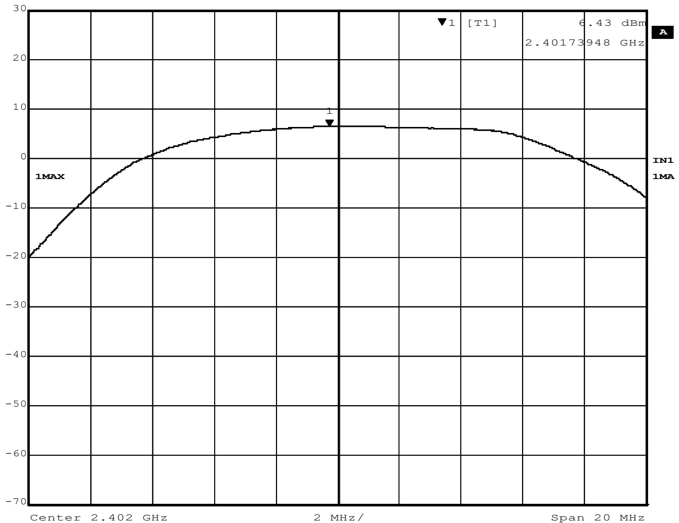
Figure 1 – Output Power, Low Channel, GMSK
