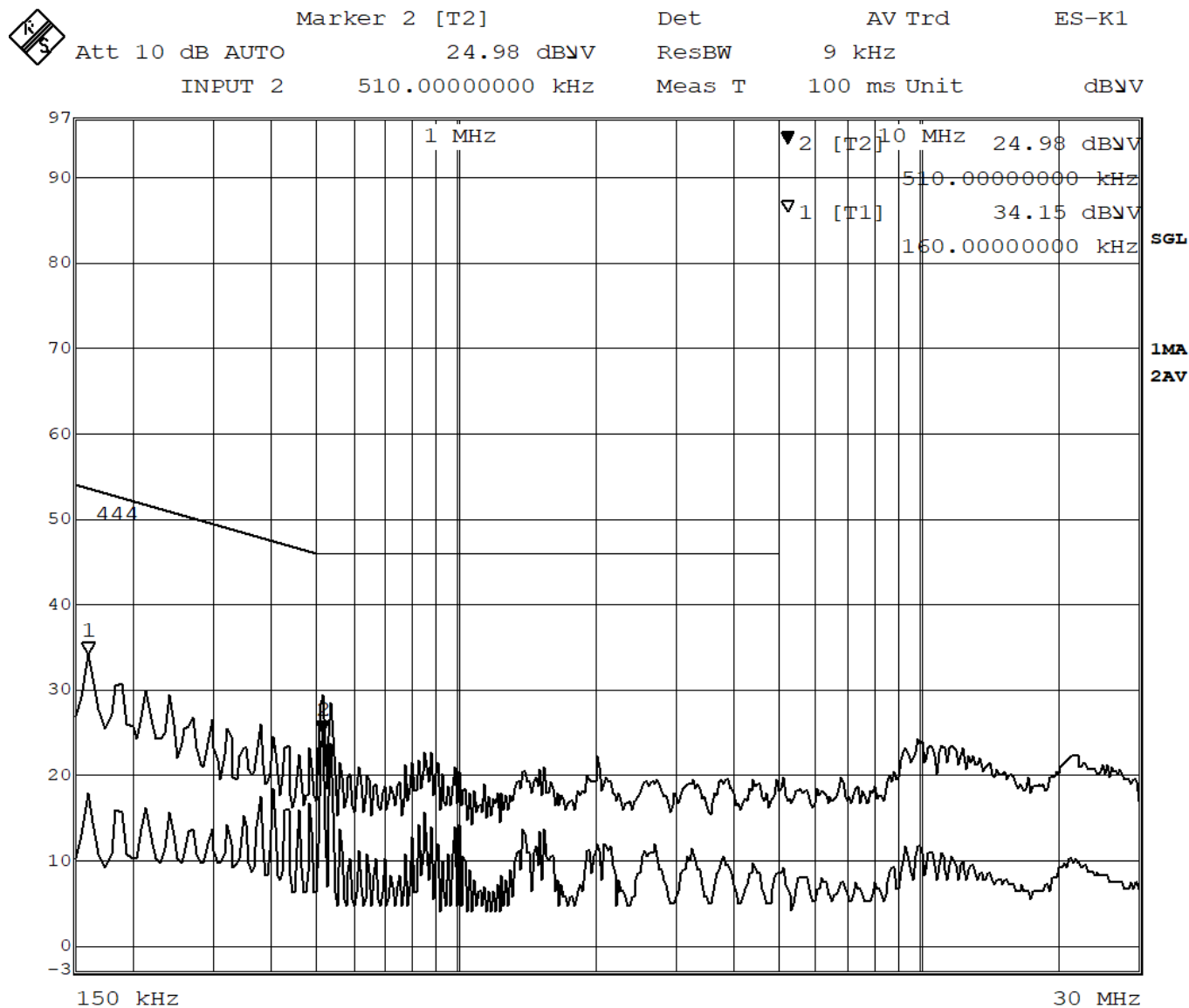
Figure 27 - Conducted Emissions Plot, L-F
