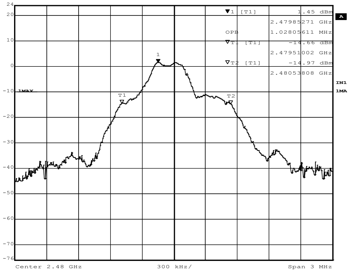
Figure 13 - Occupied Bandwidth, High Channel, GFSK
