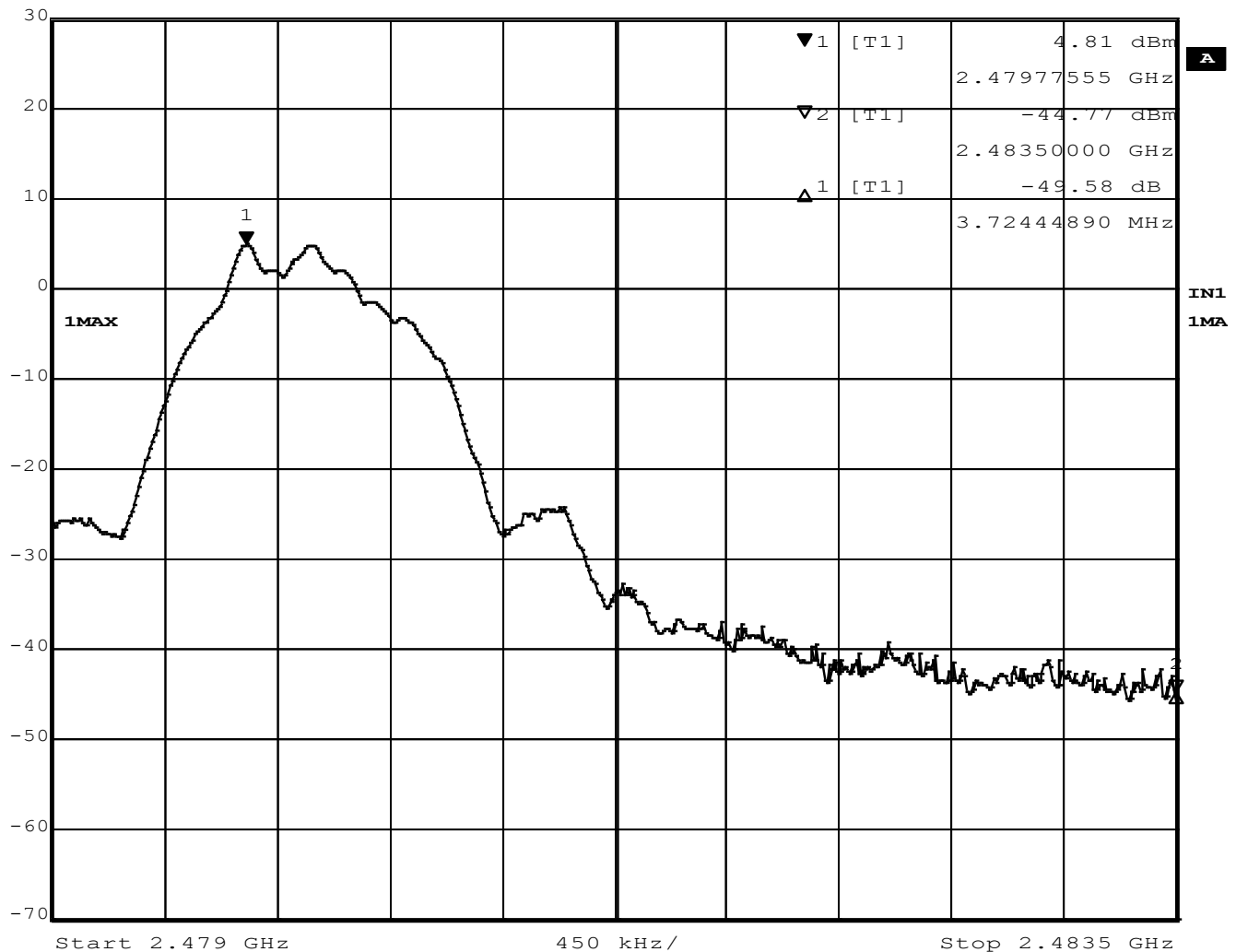
Figure 24 –Band Edge Measurement, High Channel, GMSK
