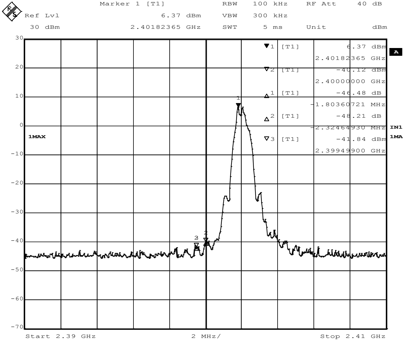
Figure 23 - Band Edge, Low Channel, GMSK
