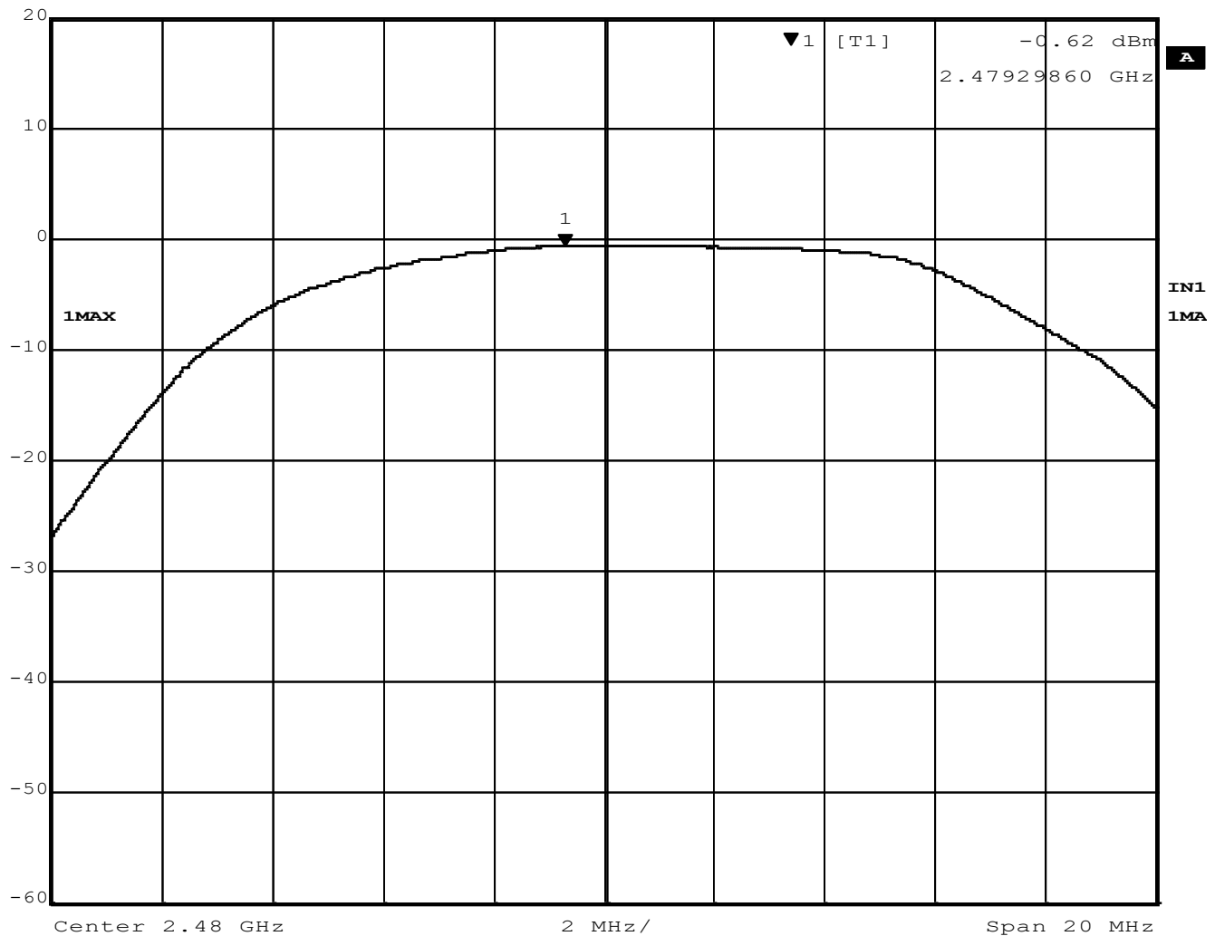
Figure 6 – Output Power, High Channel, GMSK
