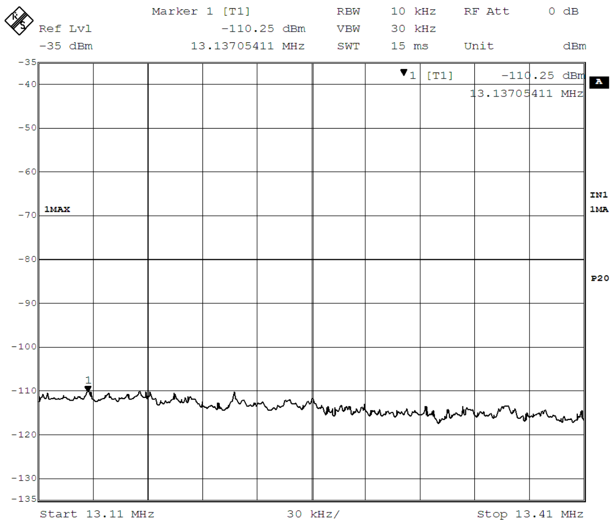
Figure 6 – Lower Bandedge
