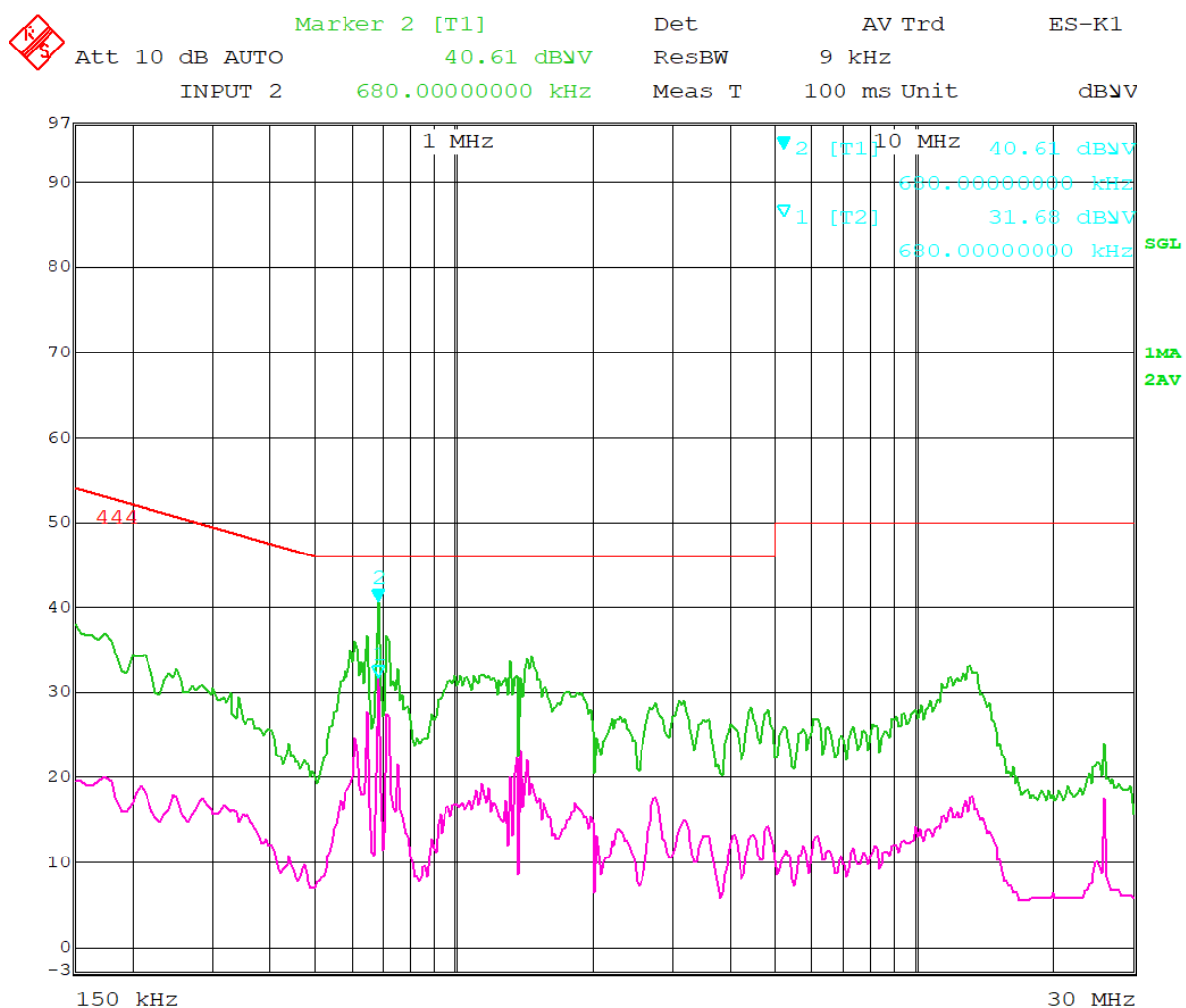
Figure 10 - Conducted Emissions, Line
