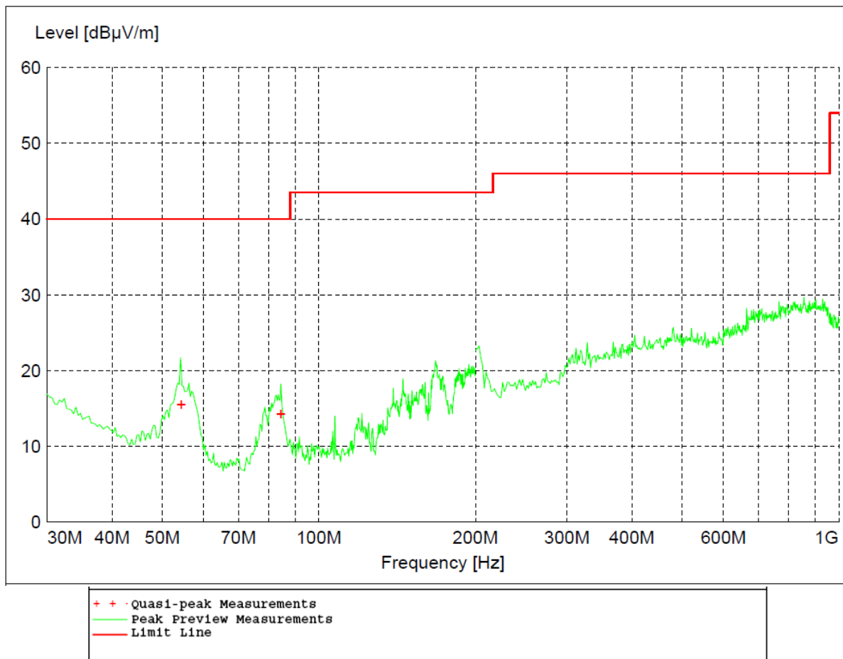
Figure 2 – Radiated Emissions Peak Plot, 30 MHz- 1 GHz
