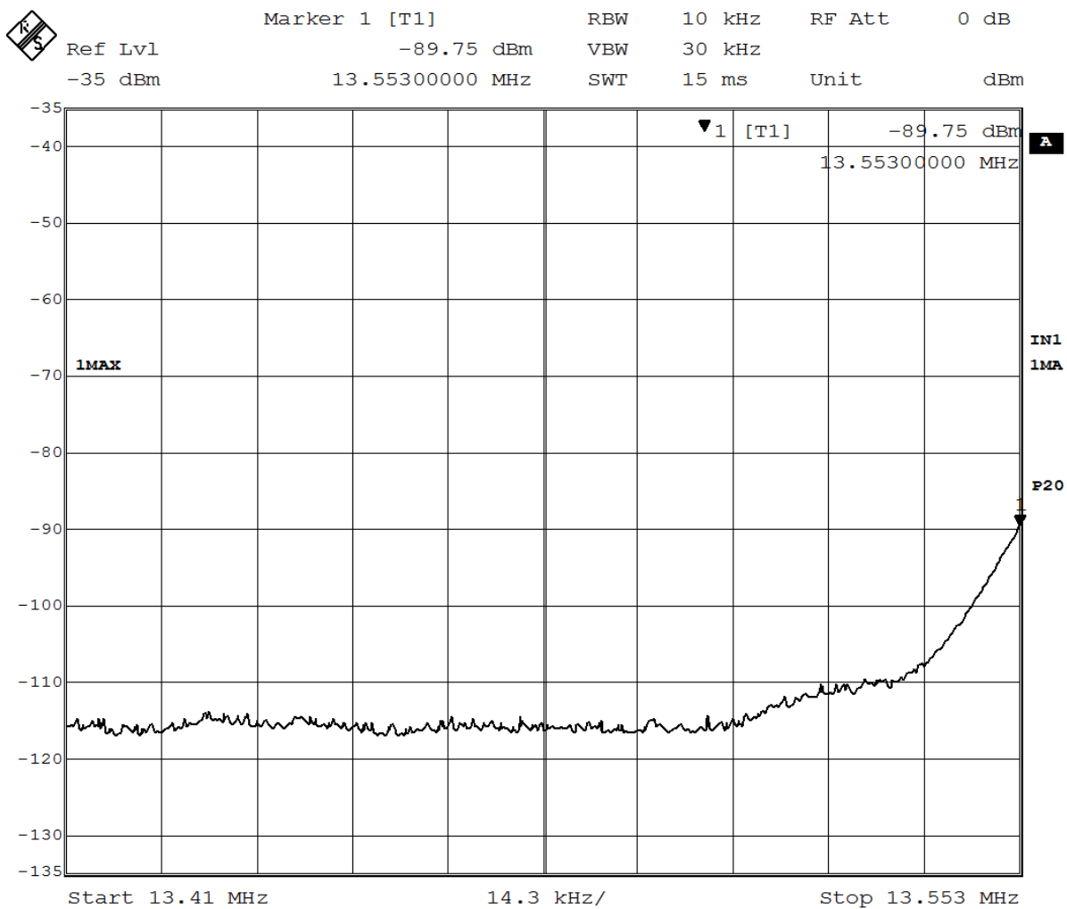
Figure 7 – Lower Bandedge
