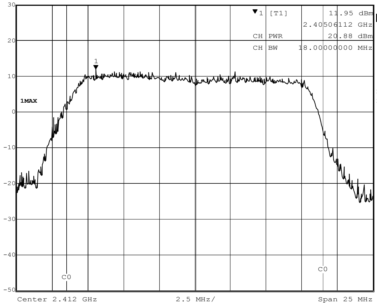
Figure 5 – Output Power Peak, Low Channel, 802.11g
