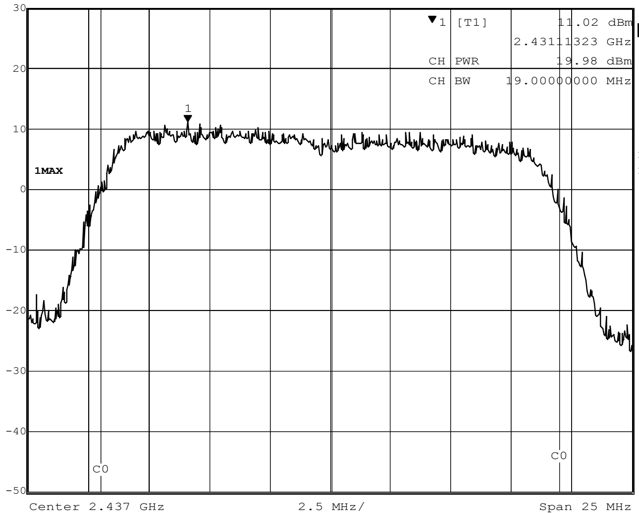
Figure 9 – Output Power Peak, Mid Channel, 802.11n
