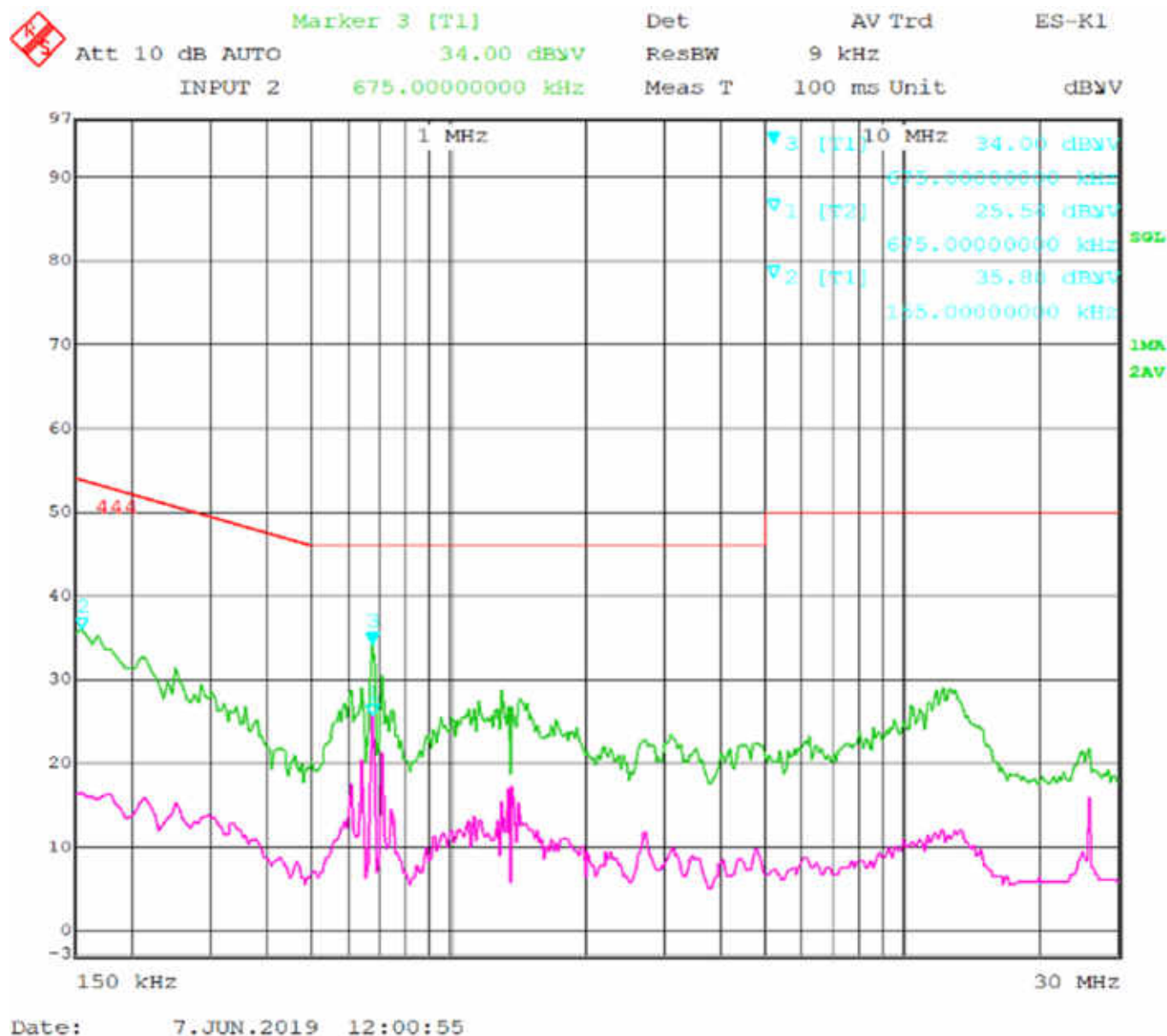
Figure 69 - Conducted Emissions Plot, Neutral
