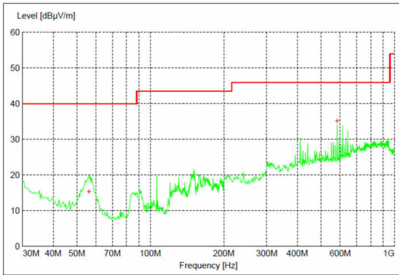
Figure 34 - Radiated Emissions Plot, 802.11n
