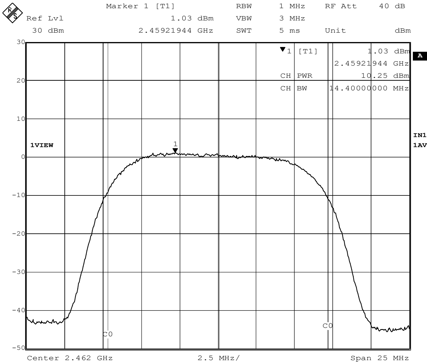
Figure 13 – Output Power Average, High Channel, 802.11b
