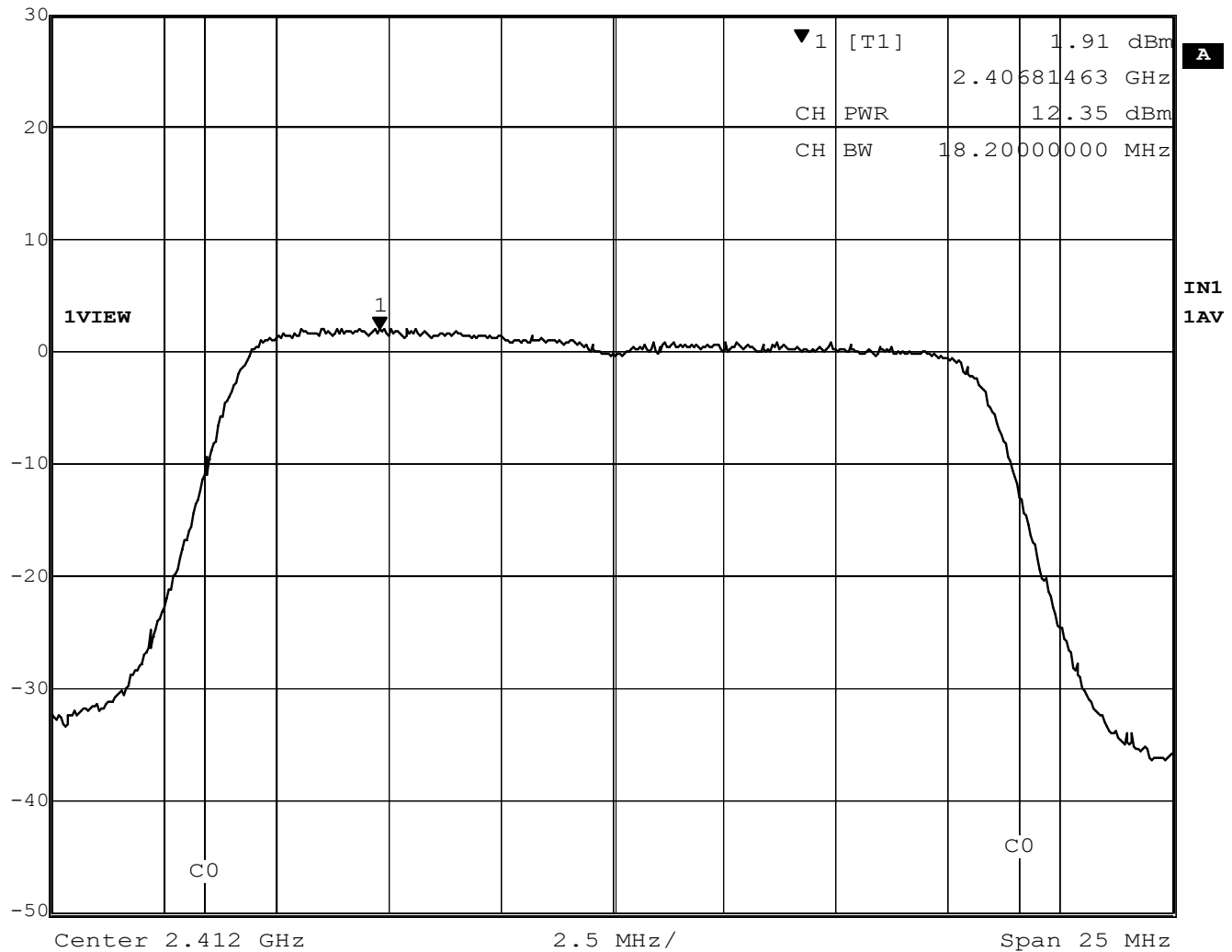
Figure 14 – Output Power Average, Low Channel, 802.11g
