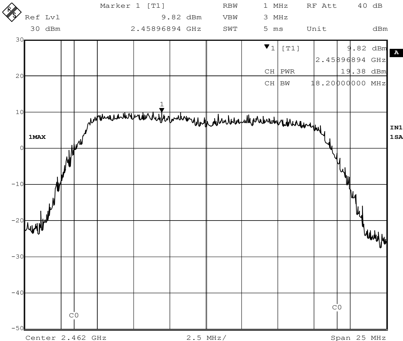
Figure 7 – Output Power Peak, High Channel, 802.11g
