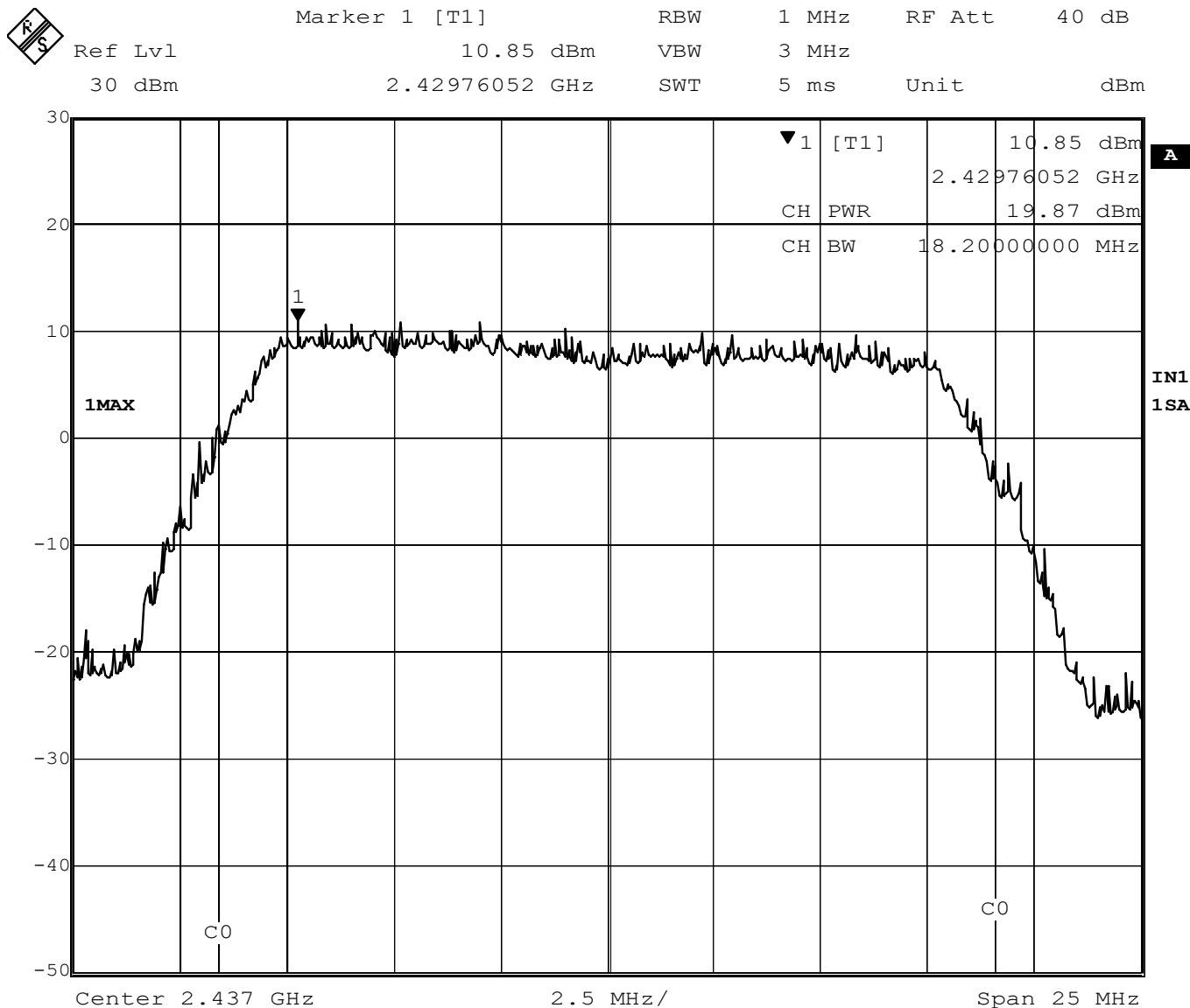
Figure 6 – Output Power Peak, Mid Channel, 802.11g
