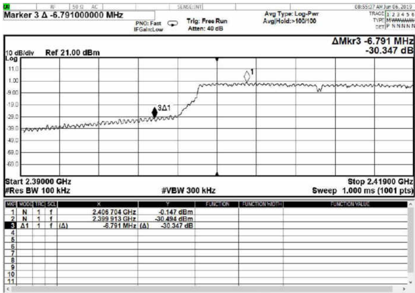
Figure 61 - Band-edge Measurement, Low Channel, Fundamental, Peak
