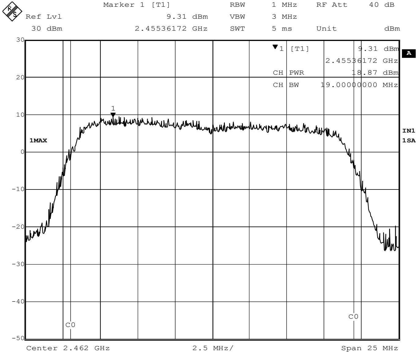
Figure 10 – Output Power Peak, High Channel, 802.11n
