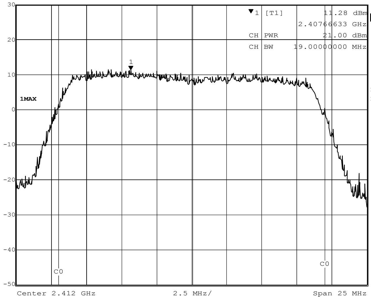
Figure 8 – Output Power Peak, Low Channel, 802.11n
