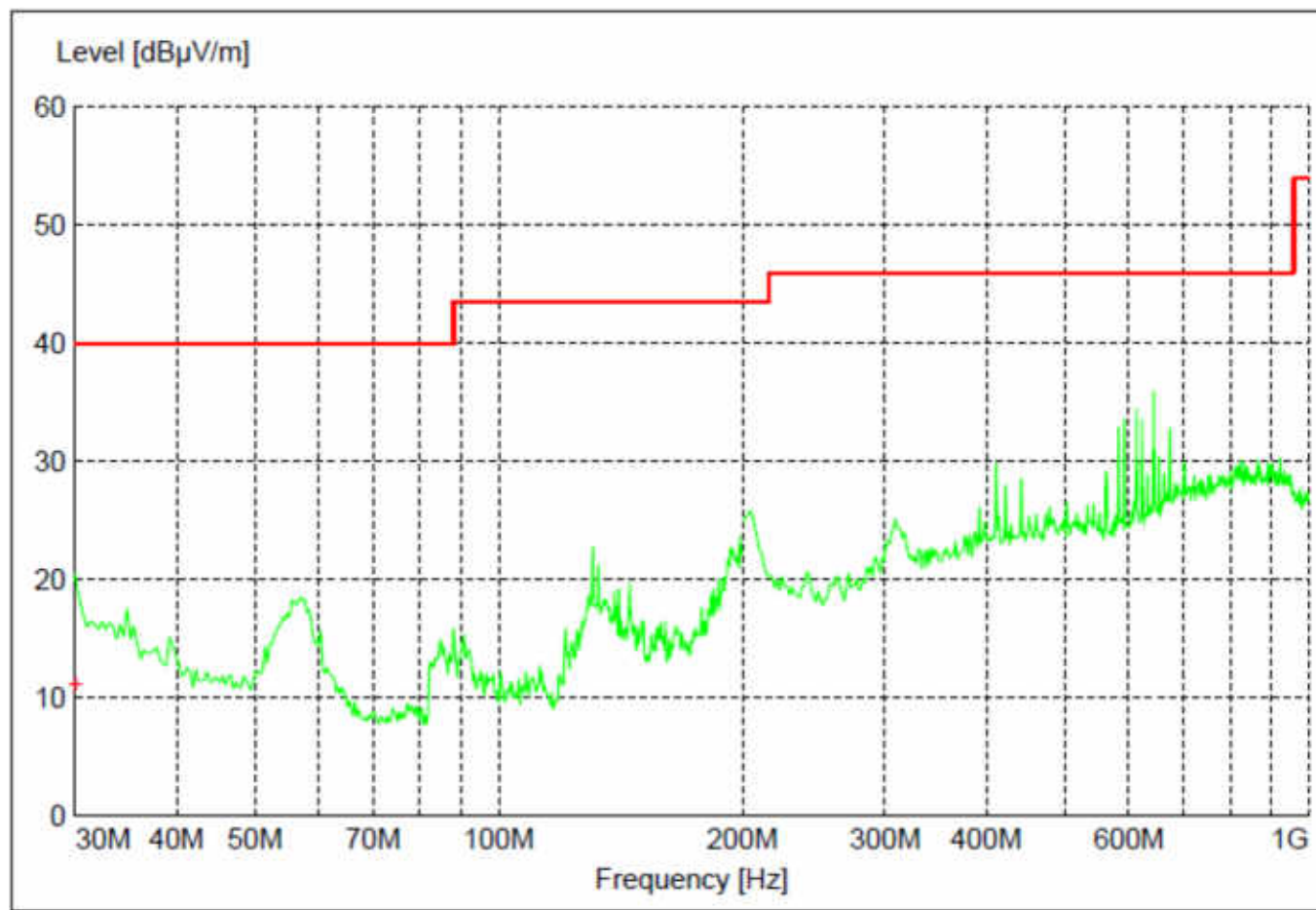
Figure 33 - Radiated Emissions Plot, 802.11g
