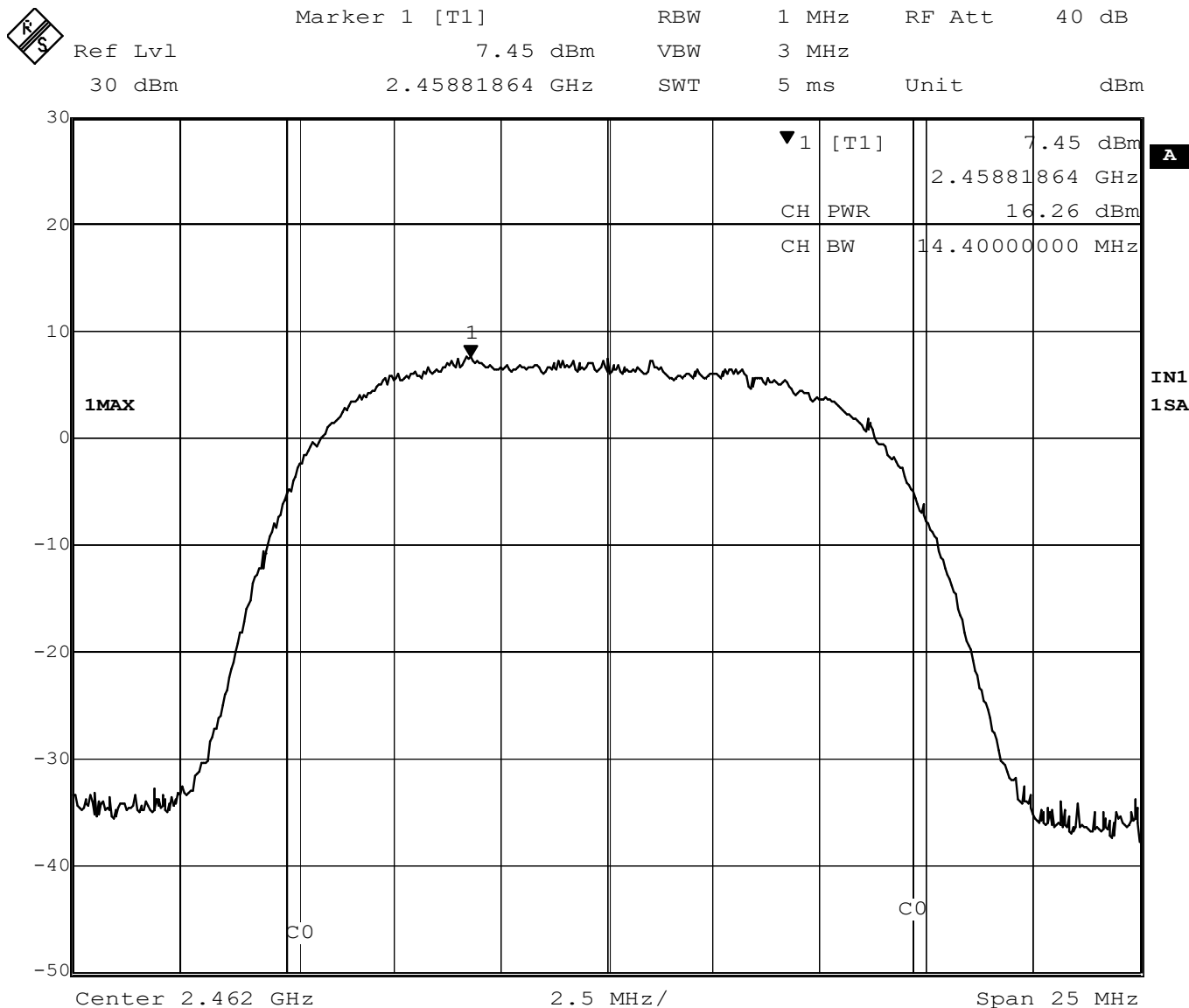
Figure 4 – Output Power Peak, High Channel, 802.11b
