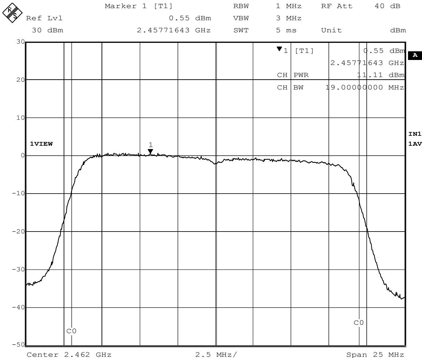
Figure 19 – Output Power Average, High Channel, 802.11n
