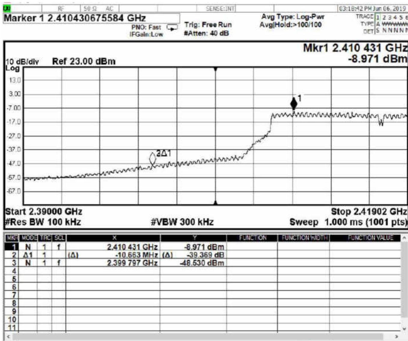
Figure 55 - Band-edge Measurement, Low Channel, Fundamental, Average
