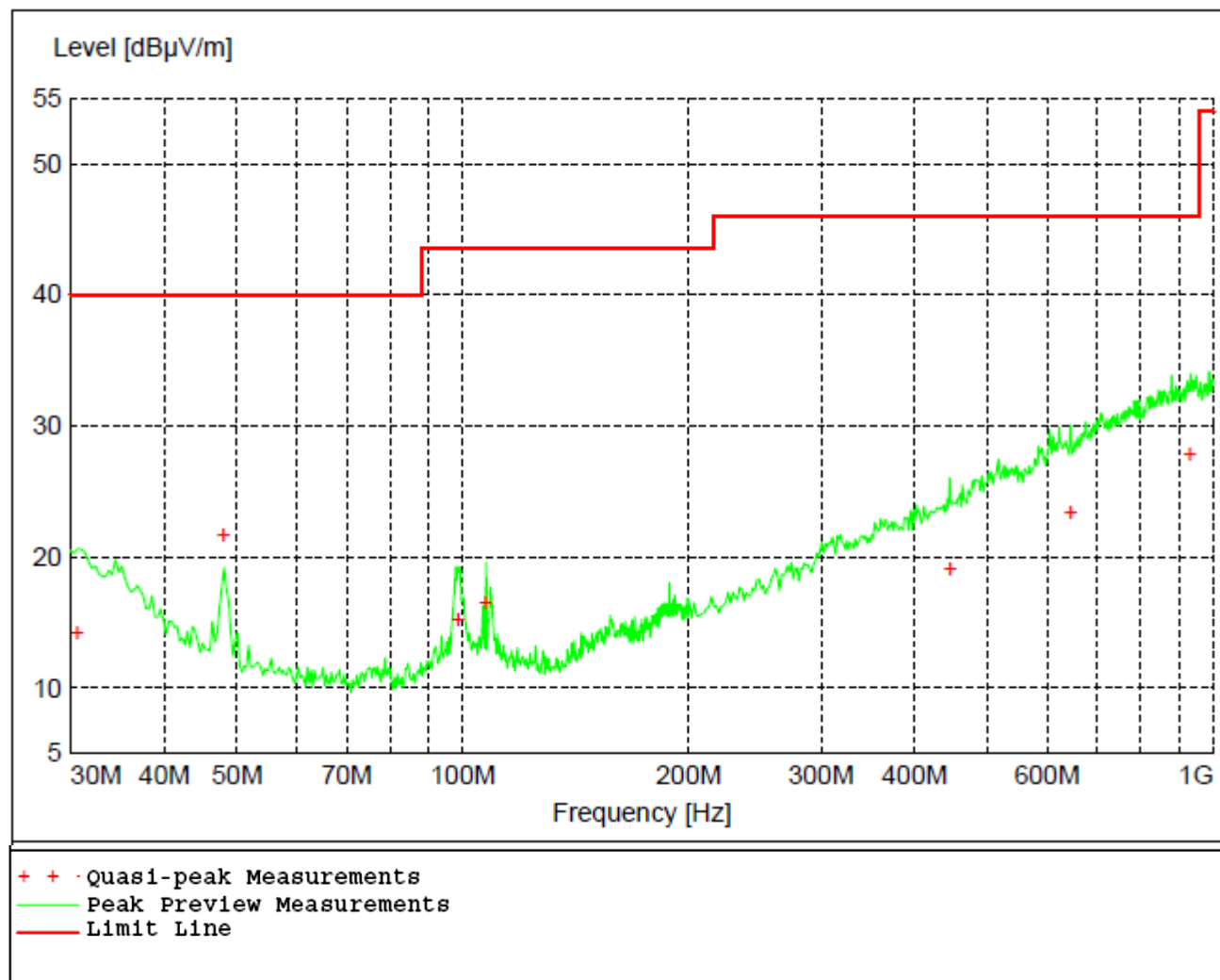
Figure 22 - Radiated Emissions Plot, Low Channel, GMSK
