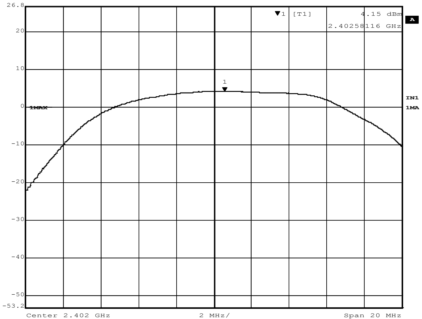
Figure 3 – Output Power, Low Channel, GMSK
