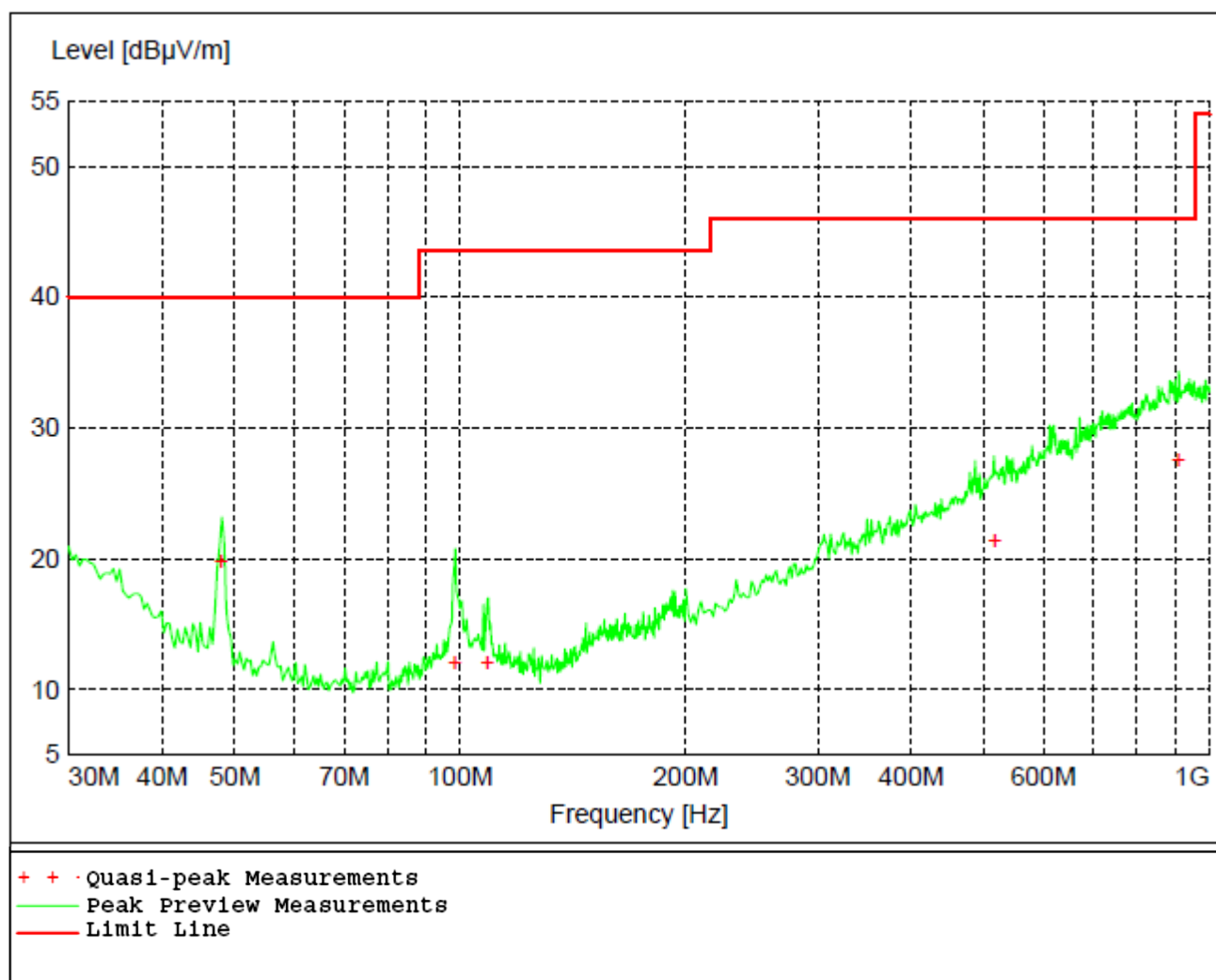
Figure 23 - Radiated Emissions Plot, Mid Channel, GMSK
