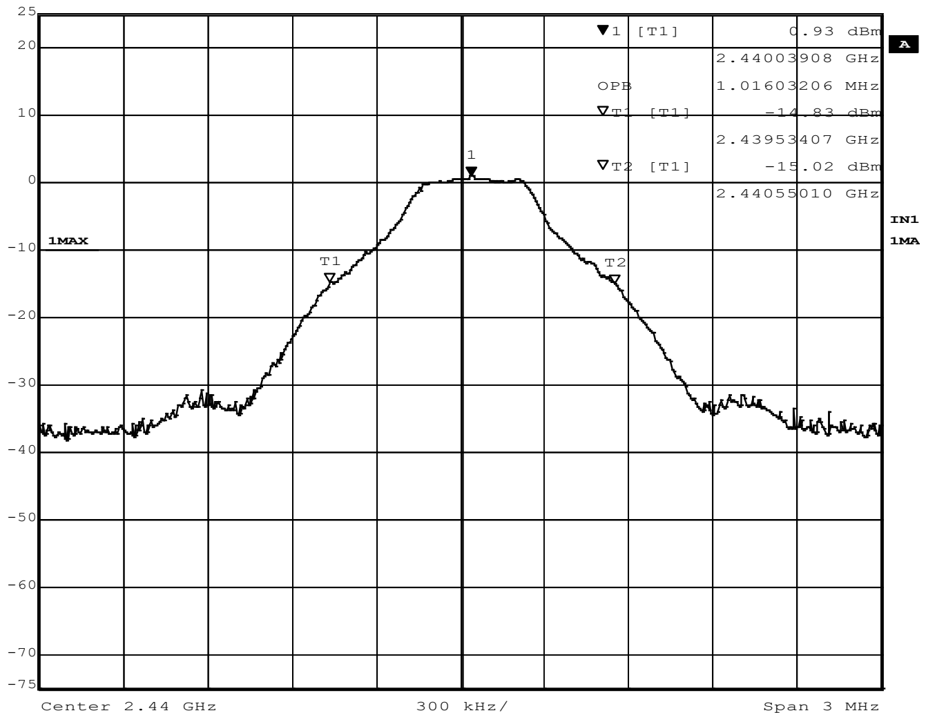
Figure 14 - Occupied Bandwidth, Mid Channel, GFSK
