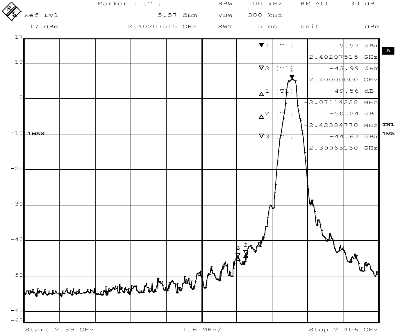
Figure 27 –Band Edge, Low Channel, GFSK
