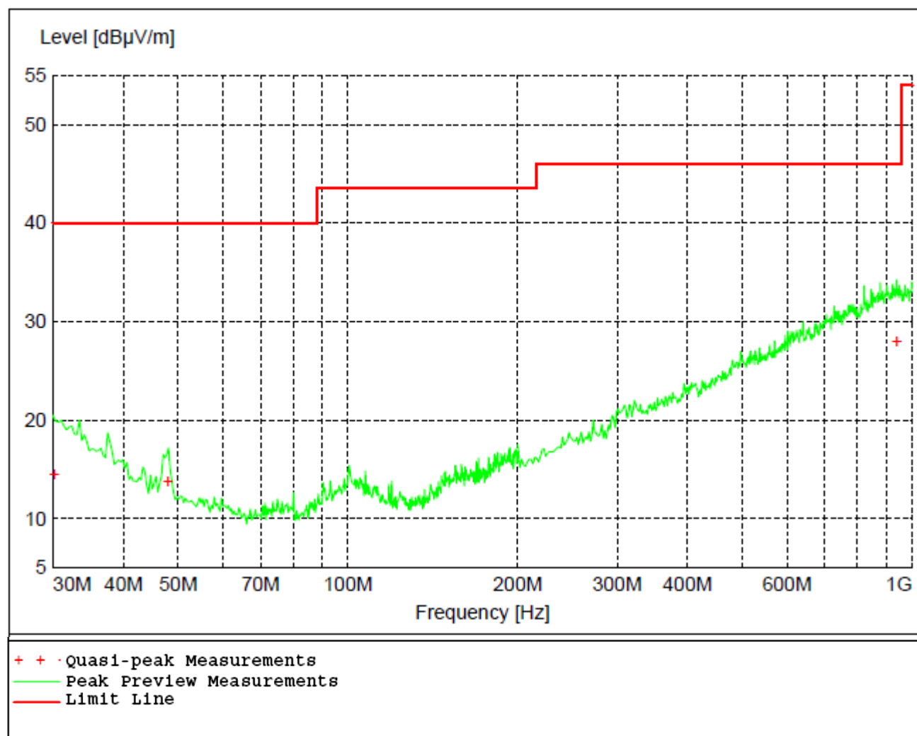
Figure 20 - Radiated Emissions Plot, Mid Channel, GFSK
