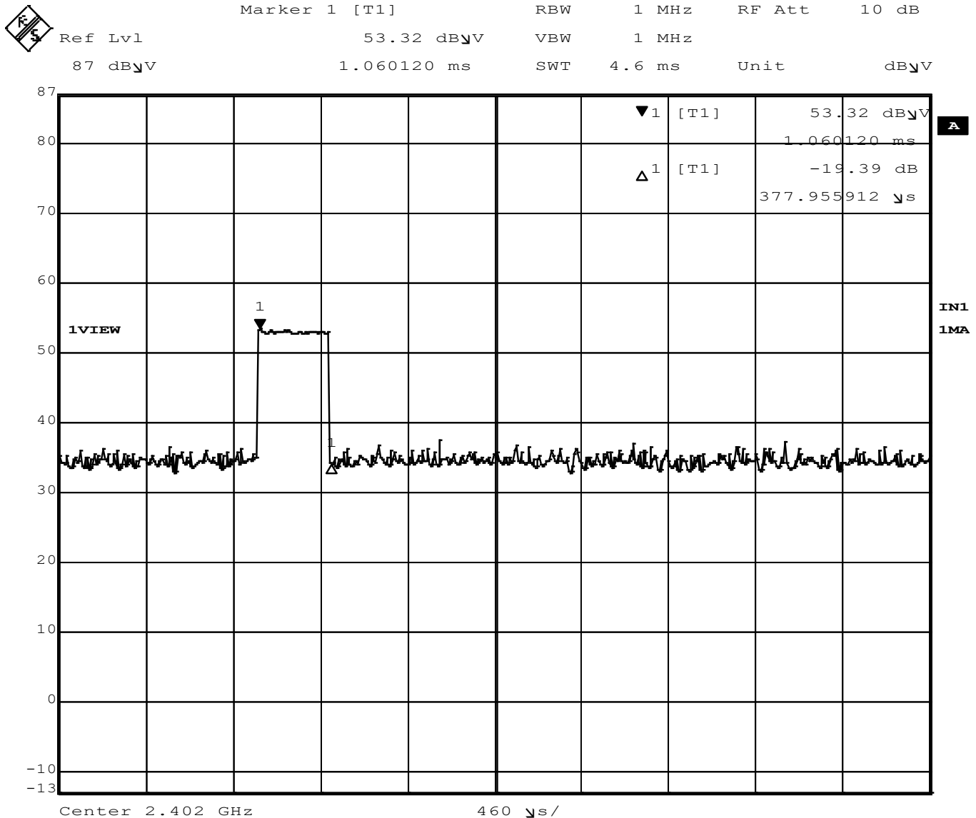
Figure 1 – Duty cycle - On Time, 0.378 ms
