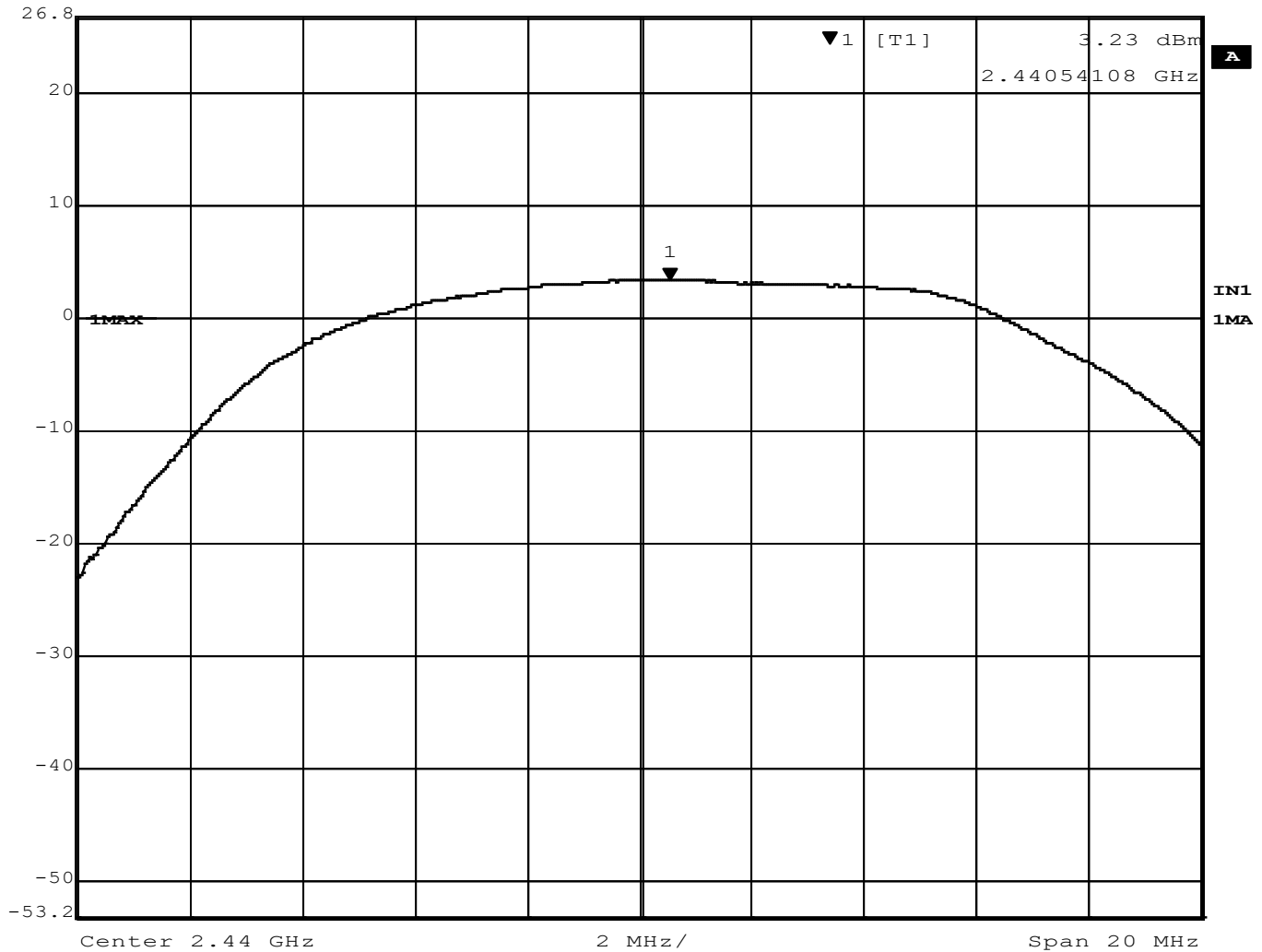
Figure 4 – Output Power, Mid Channel, GMSK
