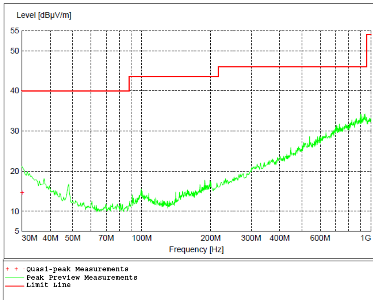
Figure 21 - Radiated Emissions Plot, High Channel, GFSK
