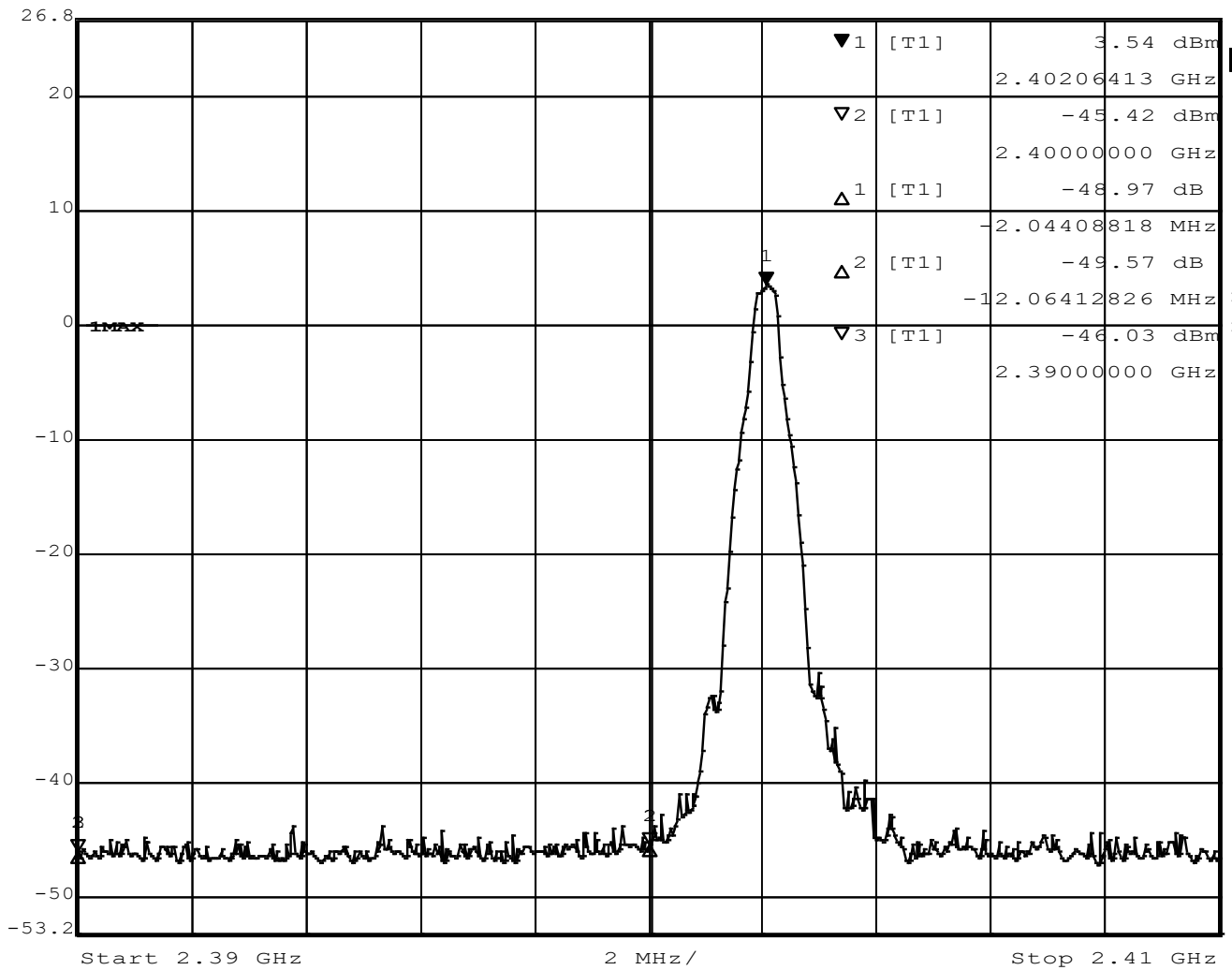
Figure 25 - Band Edge, Low Channel, GMSK
