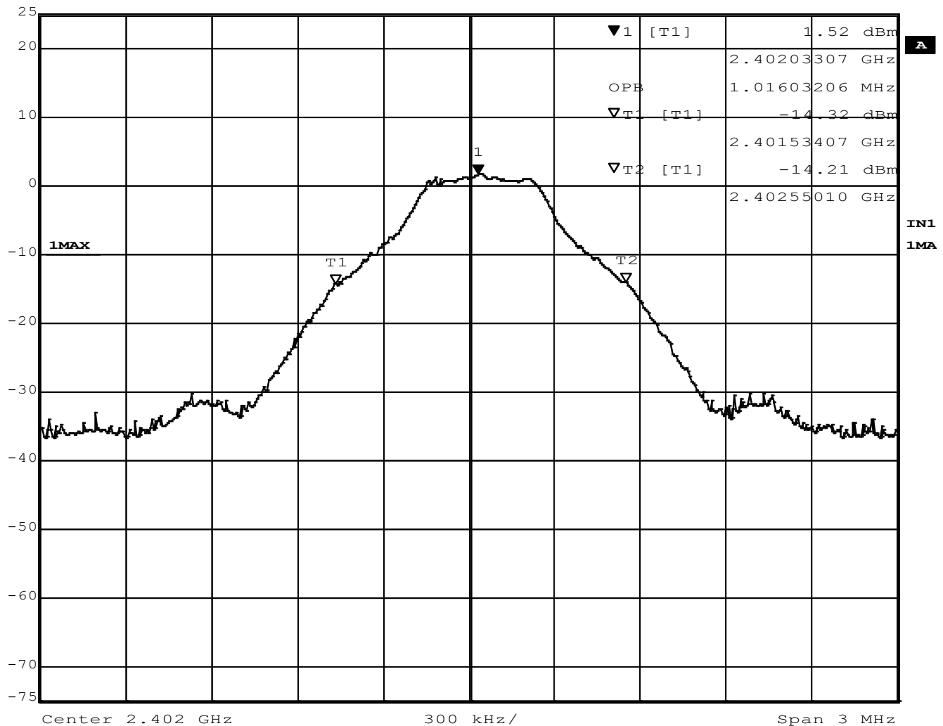
Figure 13 – Occupied Bandwidth, Low Channel, GFSK
