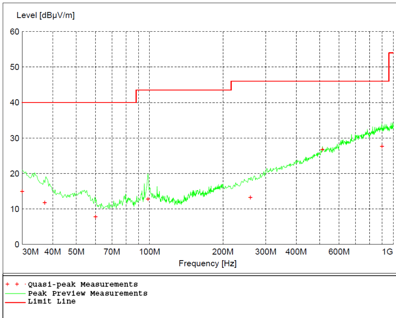
Figure 5 - Radiated Emissions Plot, High Channel, GMSK
