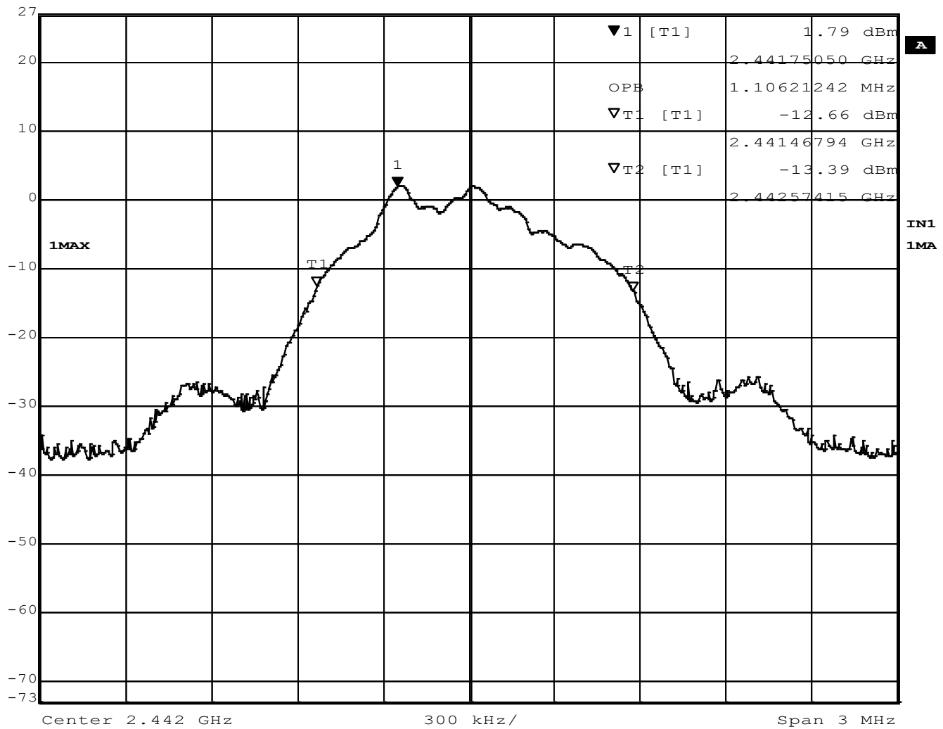
Figure 12 - Occupied Bandwidth, Mid Channel, GMSK
