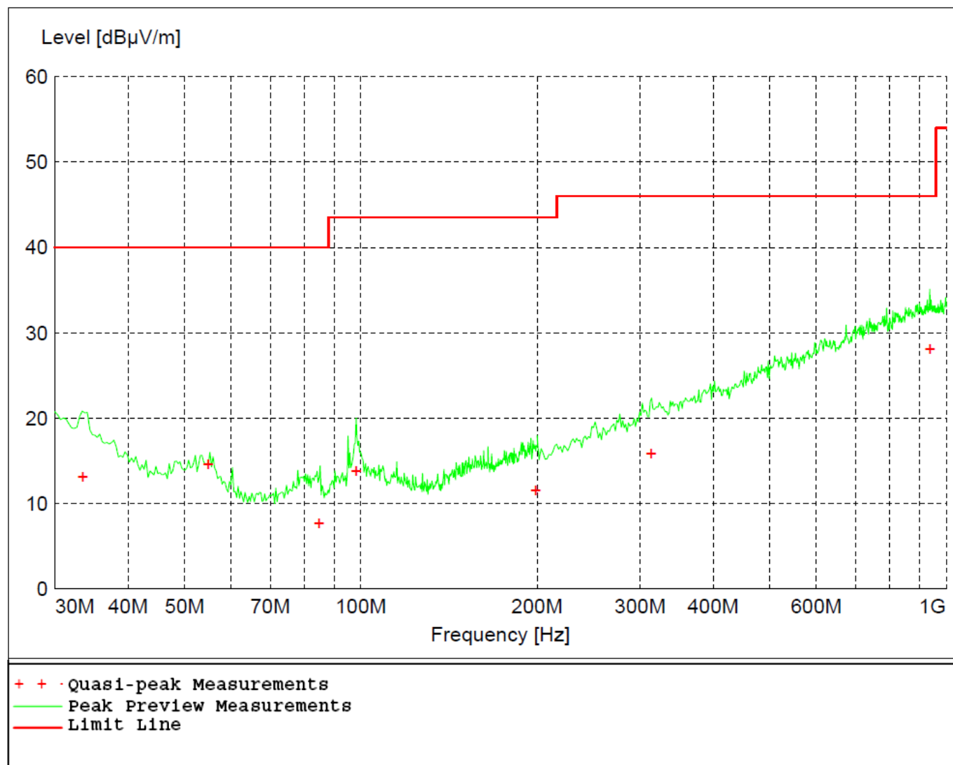
Figure 2 - Radiated Emissions Plot, Receive, GMSK
