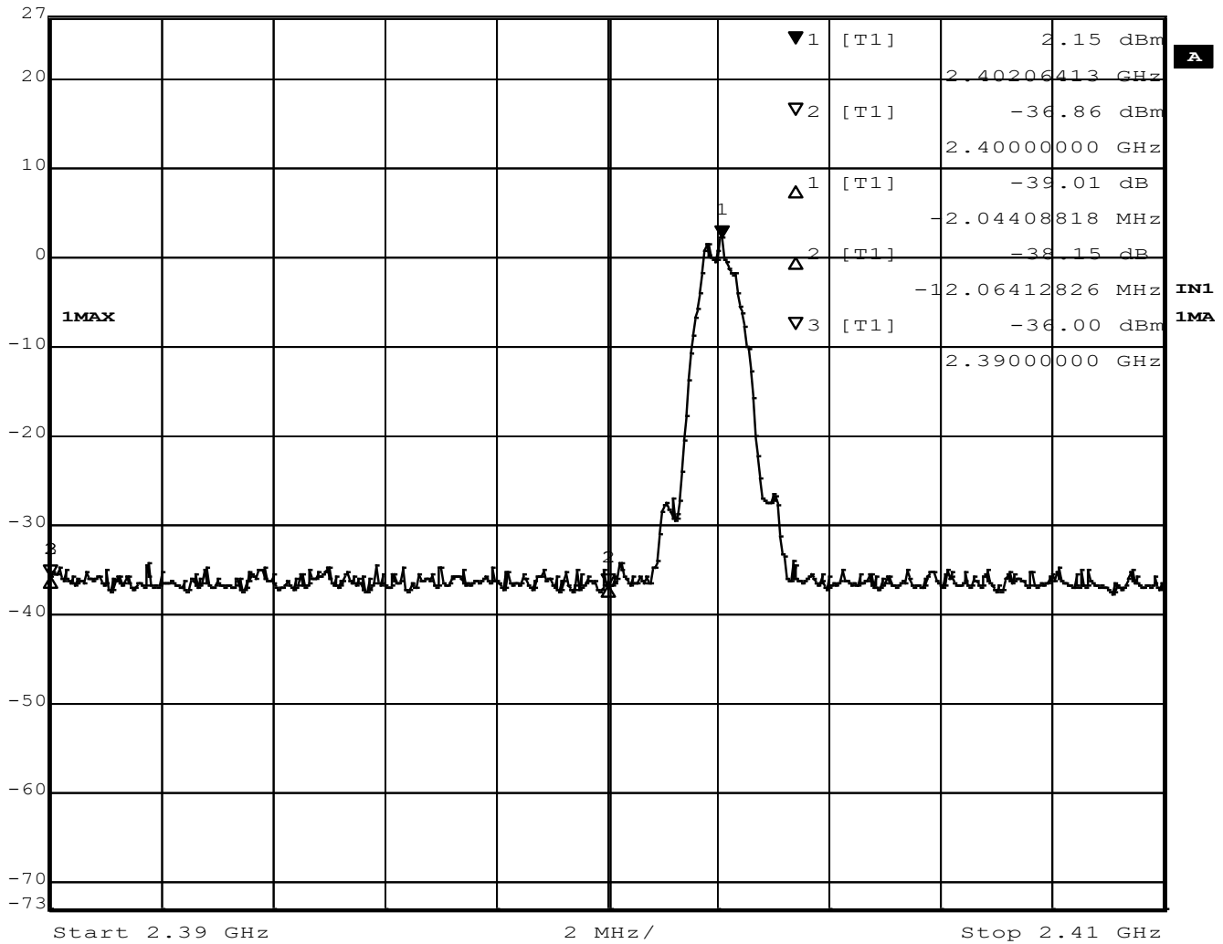
Figure 14 - Band Edge, Low Channel, GMSK
