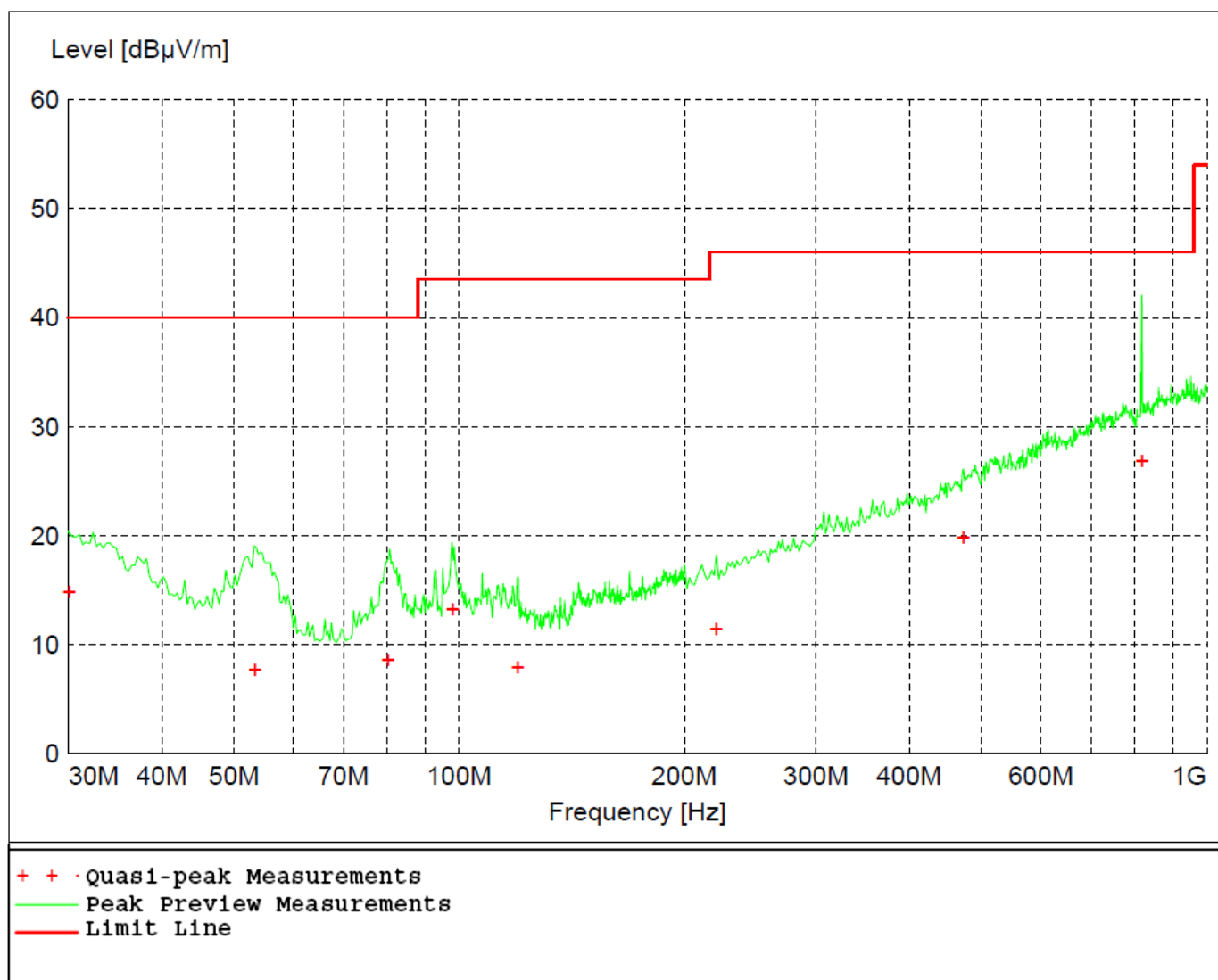
Figure 4 - Radiated Emissions Plot, Mid Channel, GMSK
