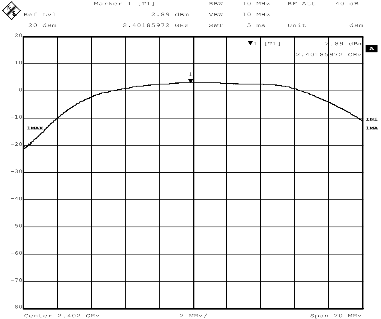
Figure 7 – Output Power, Low Channel, GMSK
