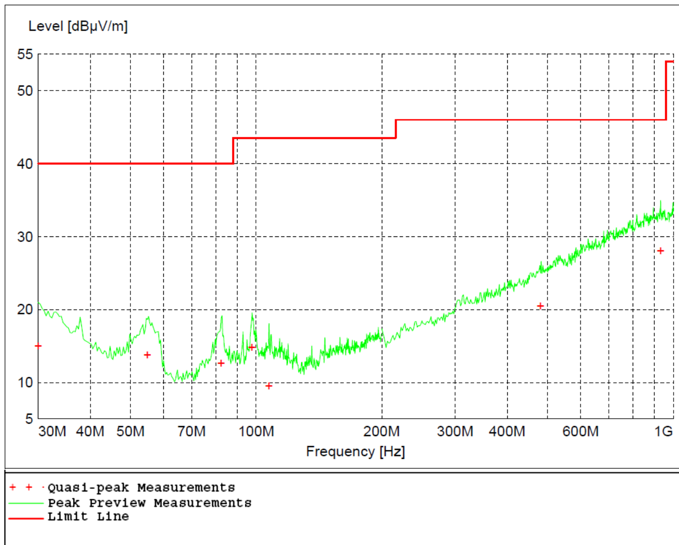
Figure 3 - Radiated Emissions Plot, Low Channel, GMSK
