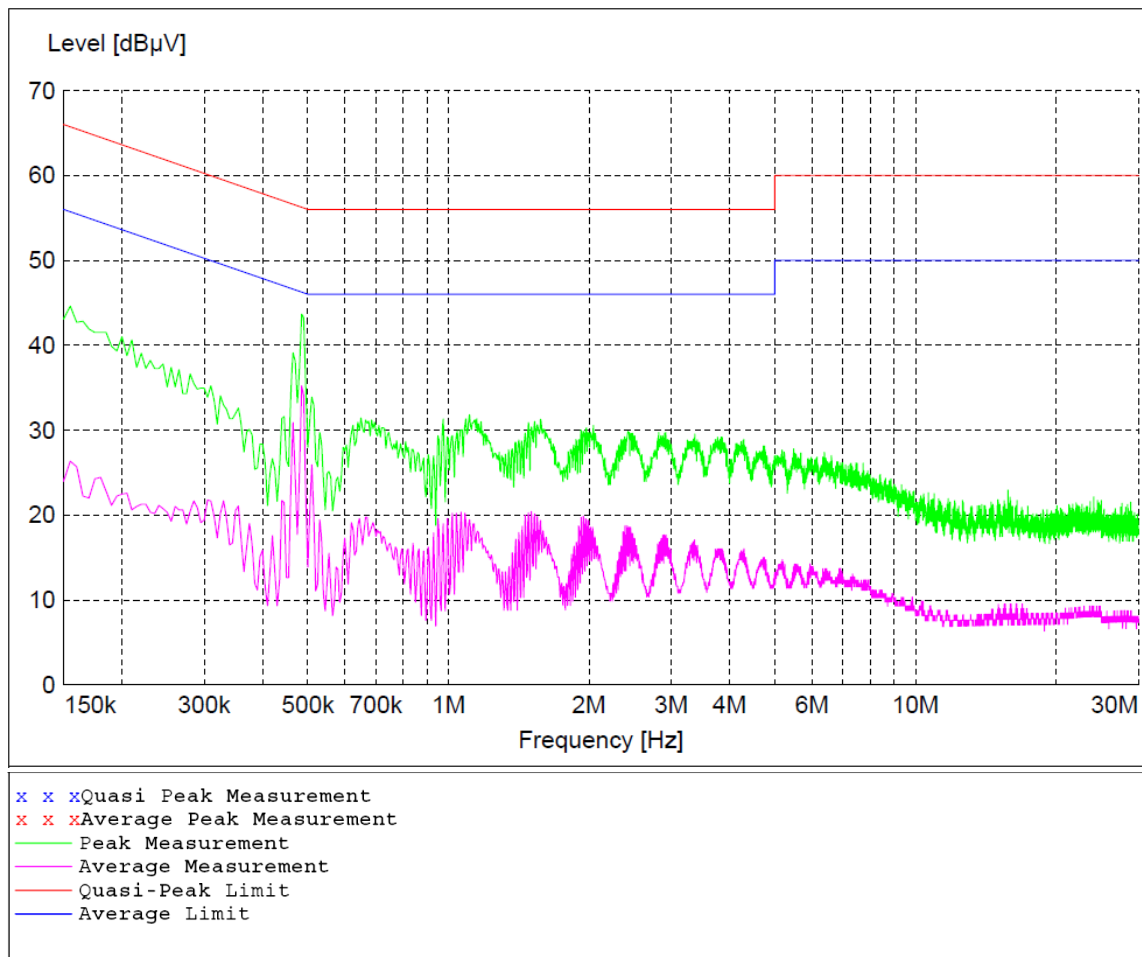
Figure 16 - Conducted Emissions Plot
