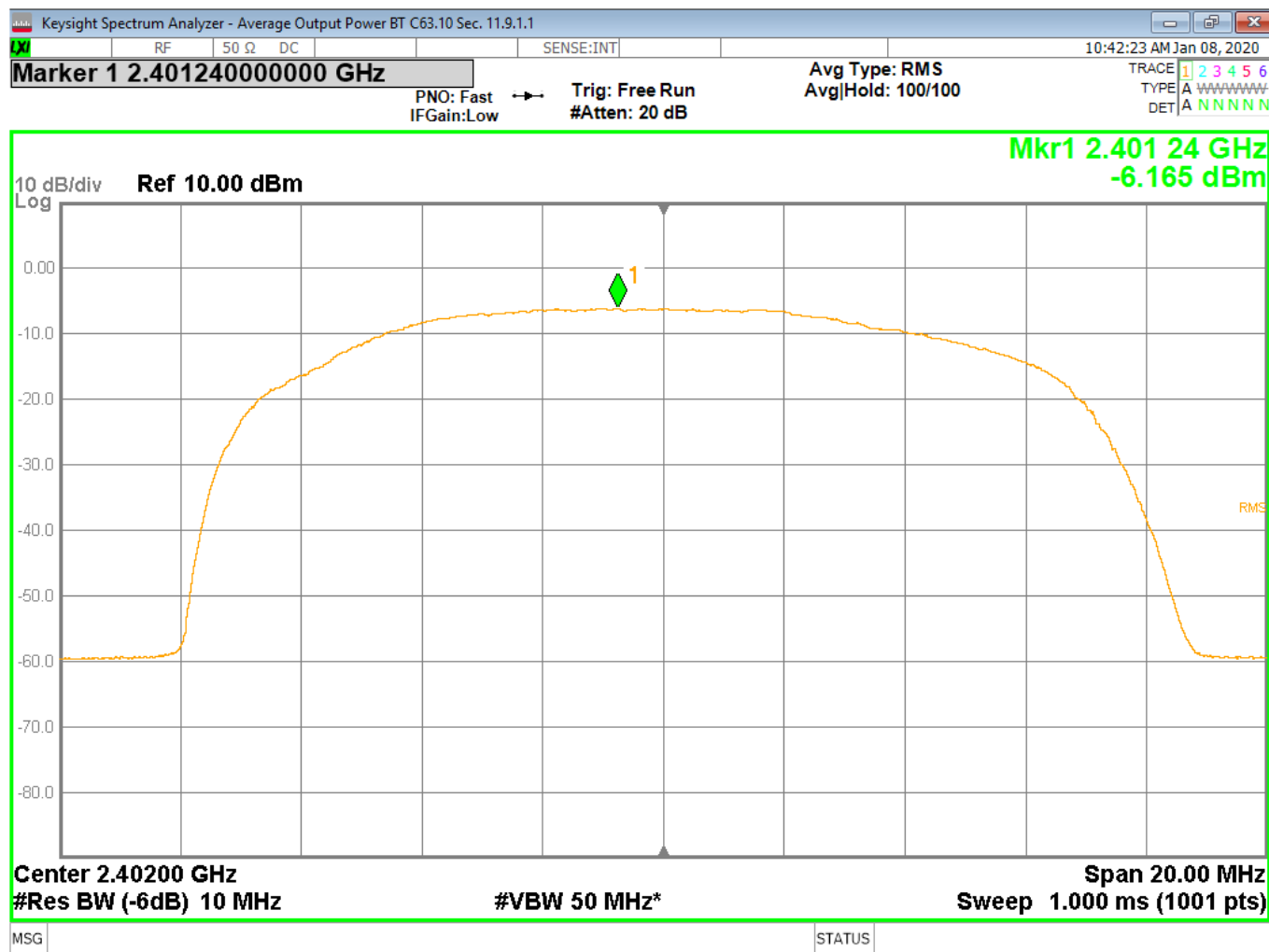
Figure 11 - Average Output Power, Low Channel, BT EDR 3MB
