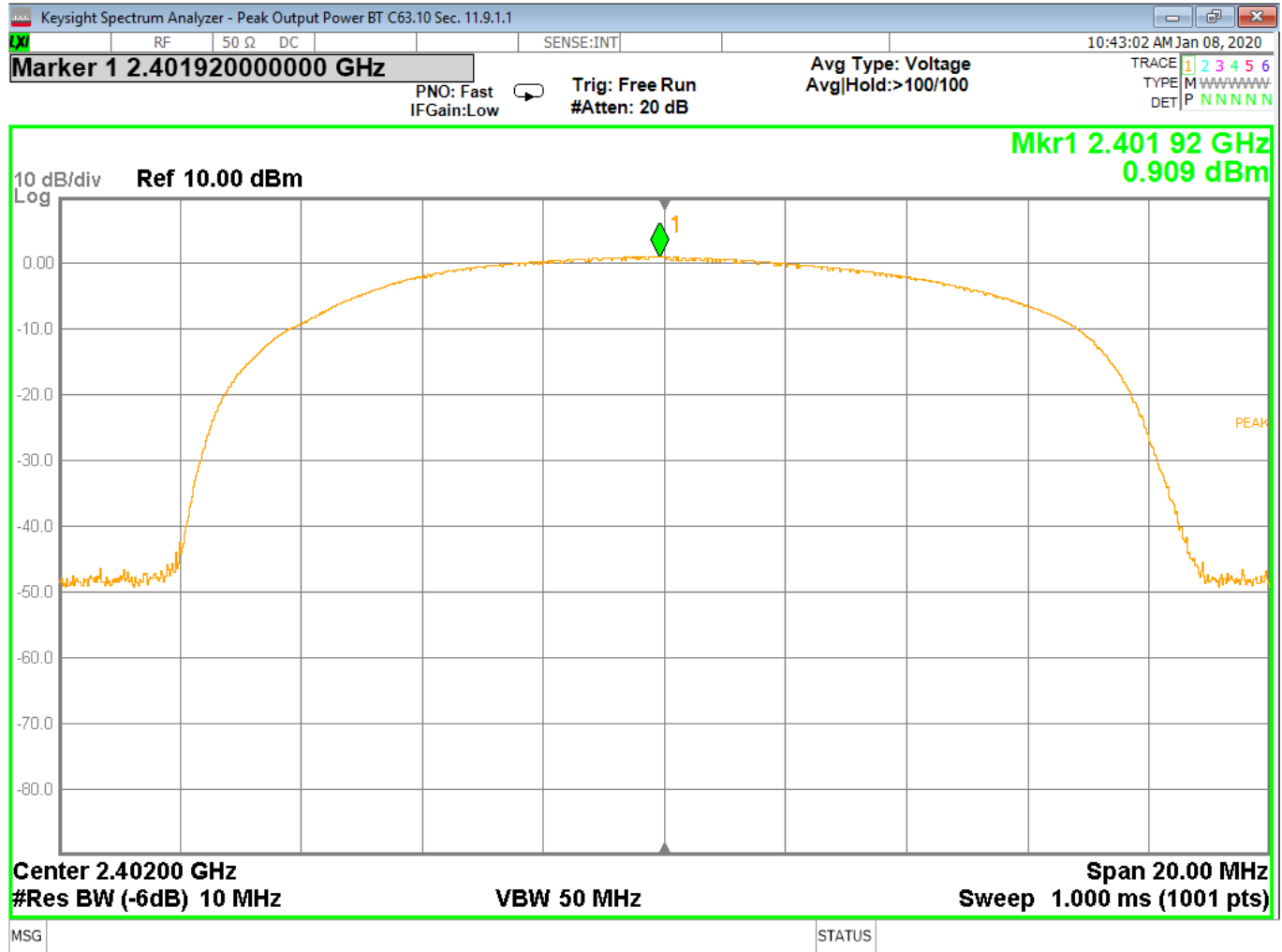
Figure 5 - Output Power, Low Channel, BT EDR 3MB
