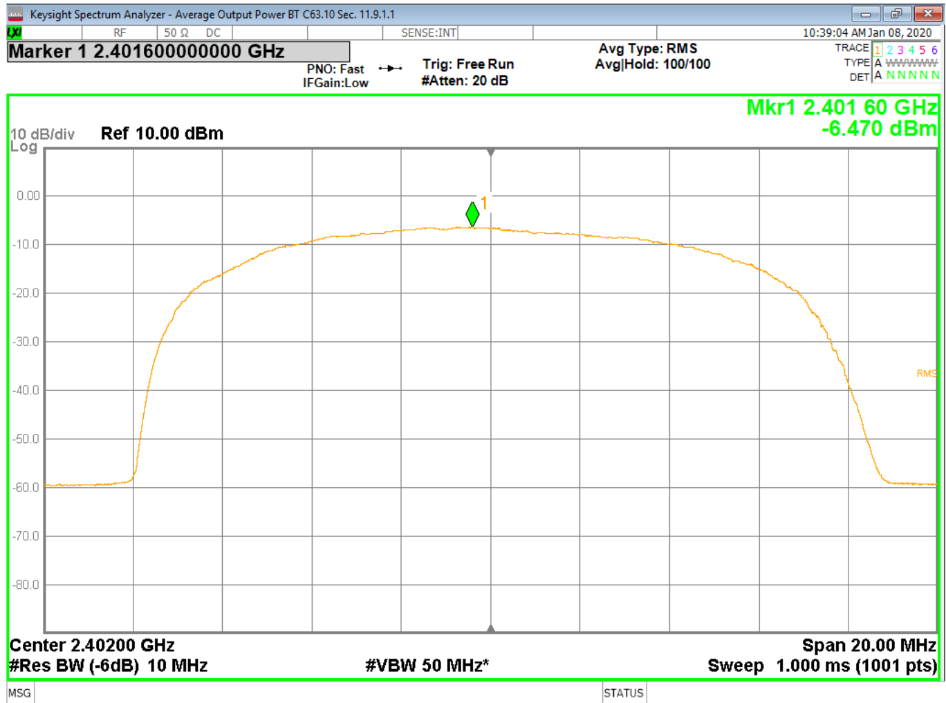
Figure 8 - Average Output Power, Low Channel, BT EDR 2MB
