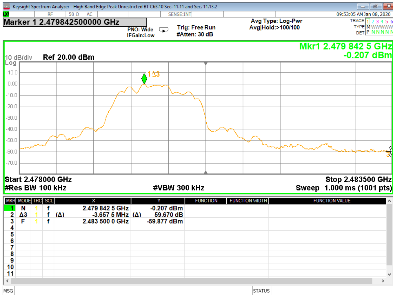
Figure 31 - Band-edge Measurement, High Channel, Fundamental, Peak
