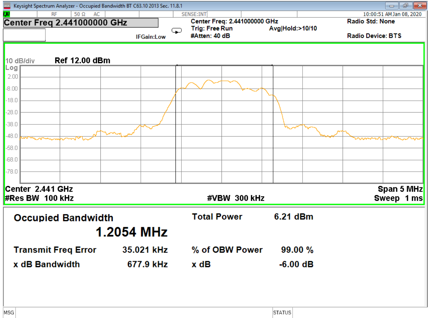
Figure 19 - Bandwidth, Mid Channel, BT EDR 2MB
