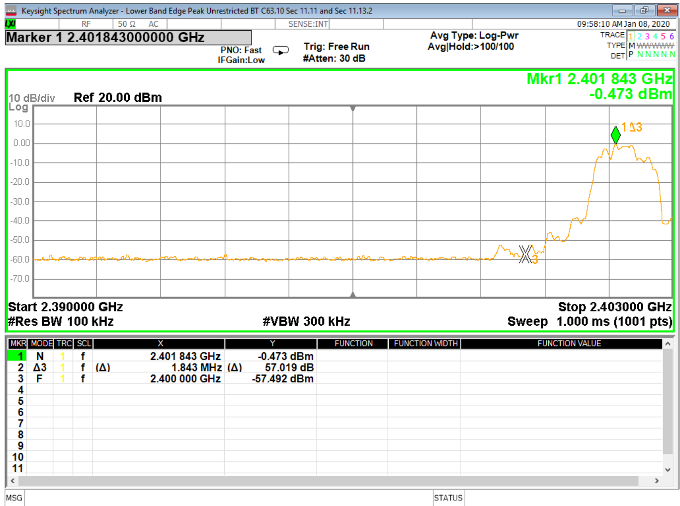
Figure 29 - Band-edge Measurement, Low Channel, Fundamental, Peak
