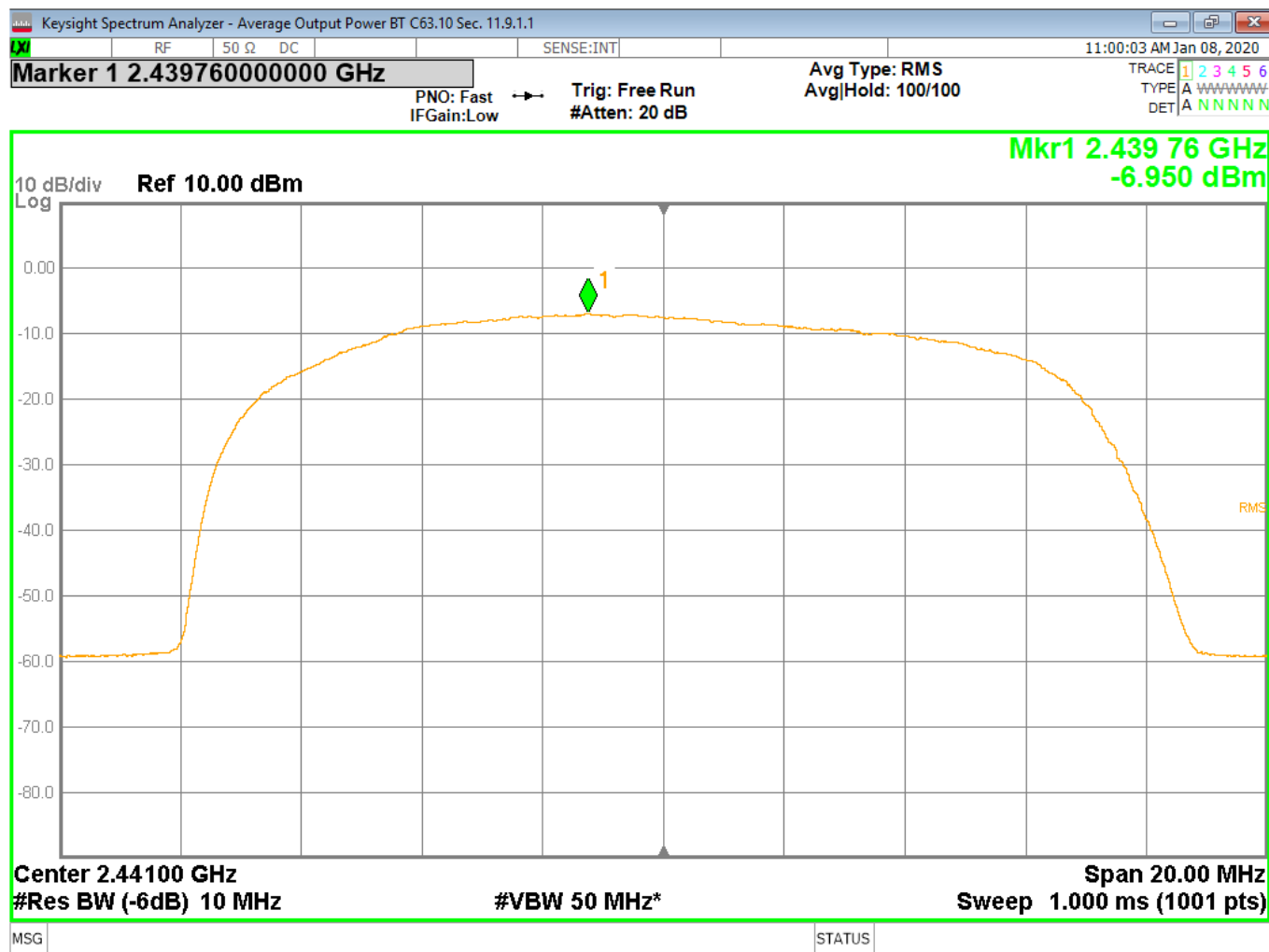
Figure 12 - Average Output Power, Mid Channel, BT EDR 3MB
