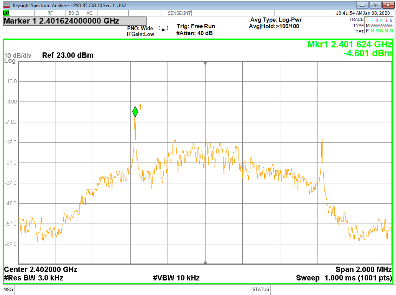
Figure 42 - Power Spectral Density, Low Channel, BT EDR 3MB
