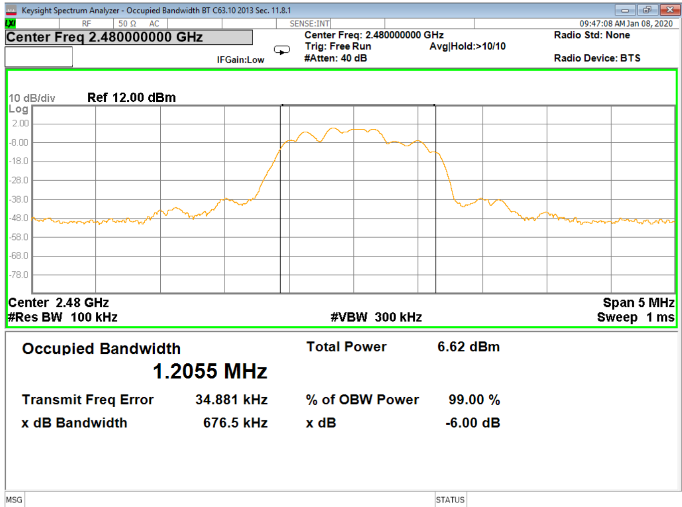
Figure 20 - Bandwidth, High Channel, BT EDR 2MB
