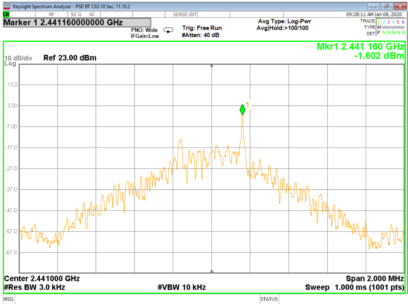
Figure 37 - Power Spectral Density, Mid Channel, BT BR (GFSK)
