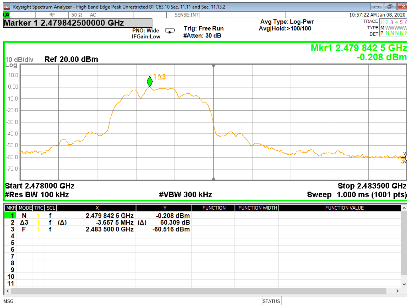
Figure 35 - Band-edge Measurement, High Channel, Fundamental, Peak
