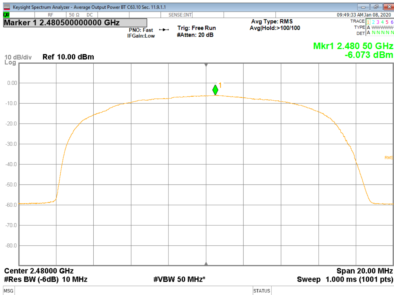
Figure 10 - Average Output Power, High Channel, BT EDR 2MB
