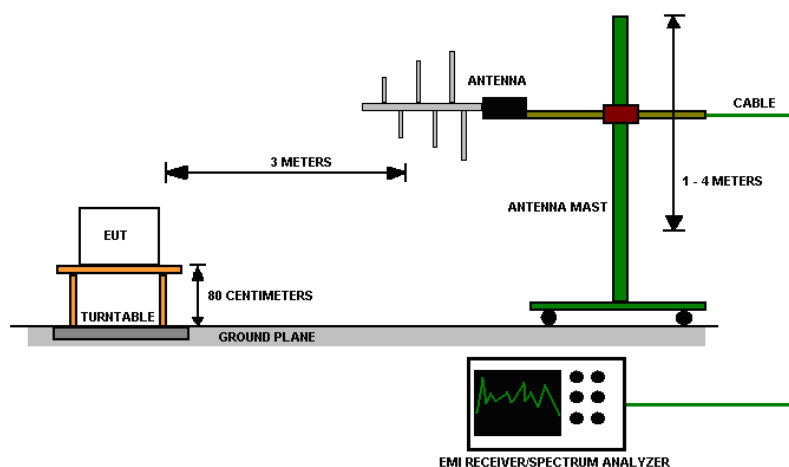
Figure 24 - Radiated Emissions Test Setup
