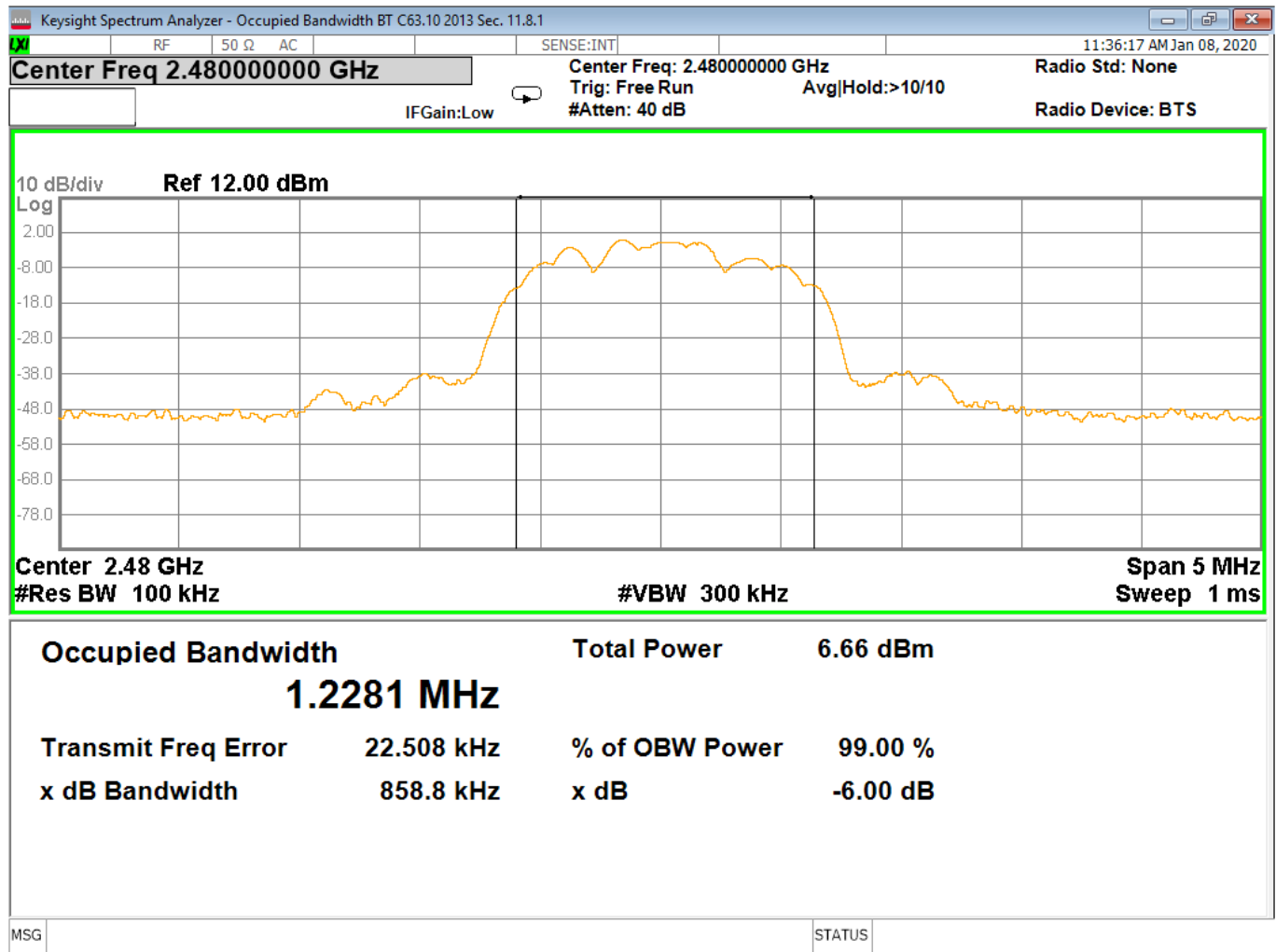
Figure 23 - Bandwidth, High Channel, BT EDR 3MB
