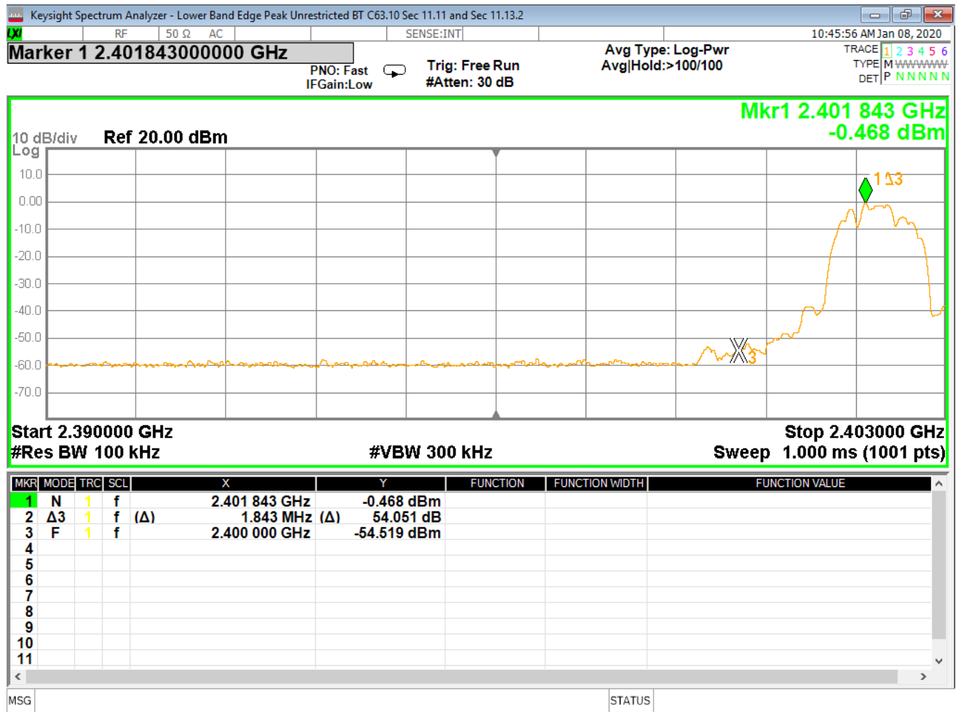
Figure 33 - Band-edge Measurement, Low Channel, Fundamental, Peak
