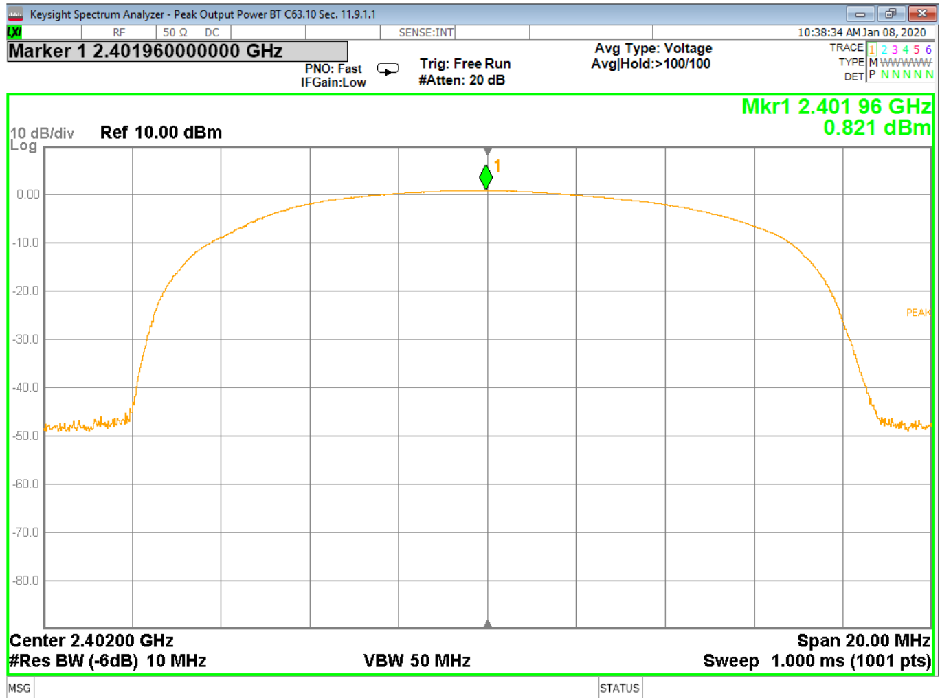
Figure 2 - Output Power, Low Channel, BT EDR 2MB
