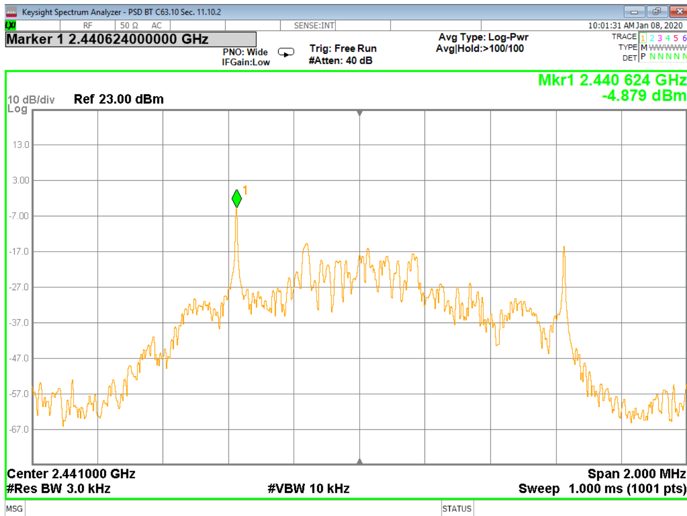
Figure 40 - Power Spectral Density, Mid Channel, BT EDR 2MB
