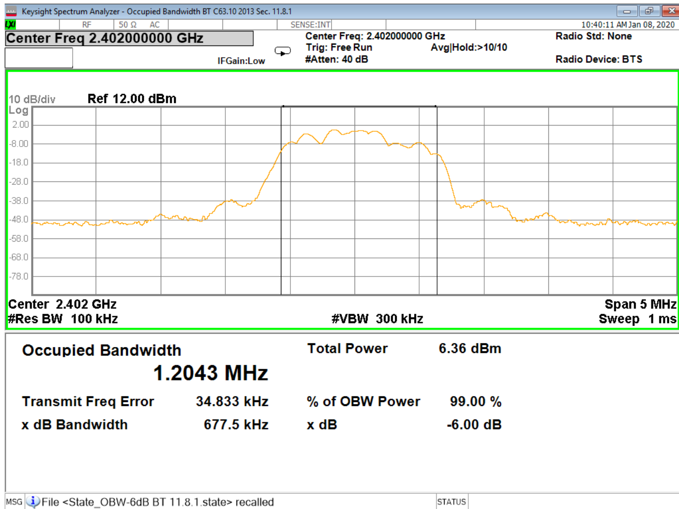
Figure 18 – Bandwidth, Low Channel, BT EDR 2MB
