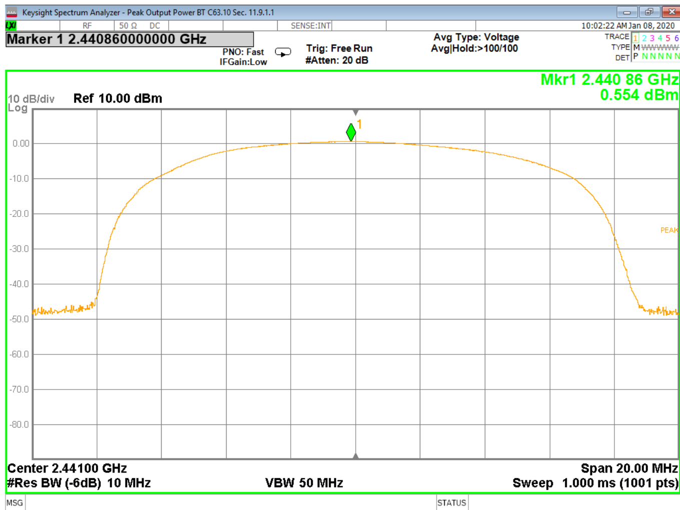
Figure 3 - Output Power, Mid Channel, BT EDR 2MB
