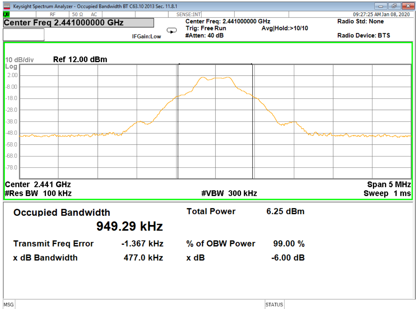
Figure 16 - Bandwidth, Mid Channel, BT BR (GFSK)
