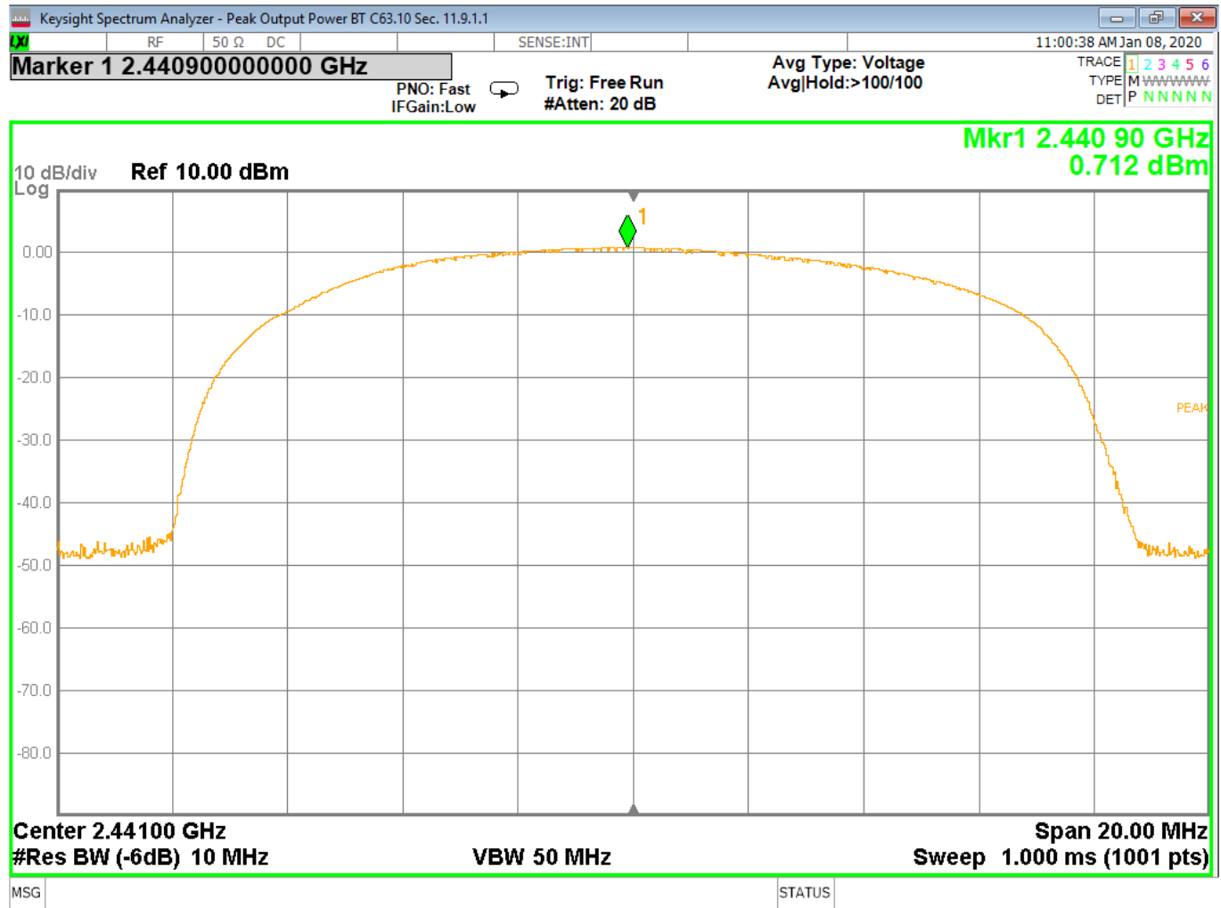
Figure 6 - Output Power, Mid Channel, BT EDR 3MB
