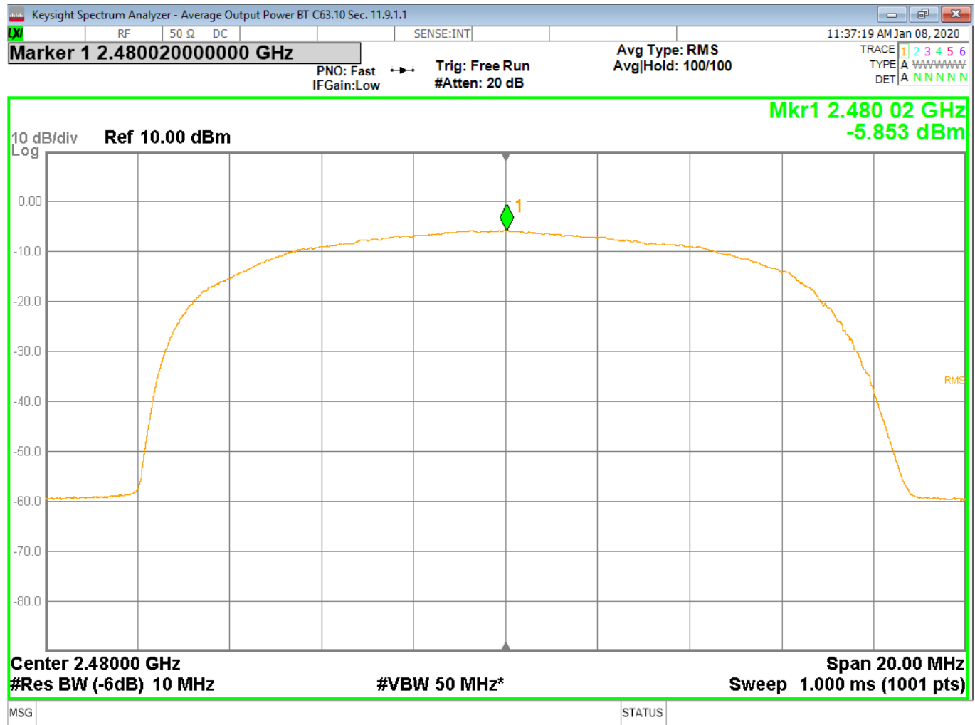
Figure 13 - Average Output Power, High Channel, BT EDR 3MB
