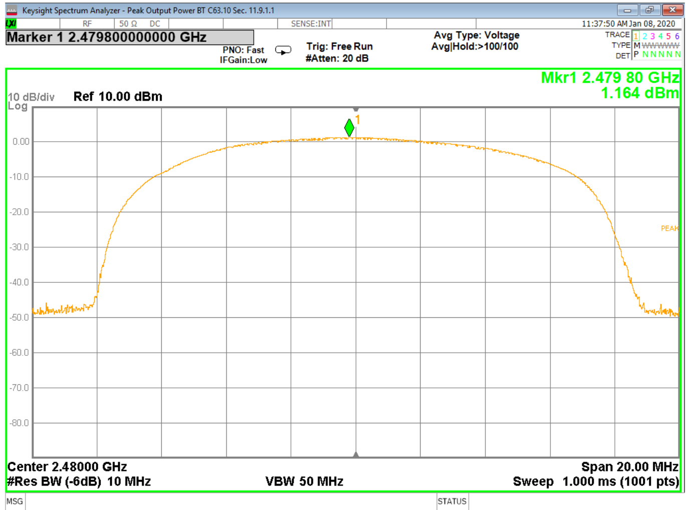
Figure 7 - Output Power, High Channel, BT EDR 3MB
