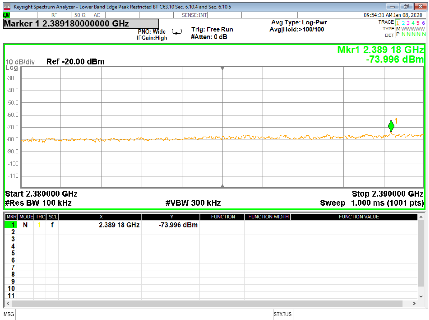
Figure 28 - Band-edge Measurement, Low Channel, Restricted Frequency, Peak
