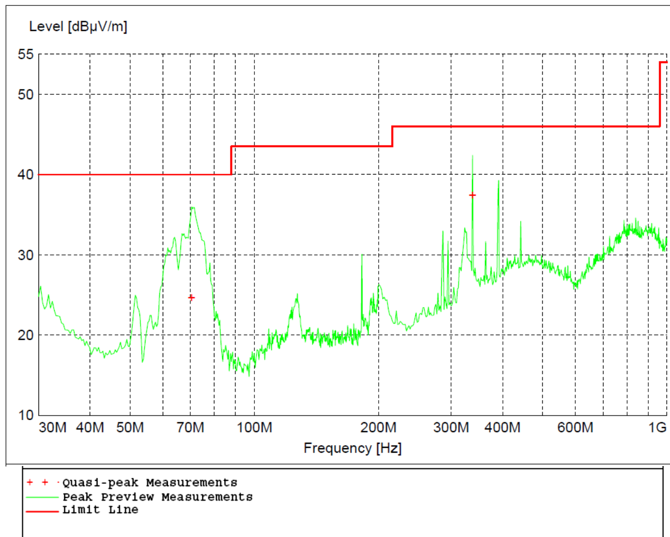
Figure 25 - Radiated Emissions Plot, Receive
