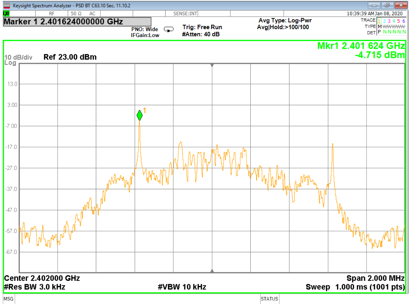
Figure 39 - Power Spectral Density, Low Channel, BT EDR 2MB
