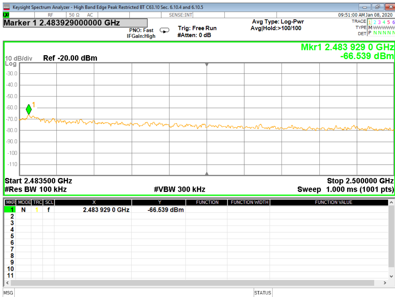
Figure 30 - Band-edge Measurement, High Channel, Restricted Frequency, Peak
