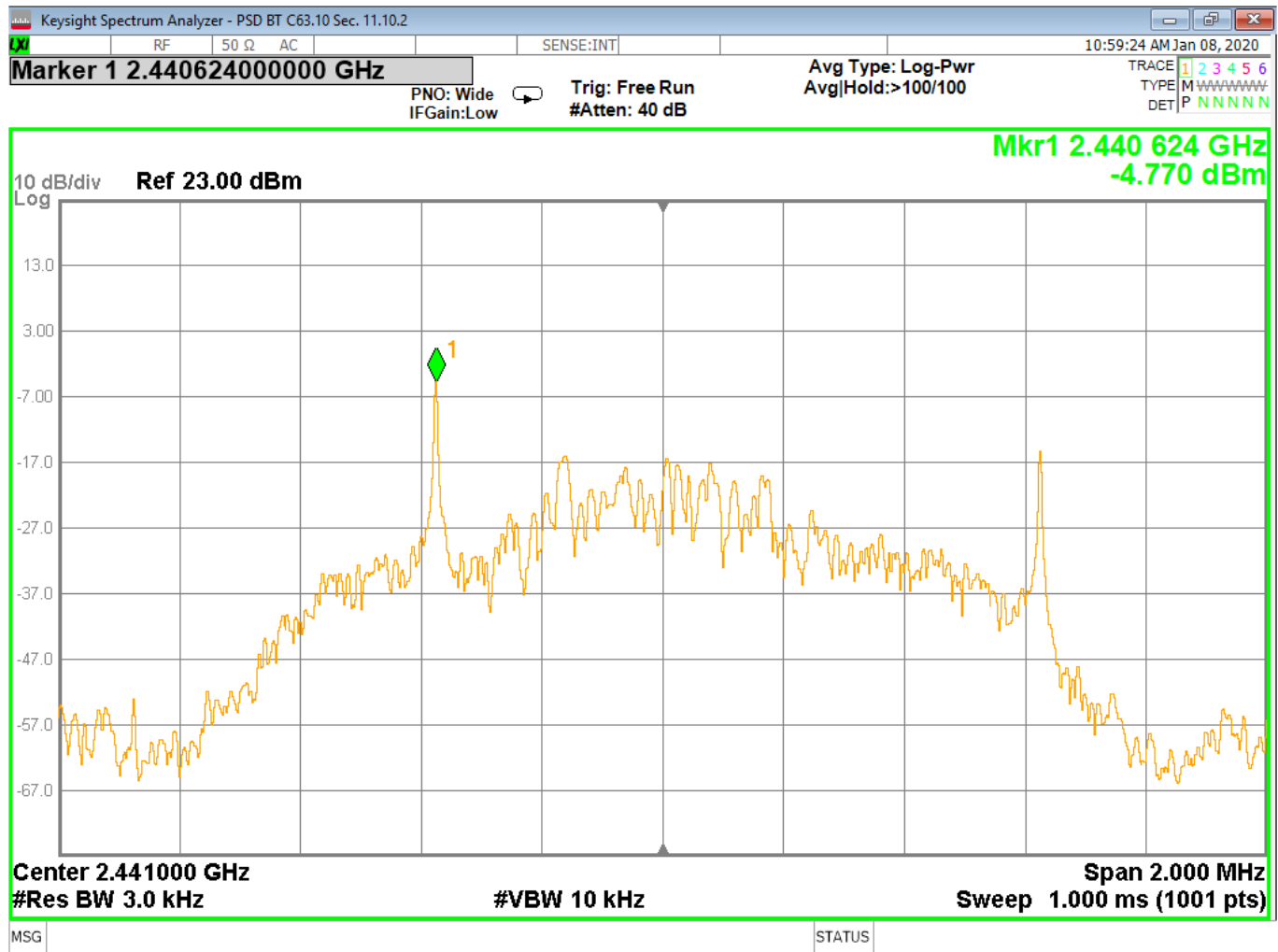
Figure 43 - Power Spectral Density, Mid Channel, BT EDR 3MB
