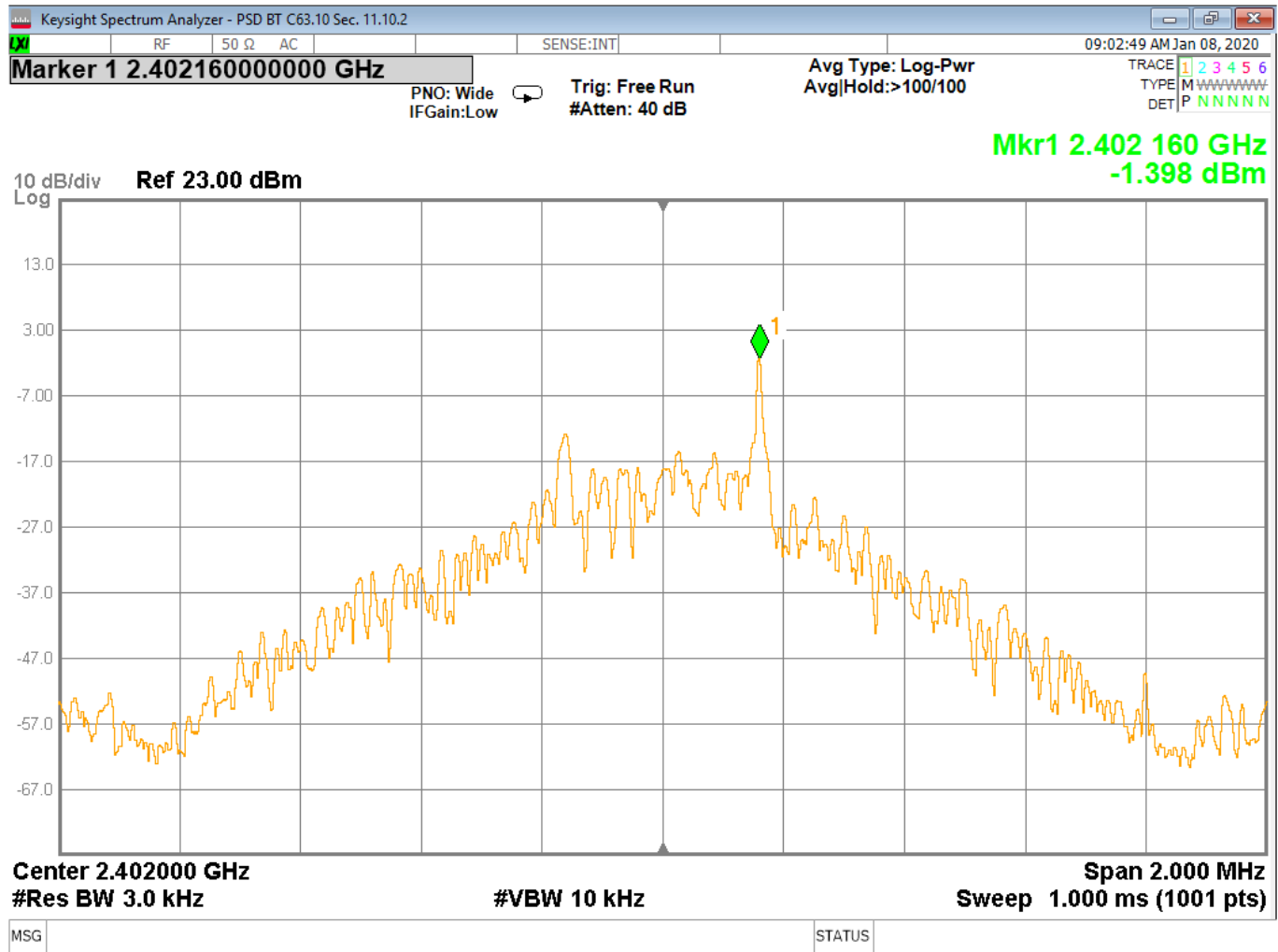
Figure 36 - Power Spectral Density, Low Channel, BT BR (GFSK)
