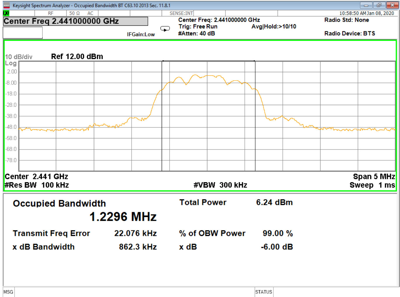
Figure 22 - Bandwidth, Mid Channel, BT EDR 3MB
