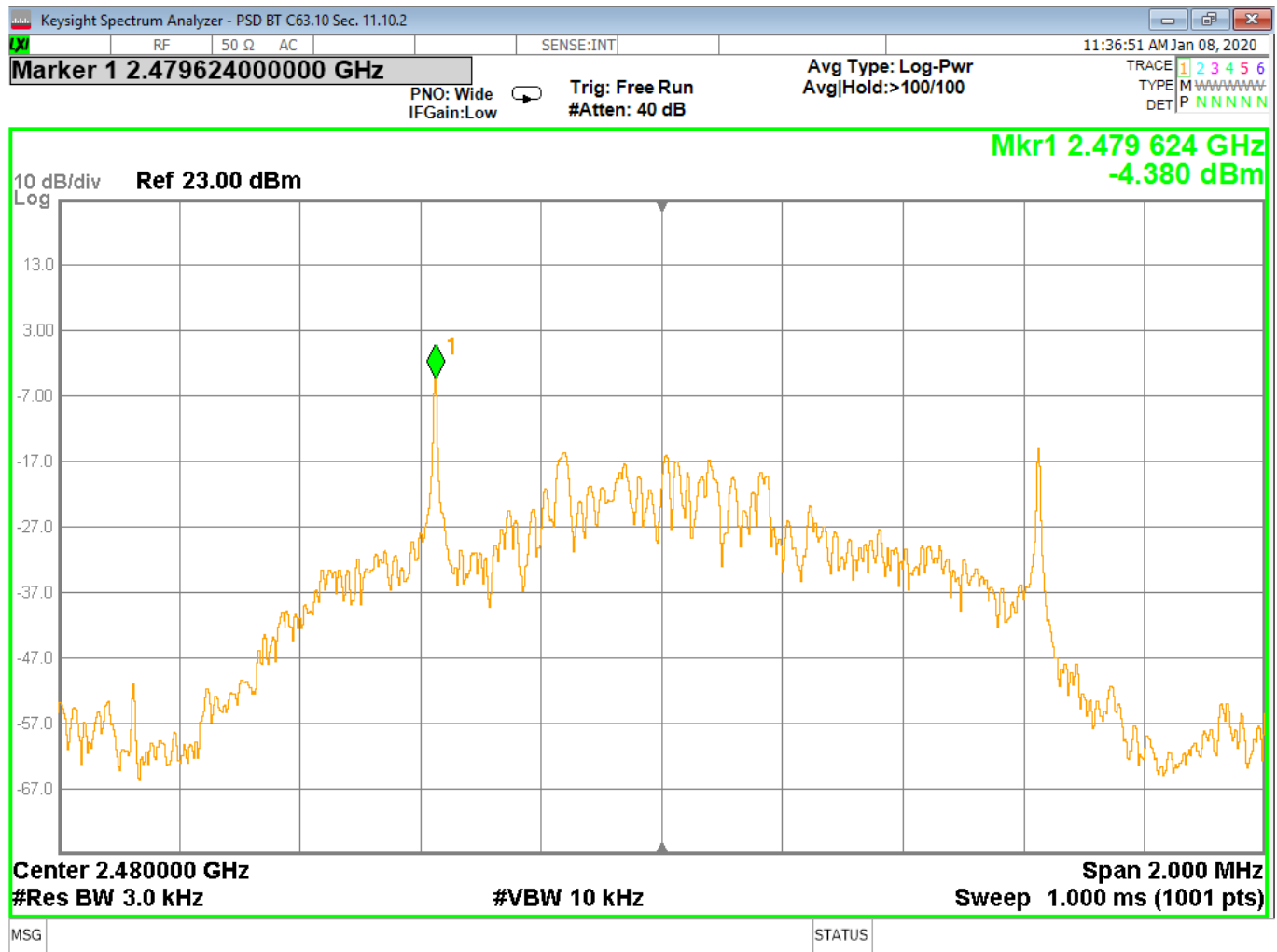
Figure 44 - Power Spectral Density, High Channel, BT EDR 3MB
