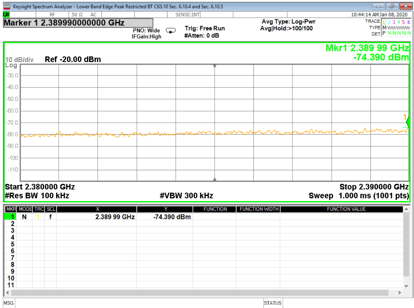
Figure 32 - Band-edge Measurement, Low Channel, Restricted Frequency, Peak
