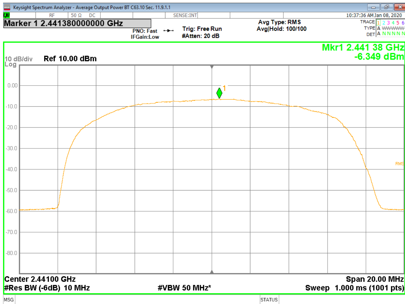
Figure 9 - Average Output Power, Mid Channel, BT EDR 2MB
