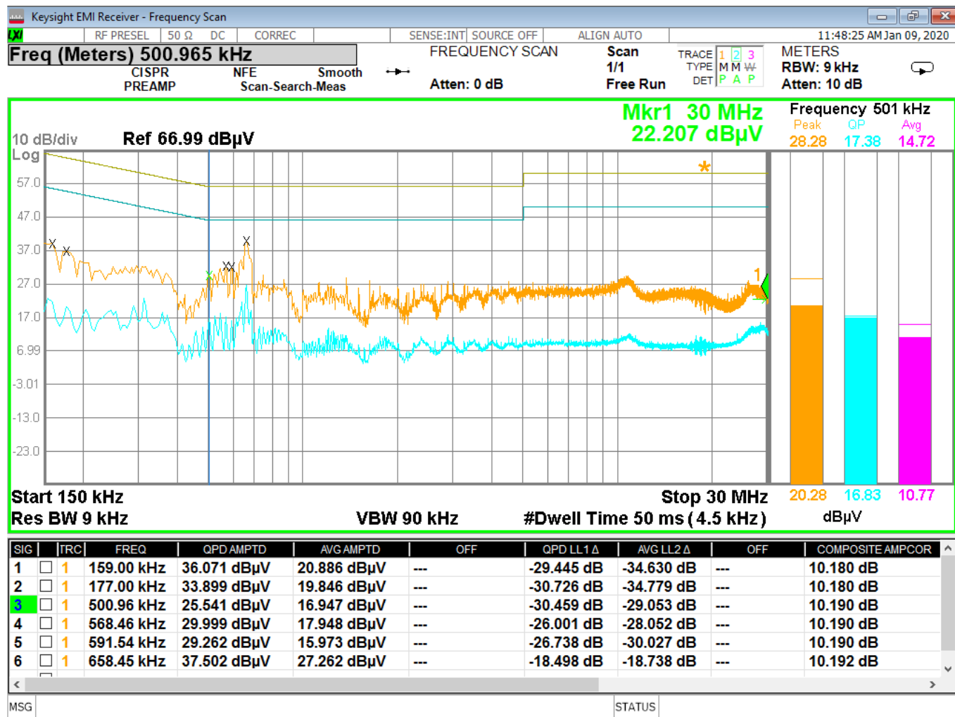
Figure 46 - Conducted Emissions, Neutral
