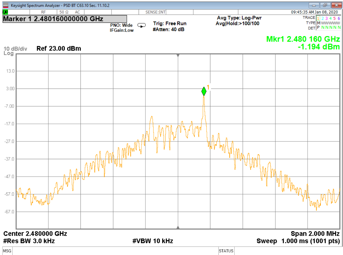
Figure 38 - Power Spectral Density, High Channel, BT BR (GFSK)
