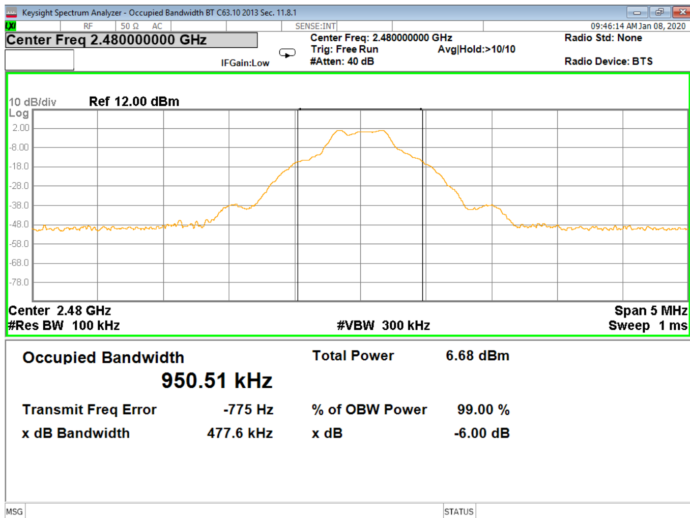
Figure 17 - Bandwidth, High Channel, BT BR (GFSK)
