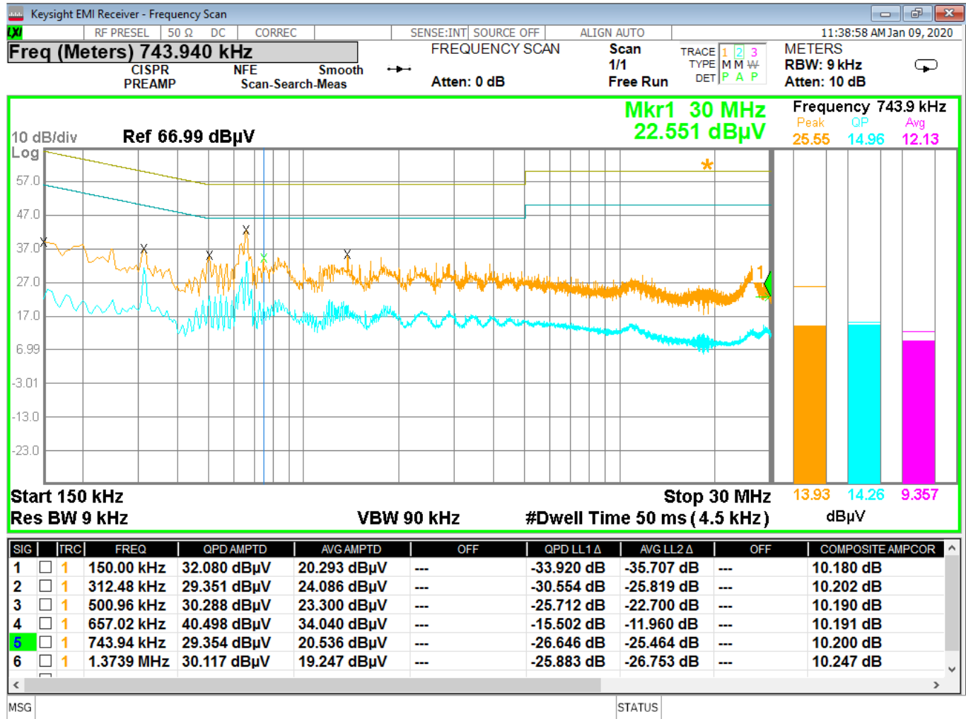
Figure 45 - Conducted Emissions, Line
