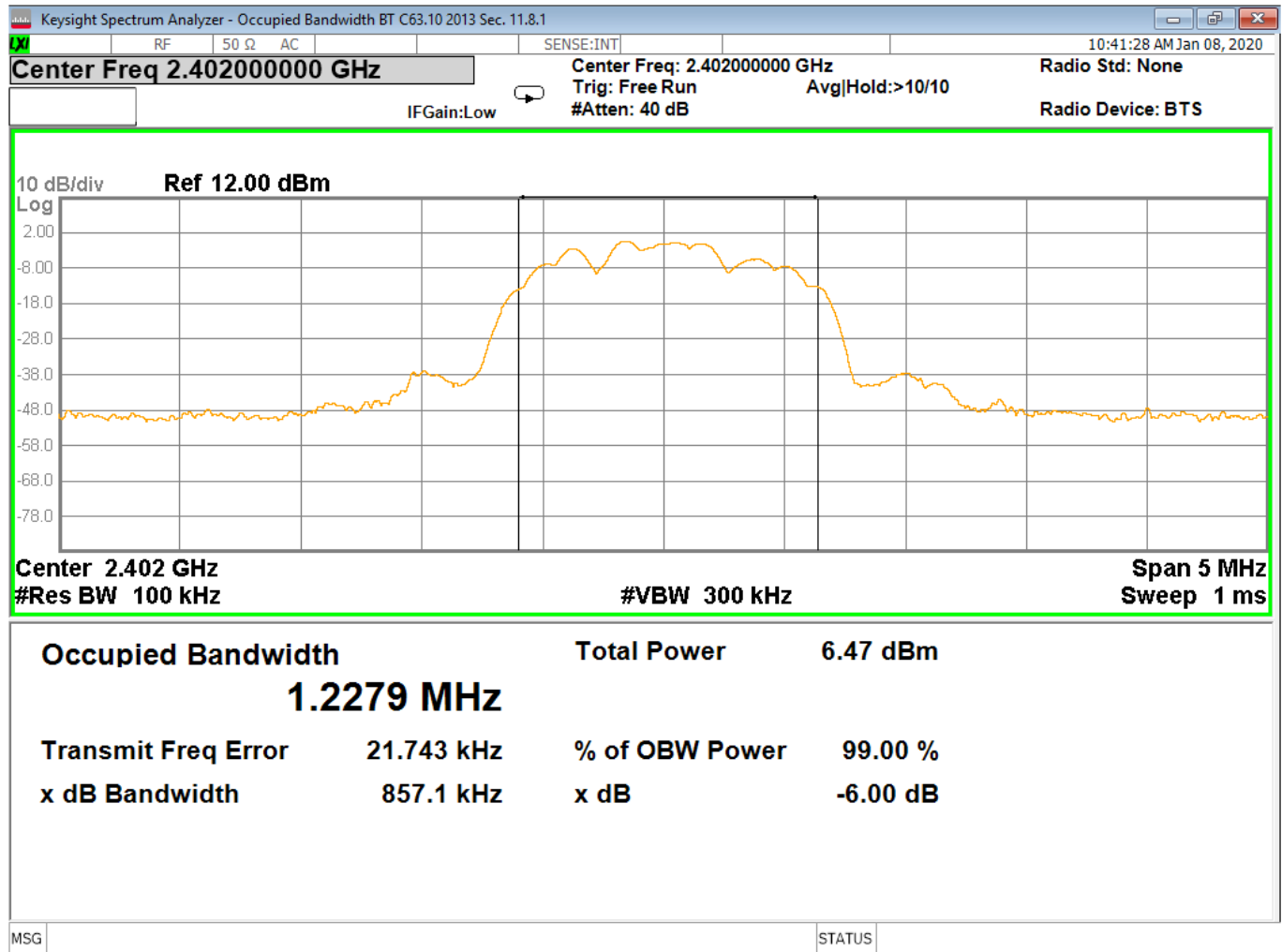
Figure 21 –Bandwidth, Low Channel, BT EDR 3MB
