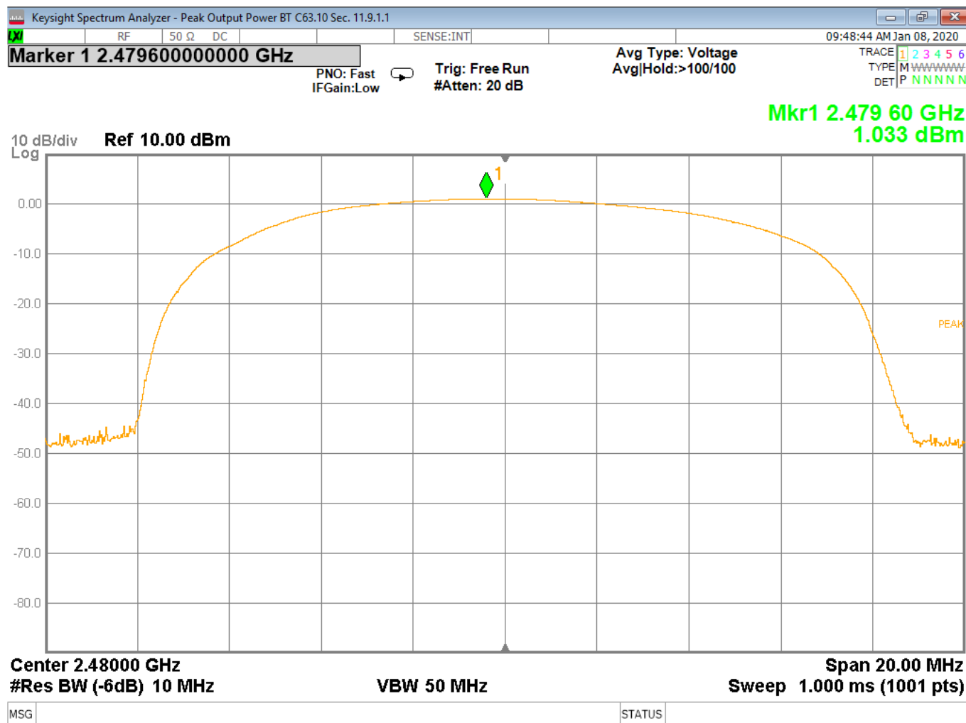
Figure 4 - Output Power, High Channel, BT EDR 2MB
