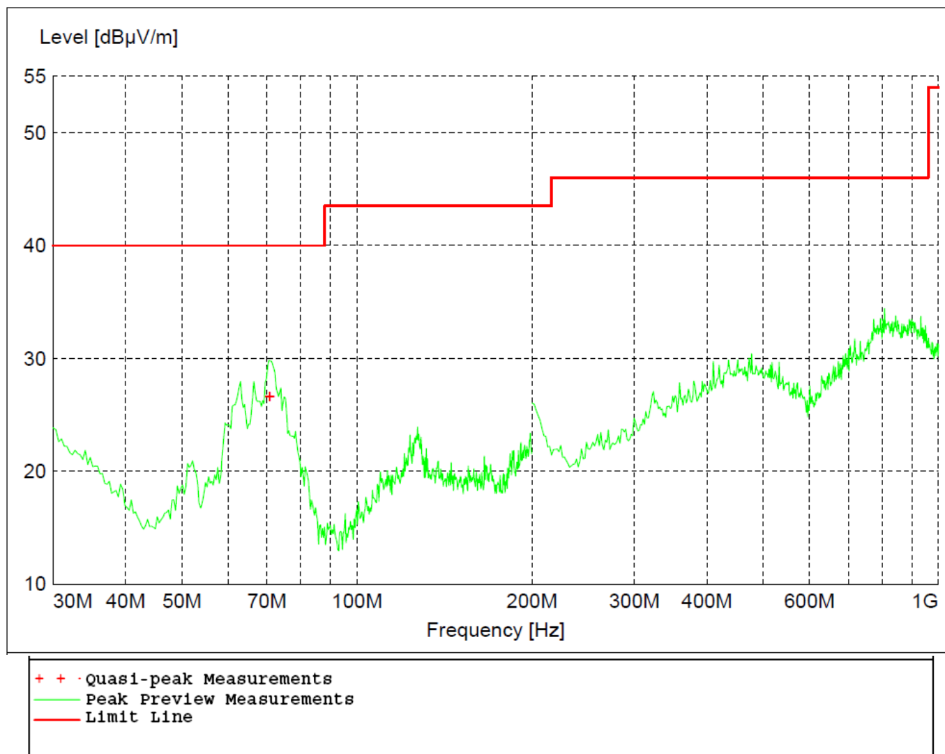
Figure 26 - Radiated Emissions Plot, 2EDR
