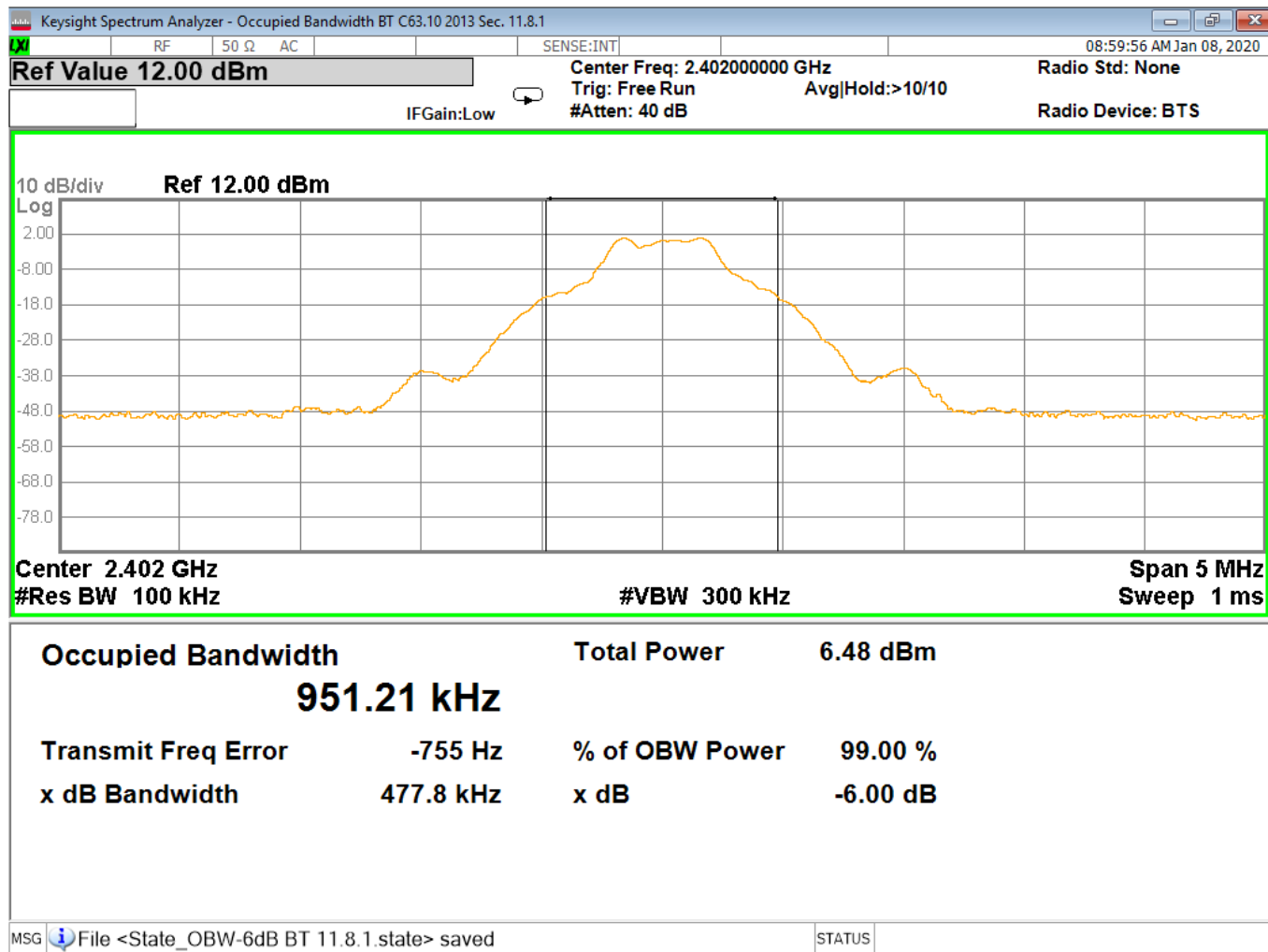
Figure 15 –Bandwidth, Low Channel, BT BR (GFSK)
