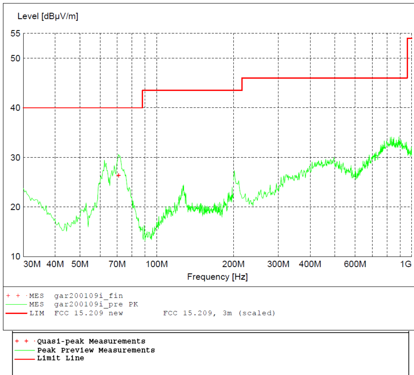
Figure 27 - Radiated Emissions Plot, 3EDR
