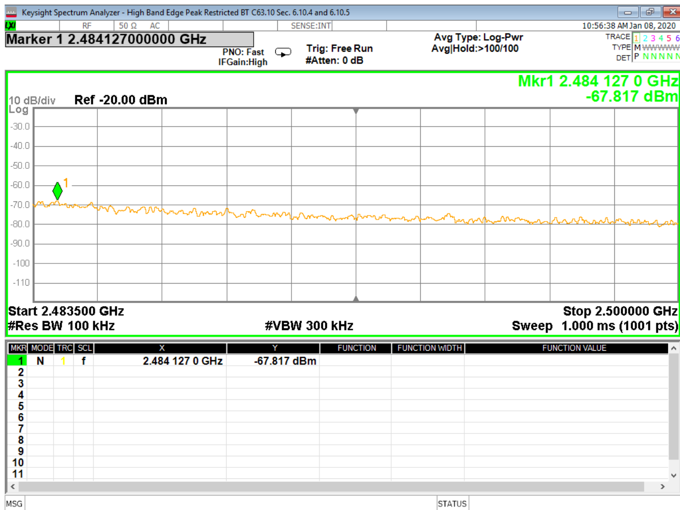
Figure 34 - Band-edge Measurement, High Channel, Restricted Frequency, Peak
