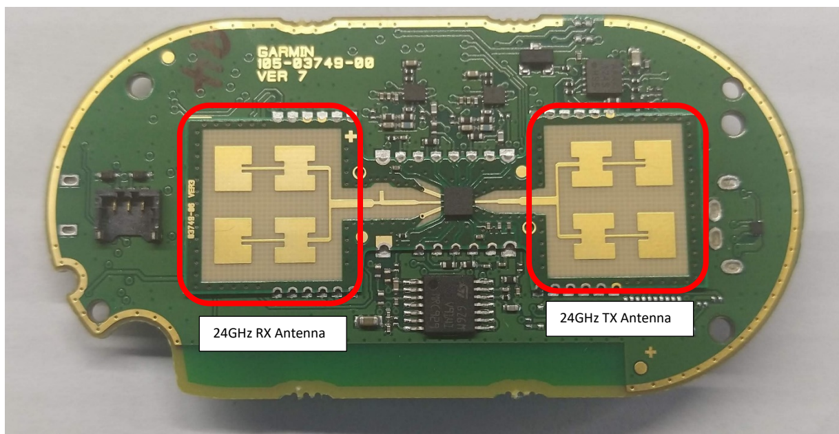
Figure 6 - PCB Front
