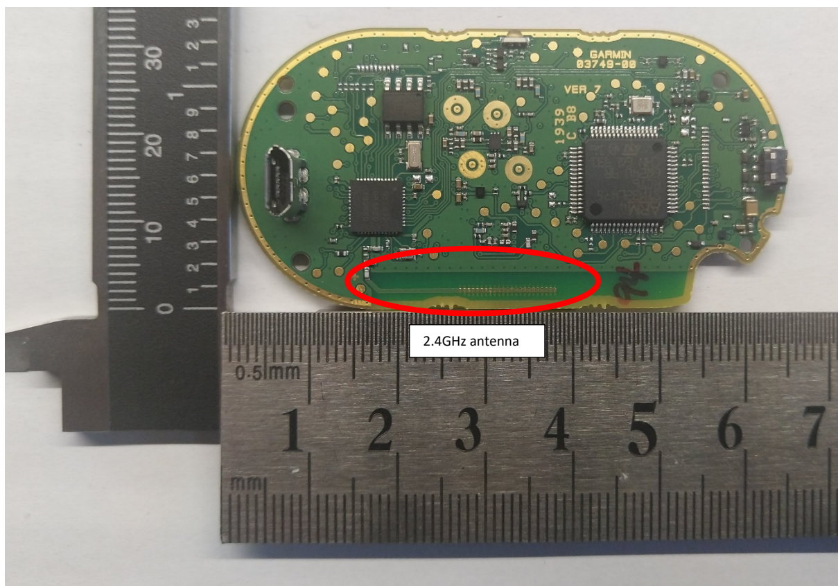
Figure 5 - PCB Rear
