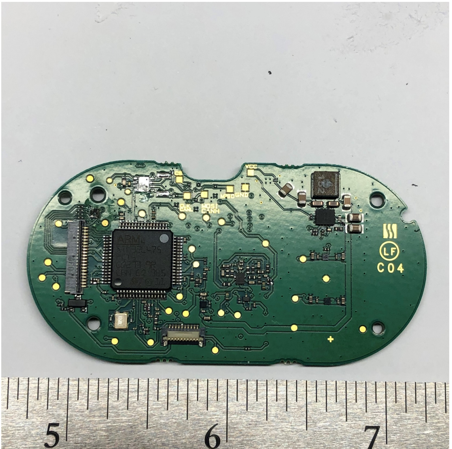
Figure 5 - PCB Rear
