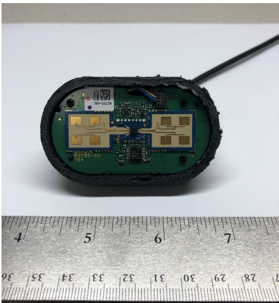
Figure 3 - Internal Front
