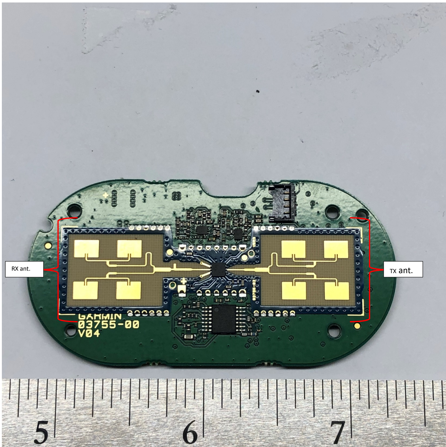
Figure 4- PCB Front
