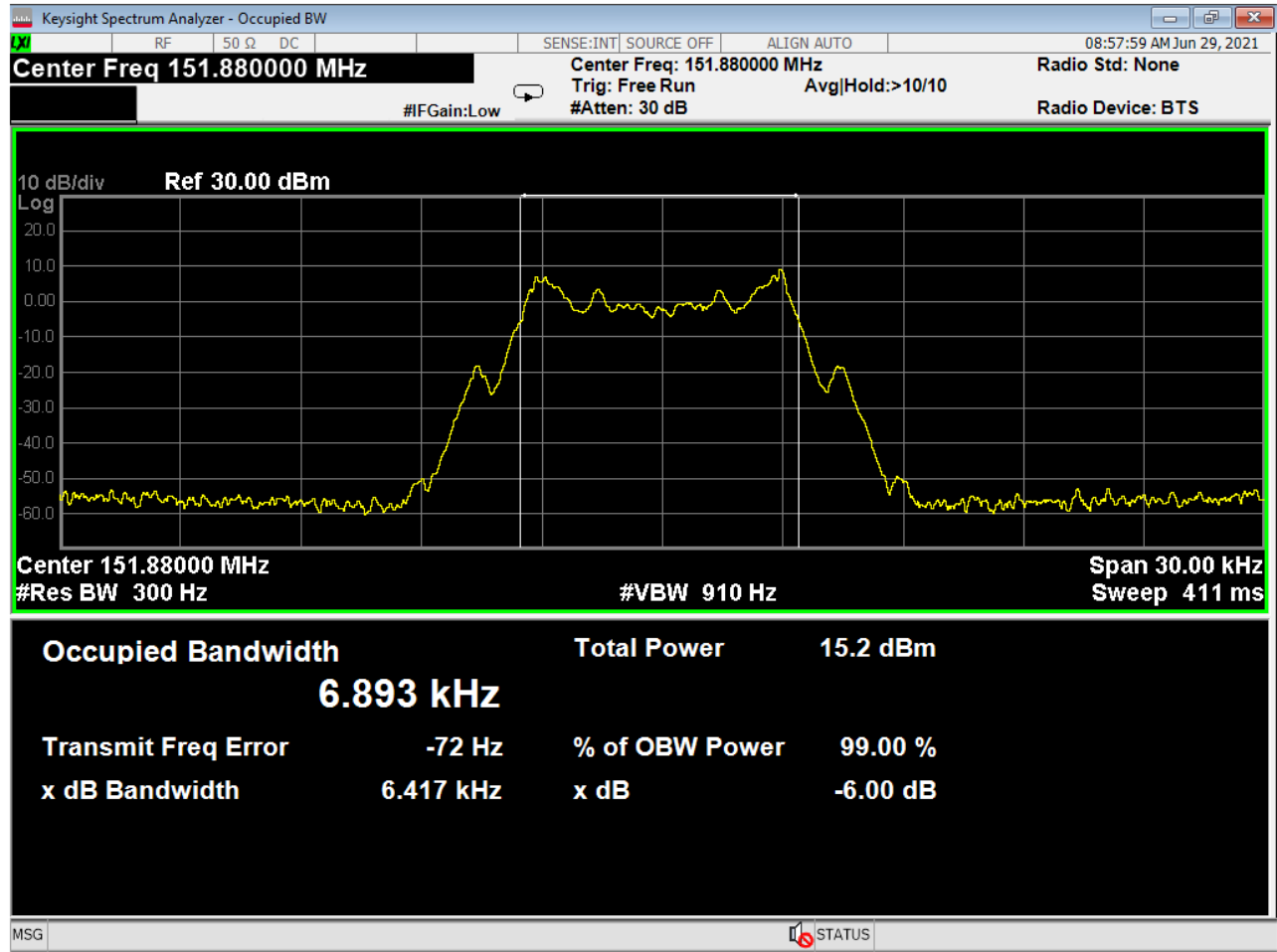
Figure 10 - Bandwidth, 151.880 MHz
