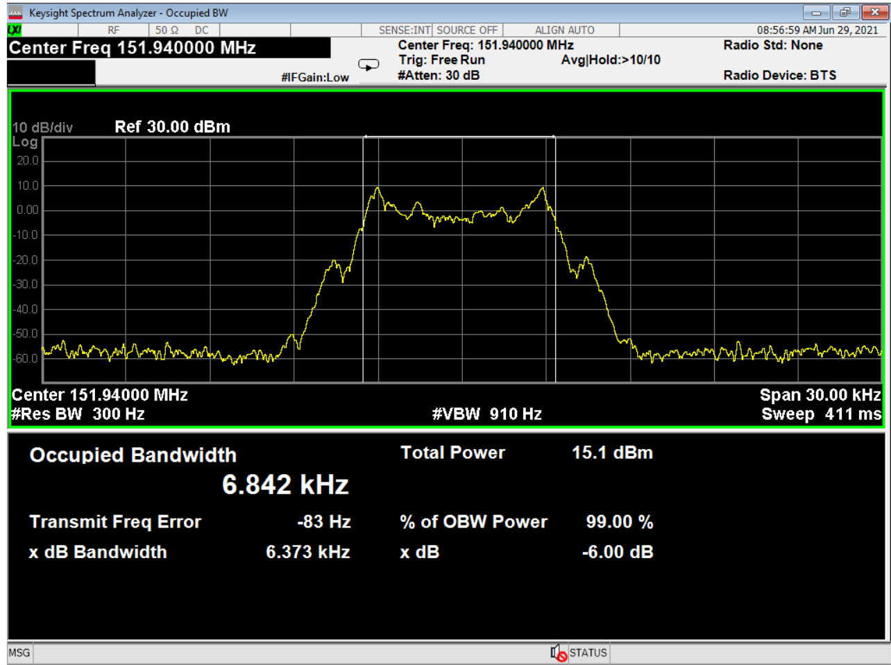
Figure 11 - Bandwidth, 151.940 MHz
