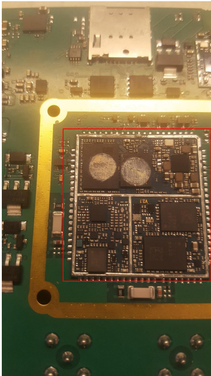
Internal Cellular Module (EG25-G)
