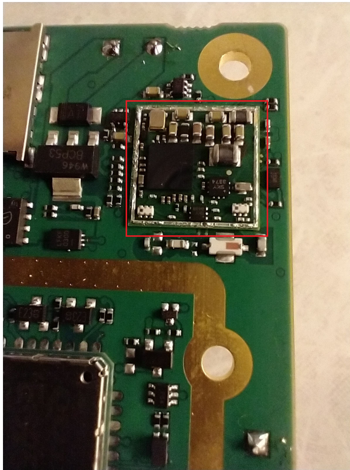
Internal WiFi 2/Bluetooth Module (WL1837MOD)
