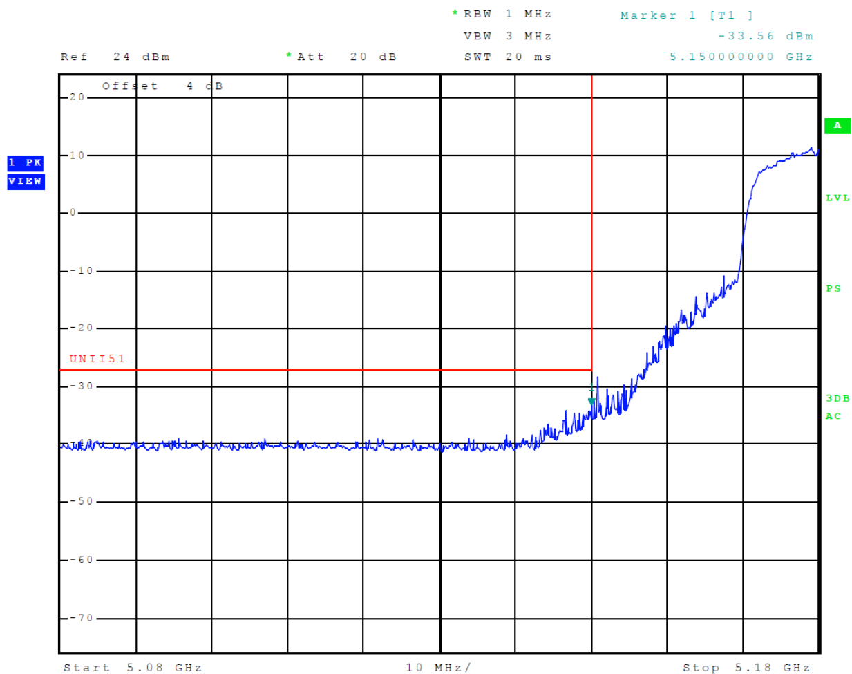
Figure 10 Plot of Lower Band Edge Across 5150-5250 MHz Band, Mode 10 (802.11n)
