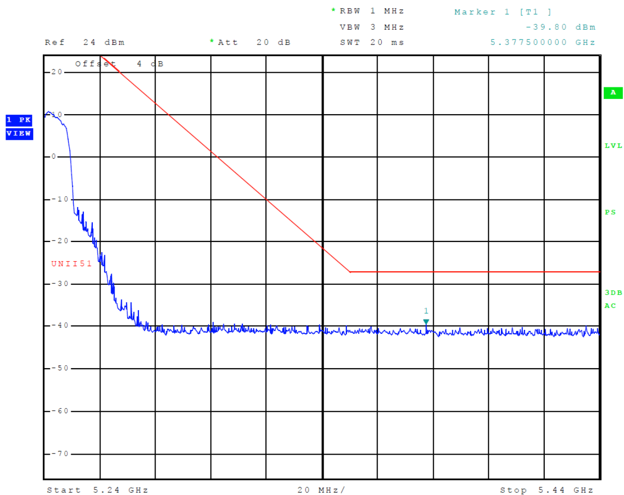
Figure 13 Plot of Upper Band Edge (Across 5150-5250 MHz Band, Mode 9 (802.11a))
