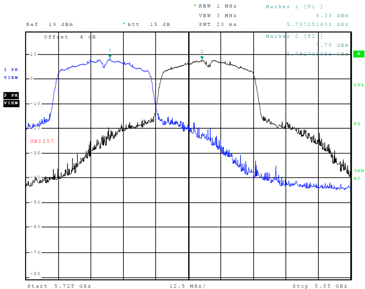
Figure 27 Plot of Transmitter Emissions (Across 5725-5850 MHz Band, Mode 15 (802.11n40))
