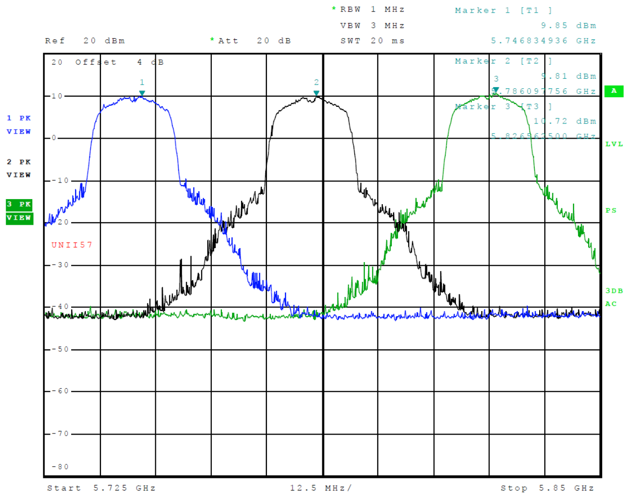
Figure 25 Plot of Transmitter Emissions (Across 5725-5850 MHz Band, Mode 13 (802.11a))
