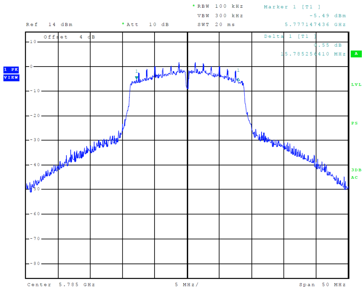
Figure 37 Plot of Transmitter 6-dB Occupied Bandwidth (5725-5850 MHz Mode 13 (802.11a))
