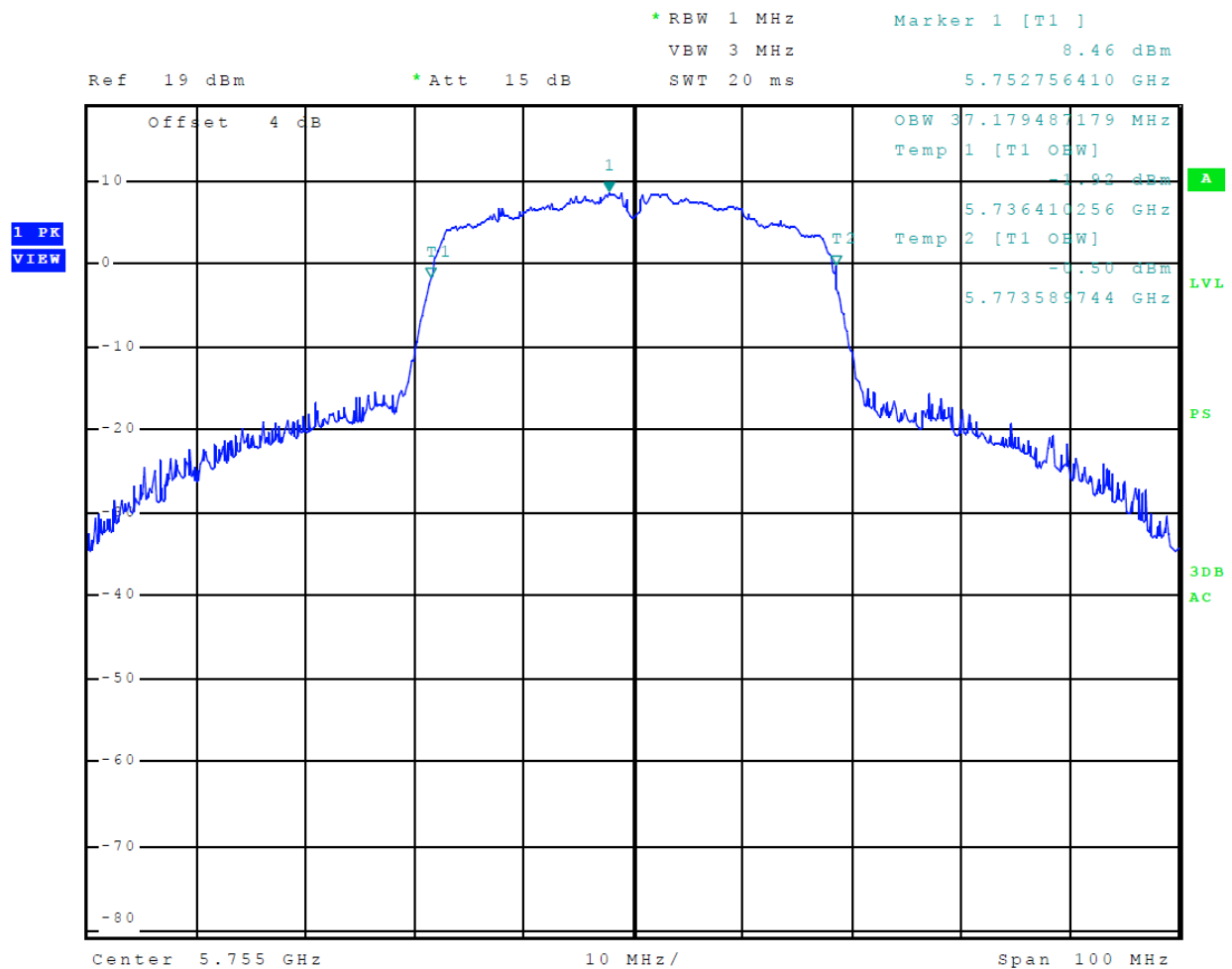
Figure 42 Plot of Transmitter 99% Occupied Bandwidth (5725-5850 MHz Mode 15 (802.11n40))
