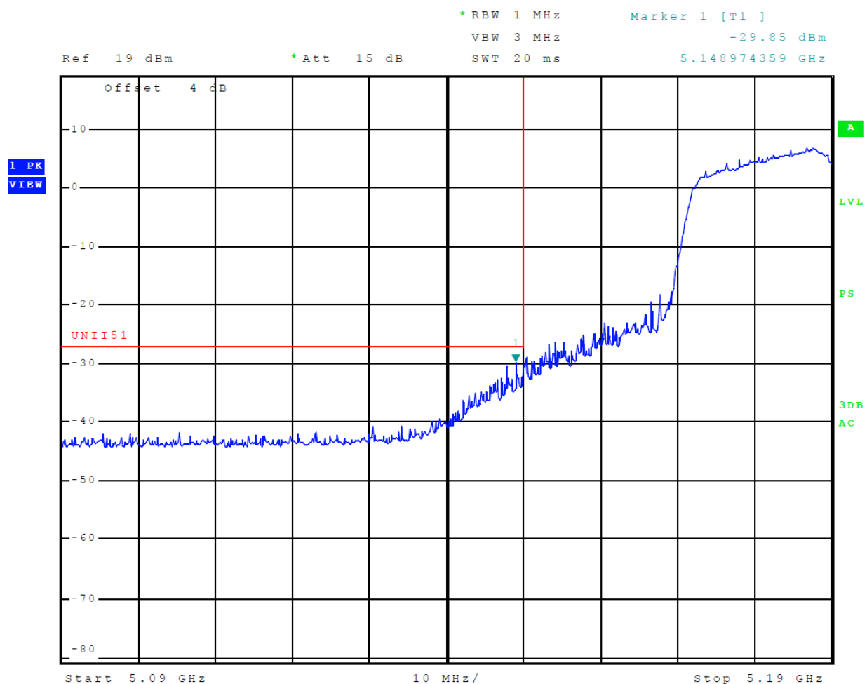
Figure 11 Plot of Lower Band Edge Across 5150-5250 MHz Band, Mode 11 (802.11n40)
