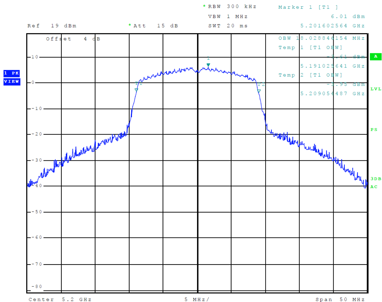
Figure 18 Plot of Transmitter 99% Occupied Bandwidth (5150-5250 MHz Mode 9 (802.11a))
