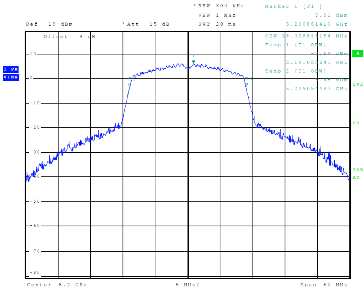
Figure 20 Plot of Transmitter 99% Occupied Bandwidth (5150-5250 MHz Mode 10 (802.11n))
