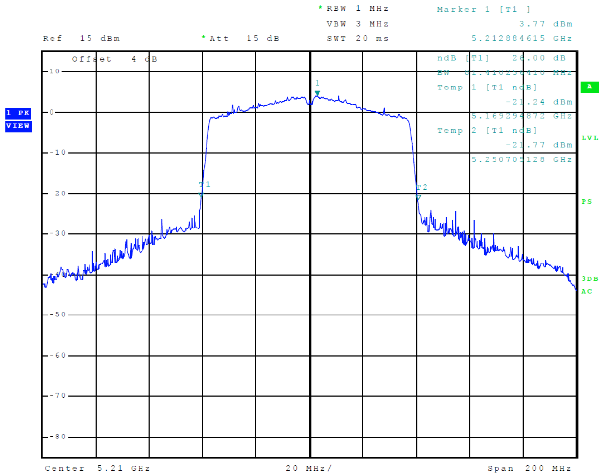
Figure 23 Plot of Transmitter 26-dB Occupied Bandwidth (5150-5250 MHz Mode 12 (802.11ac))
