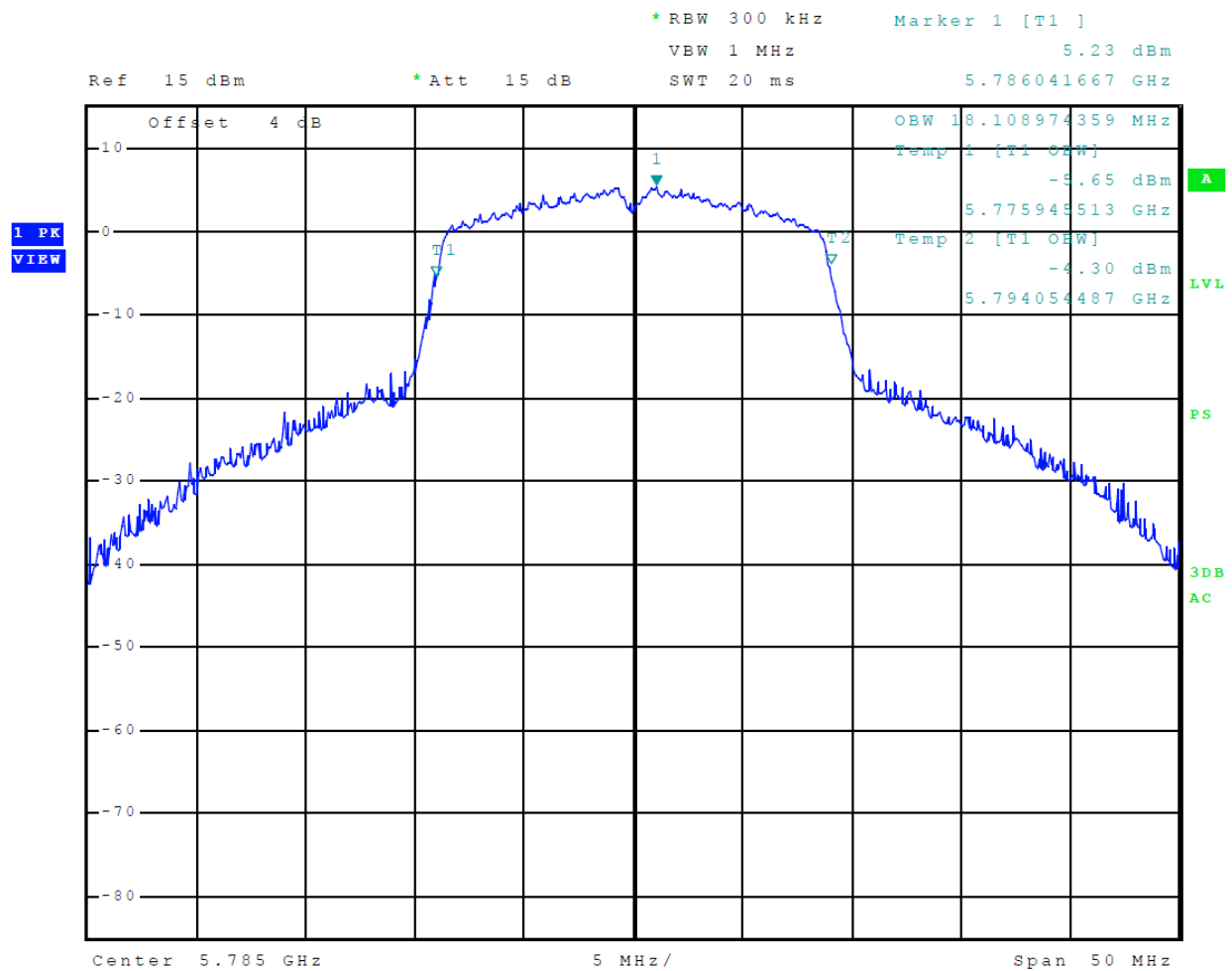
Figure 38 Plot of Transmitter 99% Occupied Bandwidth (5725-5850 MHz Mode 13 (802.11a))
