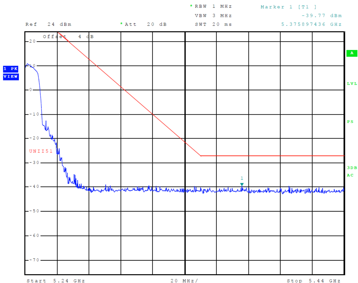
Figure 14 Plot of Upper Band Edge (Across 5150-5250 MHz Band, Mode 10 (802.11n))
