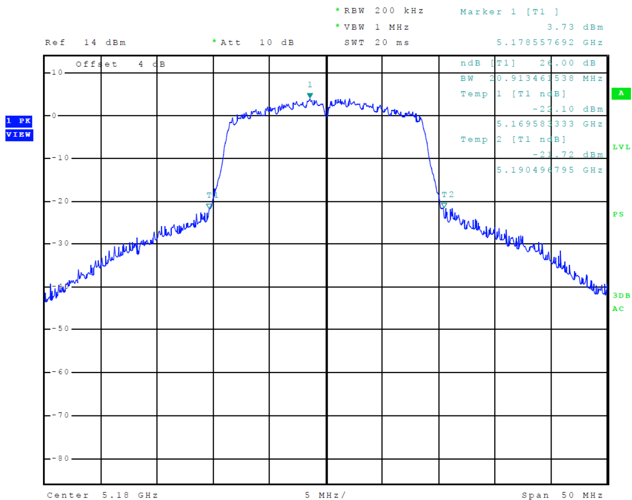
Figure 19 Plot of Transmitter 26-dB Occupied Bandwidth (5150-5250 MHz Mode 10 (802.11n))
