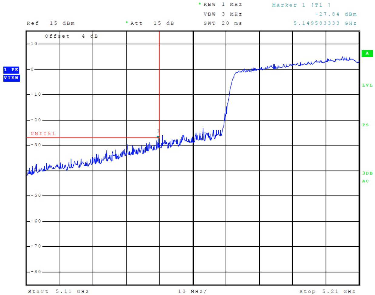
Figure 12 Plot of Lower Band Edge Across 5150-5250 MHz Band, Mode 12 (802.11ac)
