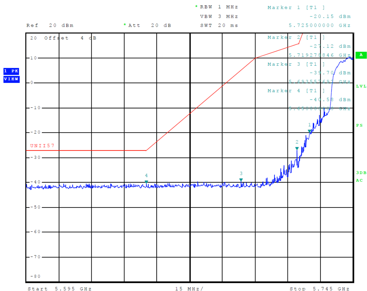
Figure 29 Plot of Lower Band Edge (Across 5725-5850 MHz Band, Mode 13 (802.11a))
