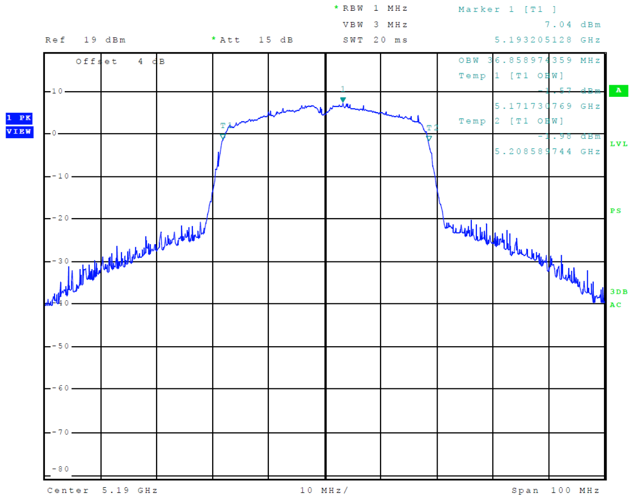
Figure 22 Plot of Transmitter 99% Occupied Bandwidth (5150-5250 MHz Mode 11 (802.11n40))
