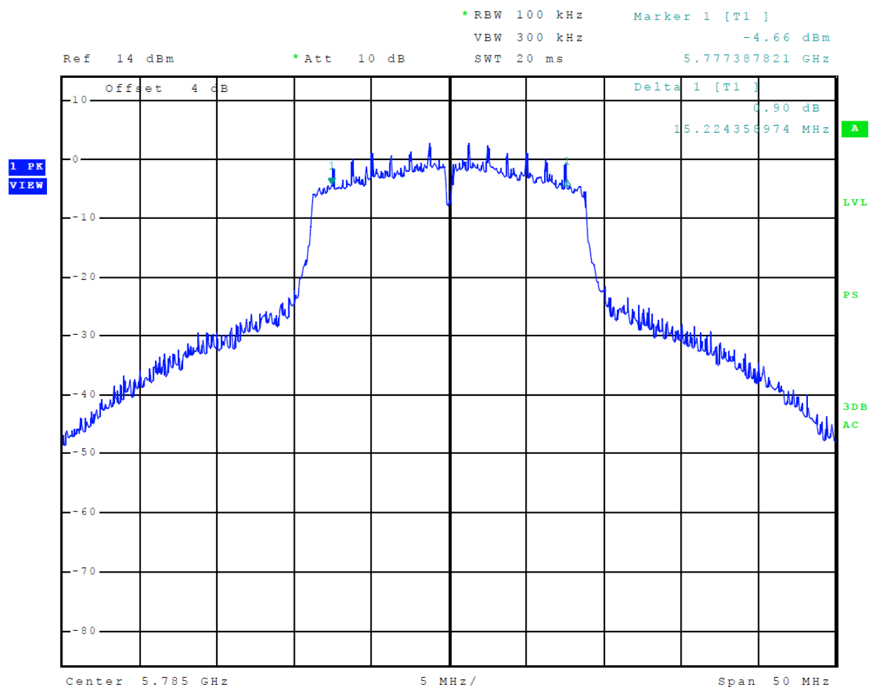
Figure 39 Plot of Transmitter 6-dB Occupied Bandwidth (5725-5850 MHz Mode 14 (802.11n))
