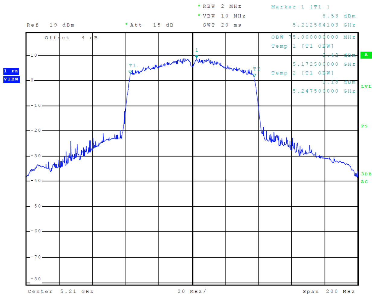
Figure 24 Plot of Transmitter 99% Occupied Bandwidth (5150-5250 MHz Mode 12 (802.11ac))
