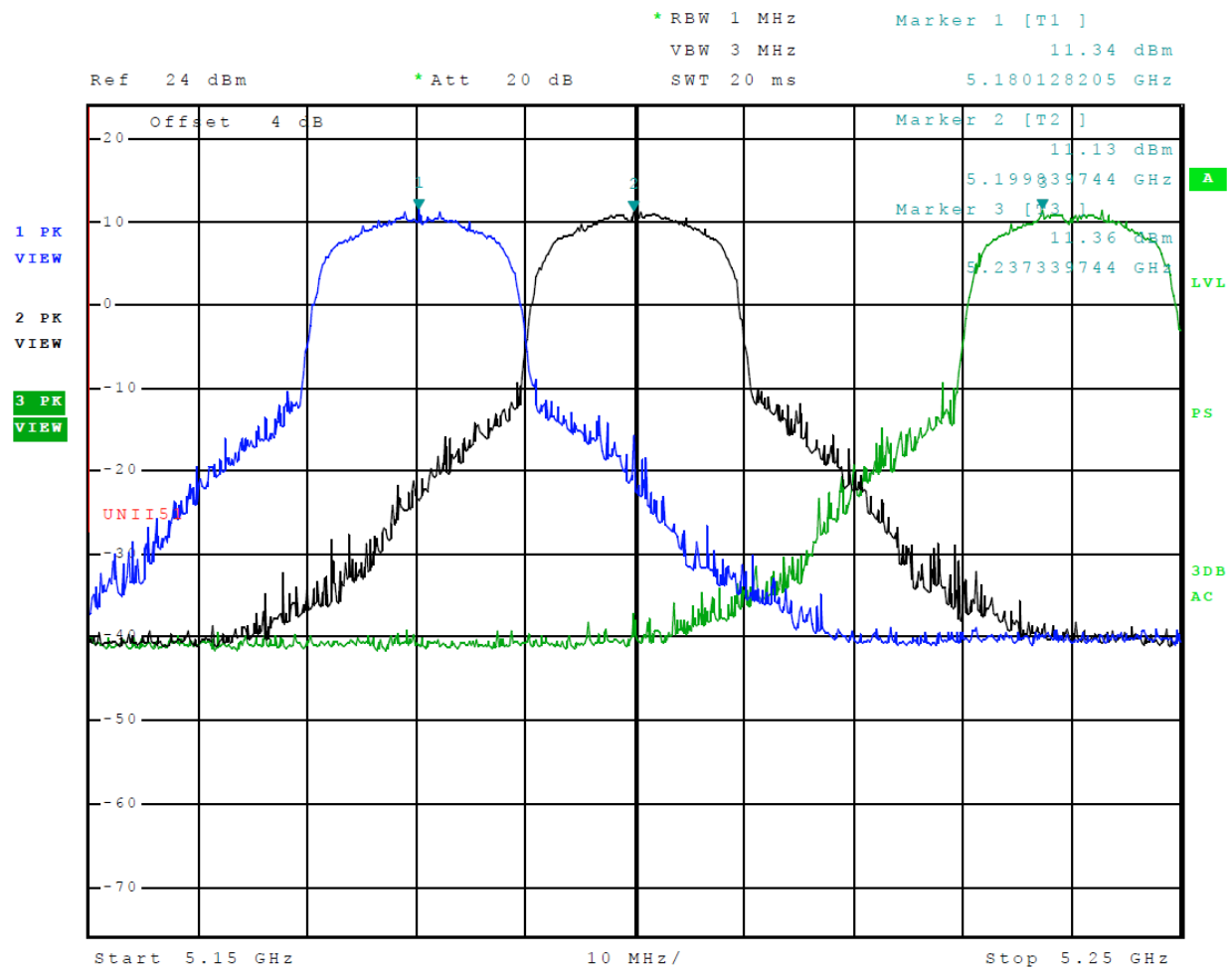
Figure 5 Plot of Transmitter Emissions Across 5150-5250 MHz Band, Mode 9 (802.11a)
