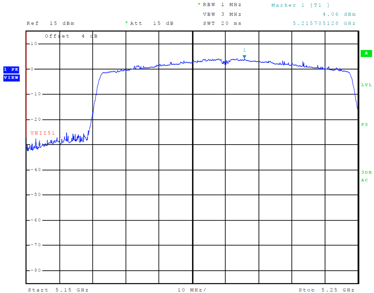
Figure 8 Plot of Transmitter Emissions Across 5150-5250 MHz Band, Mode 12 (802.11ac)
