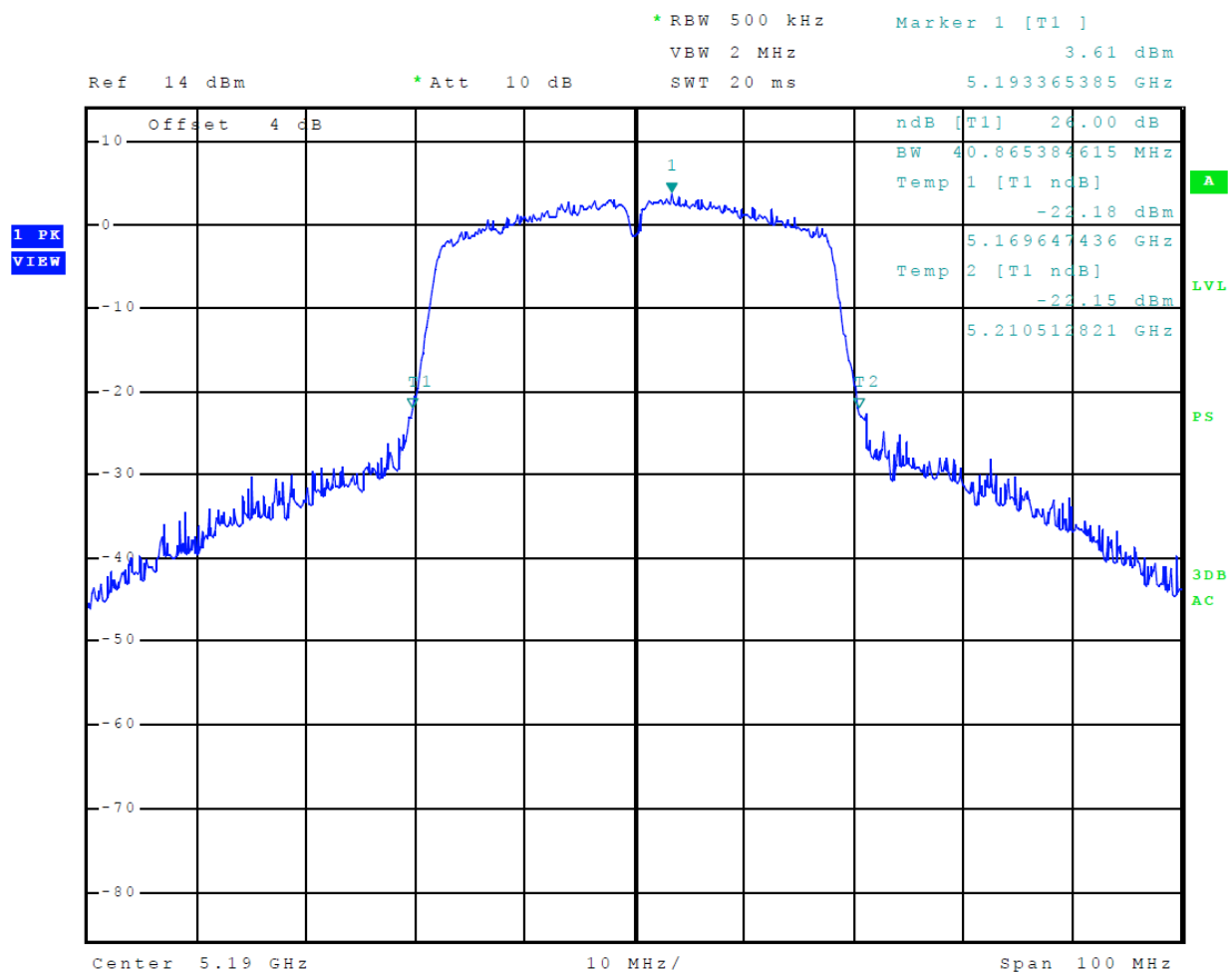
Figure 21 Plot of Transmitter 26-dB Occupied Bandwidth (5150-5250 MHz Mode 11 (802.11n40))
