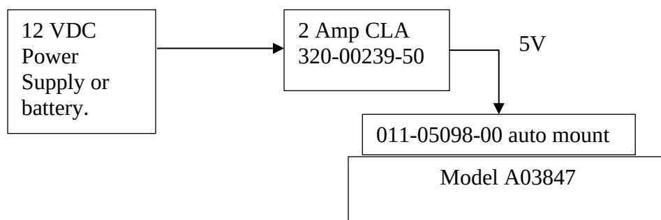
Fig. 2. Configuration 2. Automobile Mounting.
