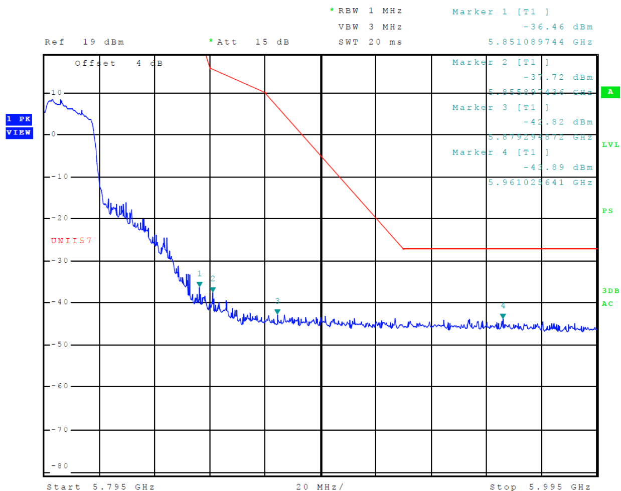
Figure 35 Plot of Upper Band Edge (Across 5725-5850 MHz Band, Mode 15 (802.11n40))
