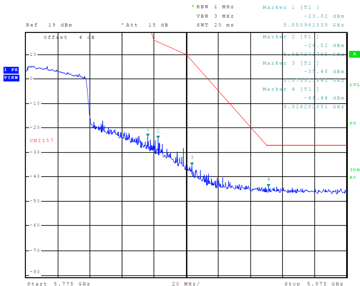
Figure 36 Plot of Upper Band Edge (Across 5725-5850 MHz Band, Mode 16 (802.11ac))
