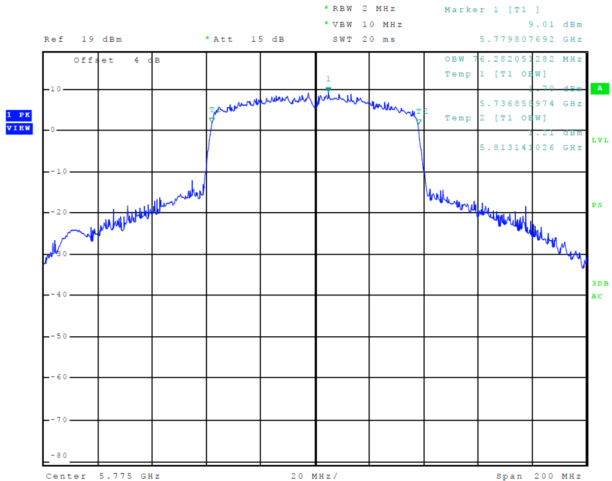
Figure 44 Plot of Transmitter 99% Occupied Bandwidth (5725-5850 MHz Mode 16 (802.11ac))
