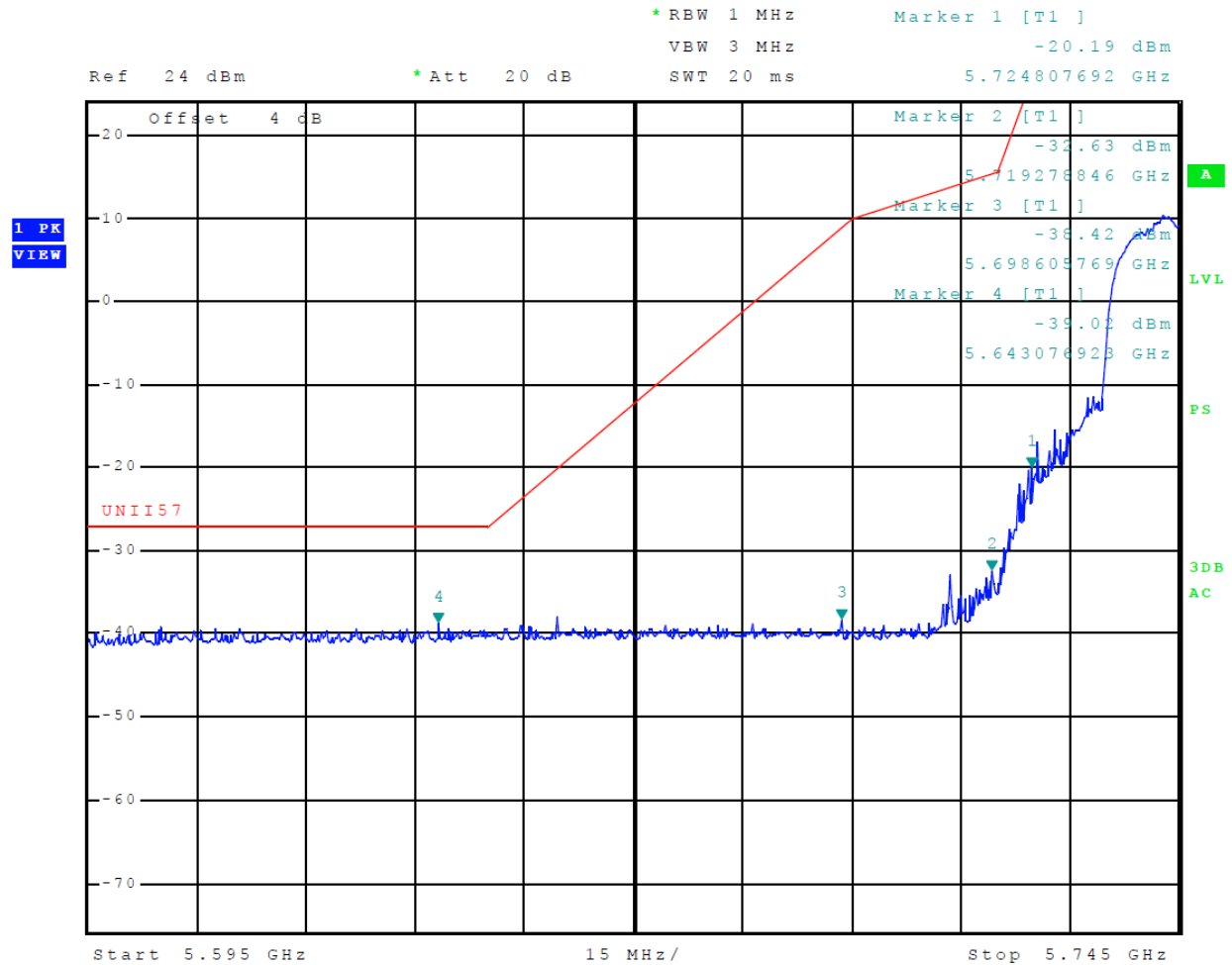
Figure 30 Plot of Lower Band Edge (Across 5725-5850 MHz Band, Mode 14 (802.11n))
