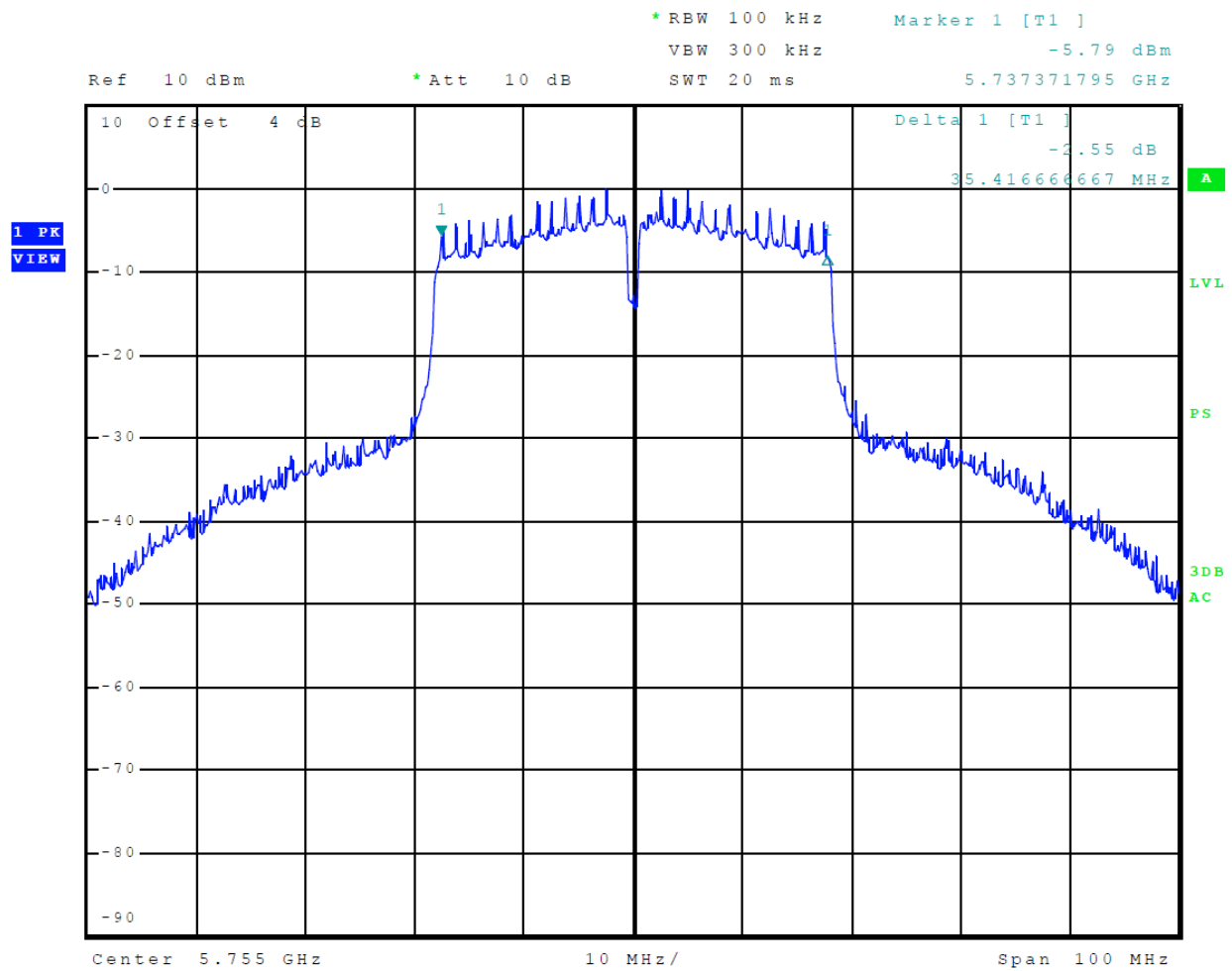
Figure 41 Plot of Transmitter 6-dB Occupied Bandwidth (5725-5850 MHz Mode 15 (802.11n40))
