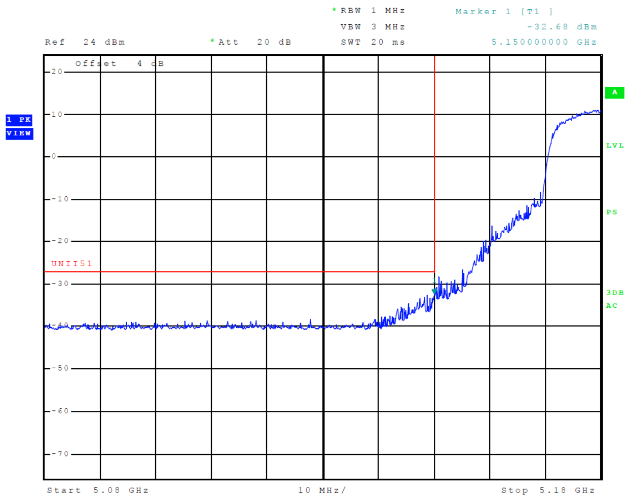
Figure 9 Plot of Lower Band Edge Across 5150-5250 MHz Band, Mode 9 (802.11a)
