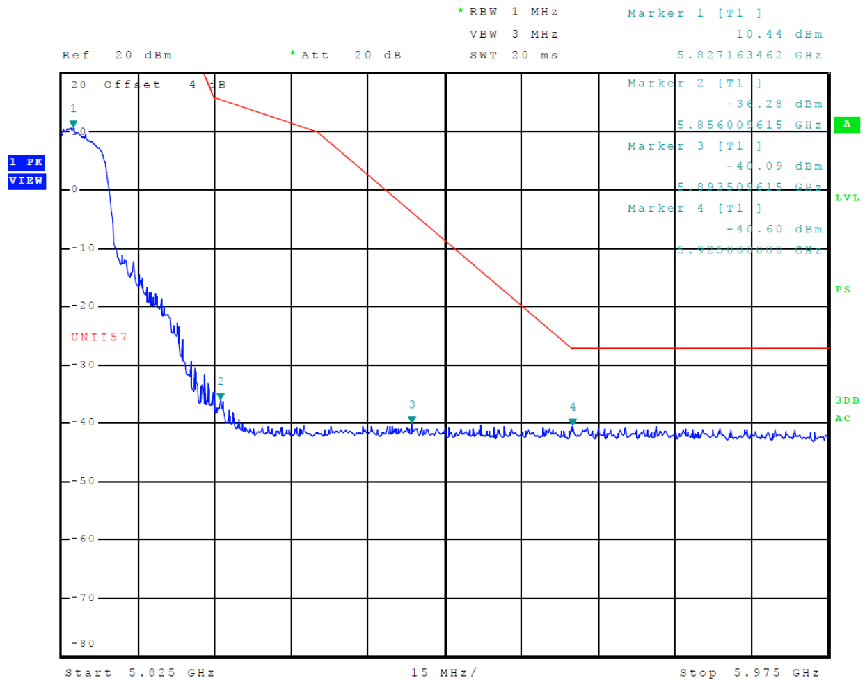
Figure 33 Plot of Upper Band Edge (Across 5725-5850 MHz Band, Mode 13 (802.11a))
