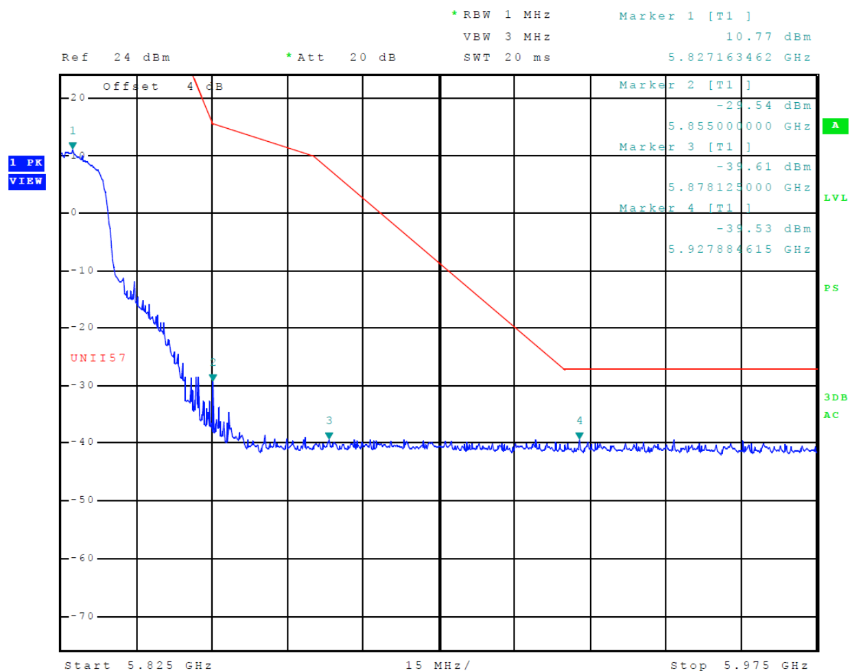
Figure 34 Plot of Upper Band Edge (Across 5725-5850 MHz Band, Mode 14 (802.11n))
