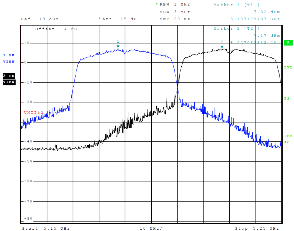
Figure 7 Plot of Transmitter Emissions Across 5150-5250 MHz Band, Mode 11 (802.11n40)
