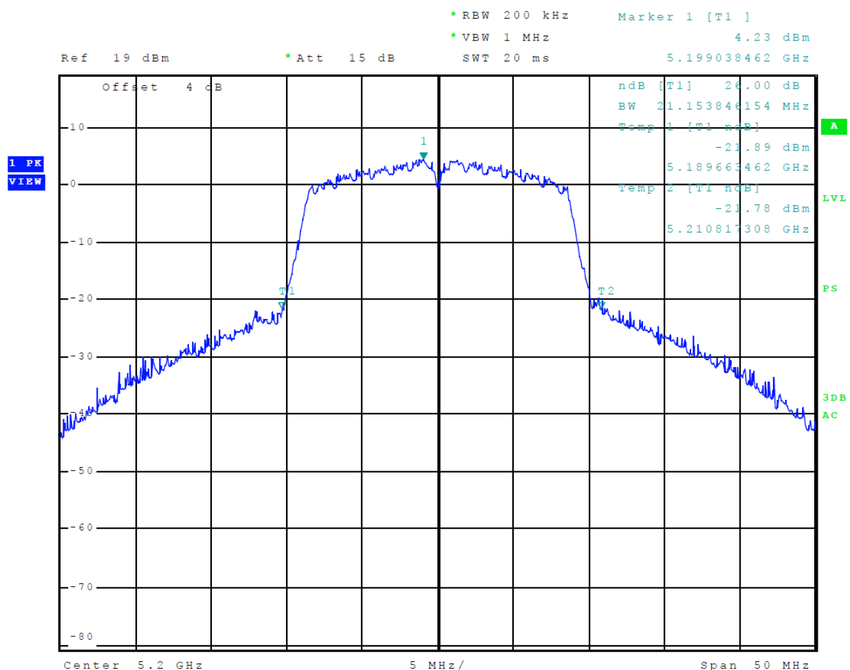
Figure 17 Plot of Transmitter 26-dB Occupied Bandwidth (5150-5250 MHz Mode 9 (802.11a))
