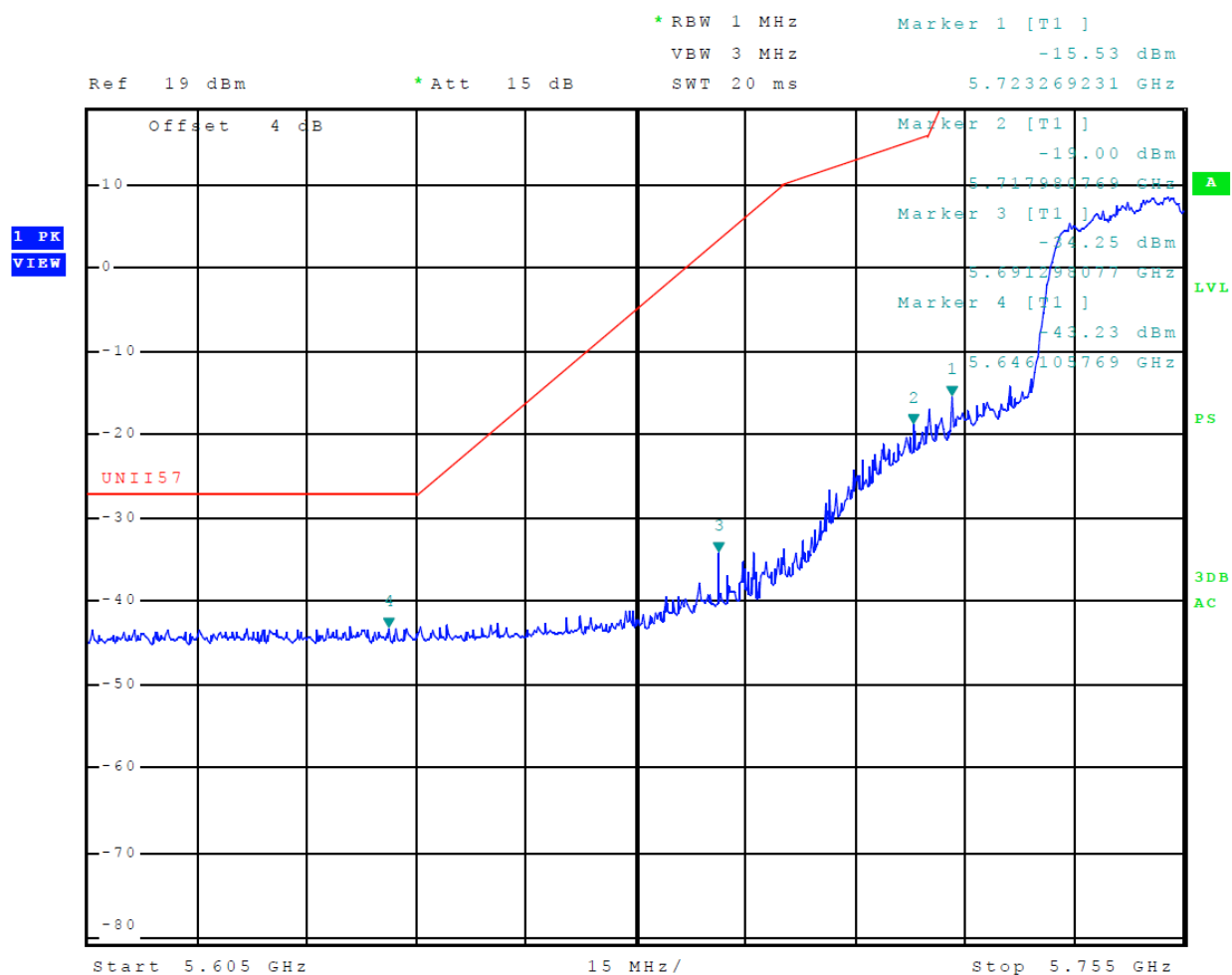
Figure 31 Plot of Lower Band Edge (Across 5725-5850 MHz Band, Mode 15 (802.11n40))
