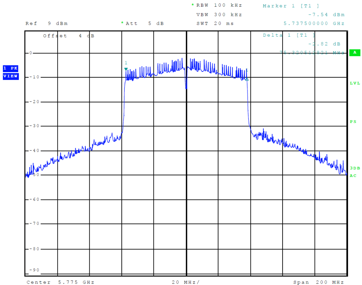
Figure 43 Plot of Transmitter 6-dB Occupied Bandwidth (5725-5850 MHz Mode 16 (802.11ac))
