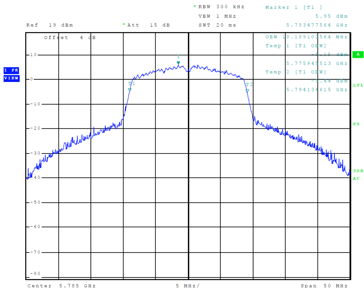
Figure 40 Plot of Transmitter 99% Occupied Bandwidth (5725-5850 MHz Mode 14 (802.11n))
