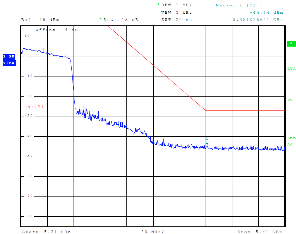
Figure 16 Plot of Upper Band Edge (Across 5150-5250 MHz Band, Mode 12 (802.11ac))
