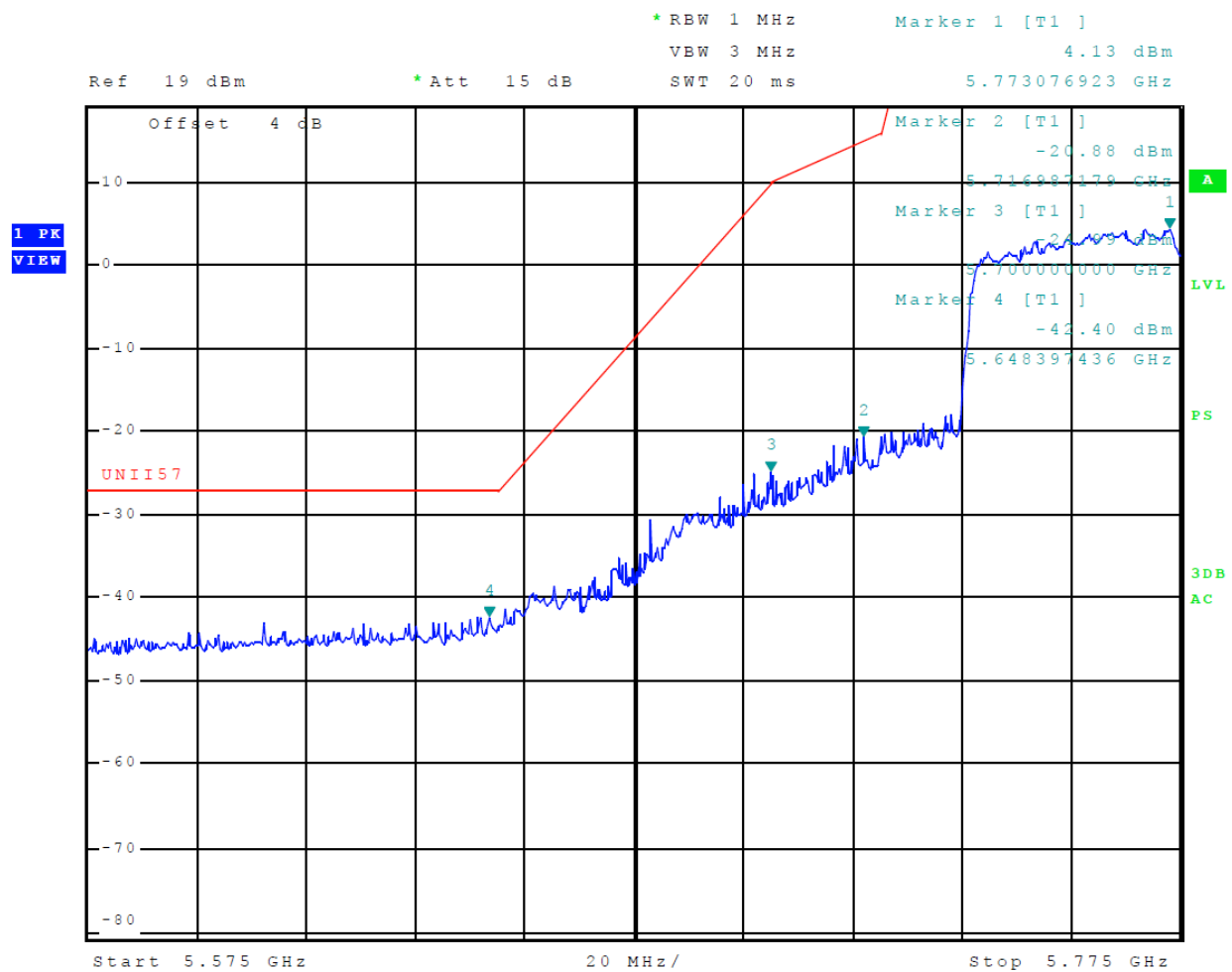
Figure 32 Plot of Lower Band Edge (Across 5725-5850 MHz Band, Mode 16 (802.11ac))
