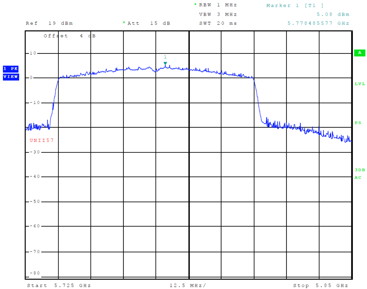
Figure 28 Plot of Transmitter Emissions (Across 5725-5850 MHz Band, Mode 16 (802.11ac))
