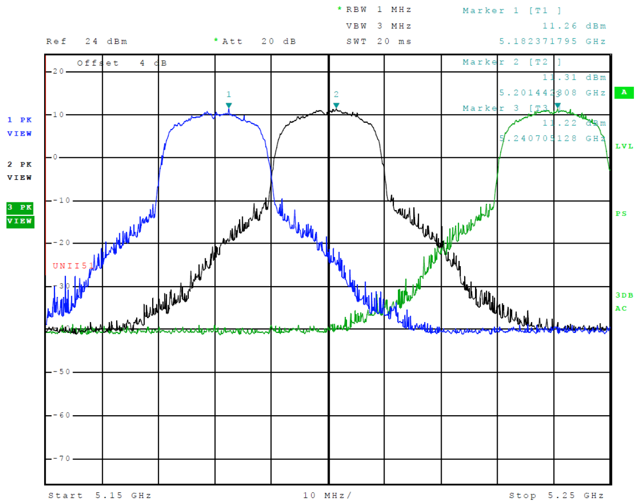
Figure 6 Plot of Transmitter Emissions Across 5150-5250 MHz Band, Mode 10 (802.11n)
