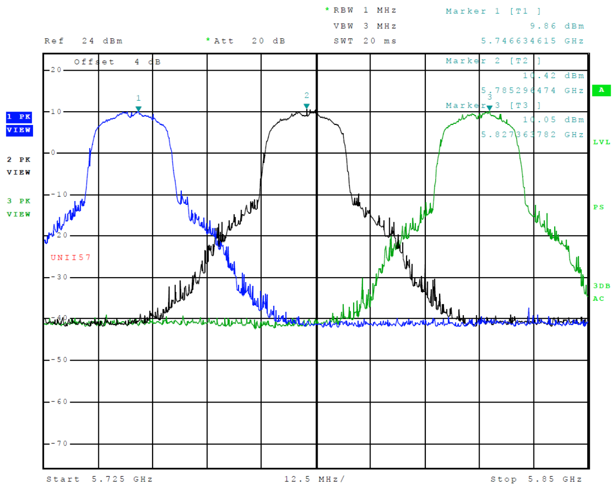
Figure 26 Plot of Transmitter Emissions (Across 5725-5850 MHz Band, Mode 14 (802.11n))
