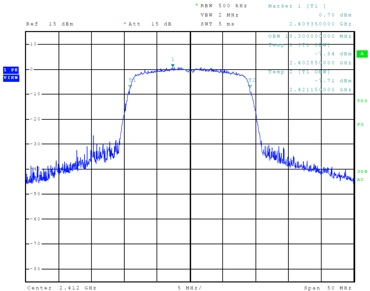
Figure 20 Plot of 99% Occupied Bandwidth Mode 3 802.11n
