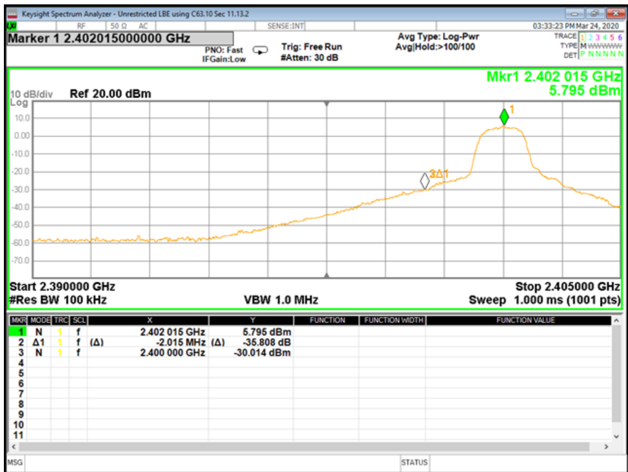
BT EDR 2MB lower band edge unrestricted
