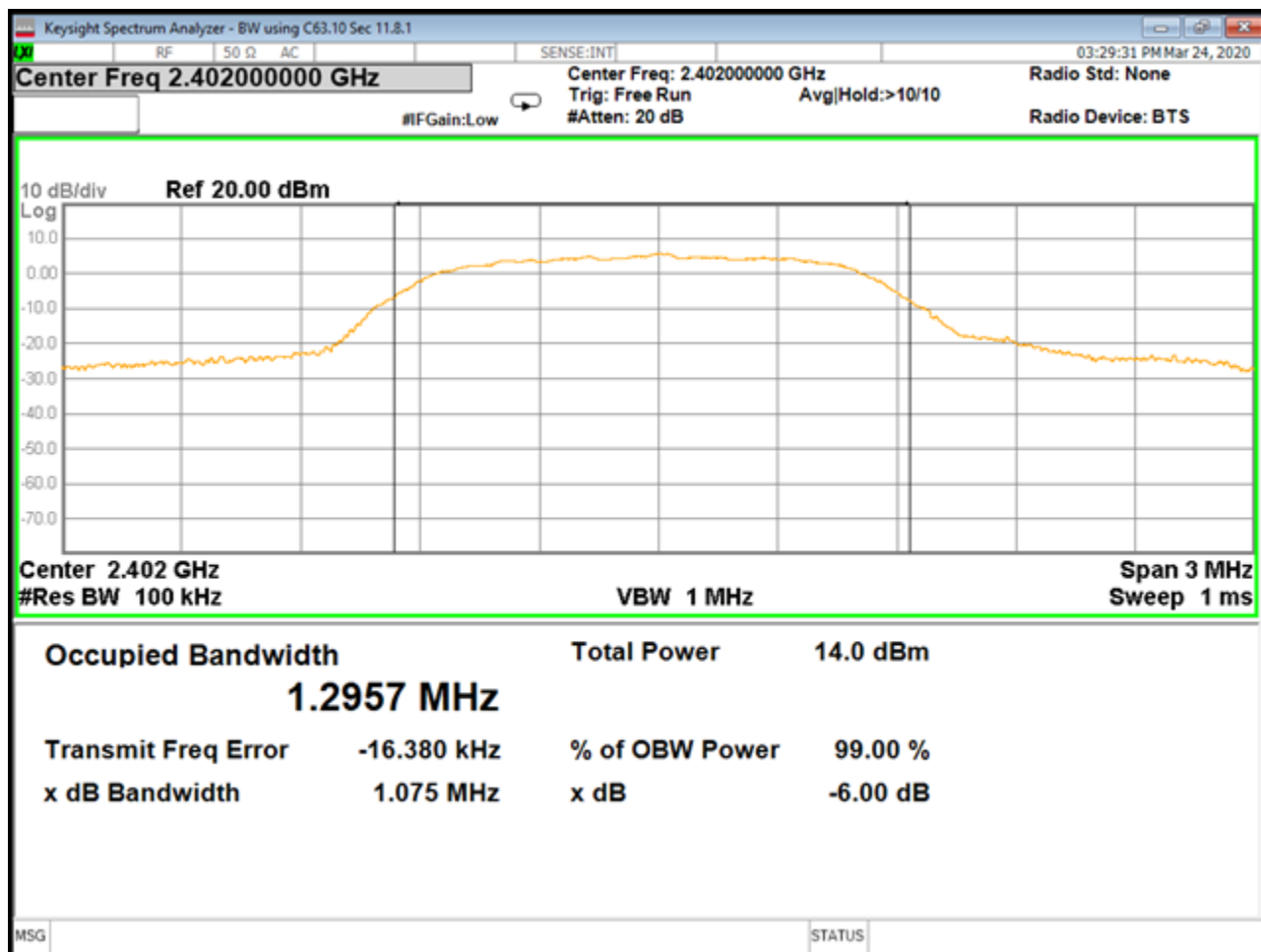
BT EDR 2MB Bandwidth low
