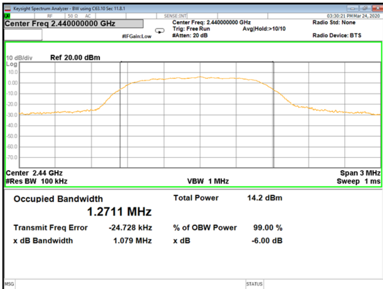
BT EDR 2MB Bandwidth mid
