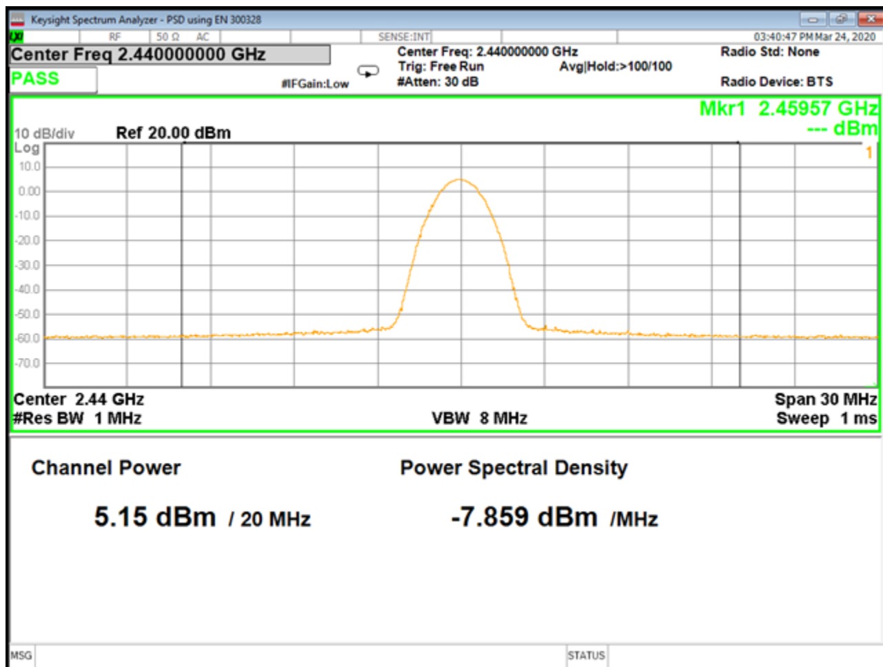
BT BR avg PSD mid
