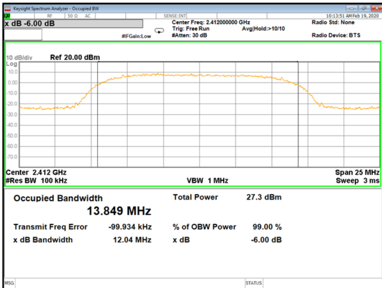
WIFI 80211 b Low channel Bandwidth
