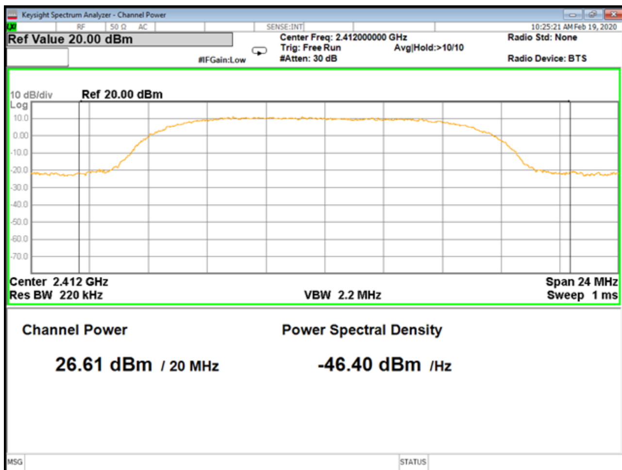
WIFI 80211 b Low channel peak power
