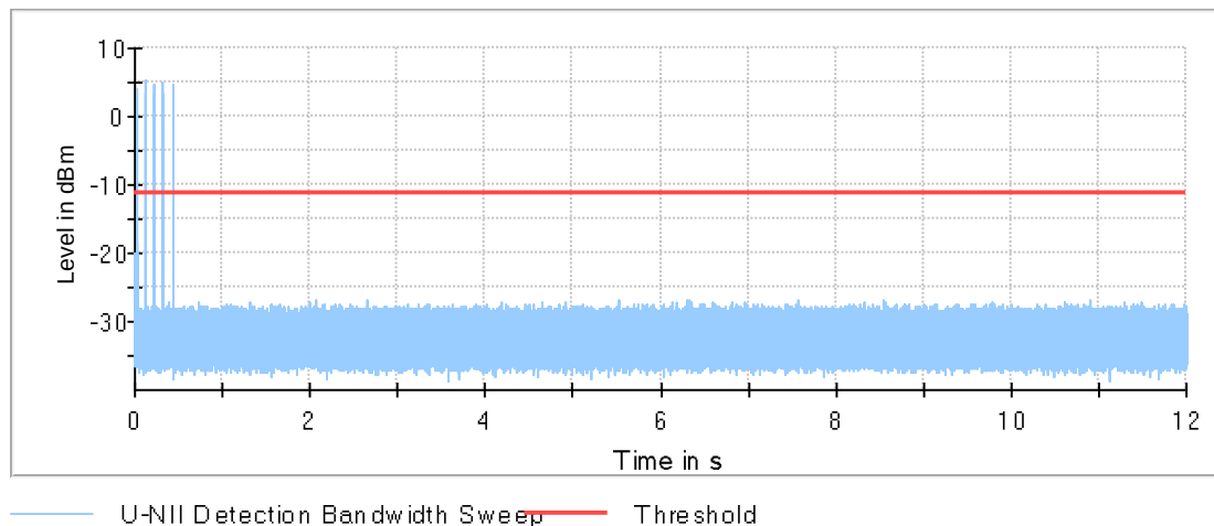
U-NII Detection Bandwidth Sweep
