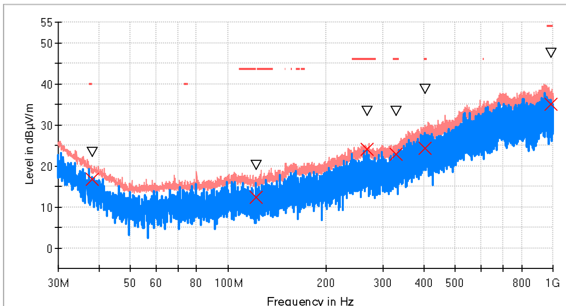
RF_FCC_15.247_E Field_30MHz_1GHz
