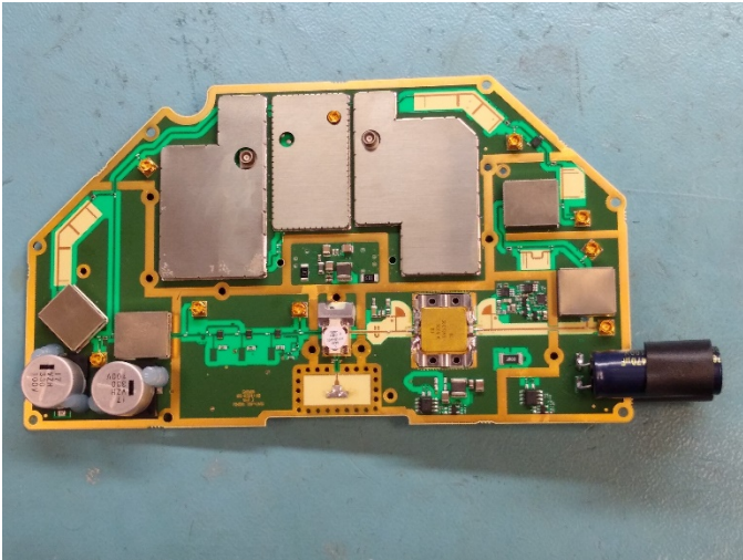
Figure 7 – Radar Module Front Shielded
