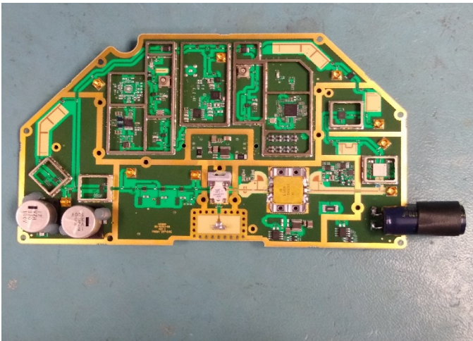
Figure 8 – Radar Module Front Unshielded
