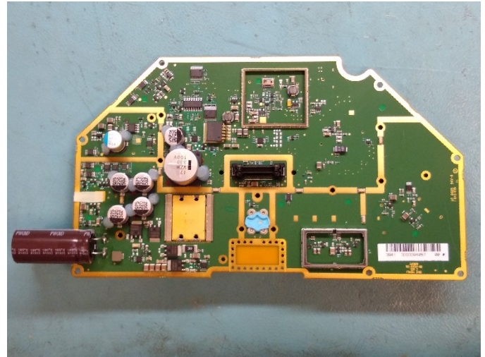
Figure 10 – Radar Module Rear Unshielded
