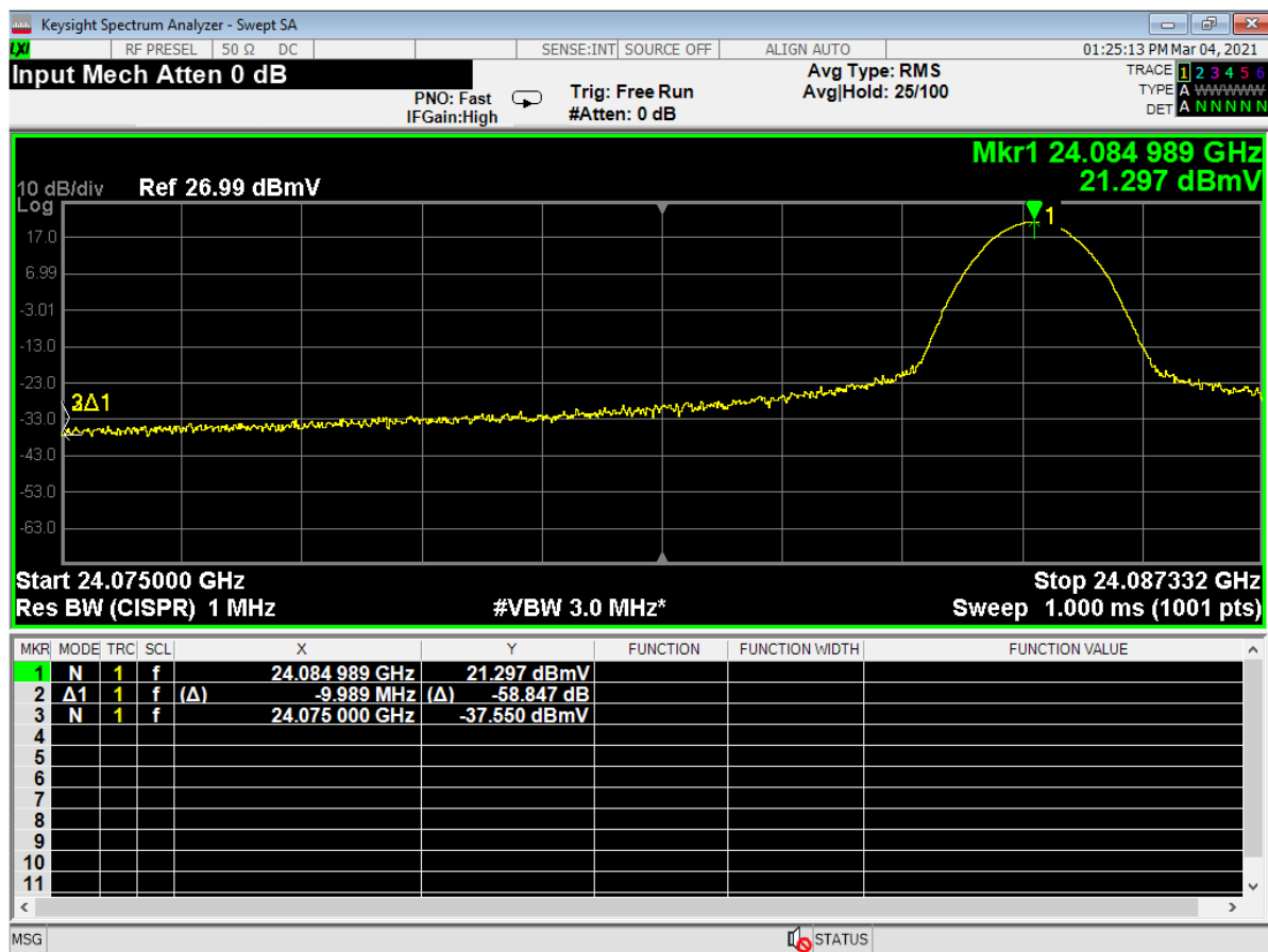
Figure 11 – Unrestricted Lower Band Edge
