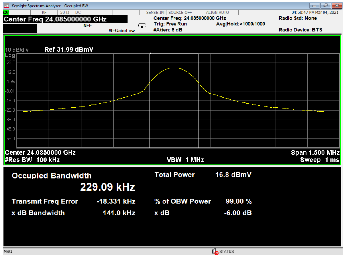
Figure 14 – Occupied Bandwidth, Low channel Uncorrected measurement as recorded on spectrum analyzer
