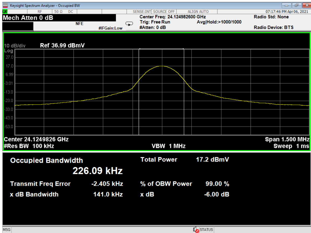
Figure 15 – Occupied Bandwidth, Mid channel Uncorrected measurement as recorded on spectrum analyzer
