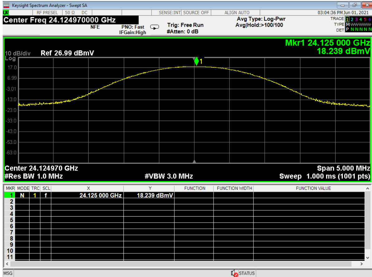
Figure 4 - Analyzer Measurement – Fundamental, Mid Channel
