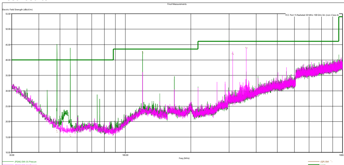
Figure 18 - Radiated Emissions Plot, Low Channel
