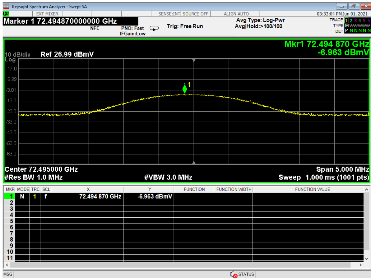
Figure 9 - Analyzer Measurement – 3 rd Harmonic, High Channel, Peak
