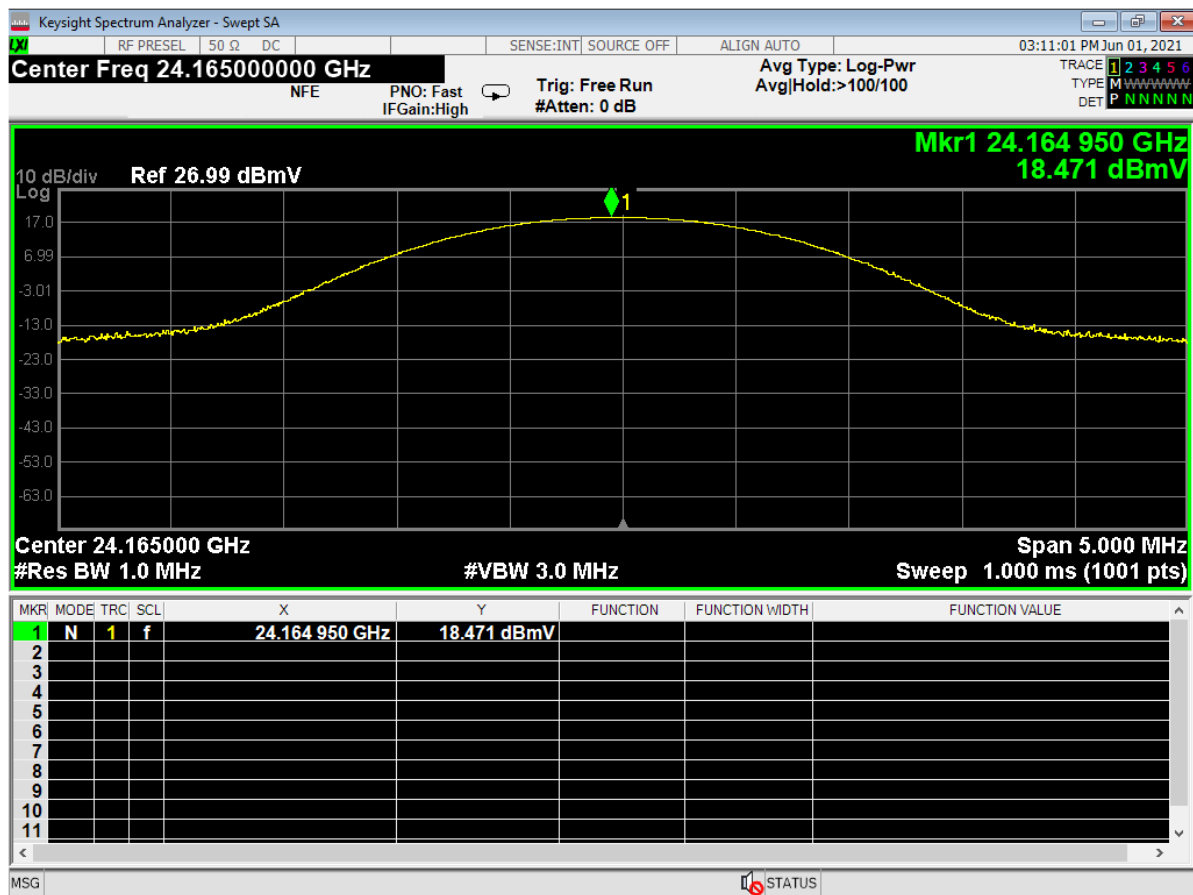
Figure 7 - Analyzer Measurement – Fundamental, High Channel
