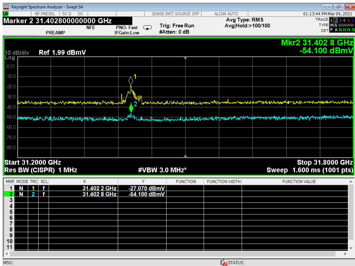
Figure 12 – Restricted Higher Band Edge
