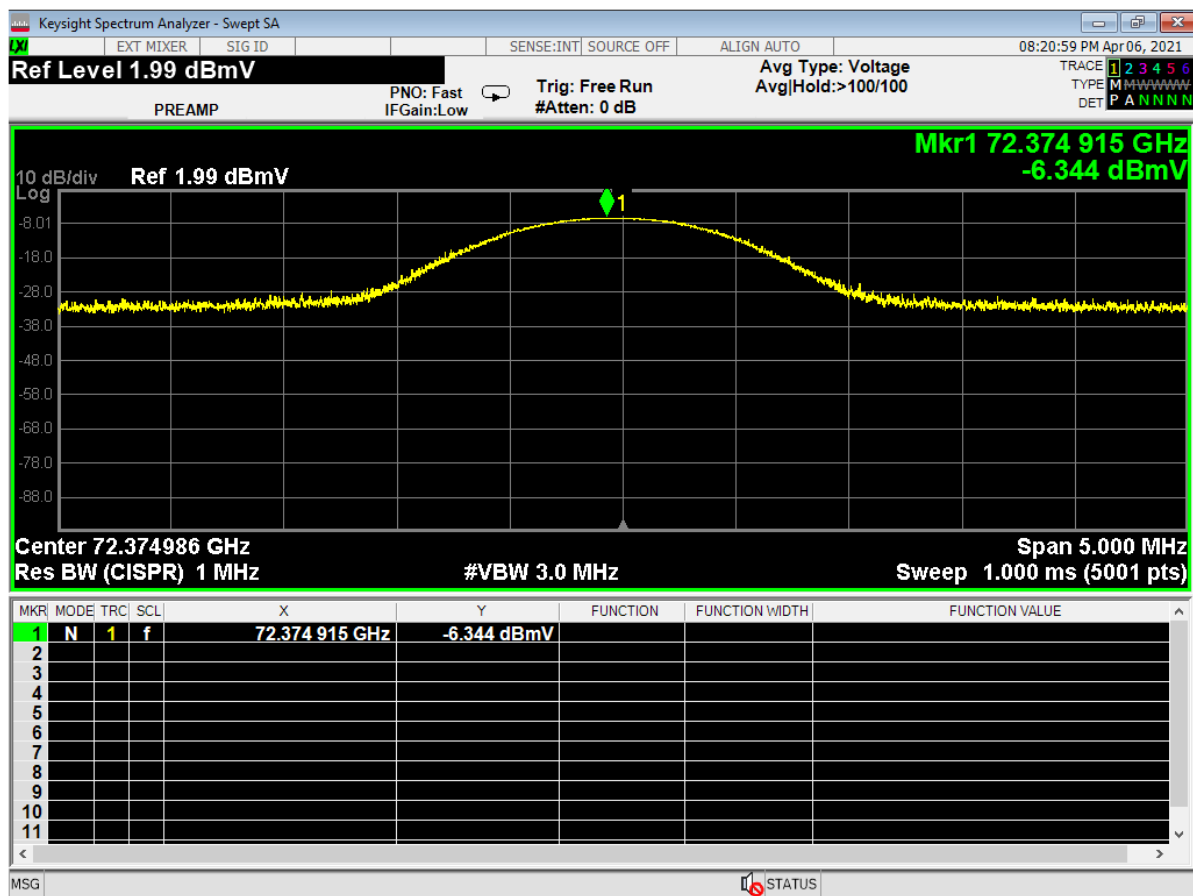
Figure 6 - Analyzer Measurement – 3 rd Harmonic, Mid Channel, Peak
