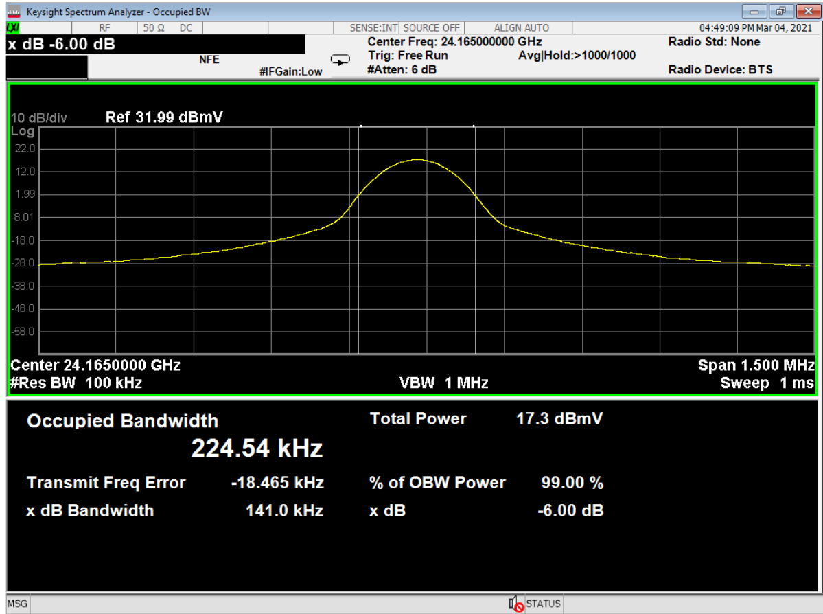
Figure 16 – Occupied Bandwidth, High channel Uncorrected measurement as recorded on spectrum analyzer
