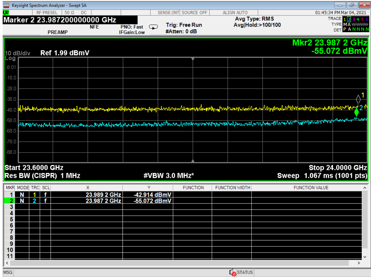
Figure 10 – Restricted Lower Band Edge
