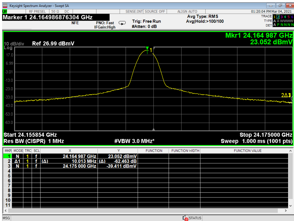
Figure 13 – Unrestricted Higher Band Edge
