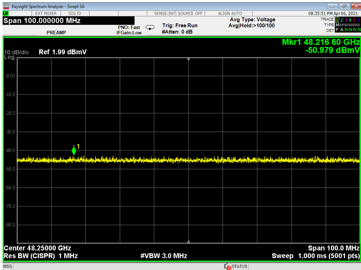
Figure 5 - Analyzer Measurement – 2 nd Harmonic, Mid Channel, Peak
