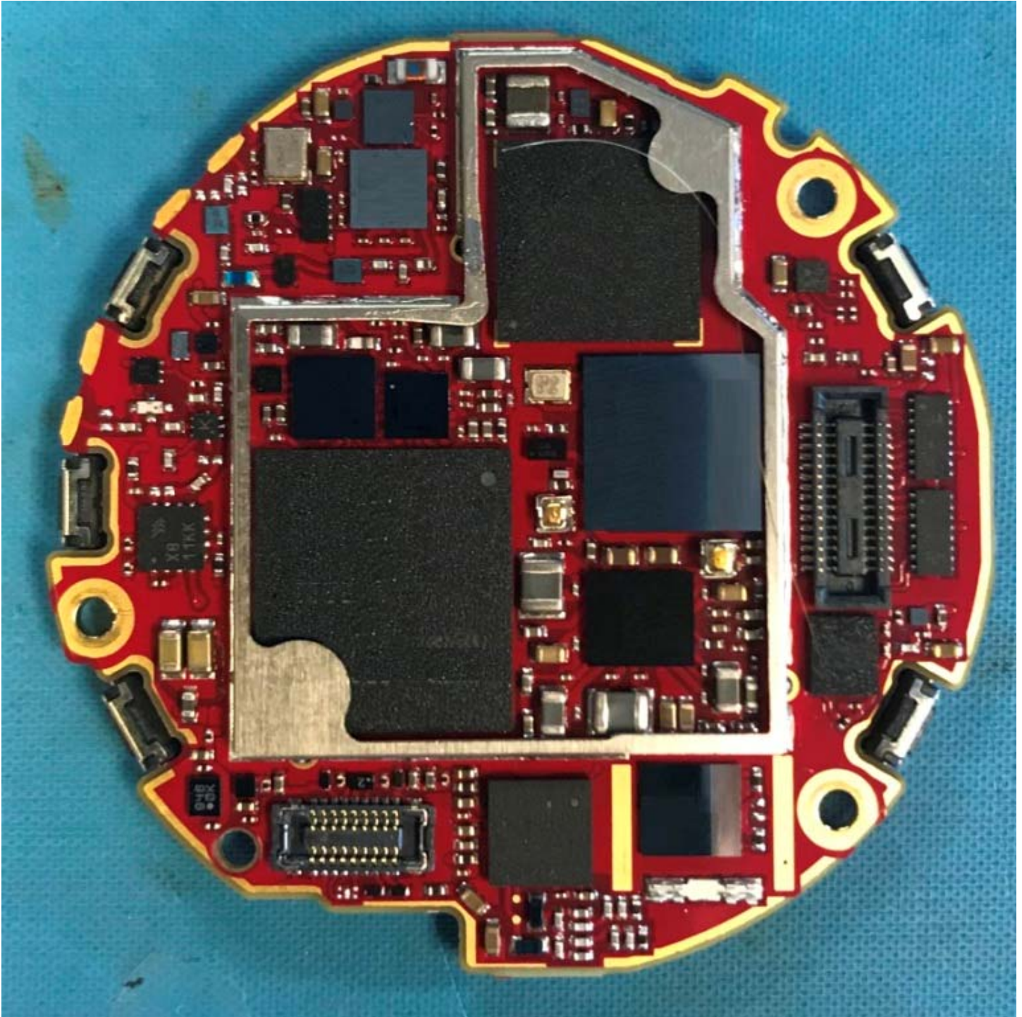
Figure E19.1 – Internal Photo – PCB Top
