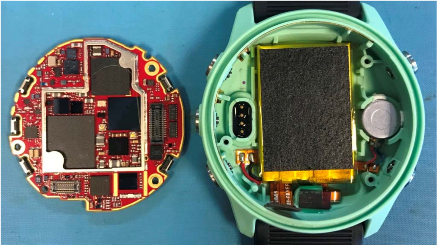
Figure E19.4 – Internal Photo – Cover and PCB Removed
