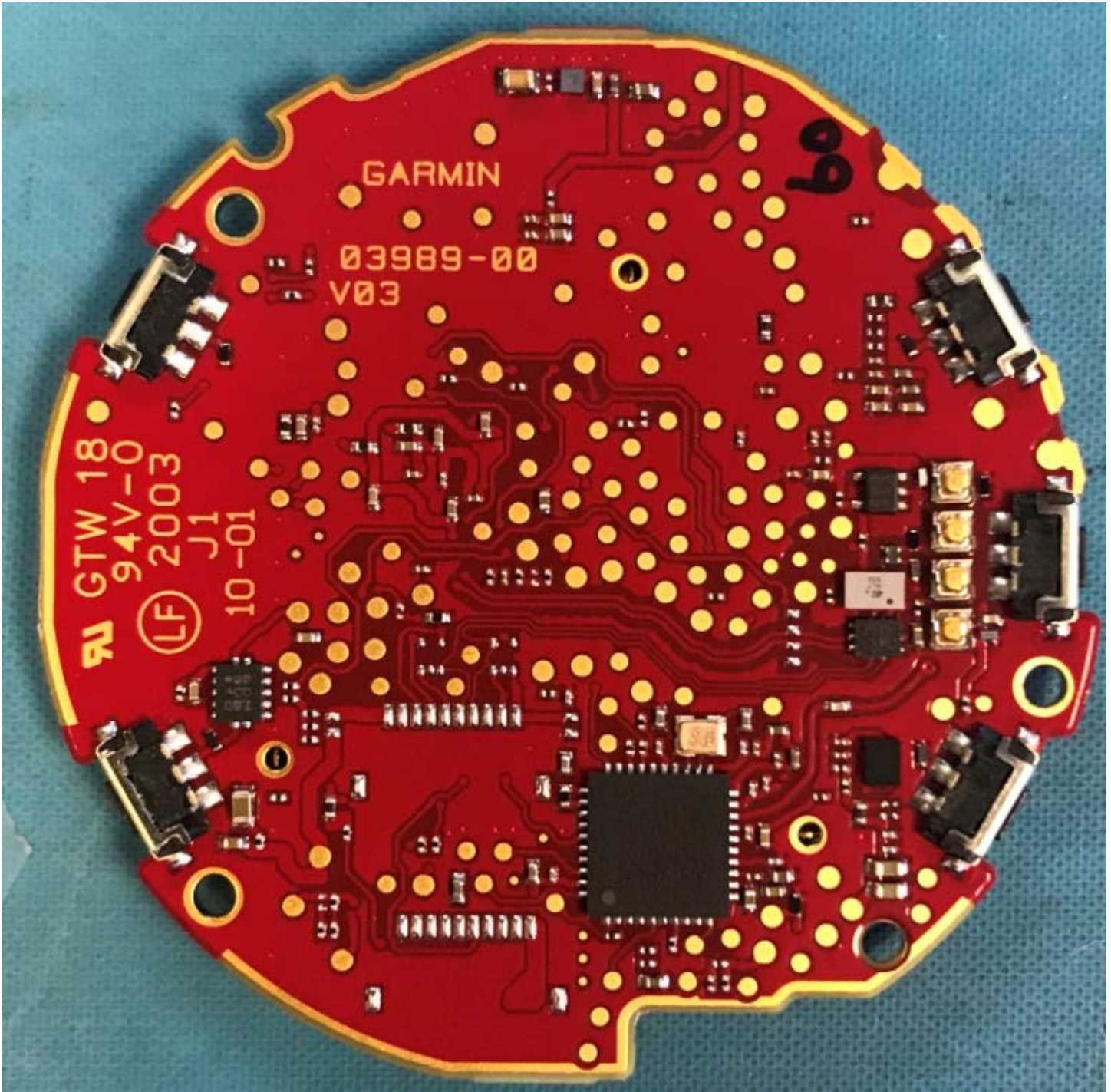
Figure E19.2 – Internal Photo – PCB Bottom
