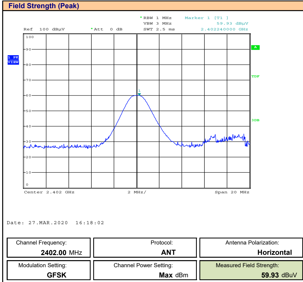
Plot D.1 – Field Strength, ANT, Peak, Horizontal, 2402MHz
