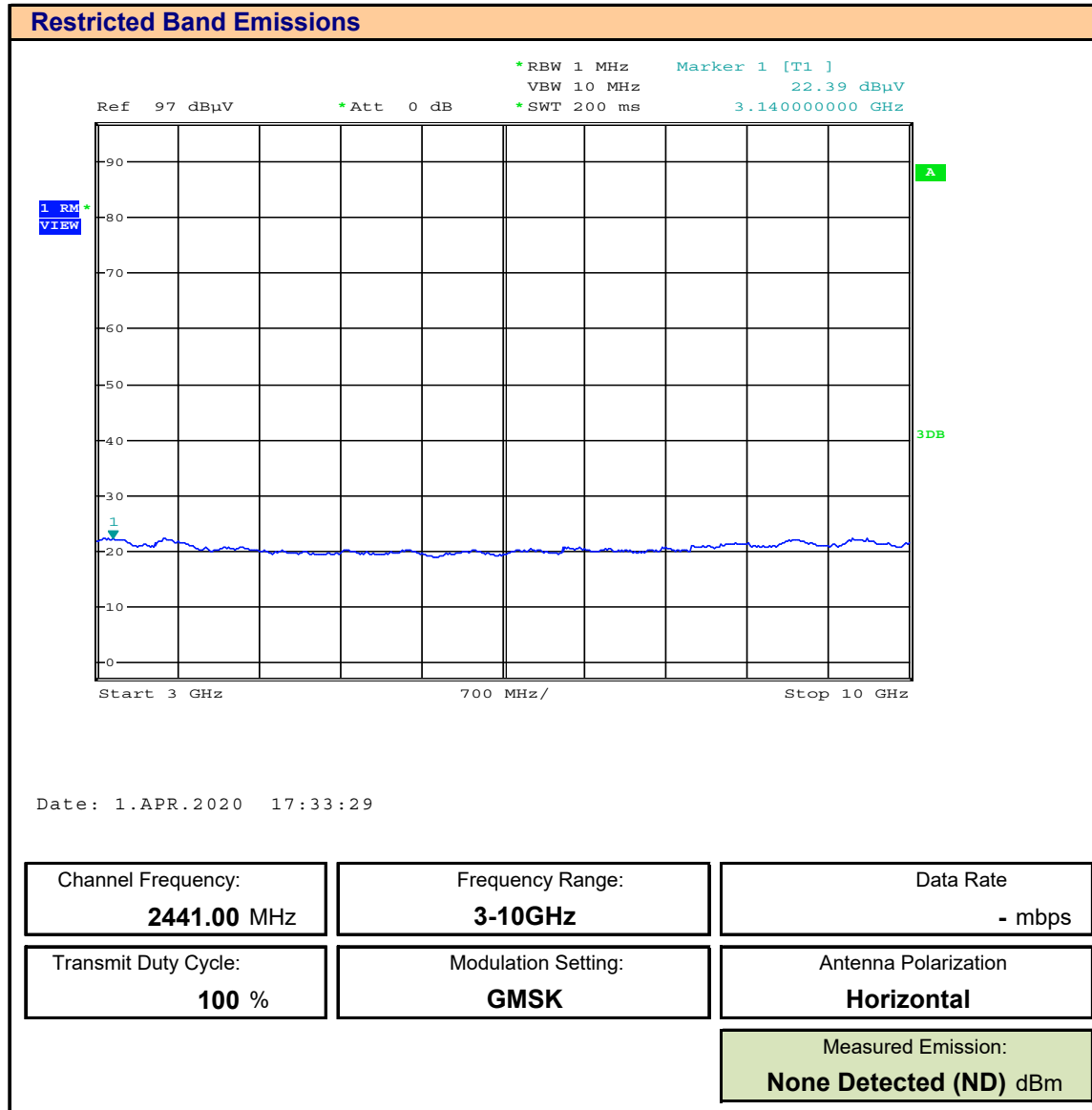
Plot E.18 – Radiated Tx Measurement, BLE, Horizontal, 3-10GHz
