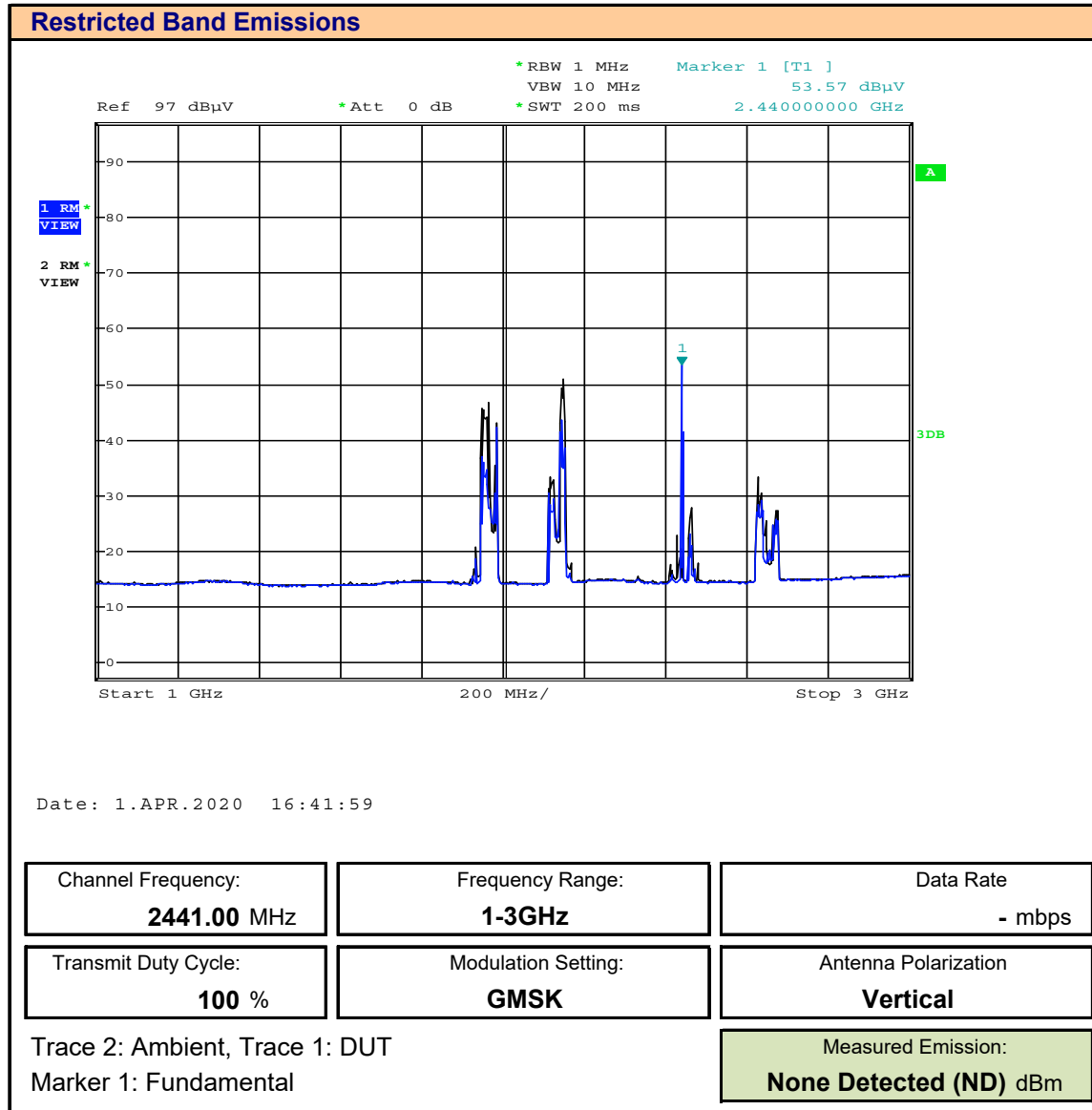
Plot E.24 – Radiated Tx Measurement, BLE, Vertical, 1-3GHz
