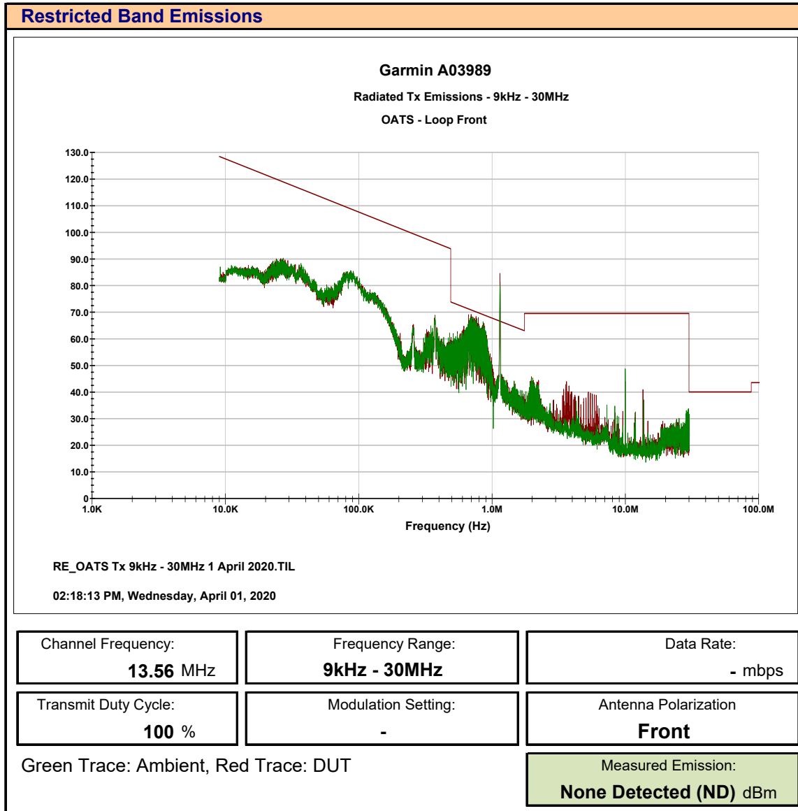
Plot E.29 – Radiated Tx Measurement, NFC, Front, 9kHz-30MHz
