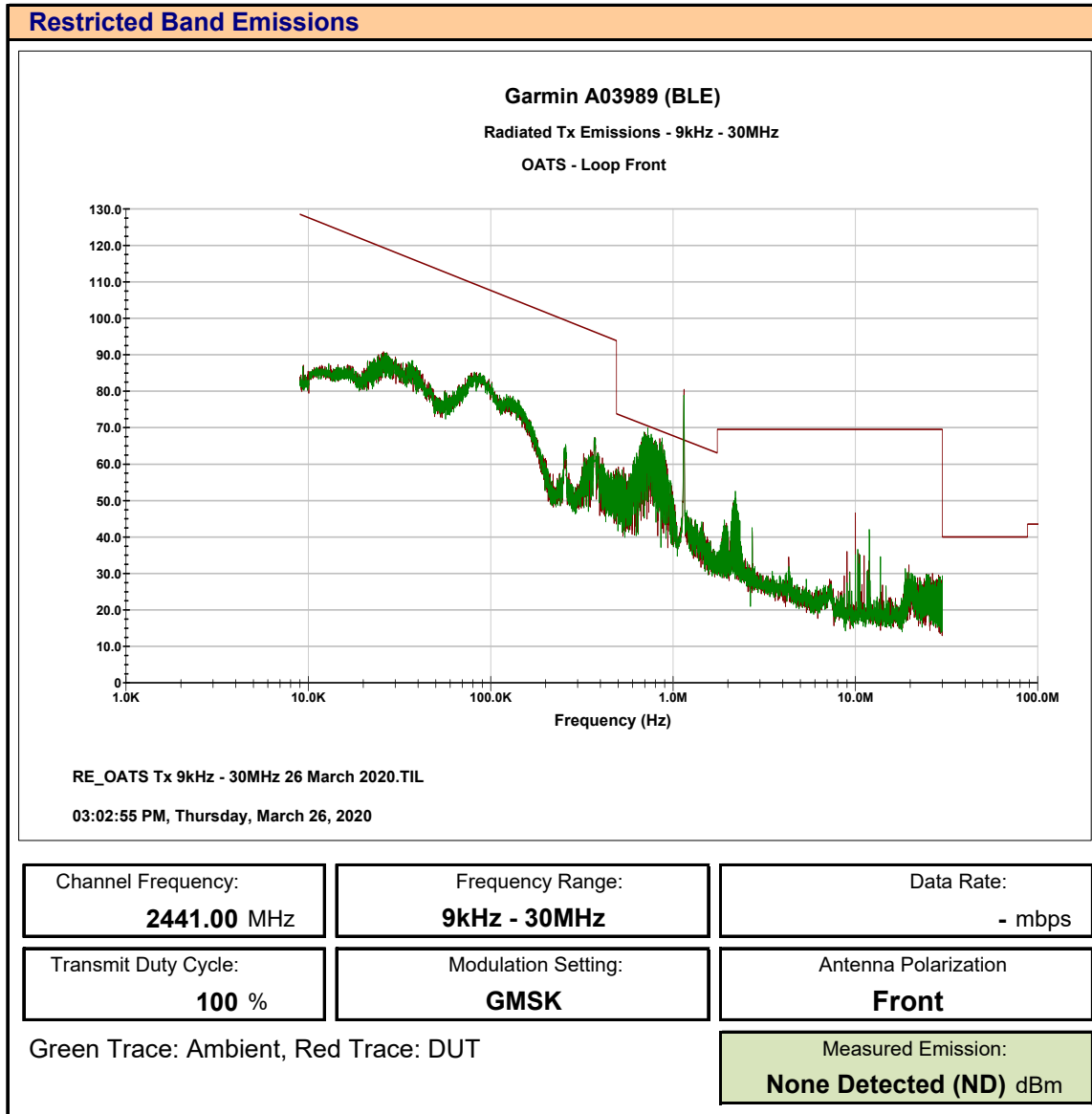
Plot E.15 – Radiated Tx Measurement, BLE, Front, 9kHz-30MHz
