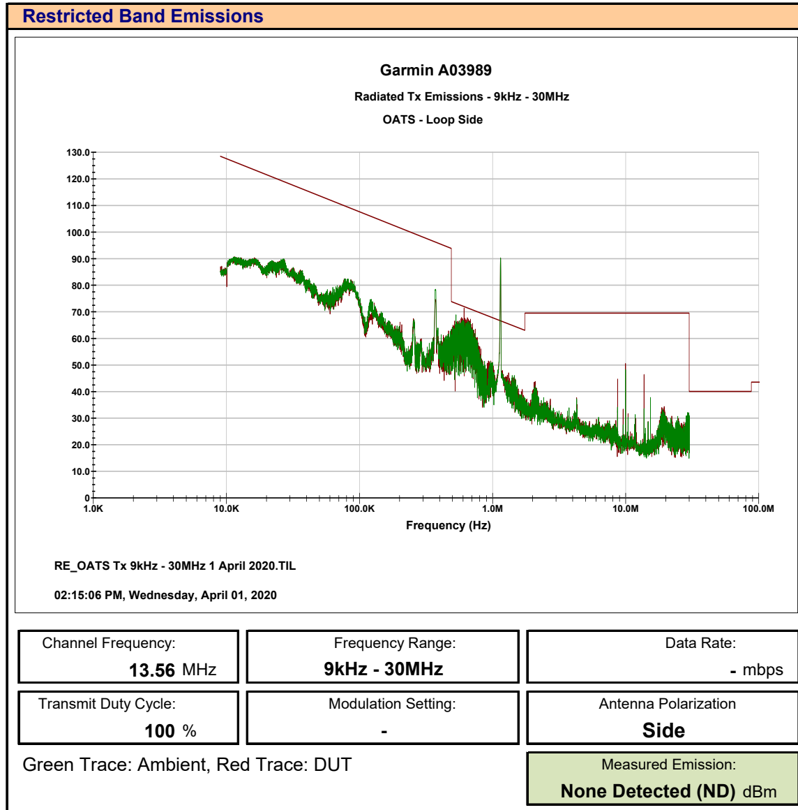
Plot E.31 – Radiated Tx Measurement, NFC, Side, 9kHz-30MHz
