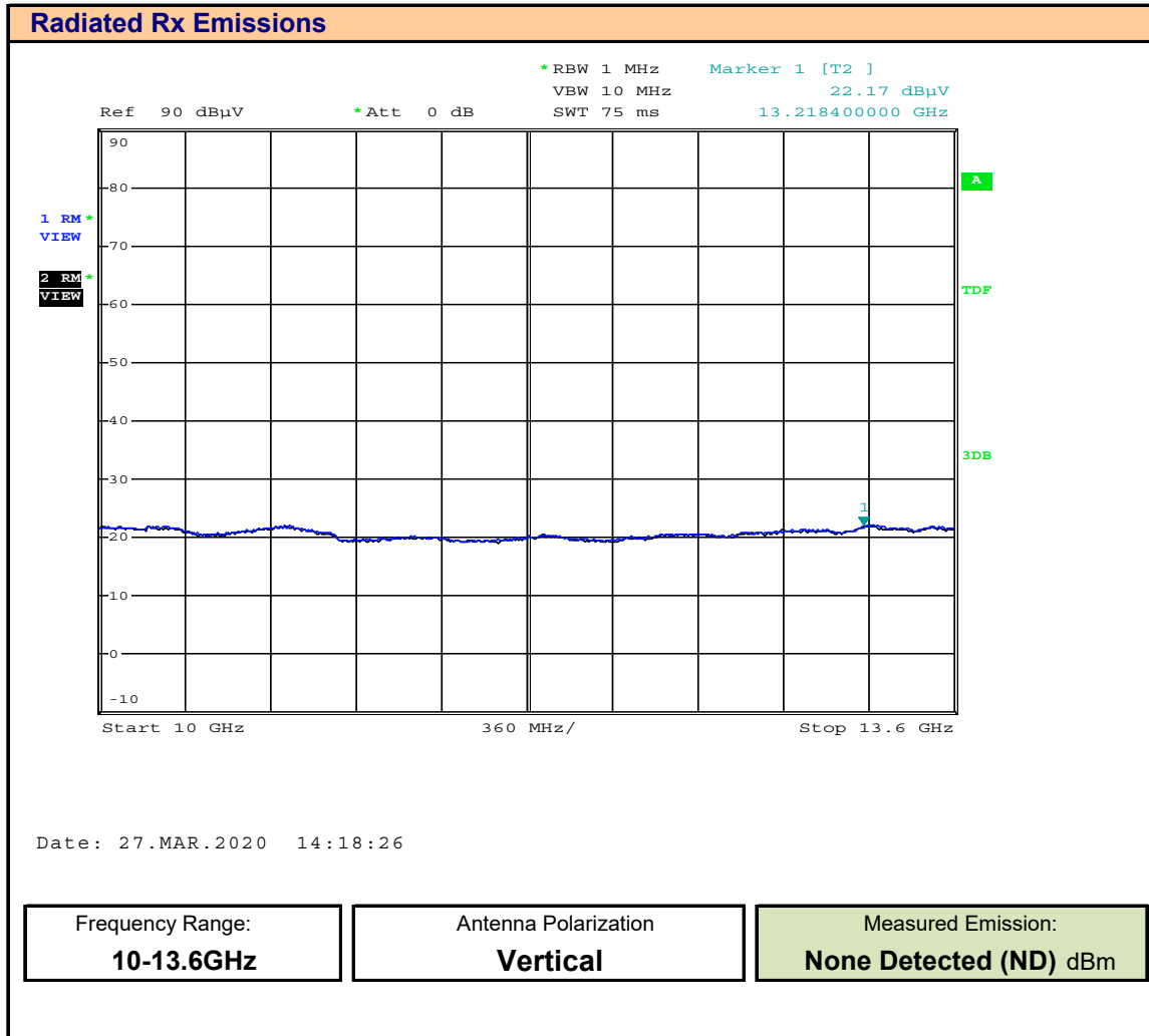
Plot F.10 – Radiated Rx Emissions, 10-13.6GHz, Vertical
