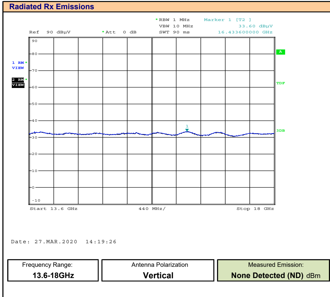
Plot F.12 – Radiated Rx Emissions, 13.6-18GHz, Vertical
