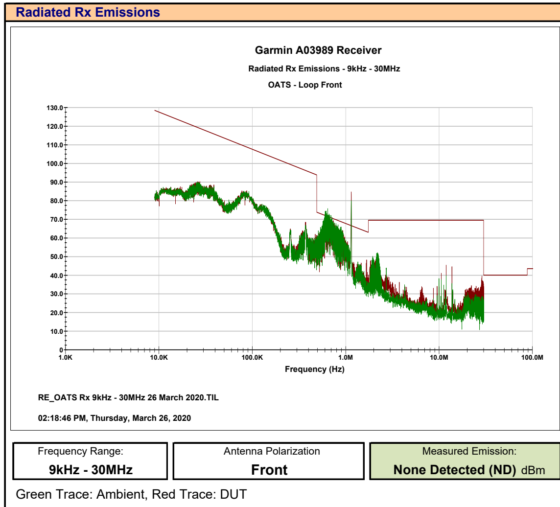
Plot F.1 – Radiated Rx Emissions, 9kHz – 30MHz, Front
