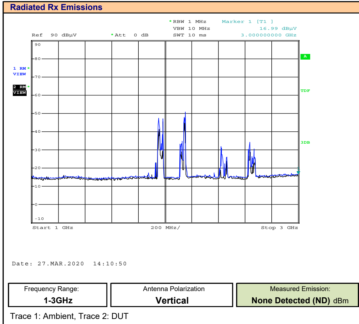
Plot F.6 – Radiated Rx Emissions, 1-3GHz, Vertical
