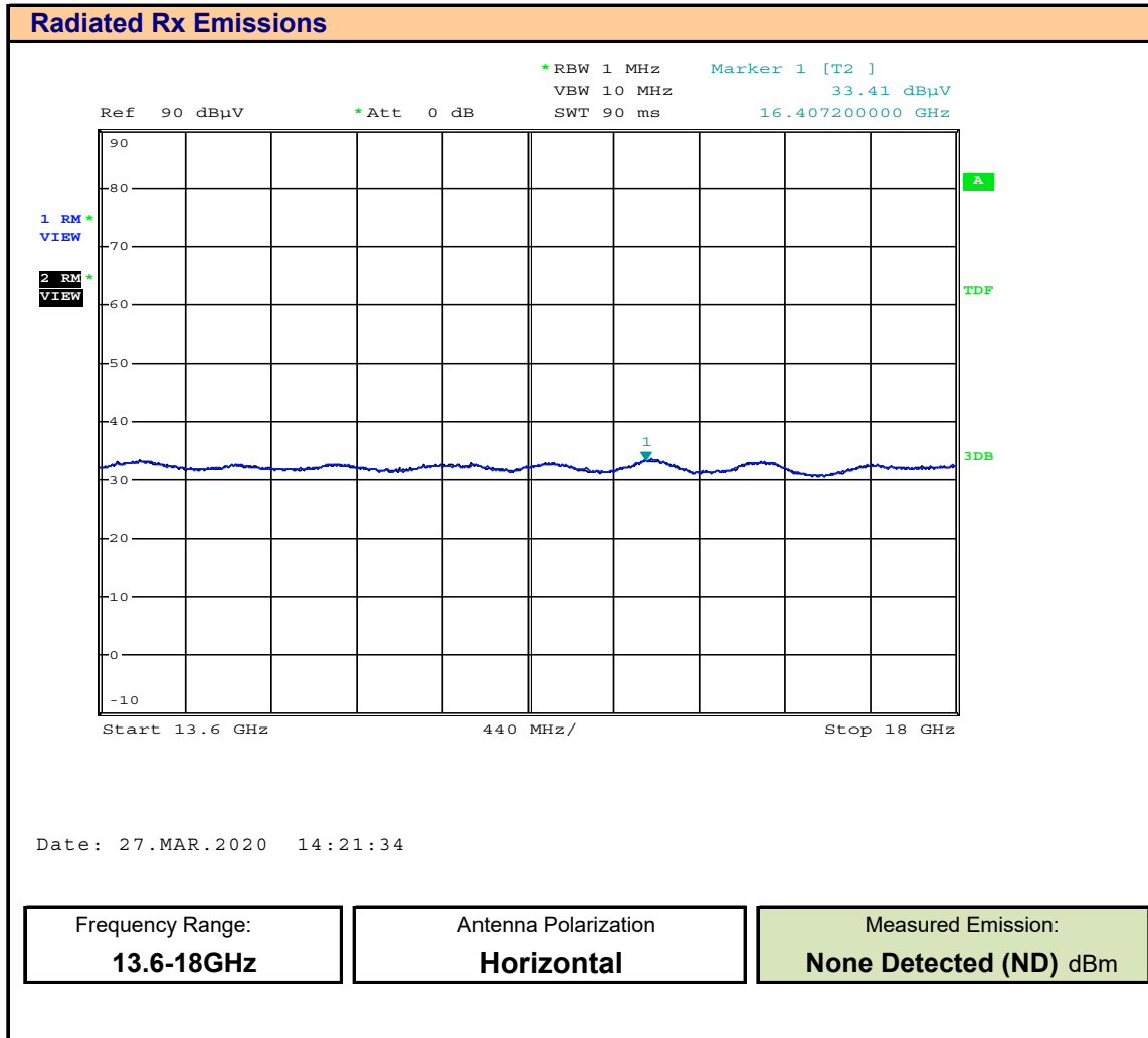
Plot F.11 – Radiated Rx Emissions, 13.6-18GHz, Horizontal
