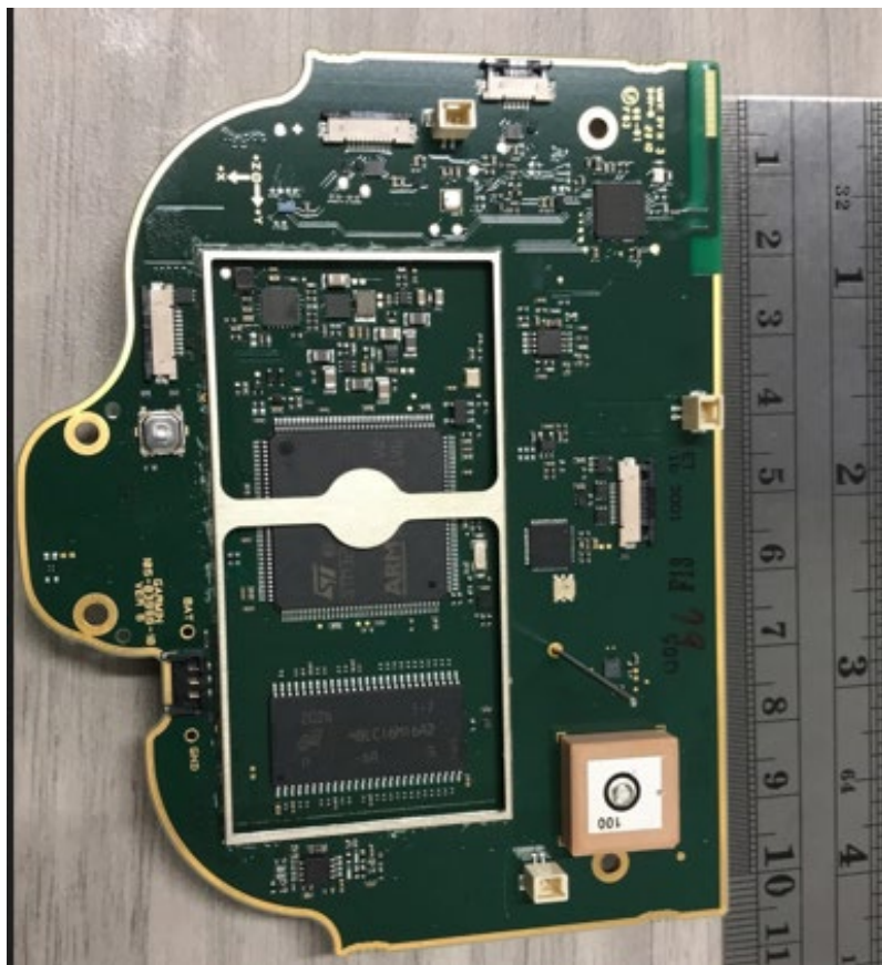
Main PCB Top:
