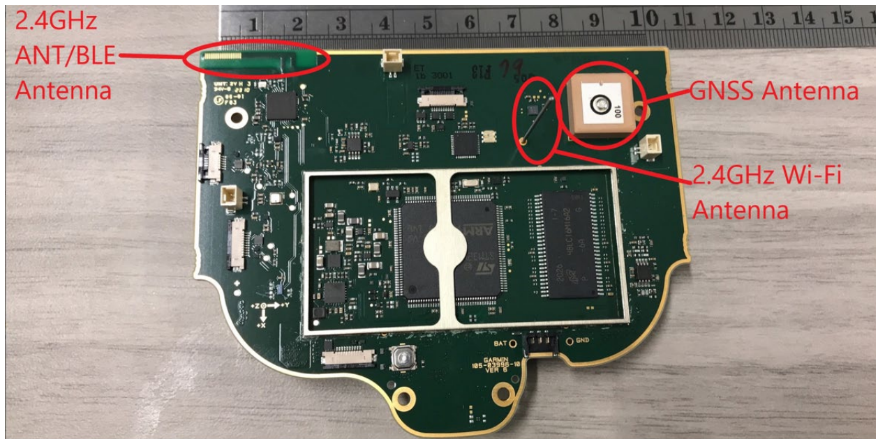
Main PCB Top with antenna labeled:
