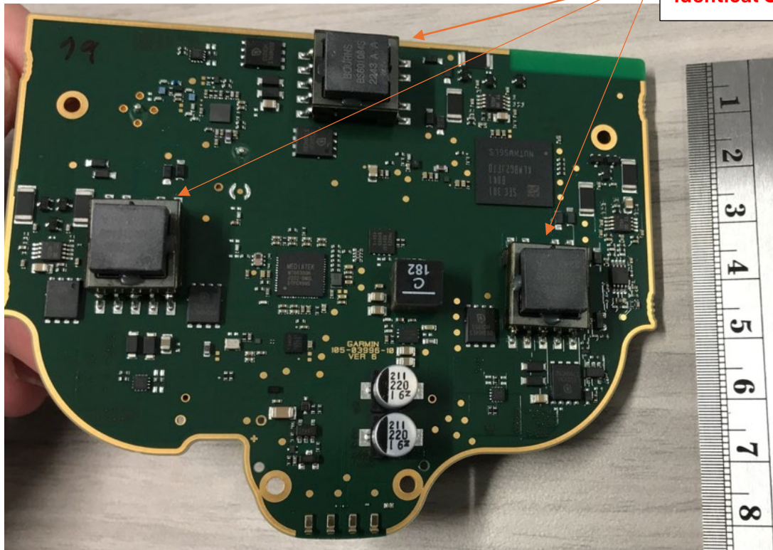
Main PCB Bottom:
