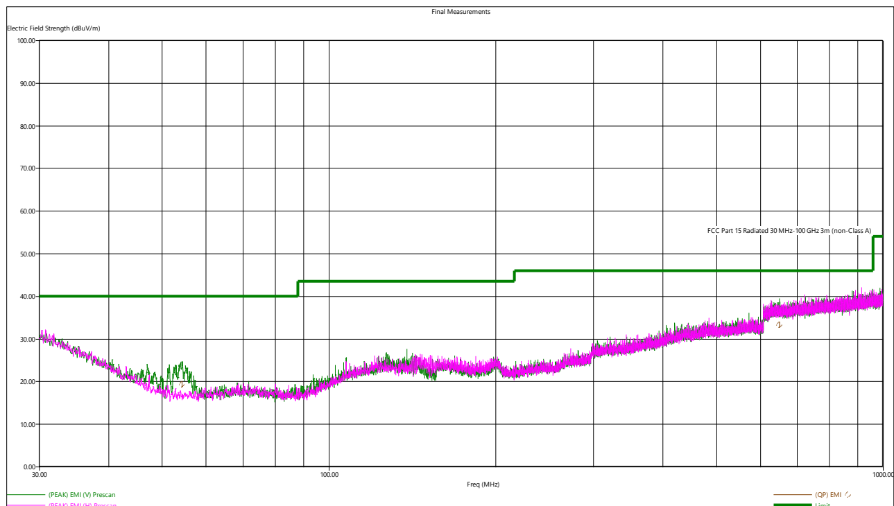
Figure 22 – Radiated Emission Plot, High Channel GFSK
