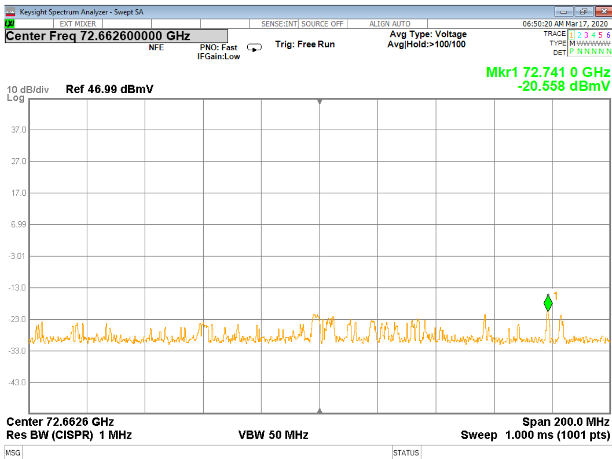
Figure 29 - Analyzer Measurement – 3 rd Harmonic, High Channel (Single Frequency)
