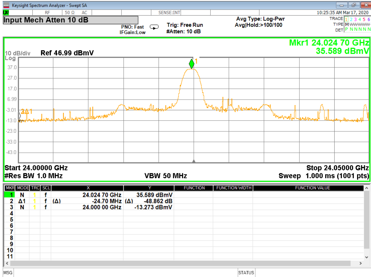
Figure 34 – Lower Band Edge (Single Frequency), 24.00 GHz Uncorrected measurement as recorded on spectrum analyzer, 5 cm test distance
