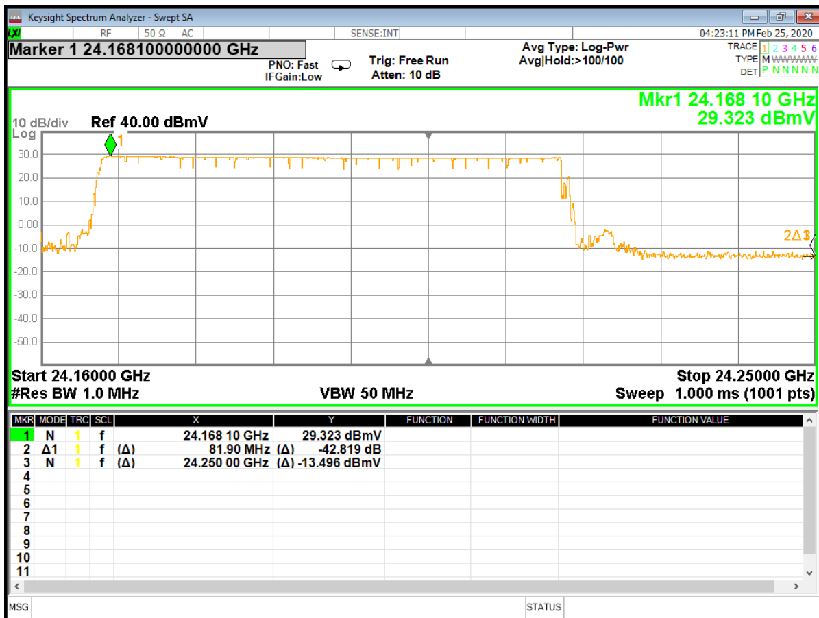
Figure 33 - Higher Band Edge (48 MHz) (swept frequency), 24.25 GHz Uncorrected measurement as recorded on spectrum analyzer, 5 cm test distance
