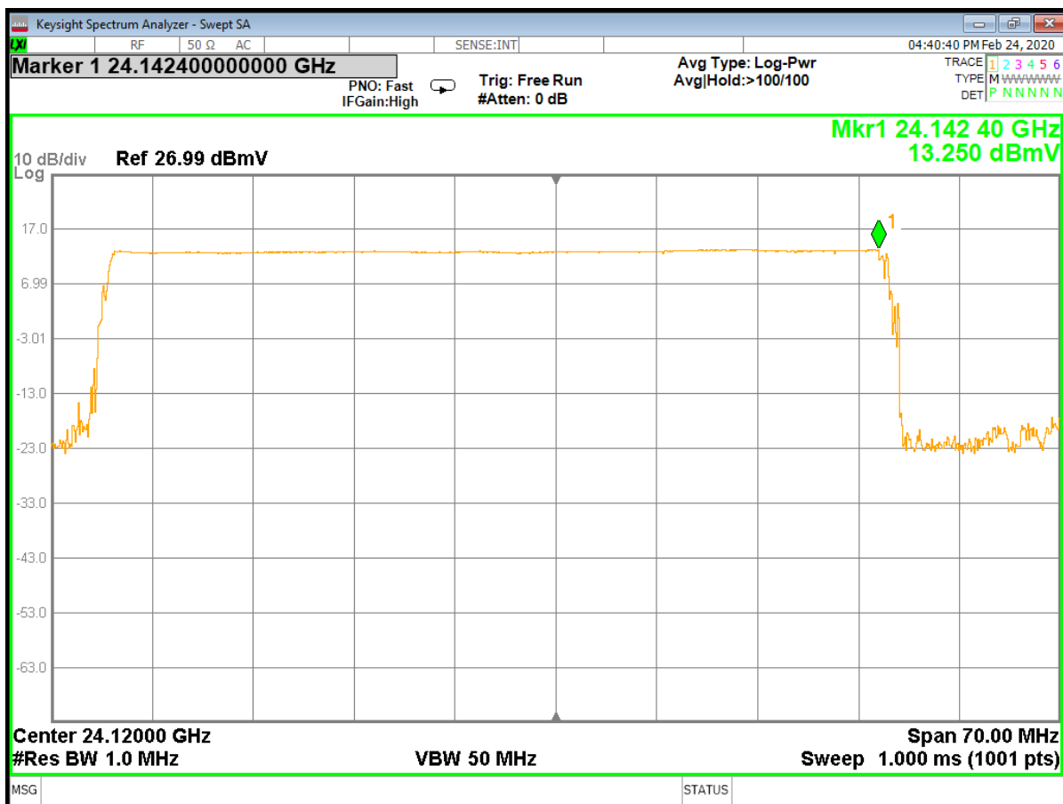
Figure 15 - Analyzer Measurement – Fundamental, Mid Channel (48 MHz) (swept frequency)
