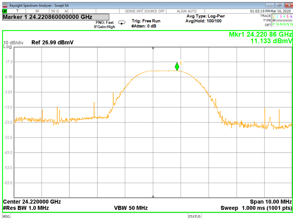
Figure 27 - Analyzer Measurement – Fundamental, High Channel (Single Frequency)
