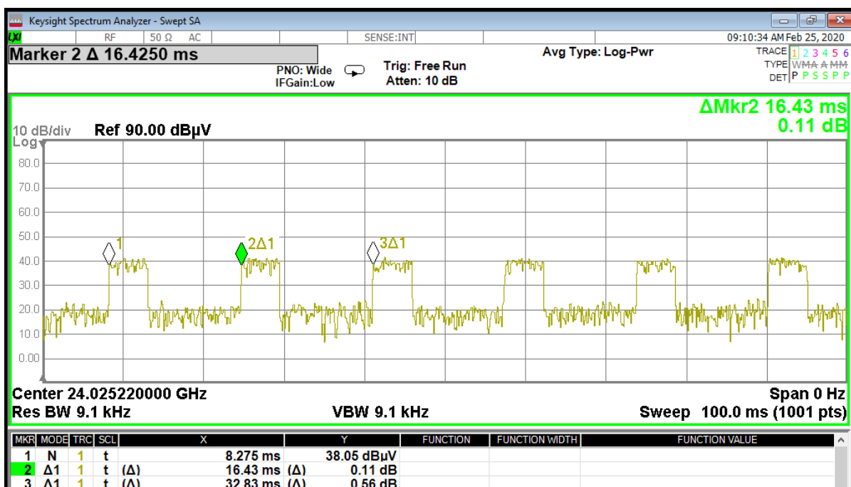
Figure 2 - Period = 16.43 ms
