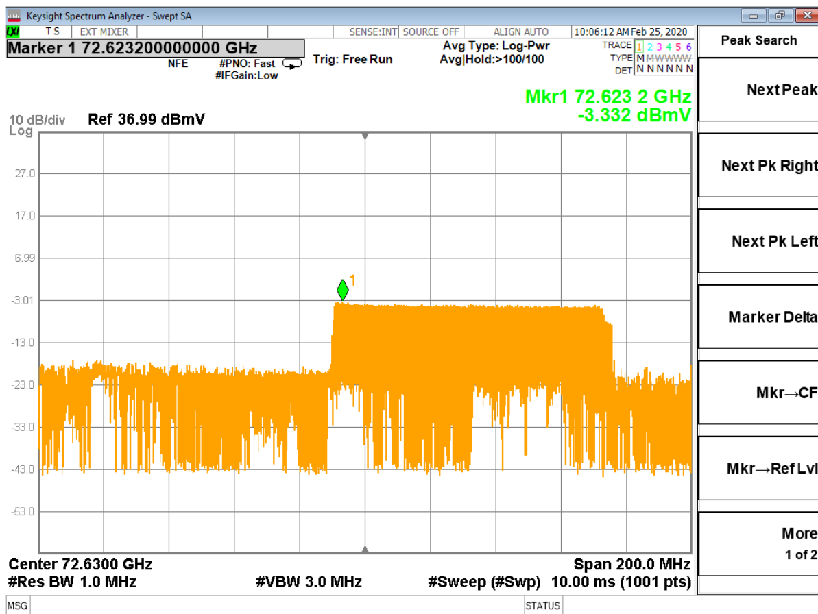
Figure 11 - Analyzer Measurement – 3 rd Harmonic, High Channel (24 MHz) (swept frequency)
