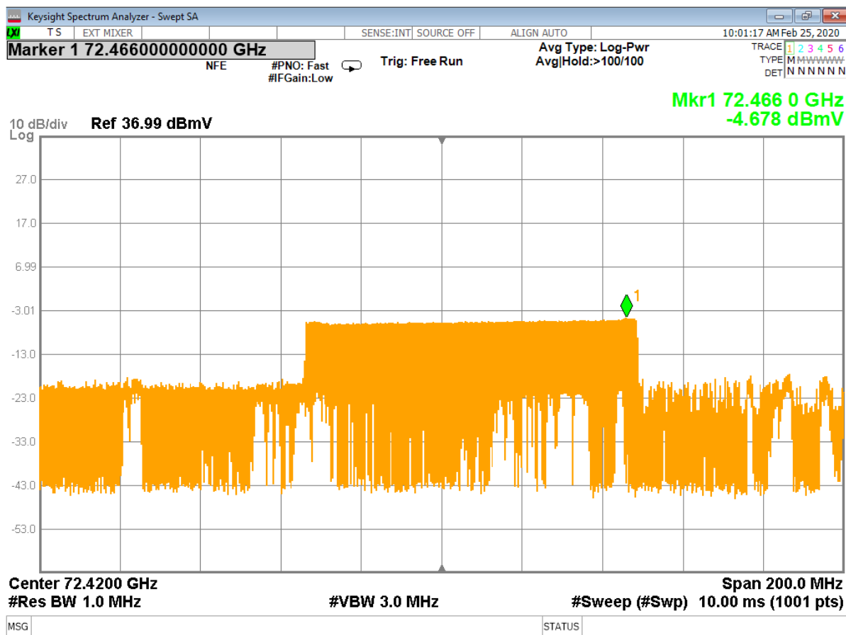
Figure 8 - Analyzer Measurement – 3 rd Harmonic, Mid Channel (24 MHz) (swept frequency)
