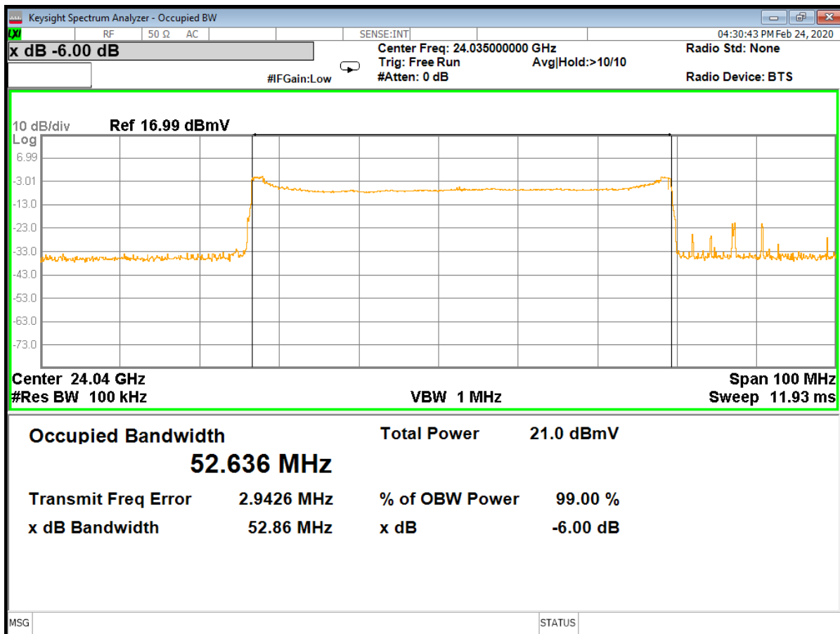
Figure 39 – Occupied Bandwidth, Low channel (48 MHz) Uncorrected measurement as recorded on spectrum analyzer
