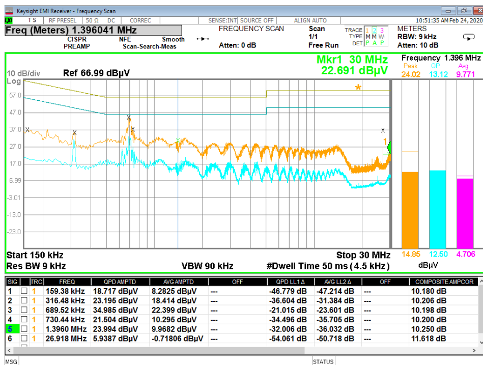
Figure 42 - Conducted Emissions Plot, Line
