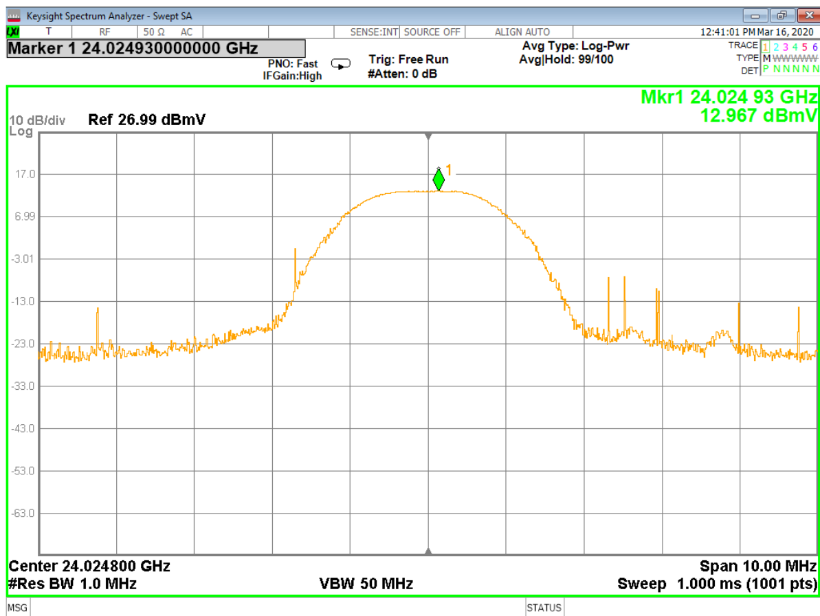
Figure 21 - Analyzer Measurement – Fundamental, Low Channel (Single Frequency)
