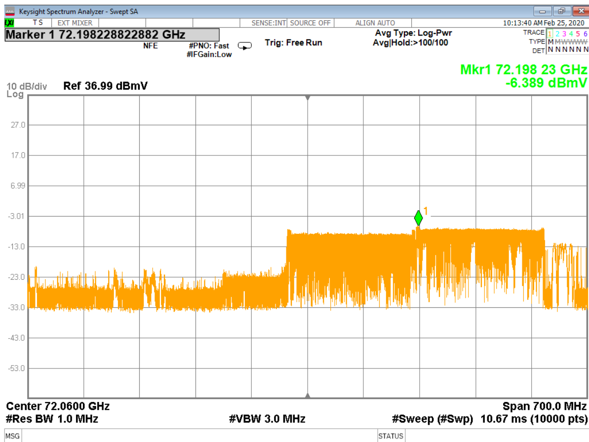
Figure 14 - Analyzer Measurement – 3 rd Harmonic, Low Channel (48 MHz) (swept frequency)
