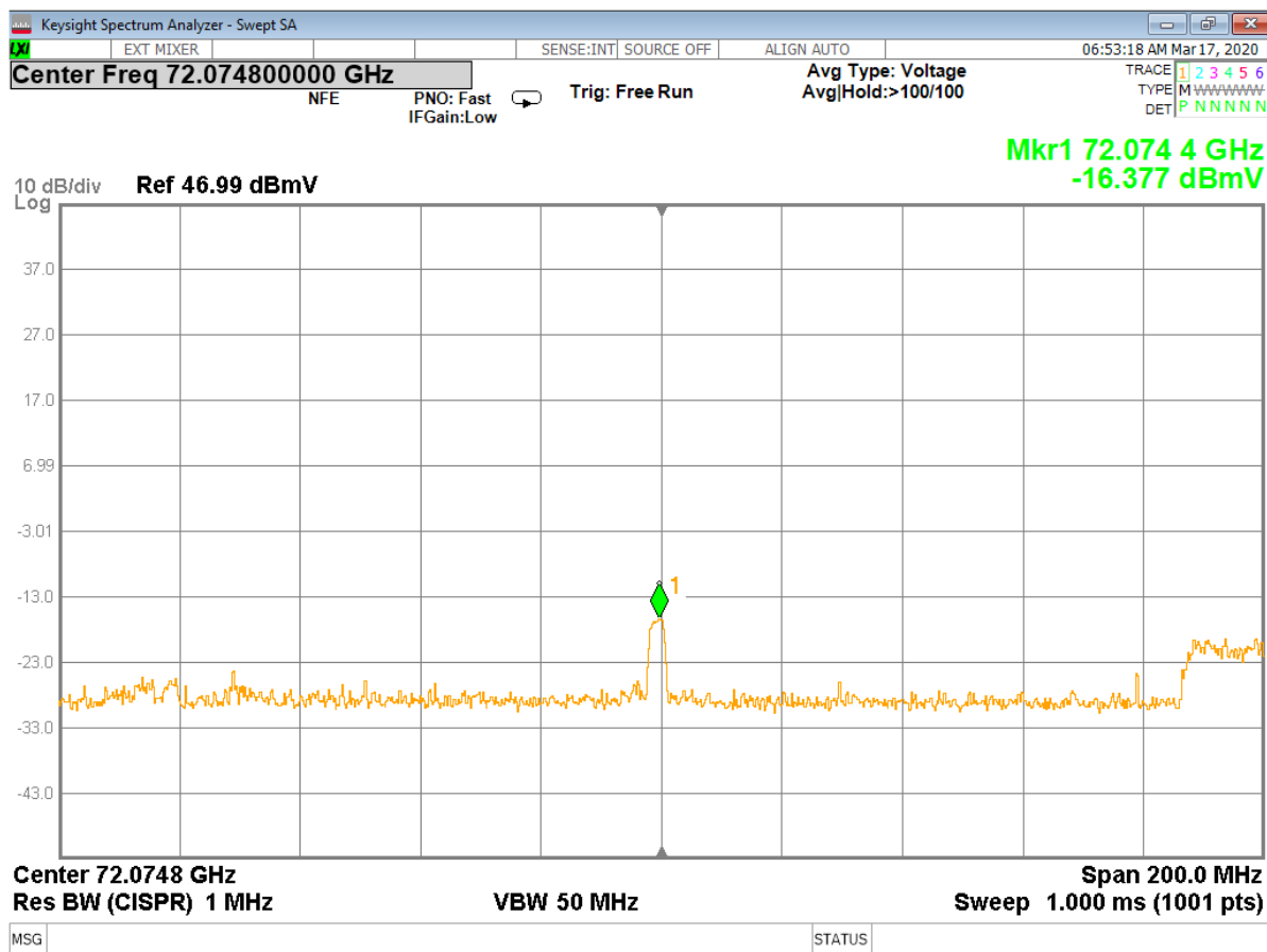
Figure 23 - Analyzer Measurement – 3 rd Harmonic, Low Channel (Single Frequency)
