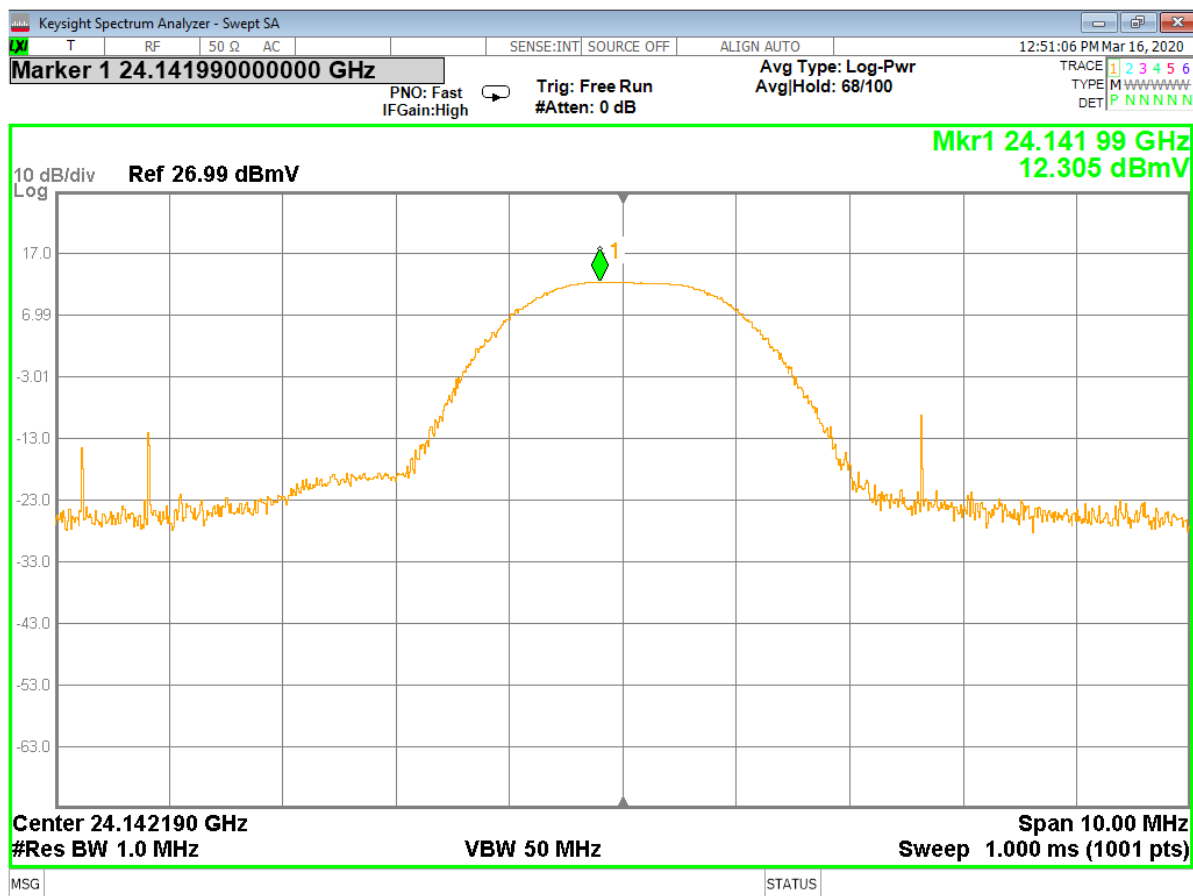
Figure 24 - Analyzer Measurement – Fundamental, Mid Channel (Single Frequency)
