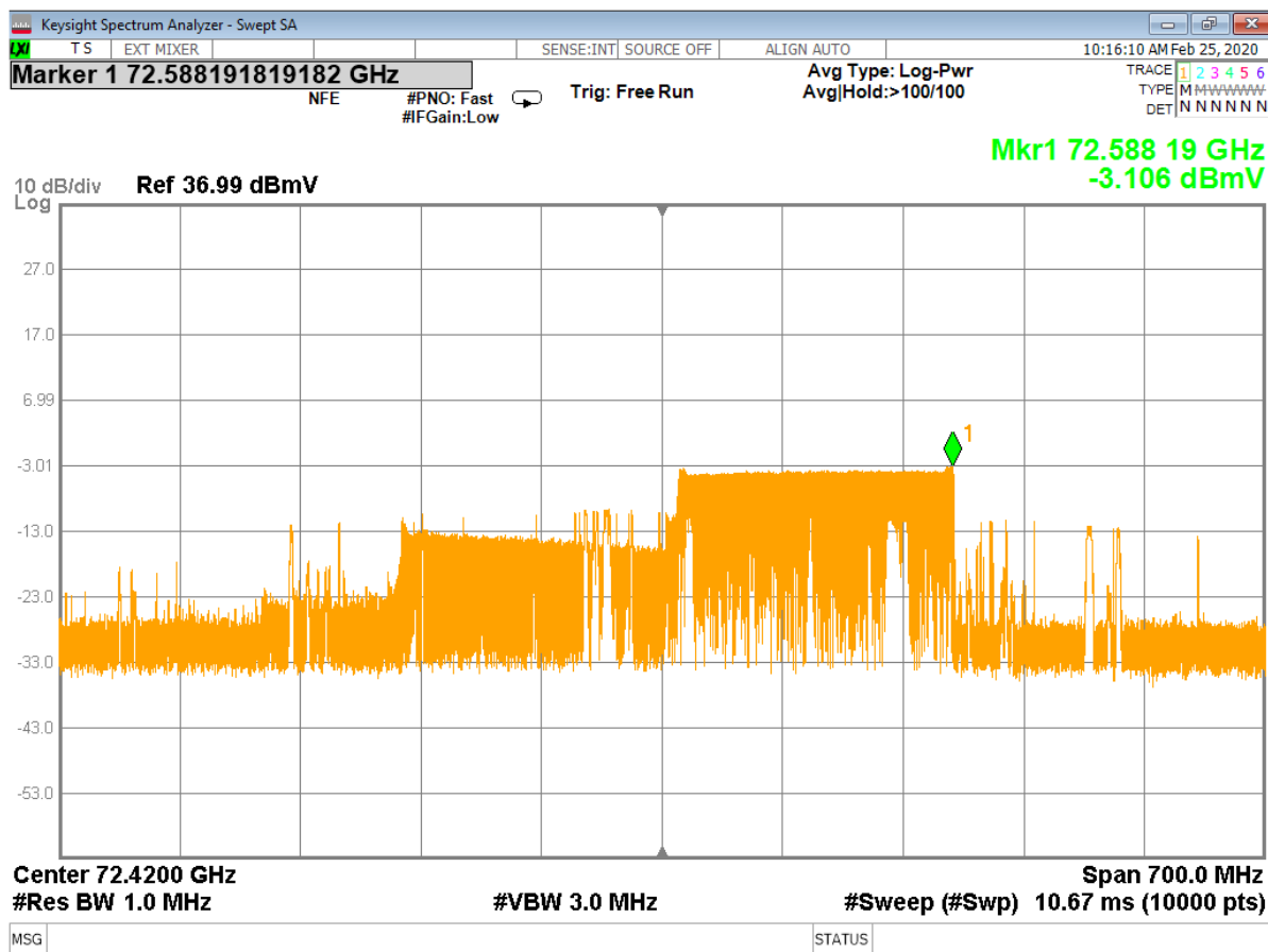
Figure 17 - Analyzer Measurement – 3 rd Harmonic, Mid Channel (48 MHz) (swept frequency)
