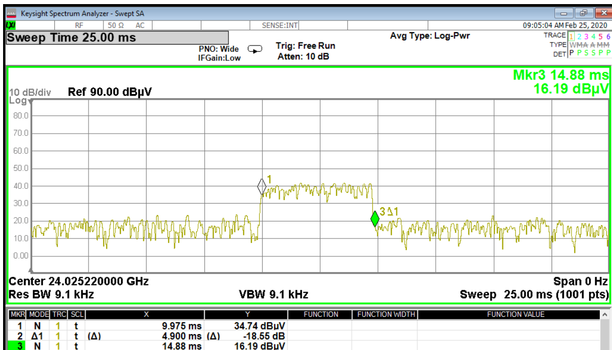
Figure 1 - On time / pulse width = 4.9 ms
