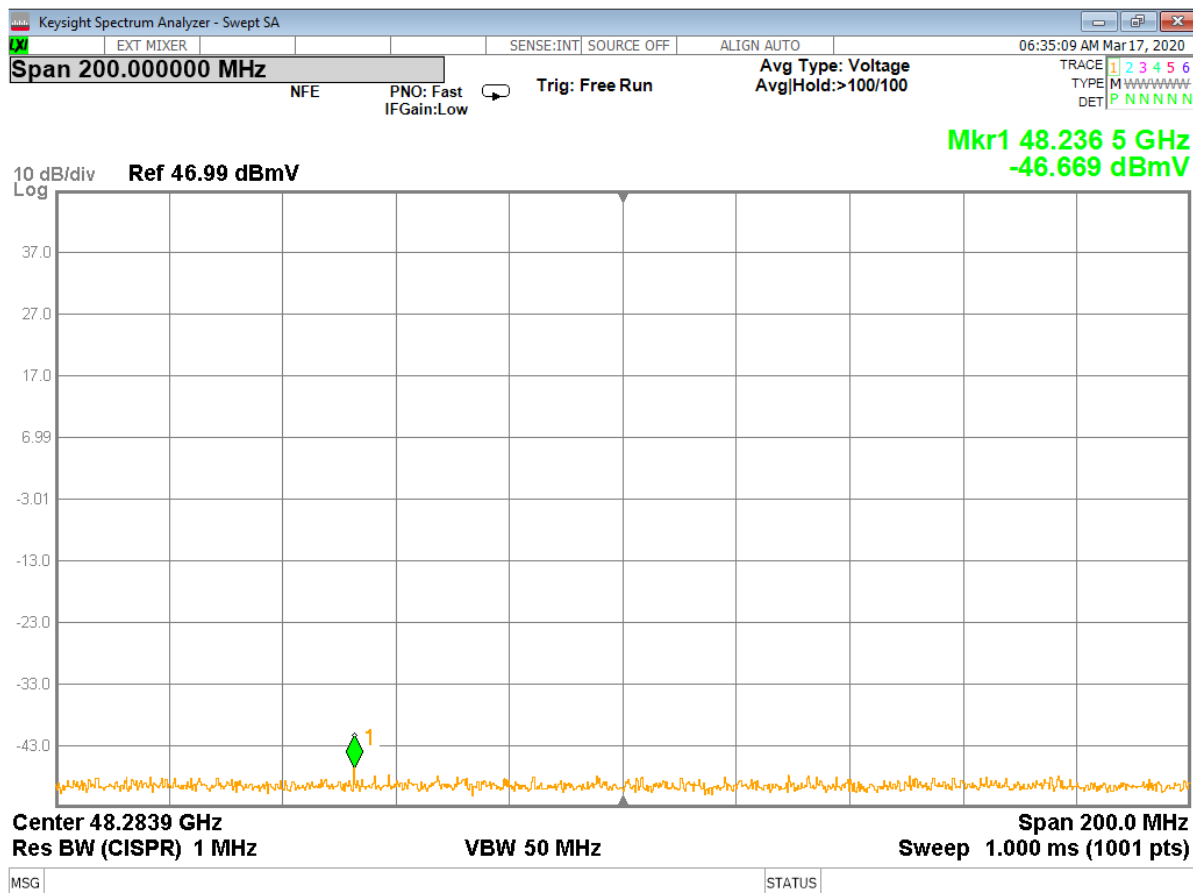
Figure 25 - Analyzer Measurement – 2 nd Harmonic, Mid Channel (Single Frequency)
