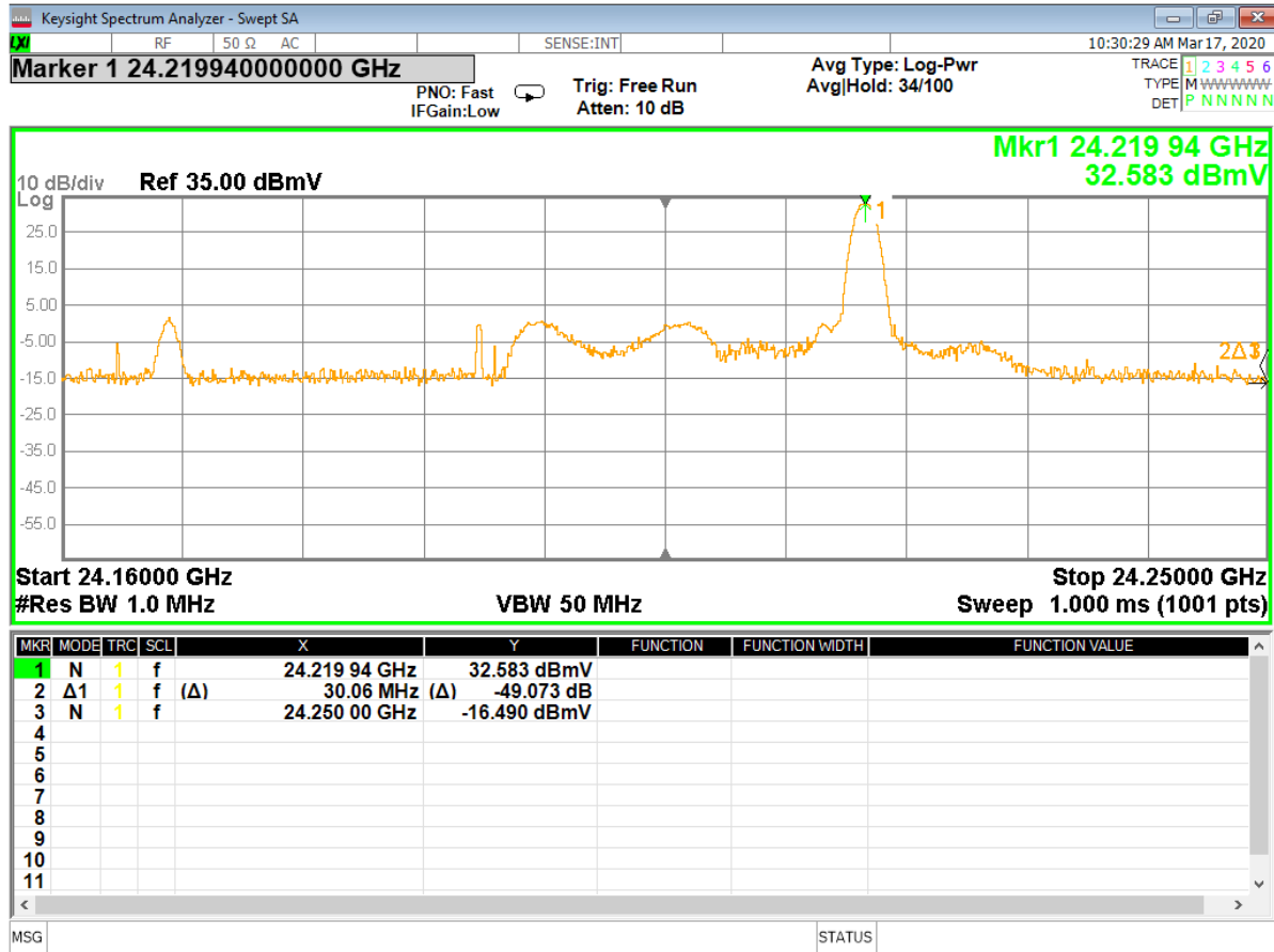
Figure 35 - Higher Band Edge (Single Frequency), 24.25 GHz Uncorrected measurement as recorded on spectrum analyzer, 5 cm test distance
