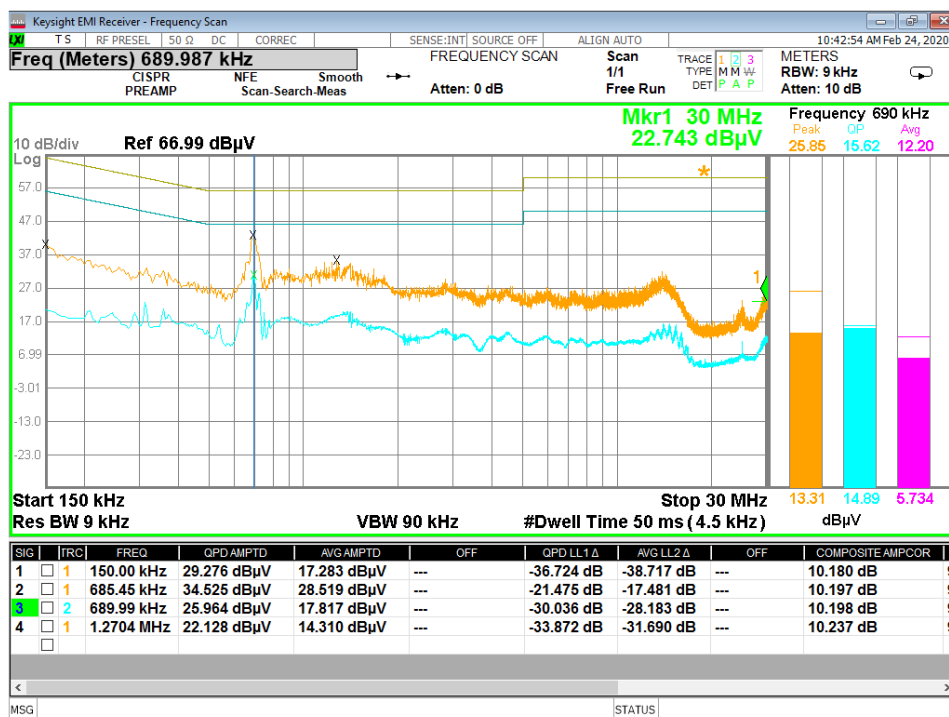
Figure 43 - Conducted Emissions Plot, Neutral
