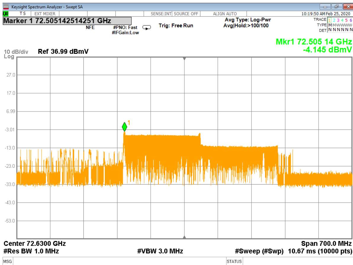
Figure 20 - Analyzer Measurement – 3 rd Harmonic, High Channel (48 MHz) (swept frequency)
