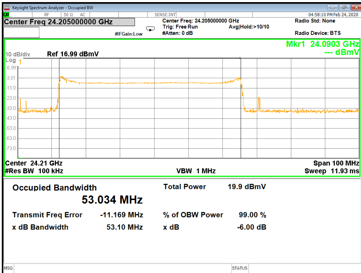
Figure 41 – Occupied Bandwidth, High channel (48 MHz) Uncorrected measurement as recorded on spectrum analyzer
