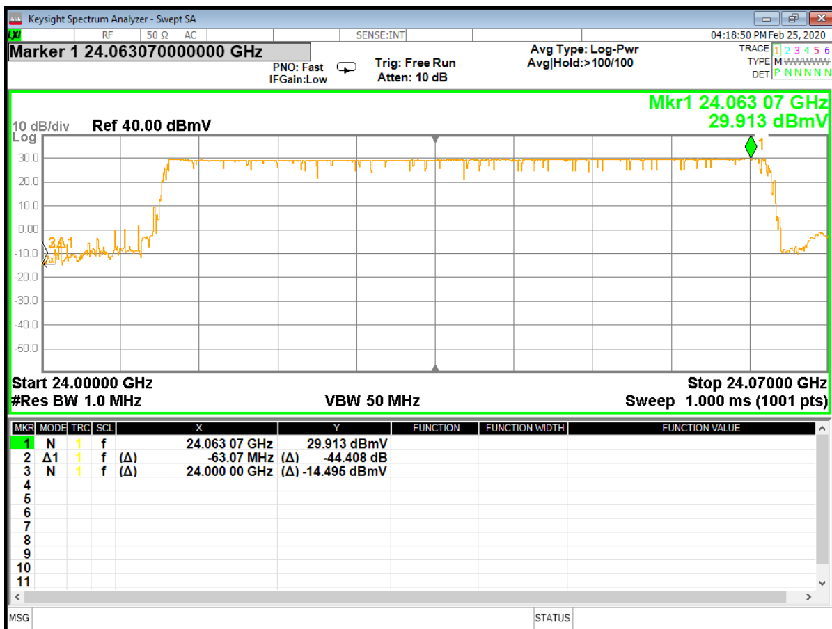
Figure 32 – Lower Band Edge (48 MHz) (swept frequency), 24.00 GHz Uncorrected measurement as recorded on spectrum analyzer, 5 cm test distance
