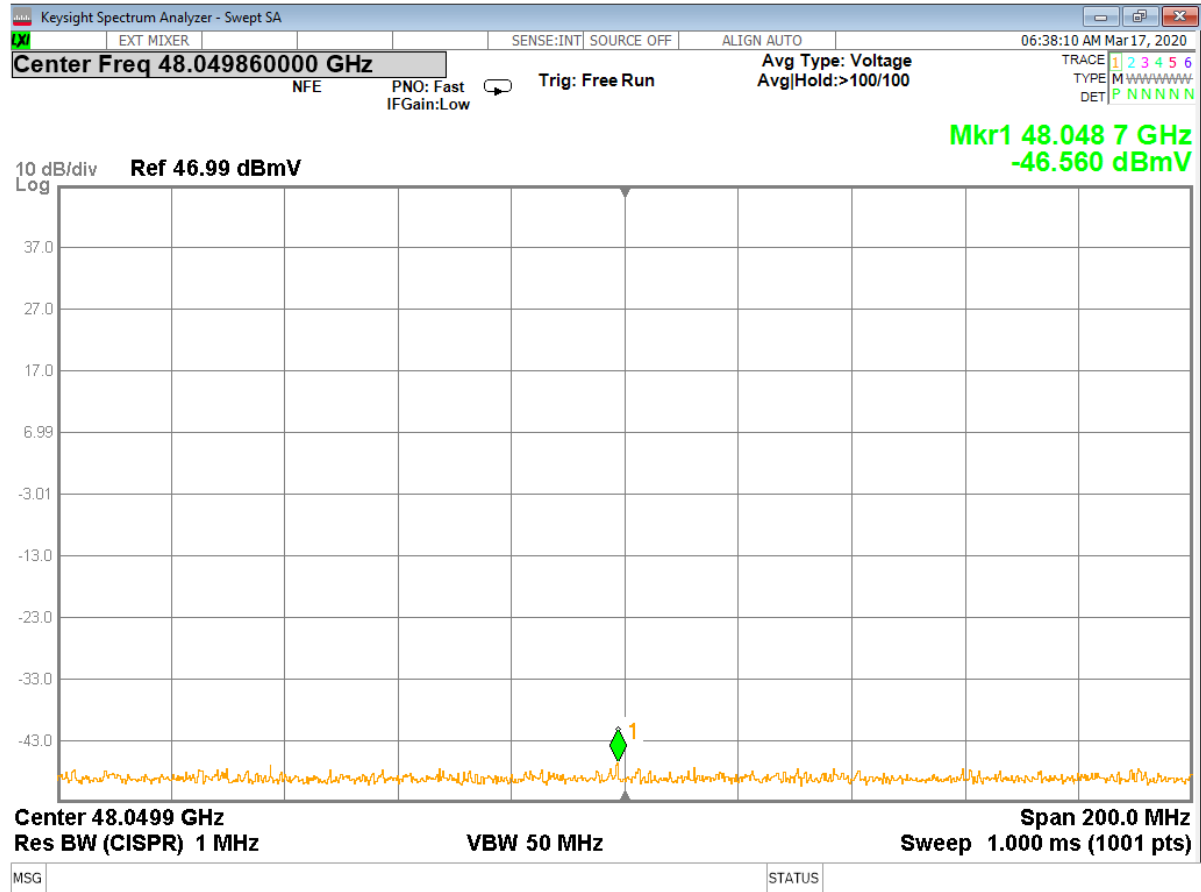
Figure 22 - Analyzer Measurement – 2 nd Harmonic, Low Channel (Single Frequency)
