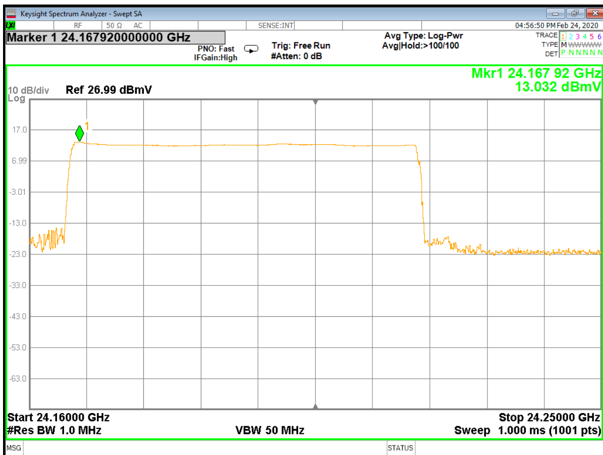
Figure 18 - Analyzer Measurement – Fundamental, High Channel (48 MHz) (swept frequency)
