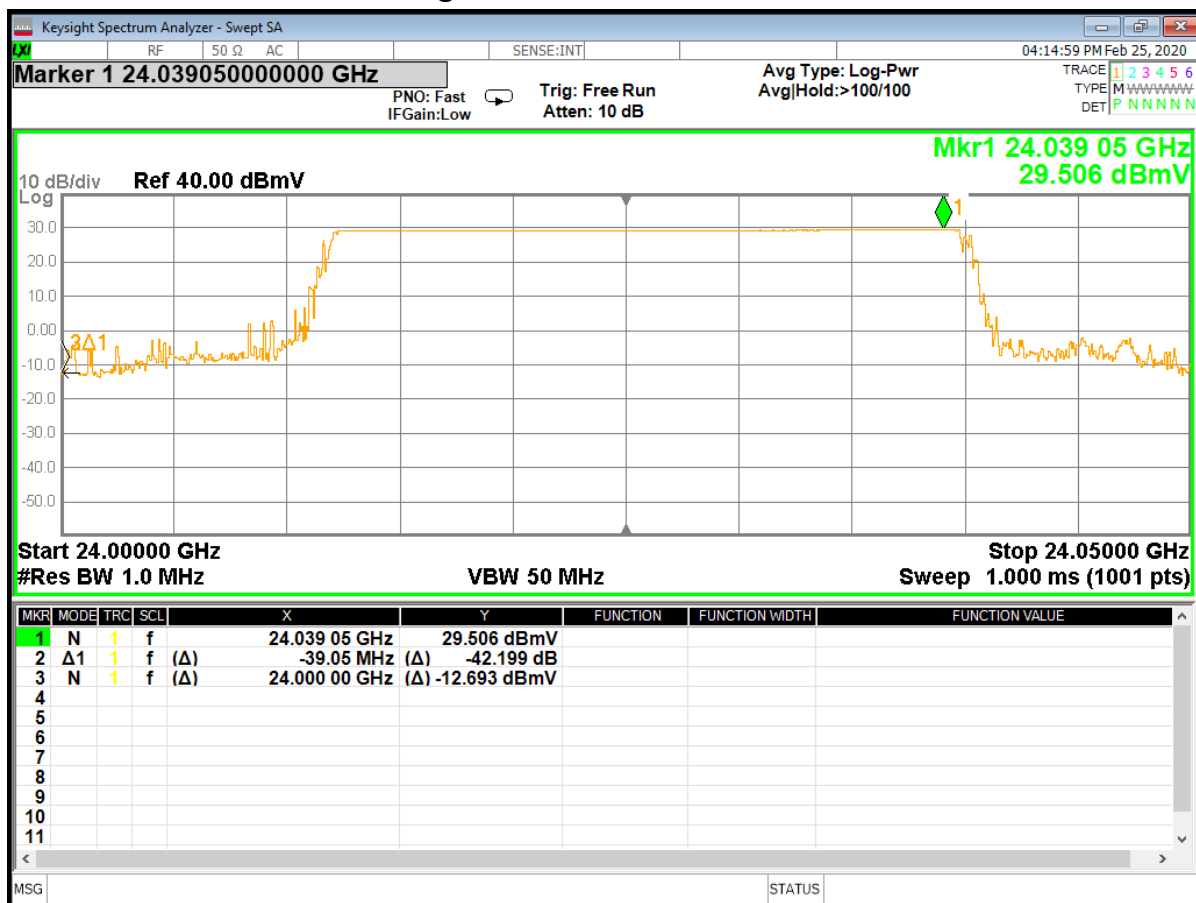
Figure 30 – Lower Band Edge (24 MHz) (swept frequency), 24.00 GHz Uncorrected measurement as recorded on spectrum analyzer, 5 cm test distance
