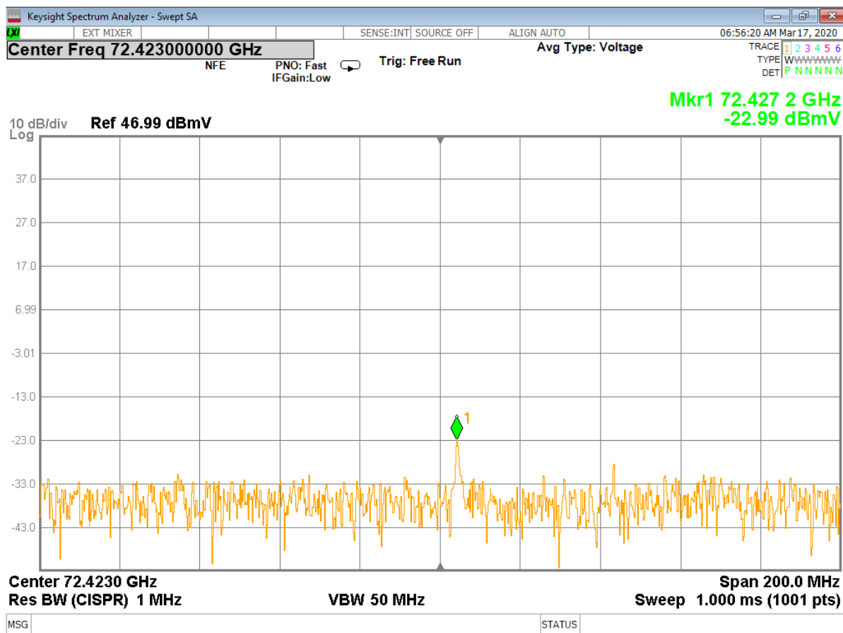
Figure 26 - Analyzer Measurement – 3 rd Harmonic, Mid Channel (Single Frequency)
