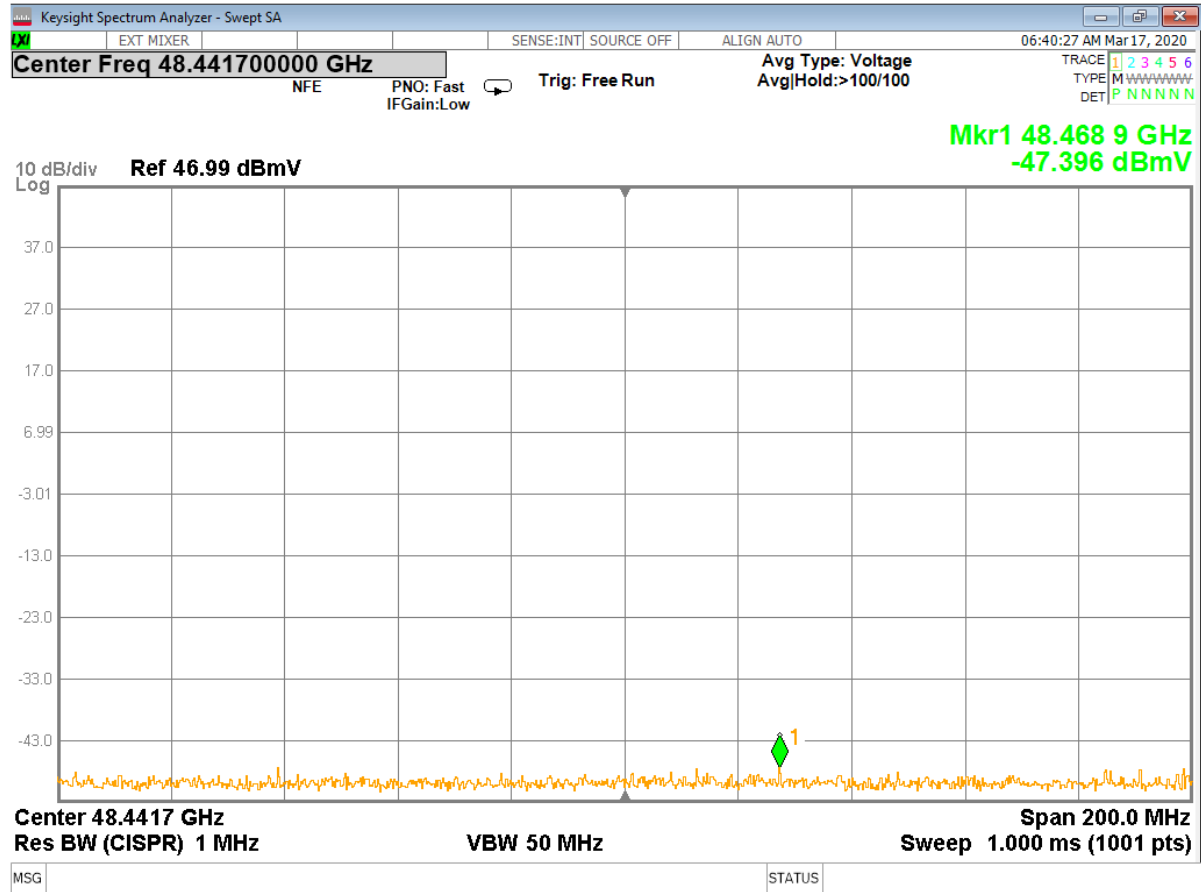
Figure 28 - Analyzer Measurement – 2 nd Harmonic, High Channel (Single Frequency)
