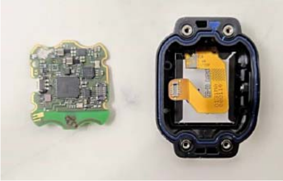
Figure E19.3 – Internal Photo –PCB / Back Cover
