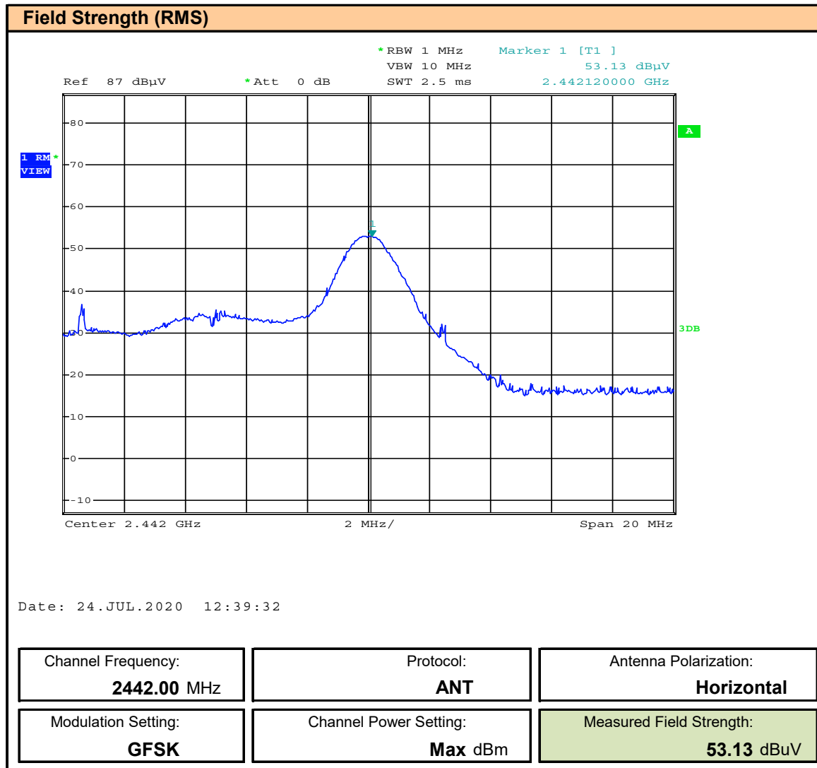
Plot D.8 – Field Strength, ANT, Average, Horizontal, 2442MHz
