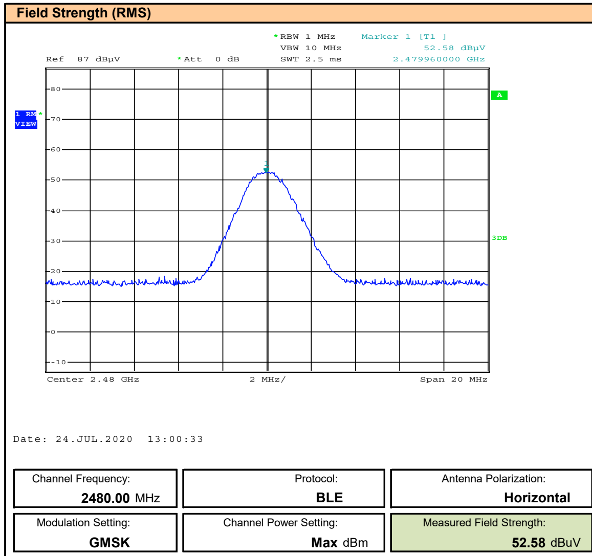
Plot D.21 – Field Strength, BLE, Average, Horizontal, 2480MHz
