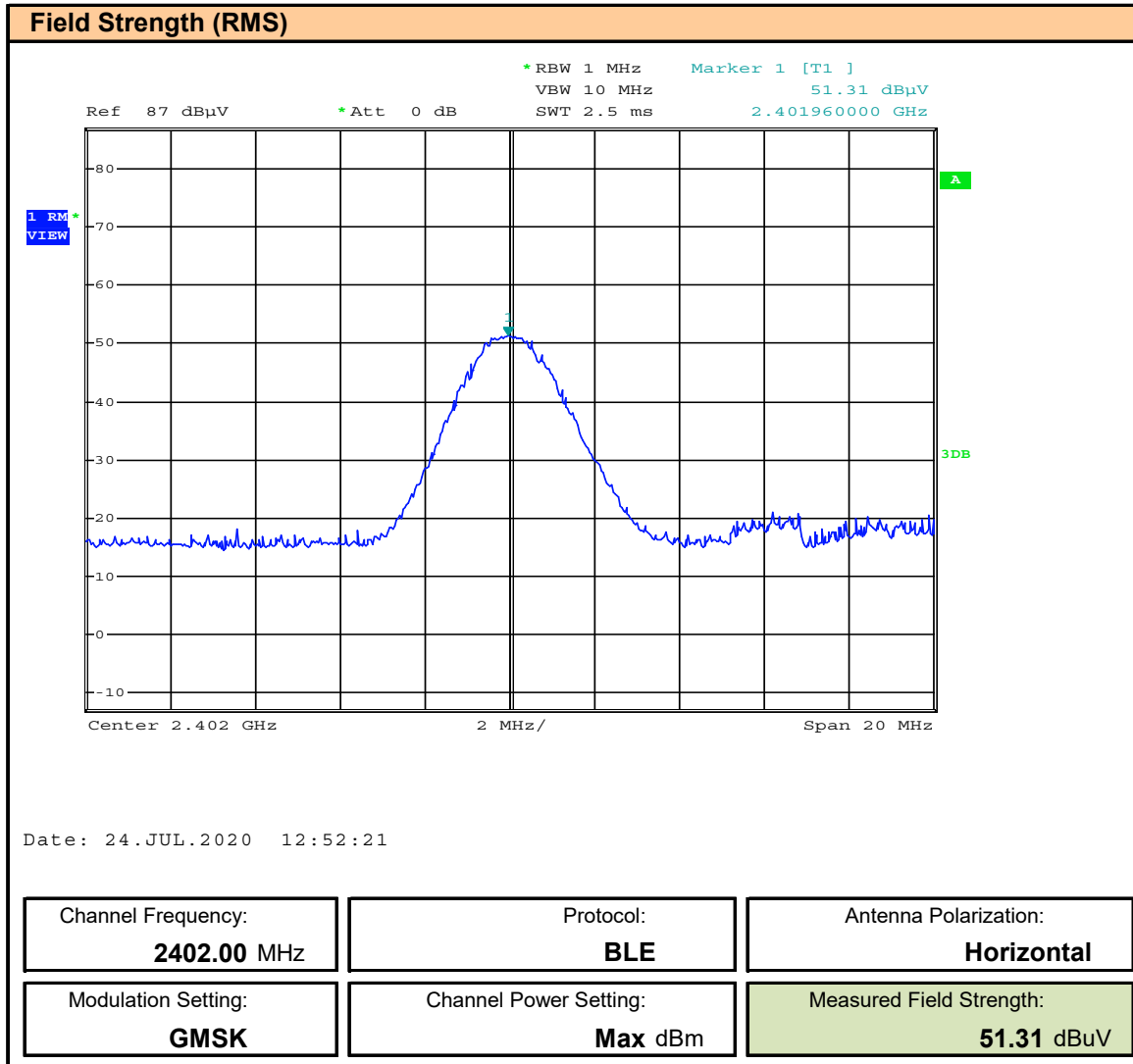
Plot D.19 – Field Strength, BLE, Average, Horizontal, 2402MHz
