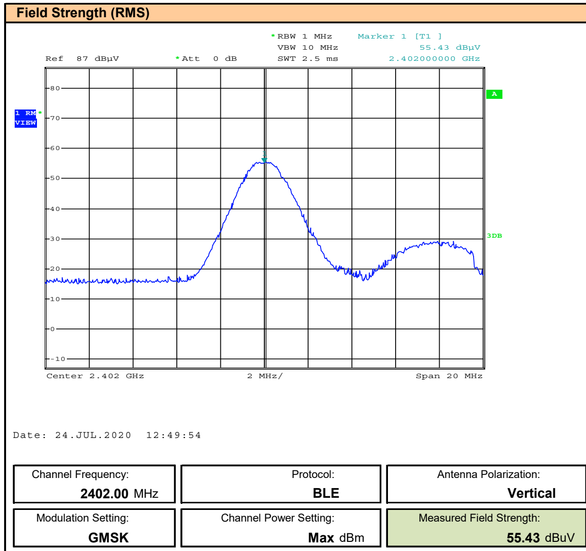
Plot D.22 – Field Strength, BLE, Average, Vertical, 2402MHz
