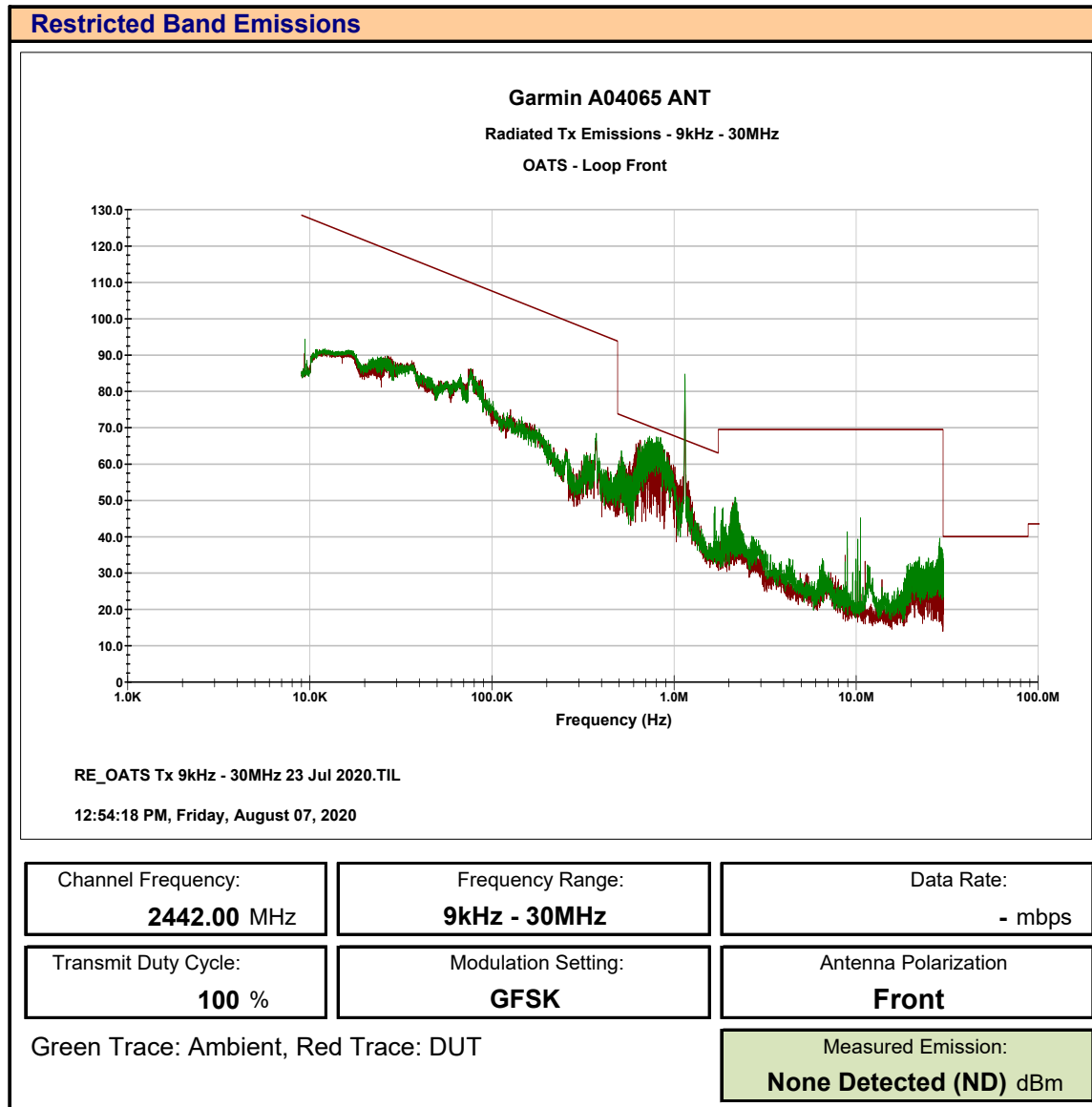
Plot E.1 – Radiated Tx Measurement, ANT, Front, 9kHz-30MHz
