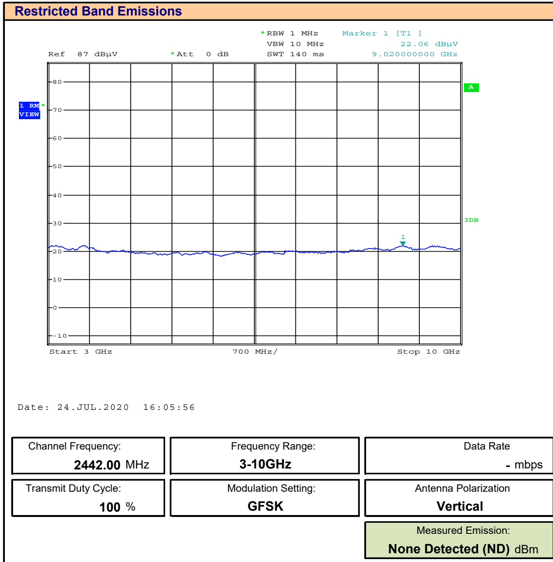
Plot E.11 – Radiated Tx Measurement, ANT, Vertical, 3-10GHz
