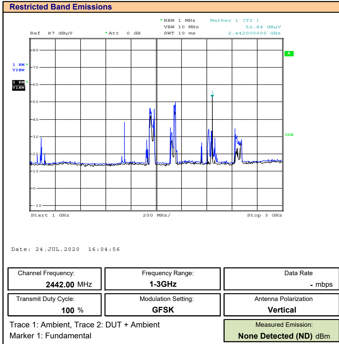
Plot E.10 – Radiated Tx Measurement, ANT, Vertical, 1-3GHz
