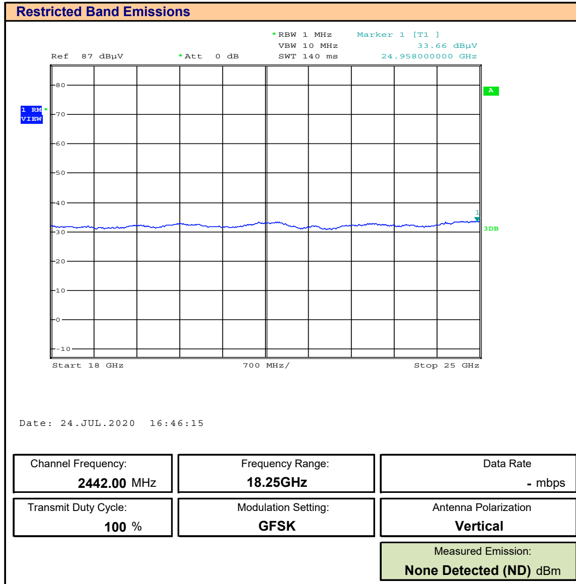
Plot E.14 – Radiated Tx Measurement, ANT, Vertical, 18-25GHz
