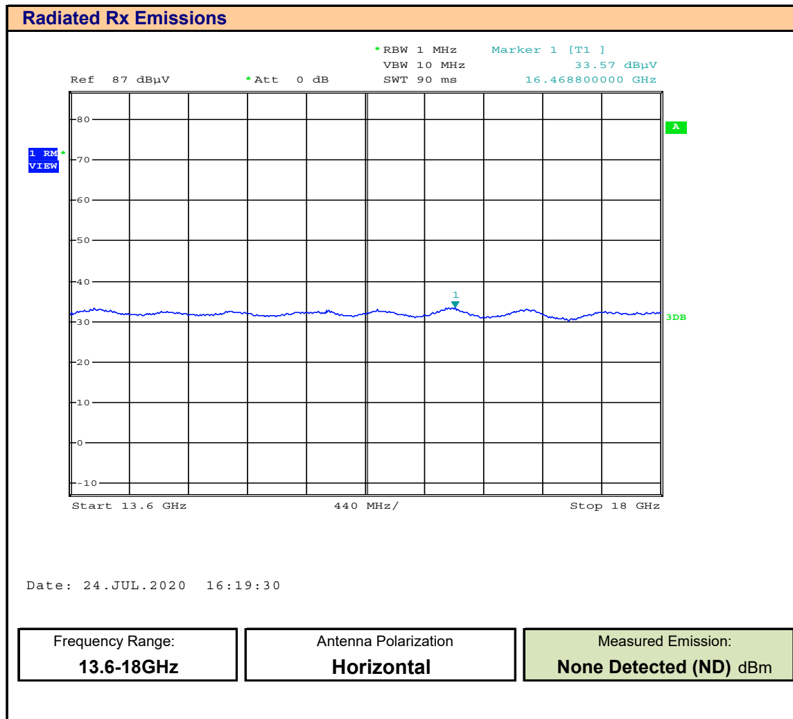
Plot F.11 – Radiated Rx Emissions, 13.6-18GHz, Horizontal
