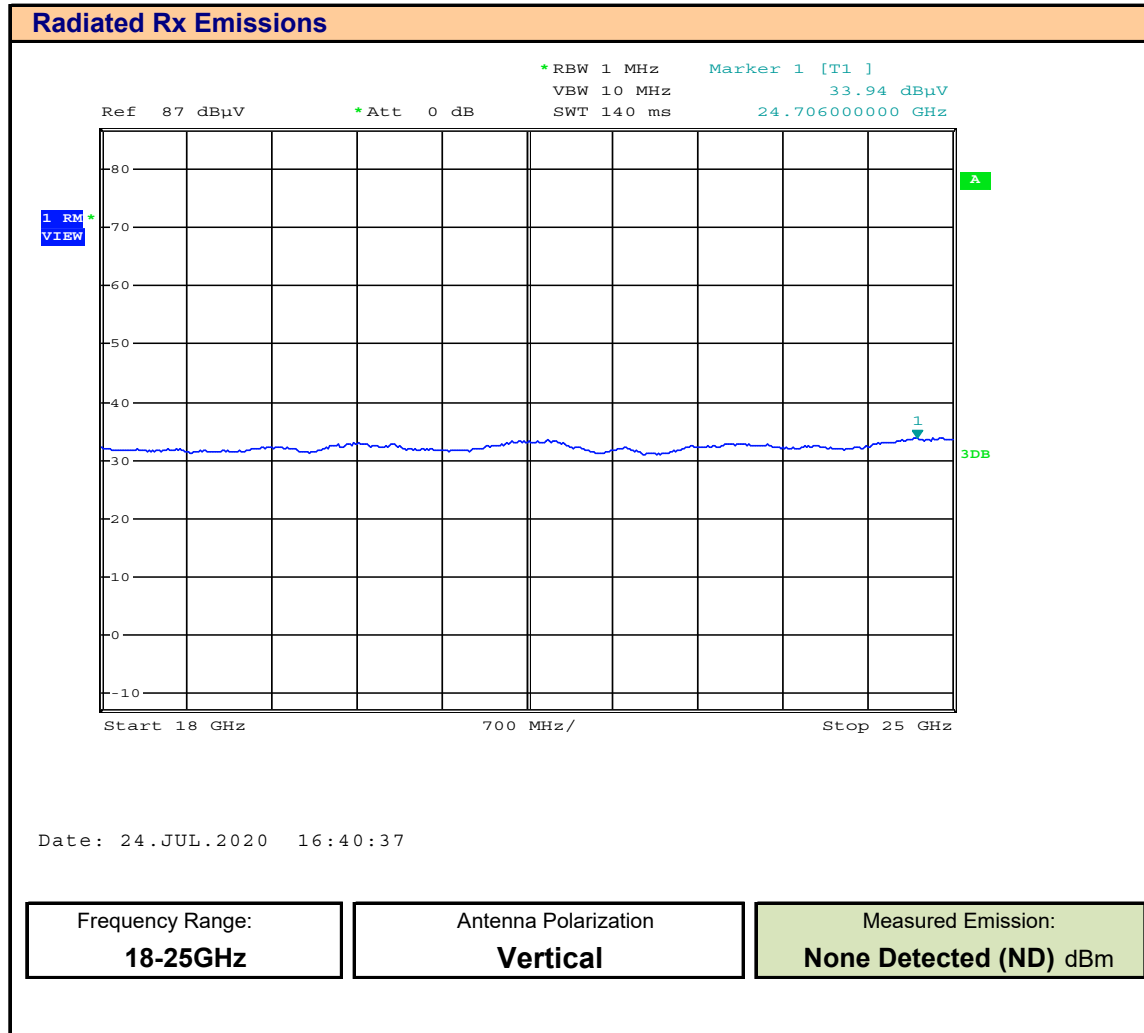
Plot F.14 – Radiated Rx Emissions, 18*25GHz, Vertical
