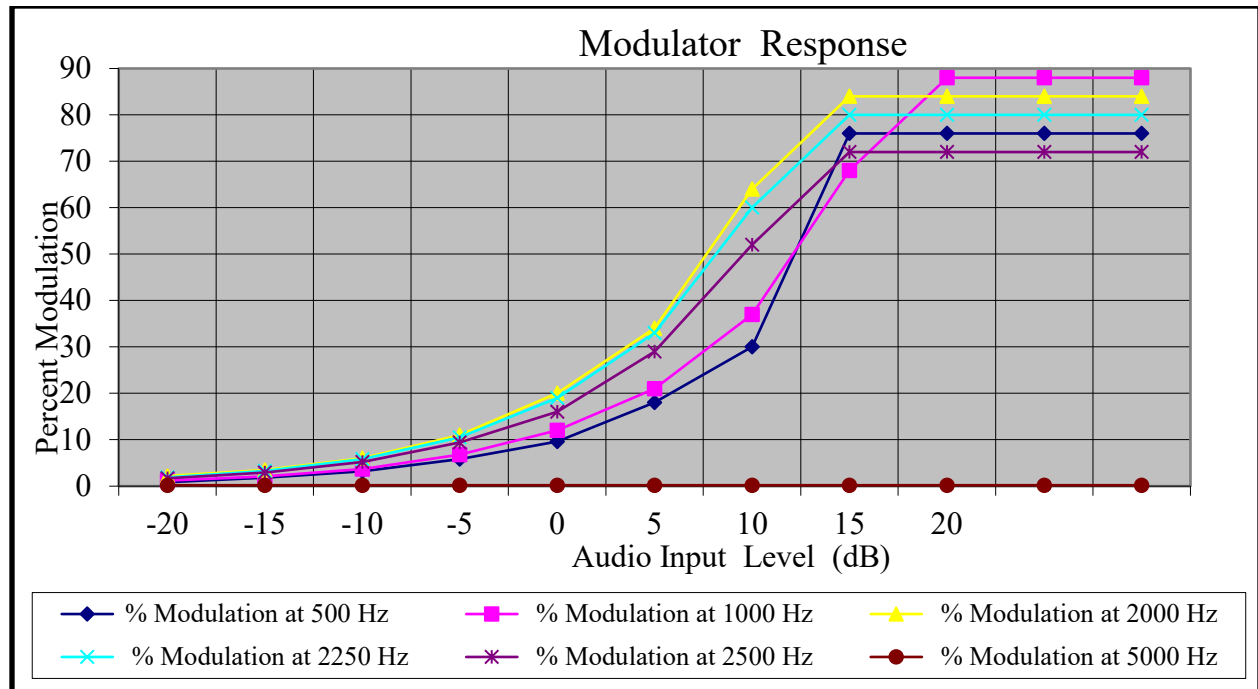
Figure 4 Modulation Characteristics
