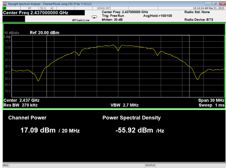
Figure 3 – Conducted Peak Power Measurement, Wifi B 1MB
