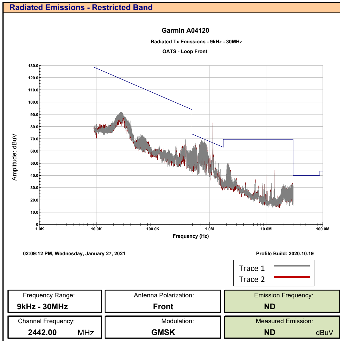
Plot 11.1 – Radiated Tx, Restricted Band, 9kHz – 30MHz, Front
