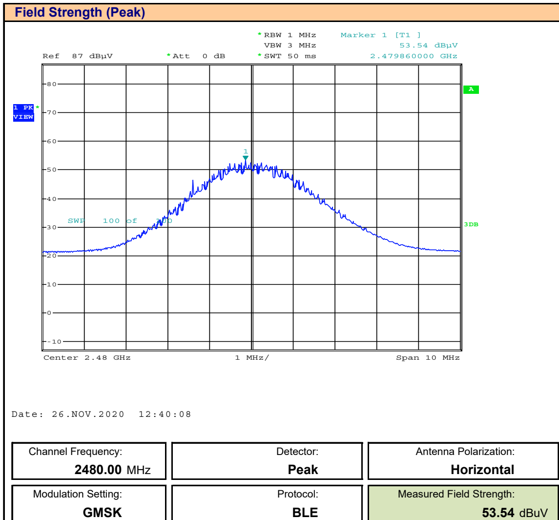
Plot 9.9 – Field Strength – 2480MHz, Peak, Horizontal
