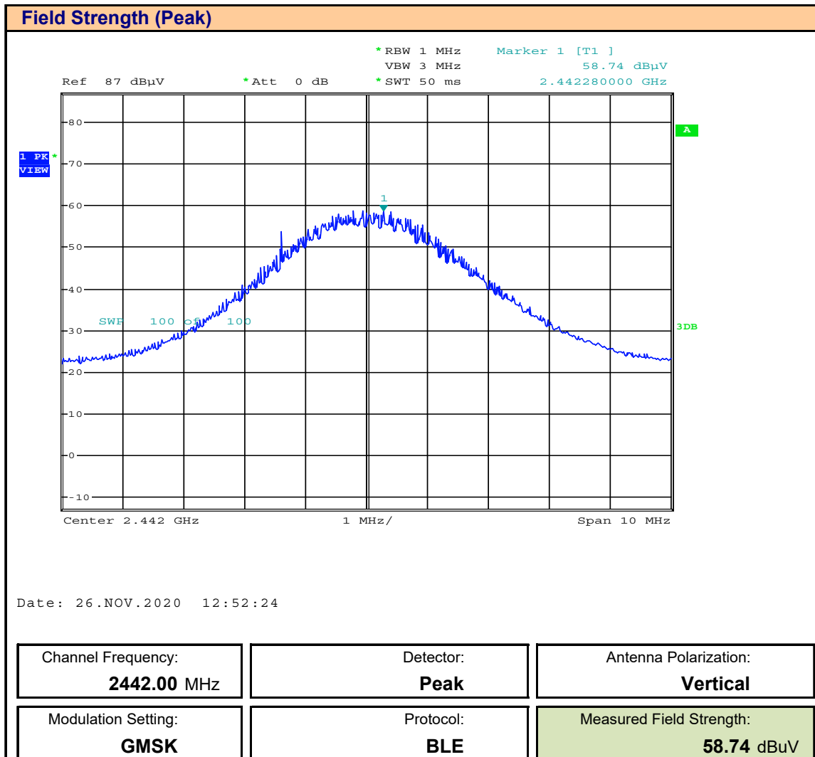
Plot 9.11 – Field Strength – 2442MHz, Peak, Vertical
