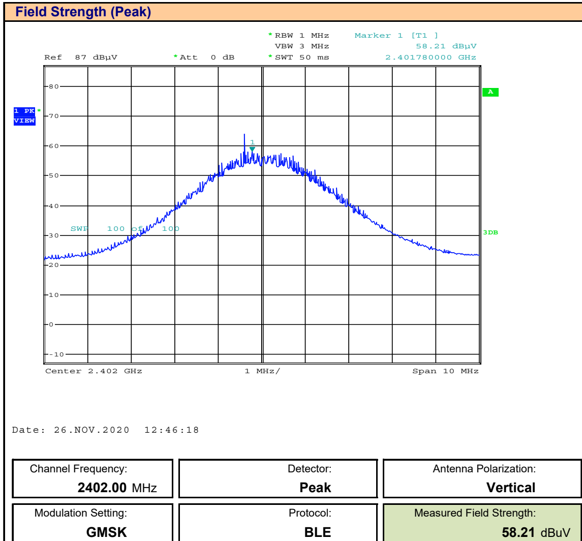
Plot 9.10 – Field Strength – 2402MHz, Peak, Vertical
