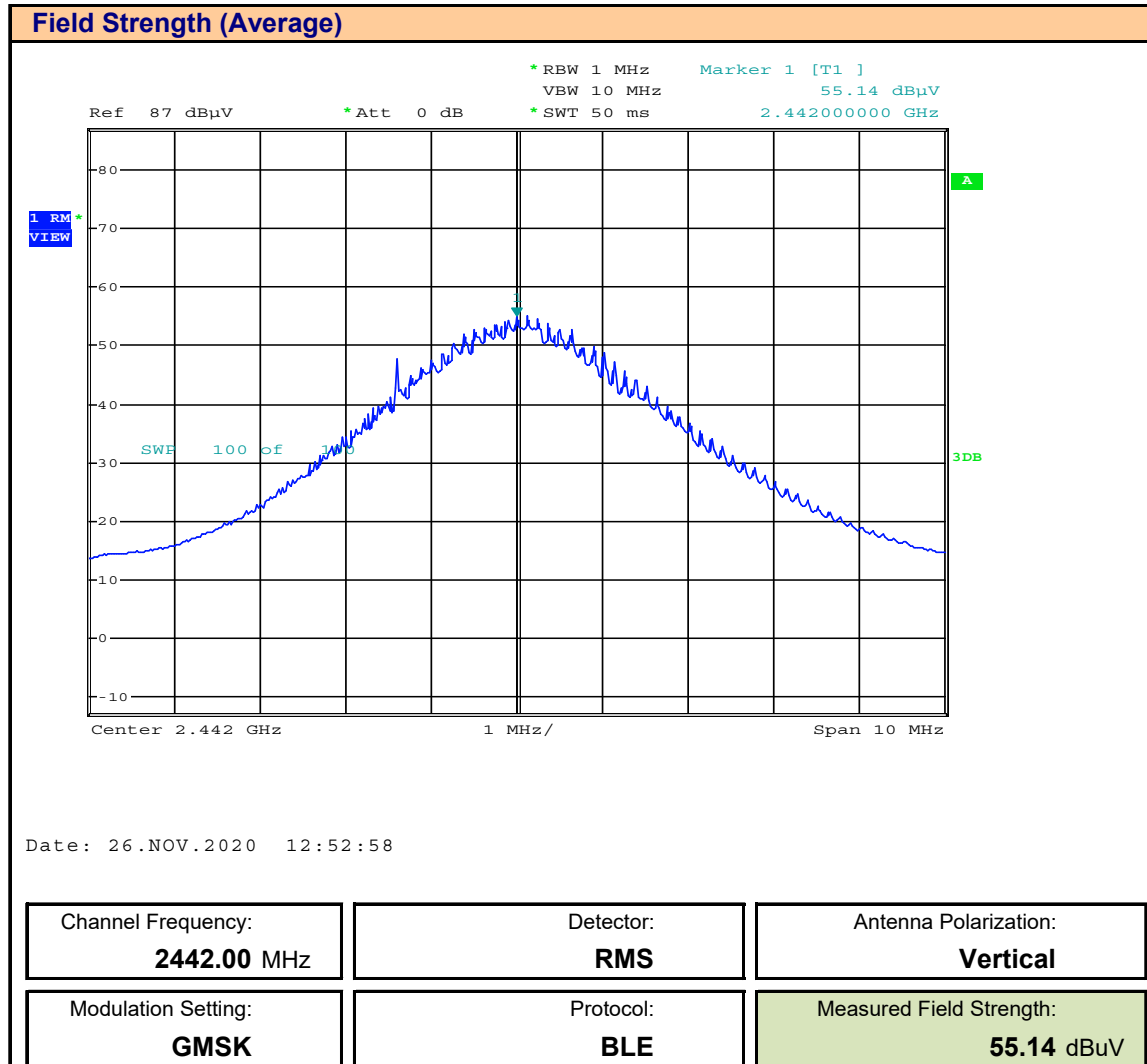
Plot 9.5 – Field Strength – 2442MHz, RMS, Vertical
