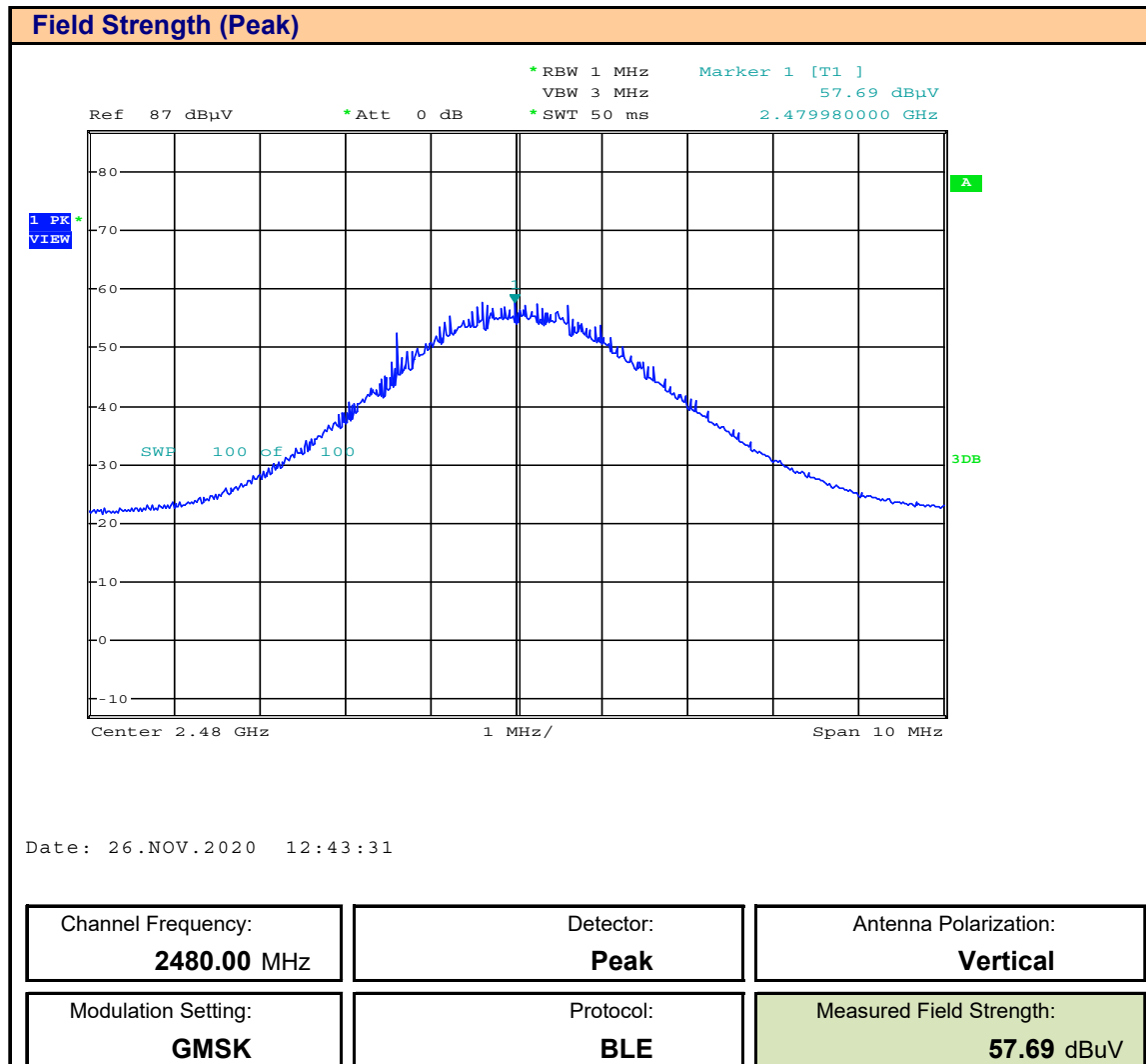
Plot 9.12 – Field Strength – 2480MHz, Peak, Vertical
