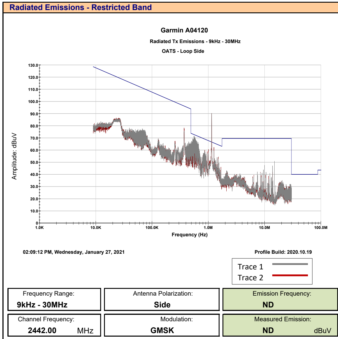
Plot 11.2 – Radiated Tx, Restricted Band, 9kHz – 30MHz, Side
