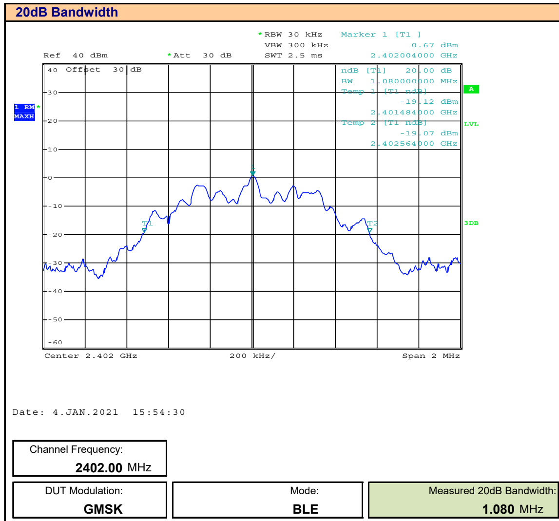
Plot 10.1 – 20dB Bandwidth, 2402MHz
