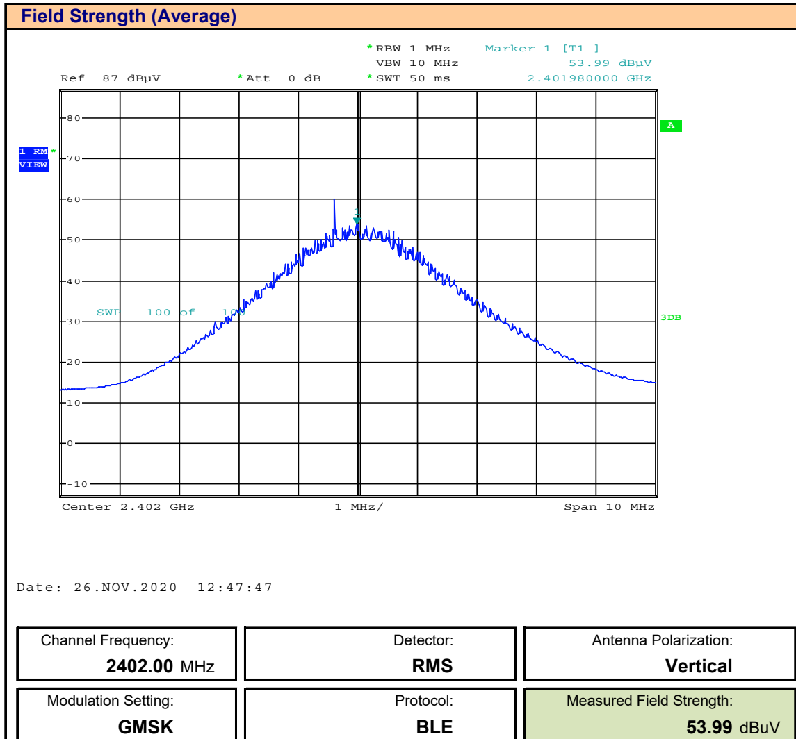
Plot 9.4 – Field Strength – 2402MHz, RMS, Vertical
