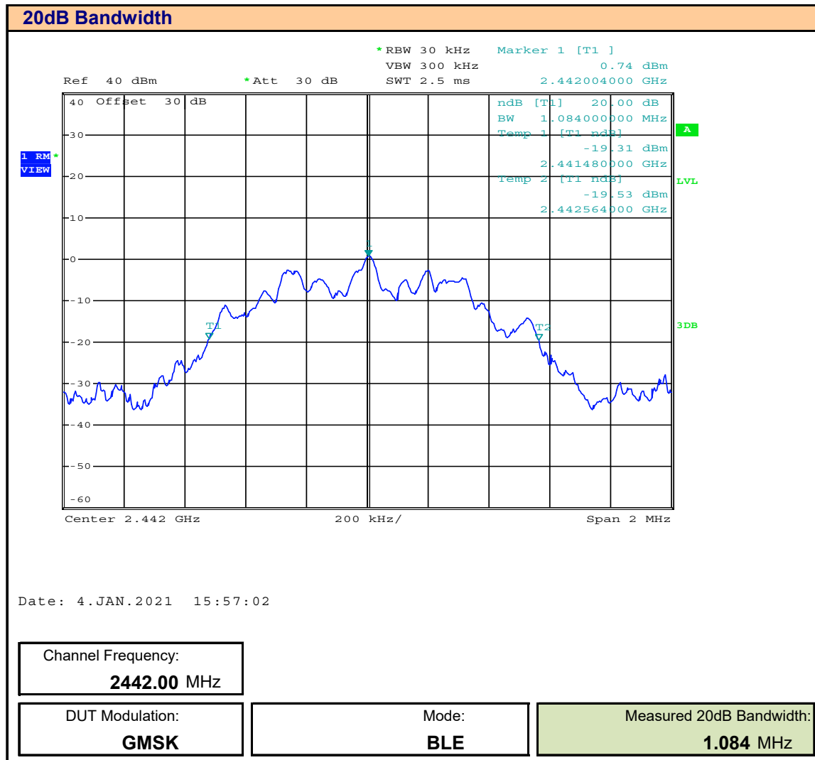
Plot 10.2 – 20dB Bandwidth, 2442MHz
