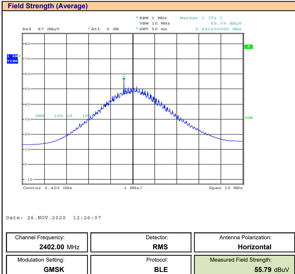
Plot 9.1 – Field Strength – 2402MHz, RMS, Horizontal
