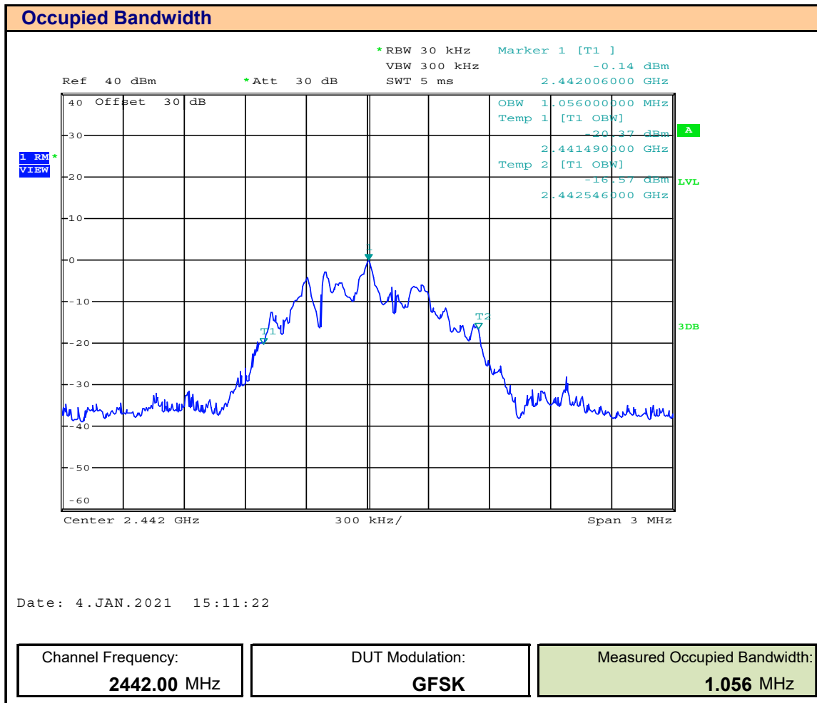
Plot 8.2 – Occupied Bandwidth – 2442MHz
