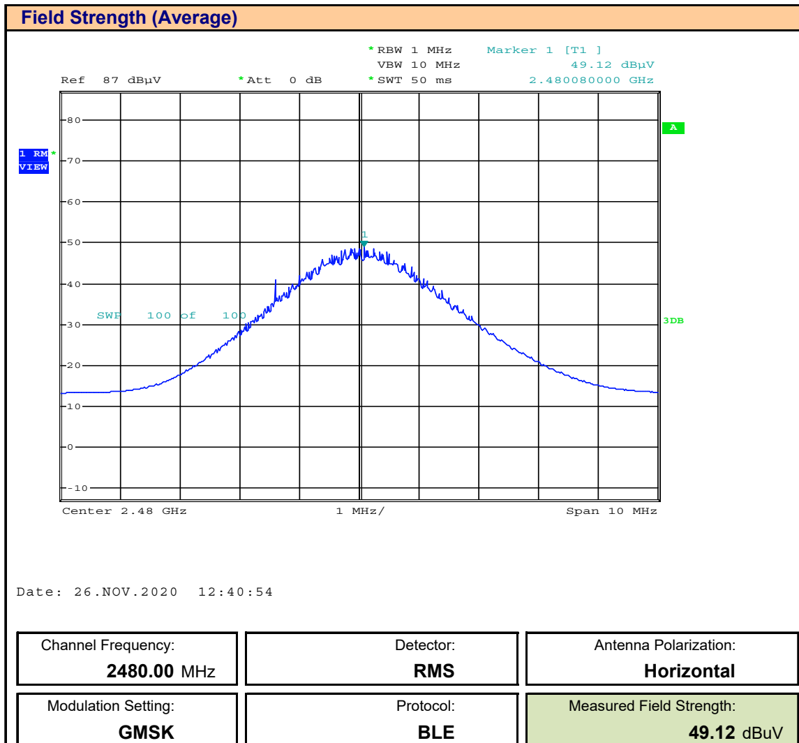
Plot 9.3 – Field Strength – 2480MHz, RMS, Horizontal
