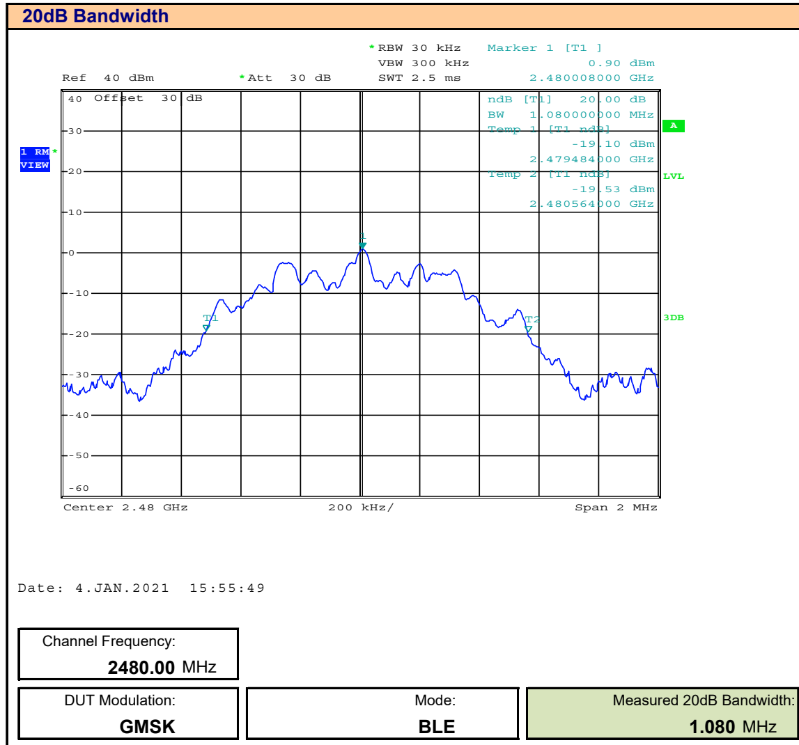
Plot 10.3 – 20dB Bandwidth, 2480MHz
