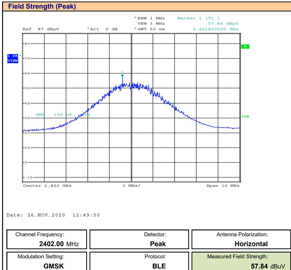
Plot 9.7 – Field Strength – 2402MHz, Peak, Horizontal
