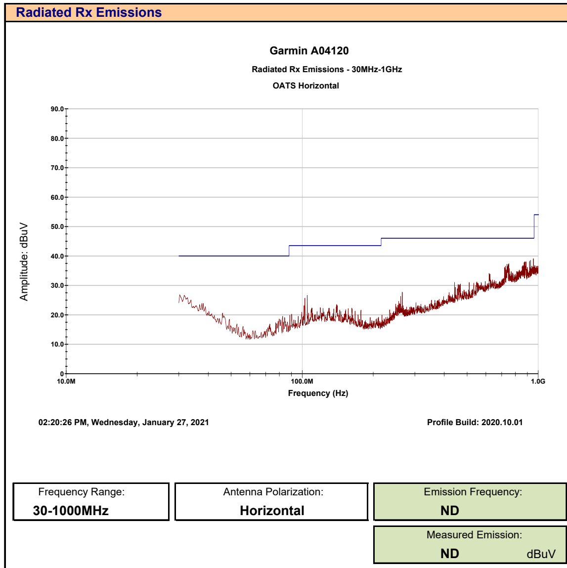
Plot 12.1 – Radiated Rx, Restricted Band, 30 - 1000MHz, Horizontal
