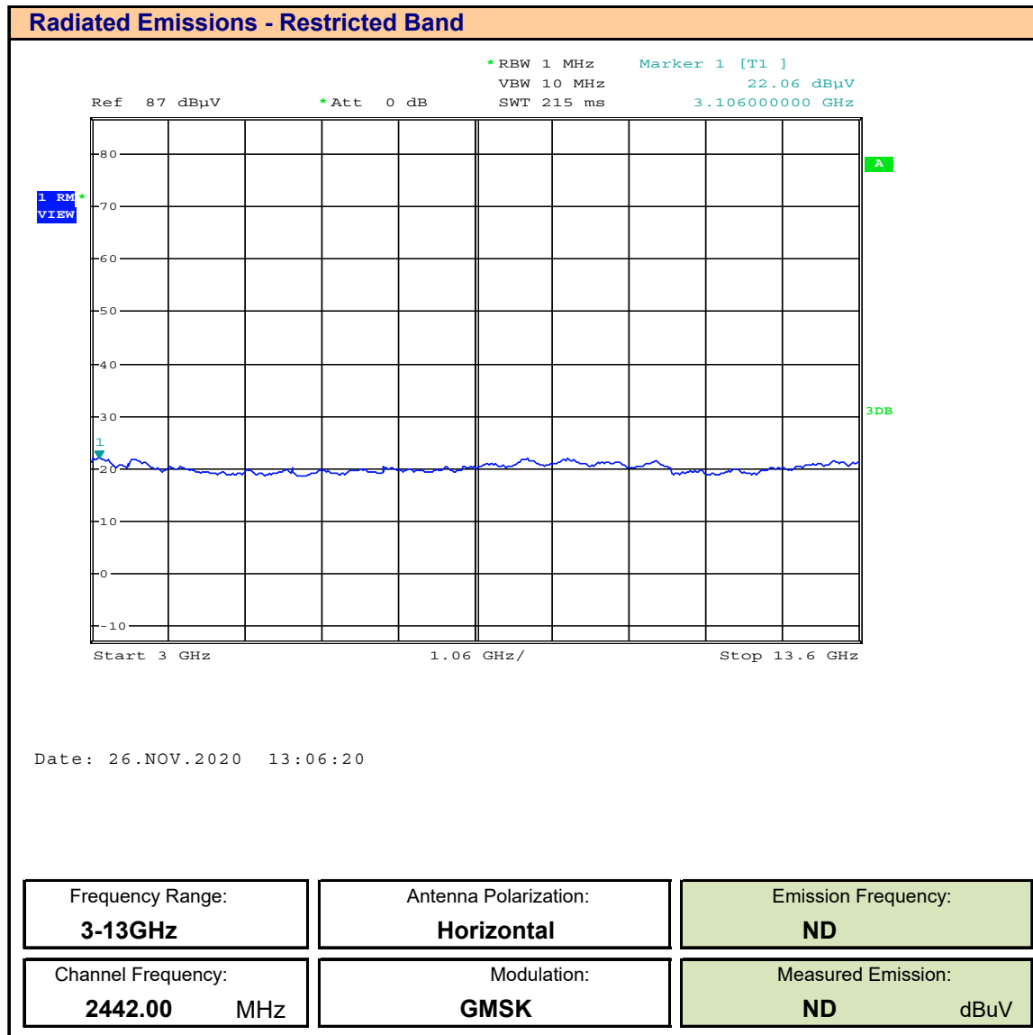
Plot 11.7 – Radiated Tx, Restricted Band, 3 – 13 GHz, Horizontal
