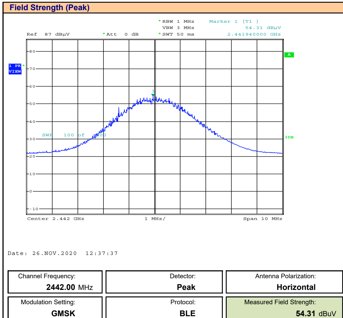
Plot 9.8 – Field Strength – 2442MHz, Peak, Horizontal
