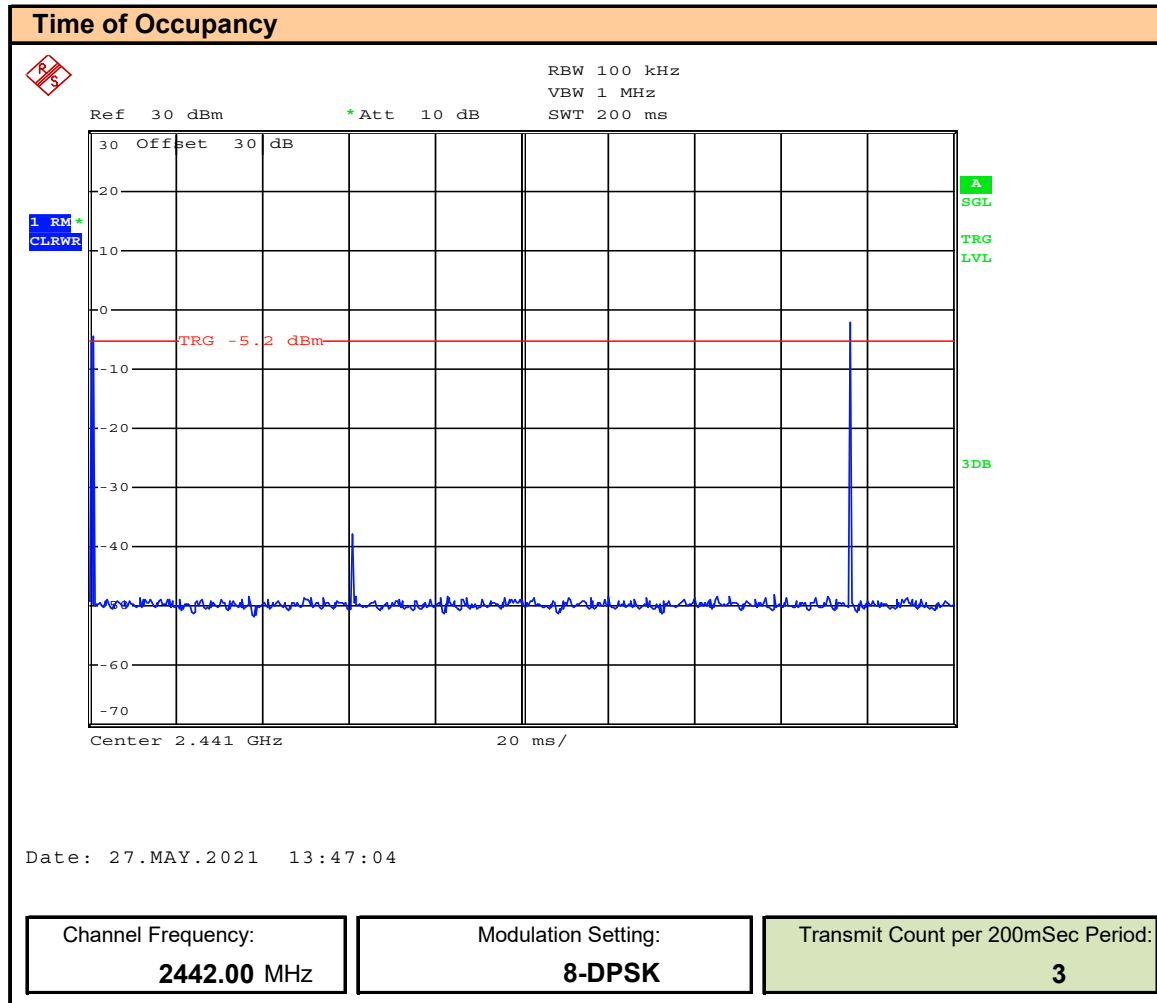
Plot 15.3 – Time of Occupancy, BT EDR 3MB
