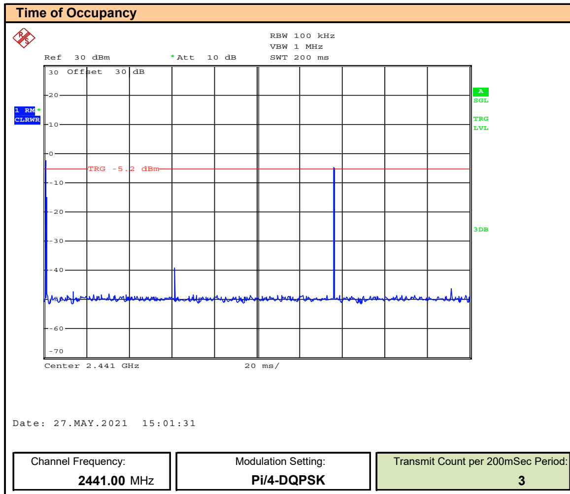
Plot 15.2 – Time of Occupancy, BT EDR 2MB
