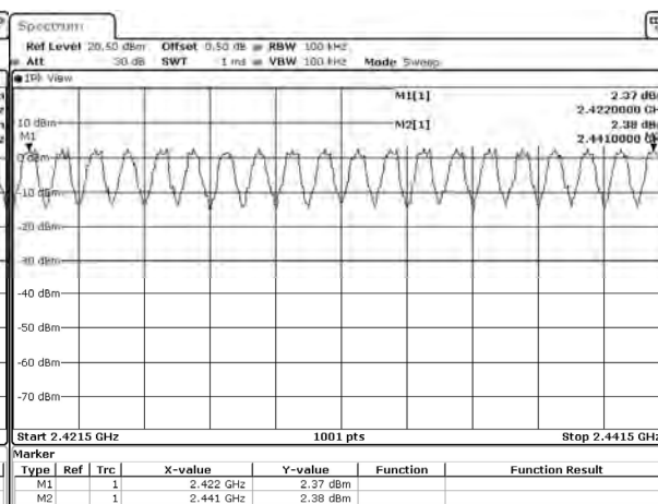
2422-2441MHz
