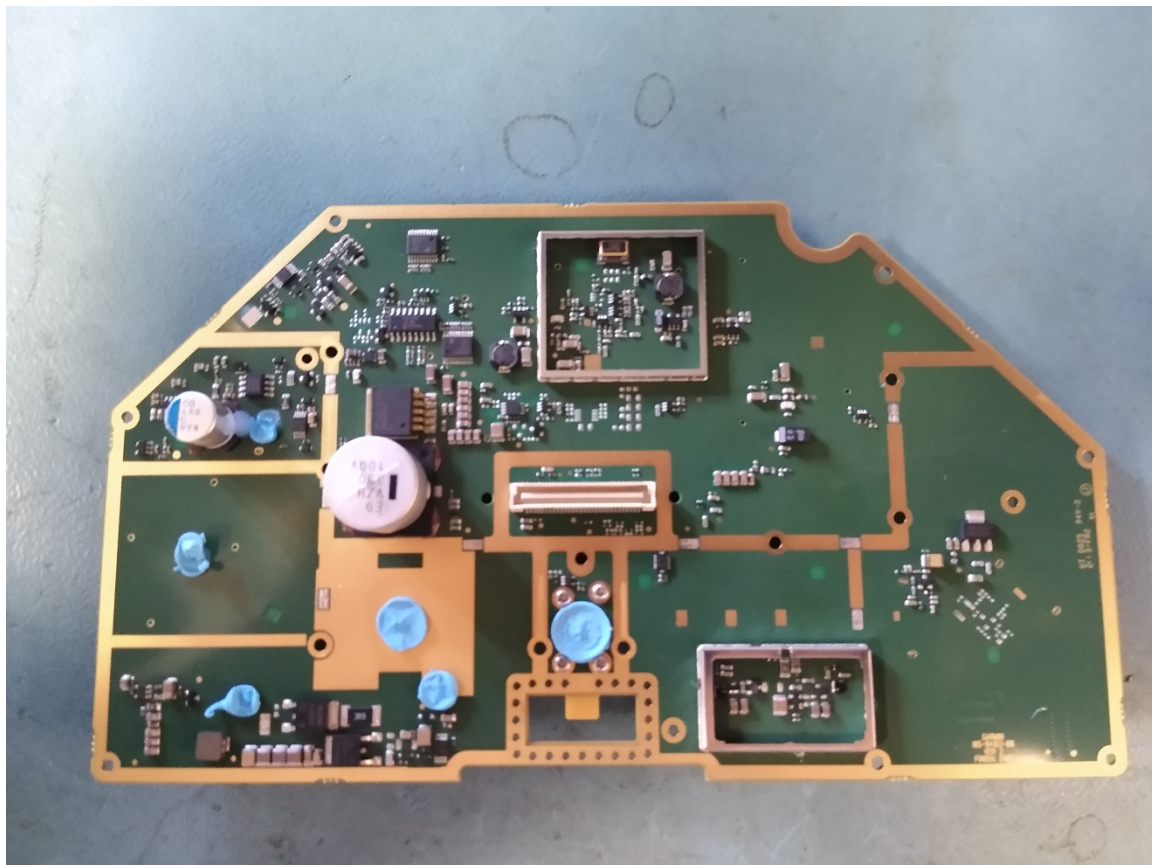
PCB 2- Side 2, without Shields
