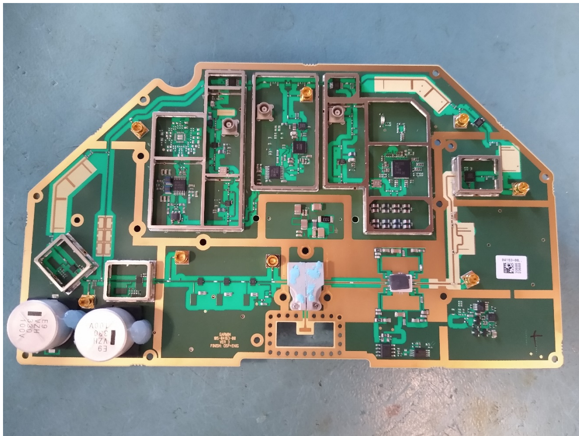
PCB 2 – Side 1, without Shields
