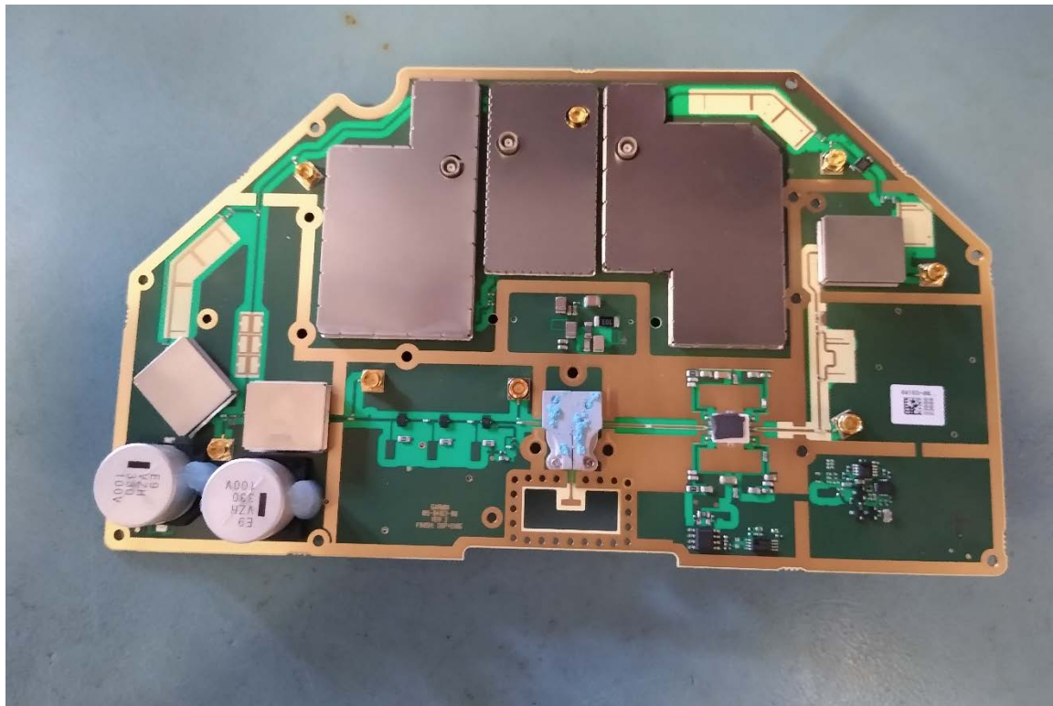
PCB 2 – Side 1, with Shields
