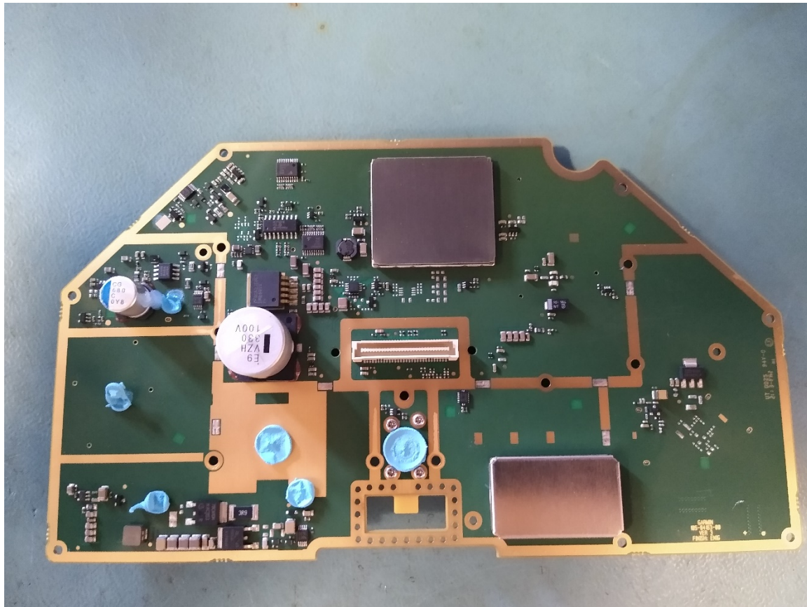
PCB2 – Side 2, with Shields
