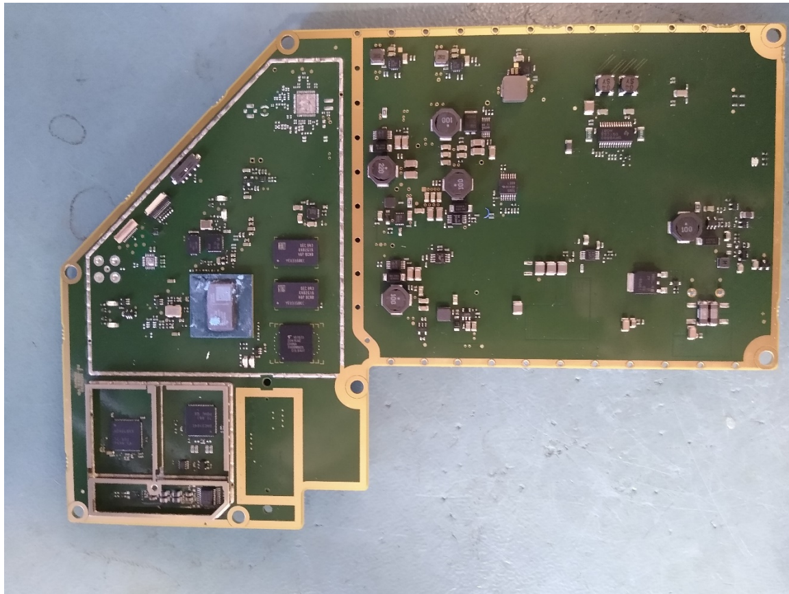
PCB 1 – Side 2, without Shields
