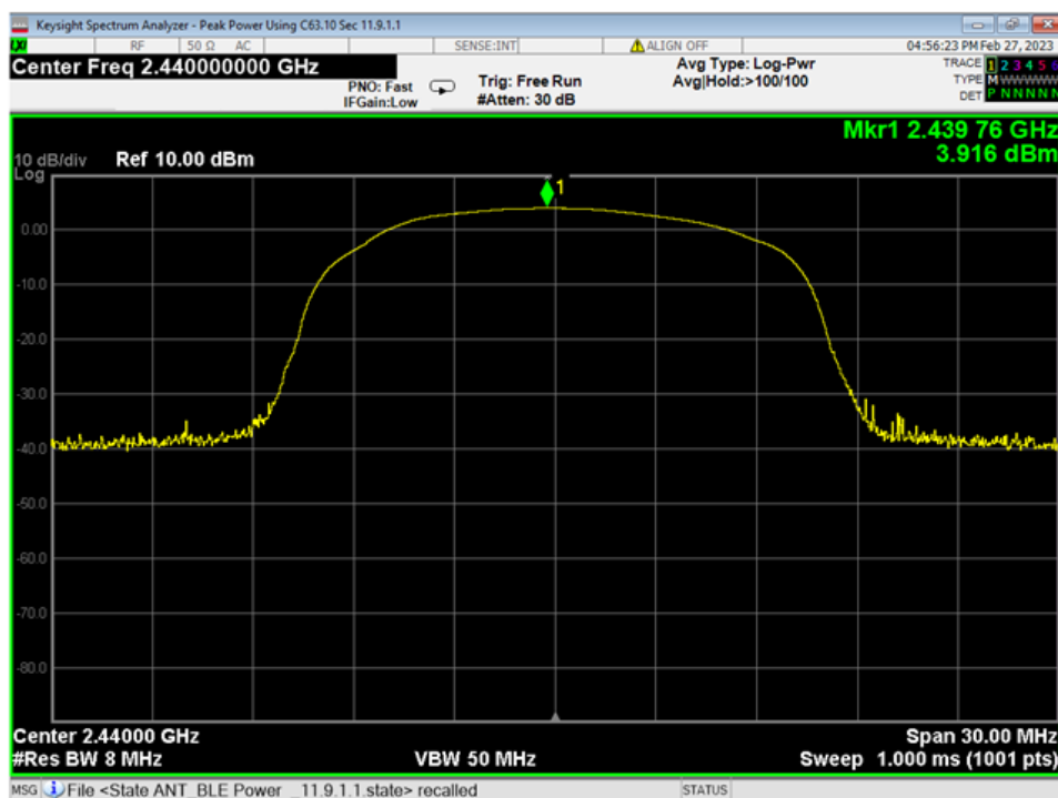
15 Peak Power, Mid Channel, GMSK 2MB
