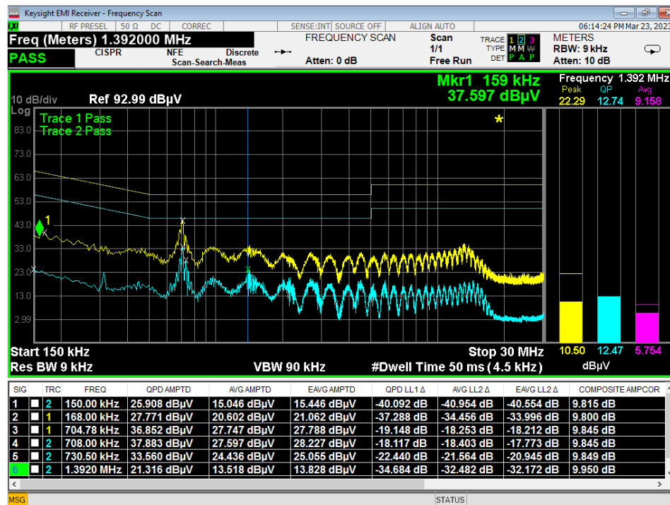
Figure 19 - Conducted Emissions Plot, Neutral, IDLE
