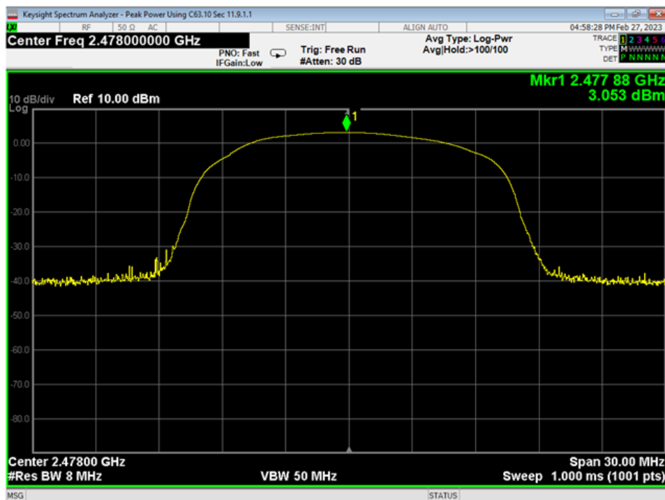
16 Peak Power, High Channel, GMSK 2MB
