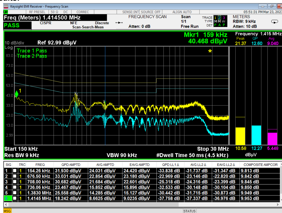
Figure 16 - Conducted Emissions Plot, Line, TX
