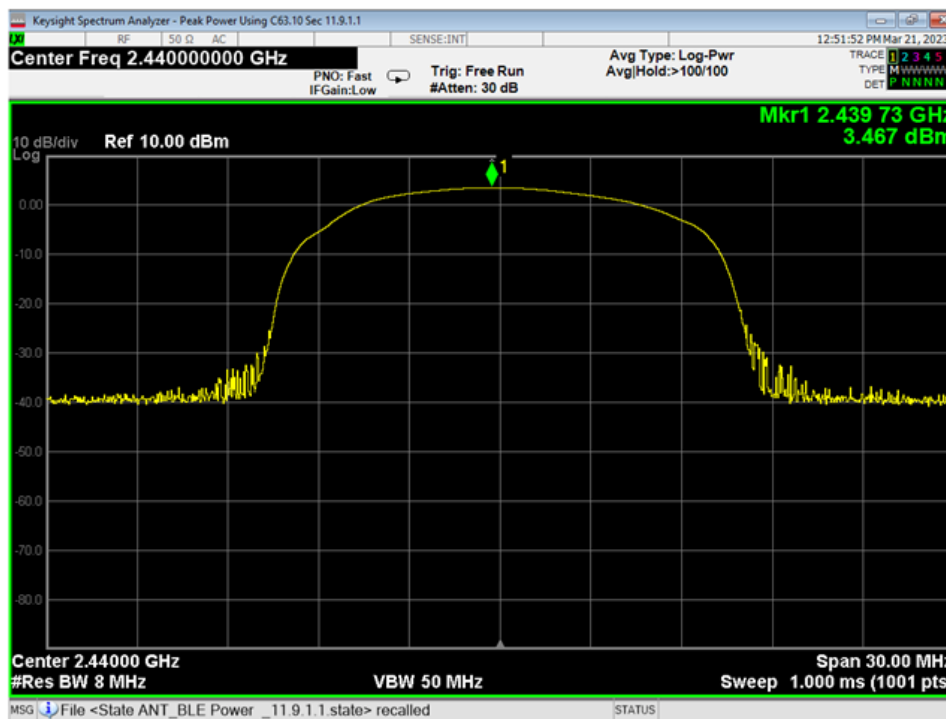
02 Peak Power, Mid Channel, GMSK 1MB
