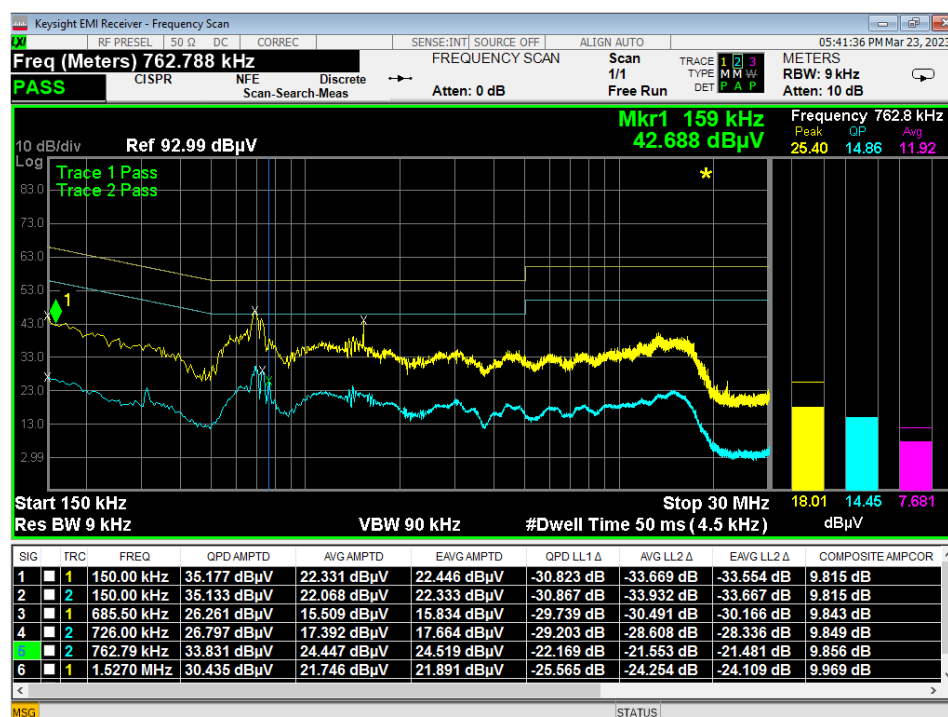
Figure 17 - Conducted Emissions Plot, Neutral, TX
