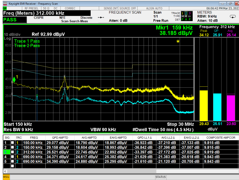
Figure 18 - Conducted Emissions Plot, Line, IDLE
