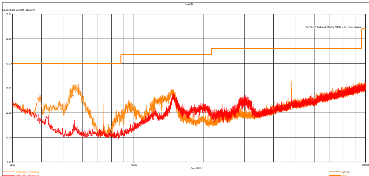
Figure 21 - Radiated Emissions Plot, Low Channel
