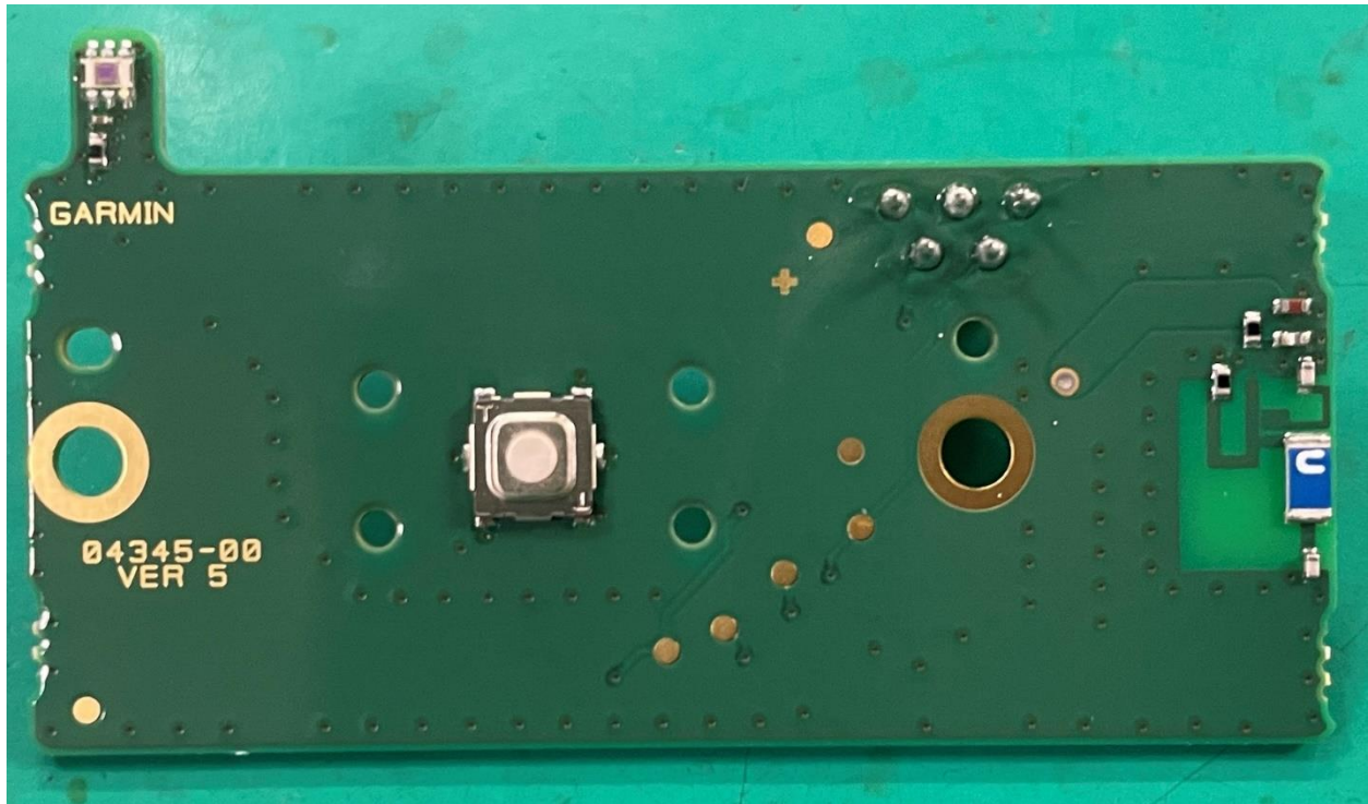
Photograph 6-5 : Front side view of the button board
