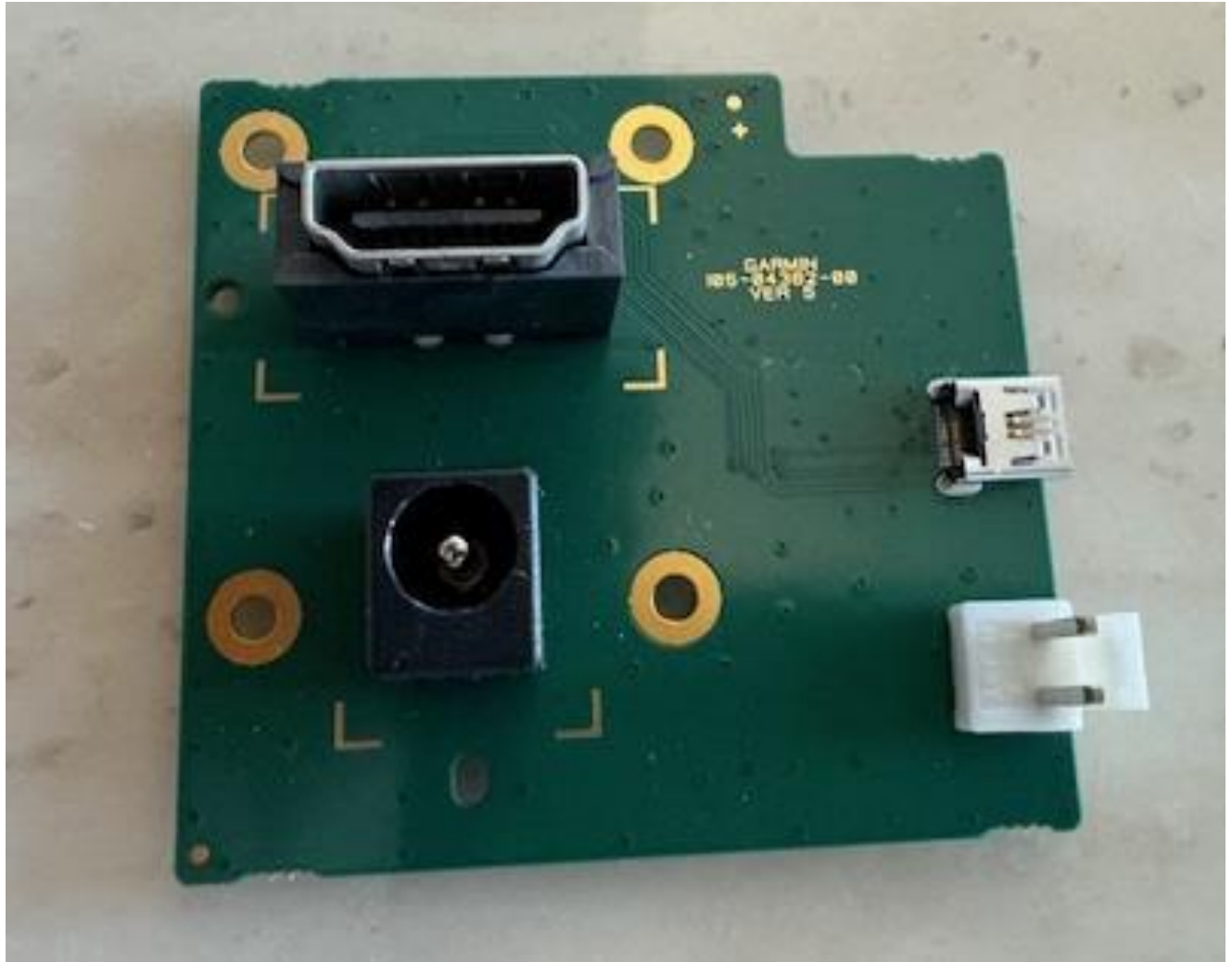
Photograph 6-15 : Front side view of the HDMI Power board
