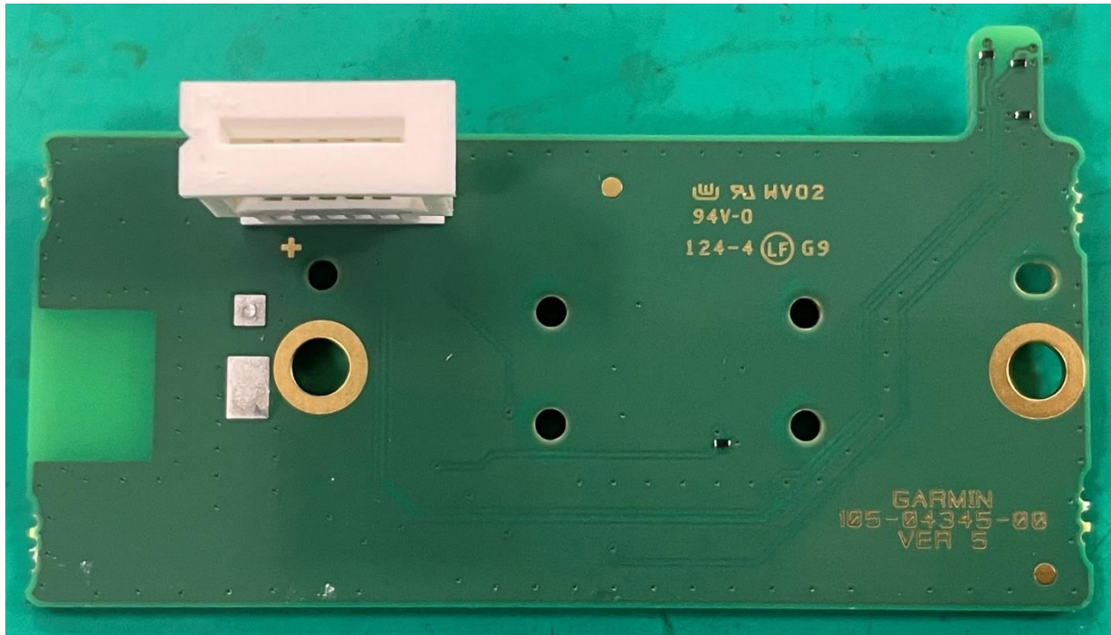
Photograph 6-6 : Back side view of the button board
