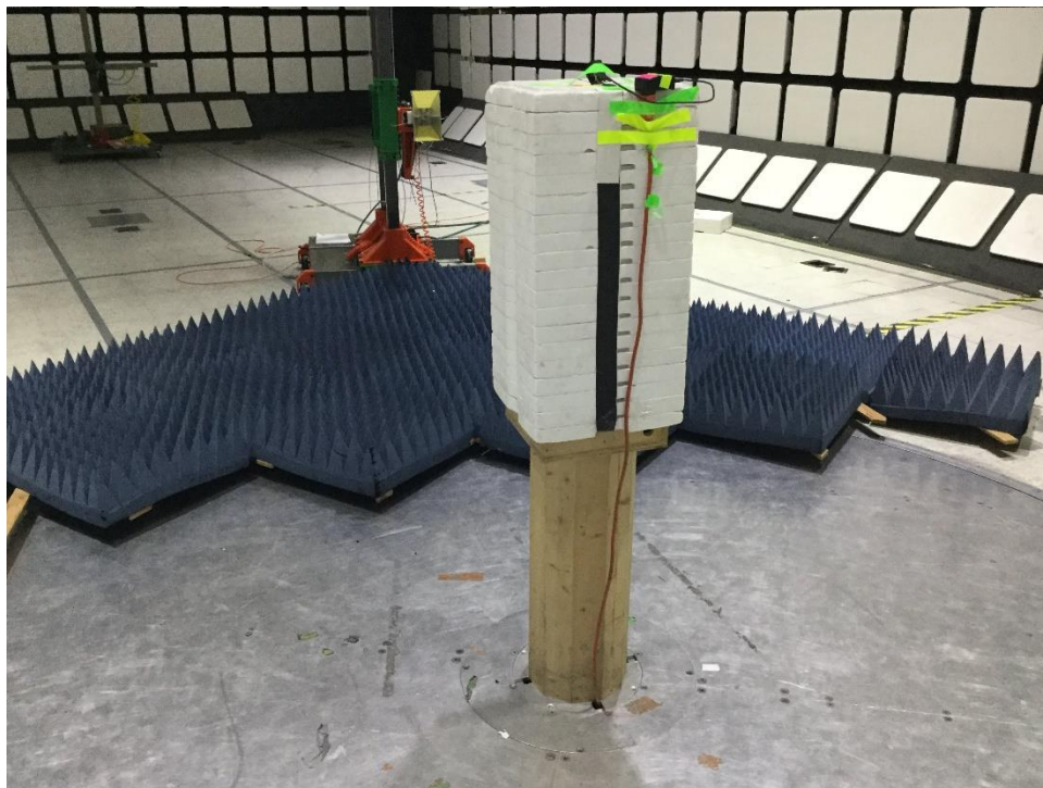
1 – 26 GHz Test Setup
