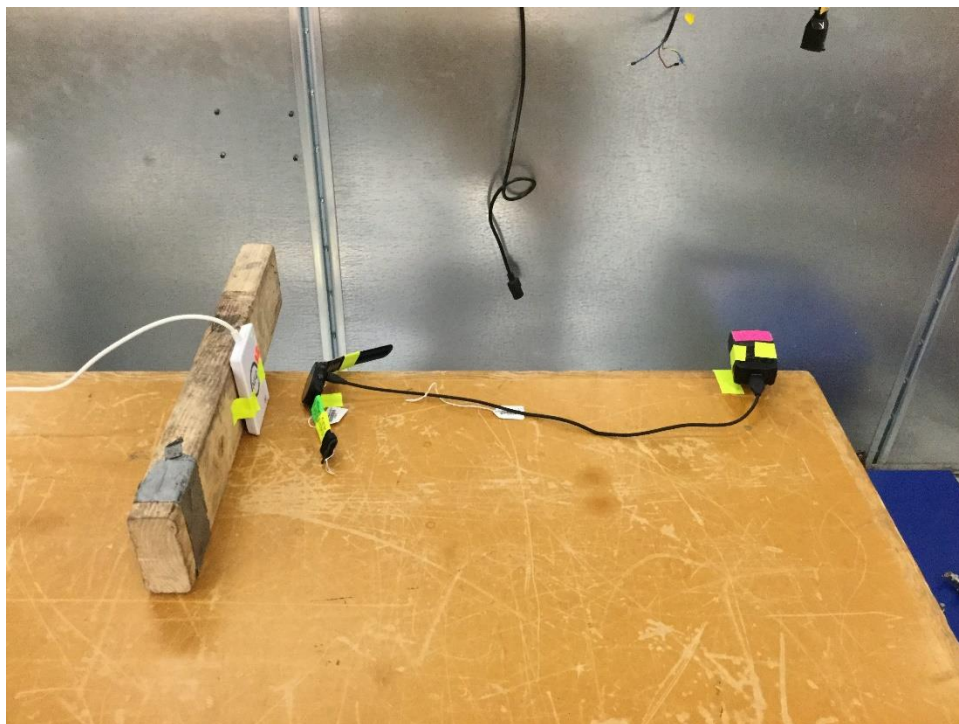
Conducted emissions test setup, NFC
