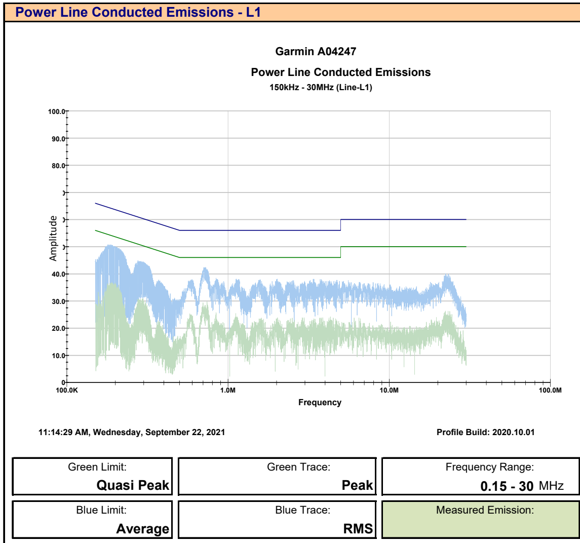
Plot 16.1 – Power Line Conducted Emissions, Line 1
