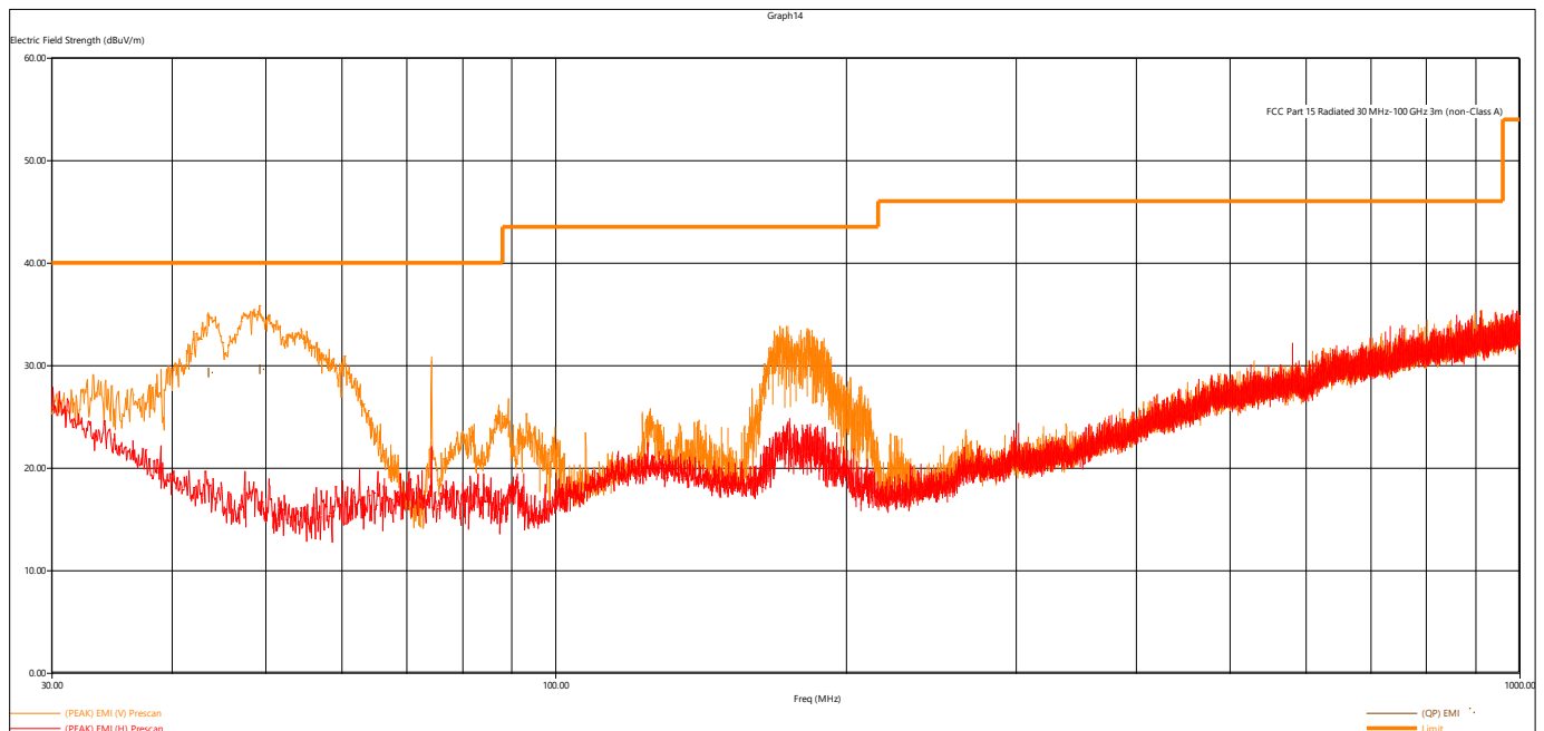
Figure 7 - Radiated Emissions Plot, BT EDR 2MB
