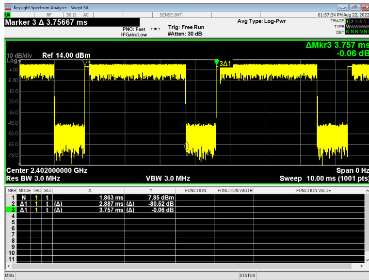
Figure 3 –Duty Cycle, 2EDR
