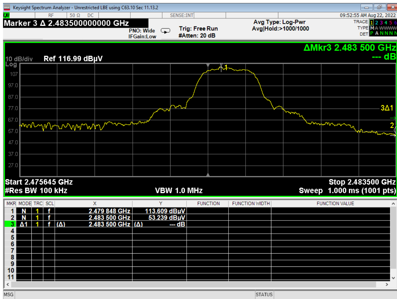
24 Higher Bandedge, Unrestricted, 3EDR
