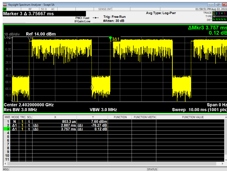
Figure 4 –Duty Cycle, 3EDR
