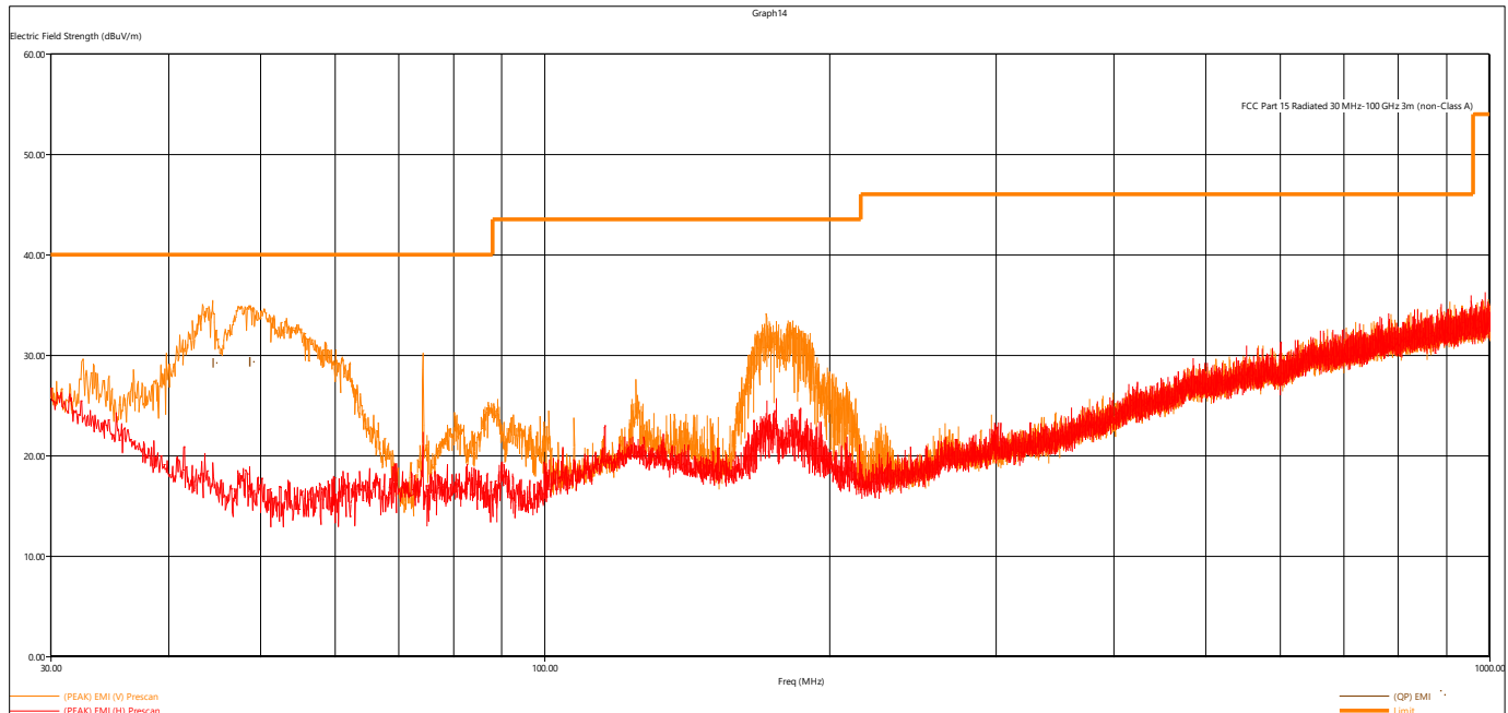
Figure 8 - Radiated Emissions Plot, BT EDR 3MB
